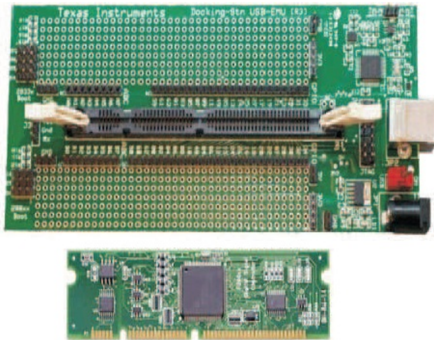
Figure 3.1. F2808 experimner kit from Texas Instruments [1].
