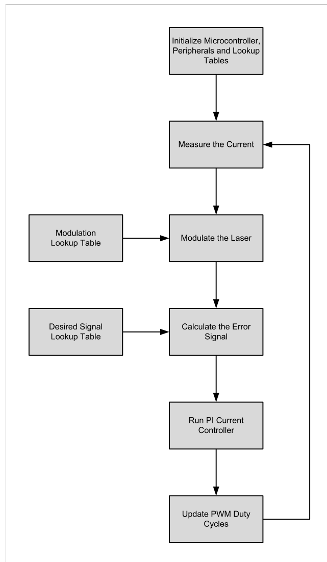
Figure 3.4. Firmware program flow block diagram.
