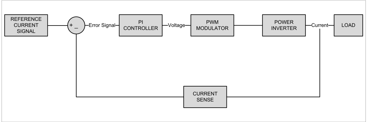
Figure 2.2. Closed loop current control block diagram.
