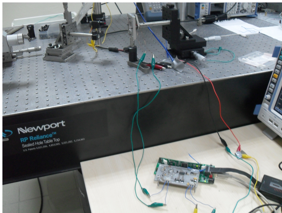
Figure 4.2. Experimental setup.
