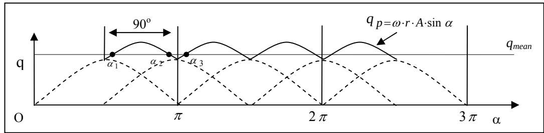
Figure 38 Flow Rate Diagram of Quad Pump
