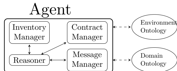
Figure 3.3. Architecture of an agent.
