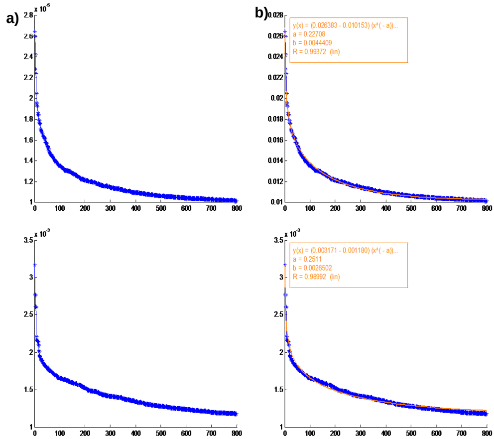
Figure 3.7: a) LPC error curves with increasing order, b) \exp(x)*1/x fitted to LPC error curve and related fit function characteristics mentioned on the right
