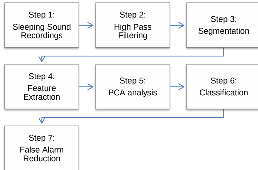
Figure 4.1: Flow of the algorithm
