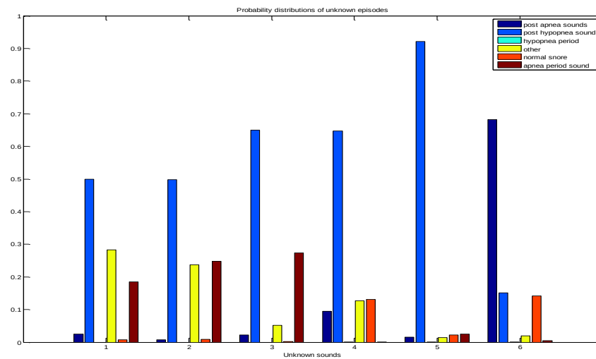
Figure 4.15:Probability values for unknown episodes
