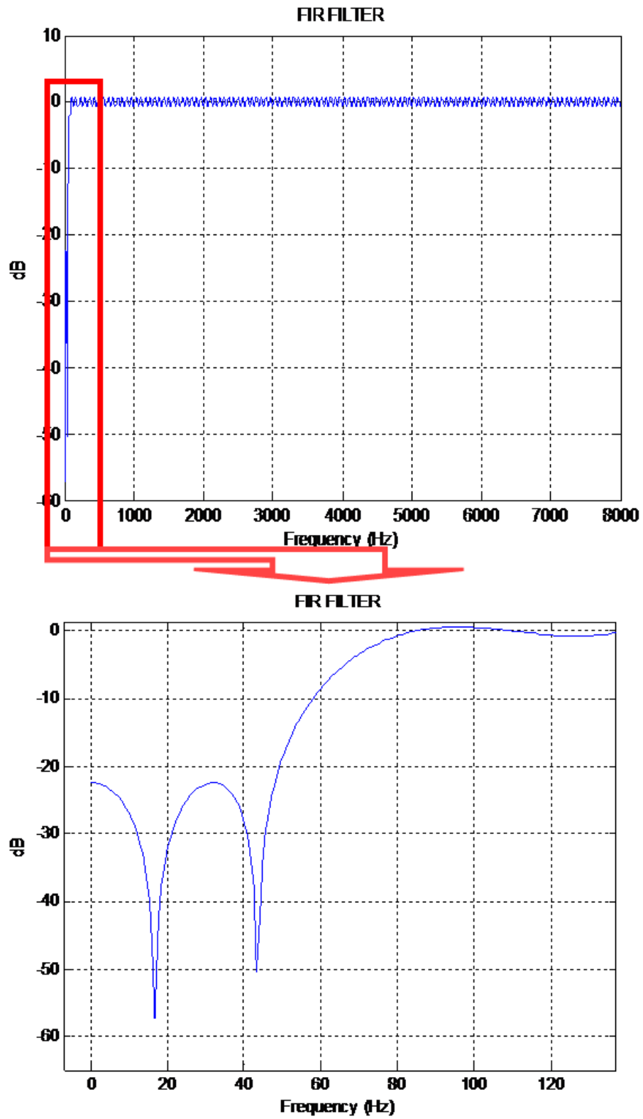
Figure 4.2: Frequency characteristic of FIR filter
