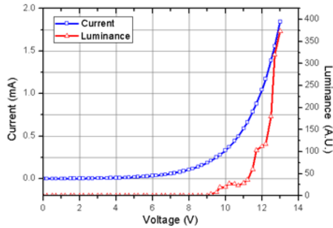
Figure 3.30. Luminance–current–voltage (L–I–V )characteristic of the fabricated PLEDs.
