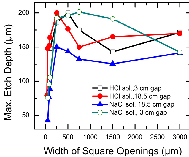
Figure 4.15. Etch depth as a function of square opening widths for different electrode gaps at a current density of 3\ \text{A}/\text{cm}^2 and for an etch time of 5 min.
