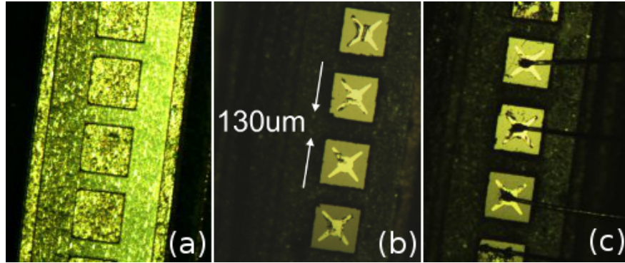
Figure 3.13. Integration steps of LED dies on FR4 actuator. (a) SU8 trenches of 300 \times 300\text{ }\mu\text{m} for LED placement. (b) LED placement with 130\text{ }\mu\text{m} gap in between them. (c) LEDs wirebonded to Cu pads.
