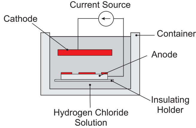
Figure 4.14. Electrochemical etch setup used in the proposed process.
