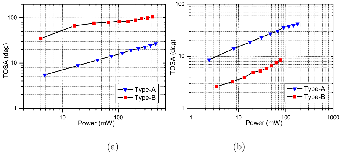
Figure 4.9. Drive power versus total optical scan angle (TOSA) relationship for the cantilever type gimballed (Type-A) scanner and the torsional type gimballed (Type-B) scanner (a) Slow scan characteristics (b) Fast scan characteristics.
