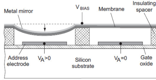
Figure 1.4. Simplified view of the cross-section of DMD. After [13].
