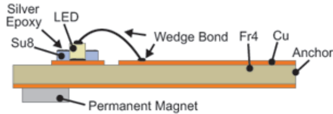
Figure 3.12. Fabrication profile of solid-state LED integrated FR4 Scanners.
