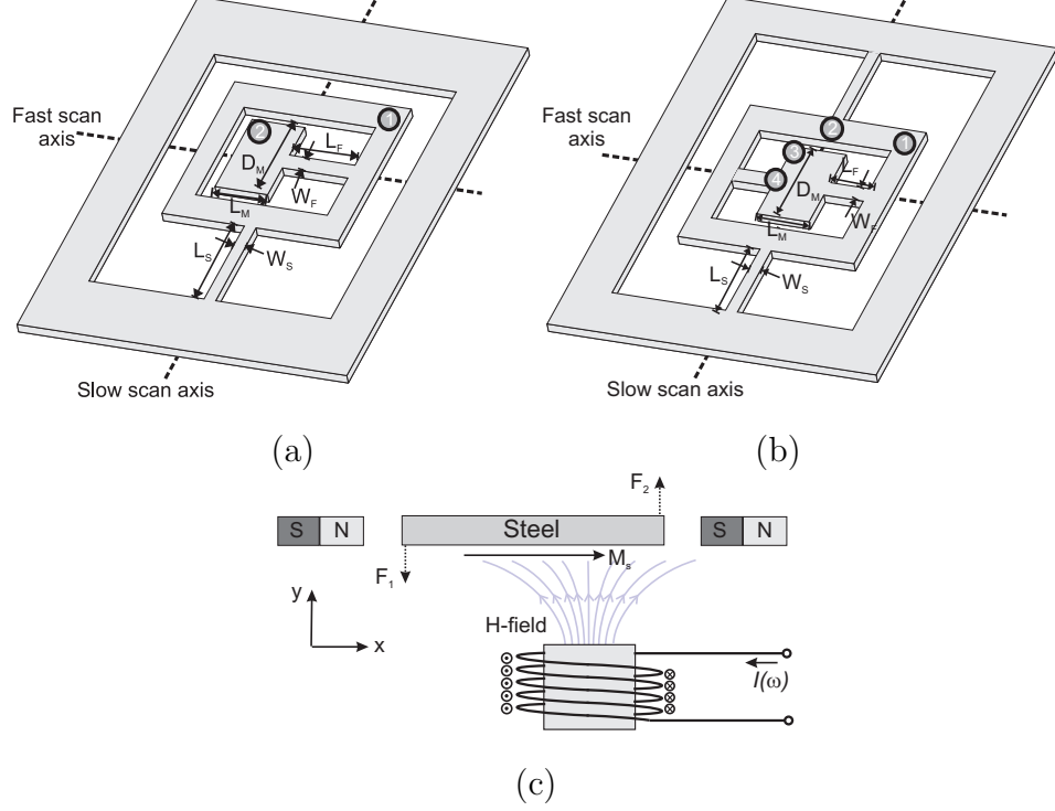
Figure 4.1. Schematics and operation of the 2D scanner devices. (a) Gimballed cantilever scanner (Type-A) (b) Gimballed torsional scanner (Type-B) (c) Magnetic actuation scheme used for both types of the devices.
