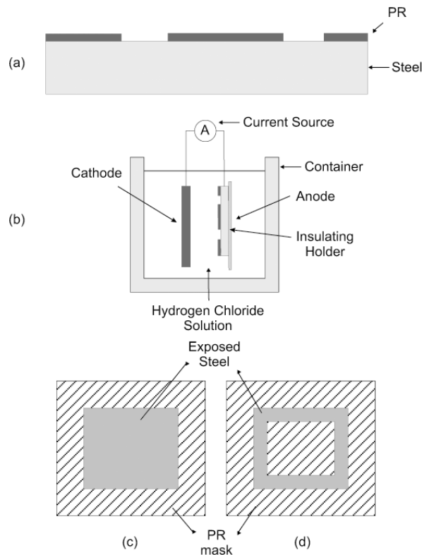
Figure 4.4. (a) 100\ \mu\text{m} thick SS301, spin coated and patterned with 6\ \mu\text{m} PR mould (b) Schematics of the electrochemical cell (c) Standard electrochemical etching mask (d) Electrochemical etching mask maximizing the current density.
