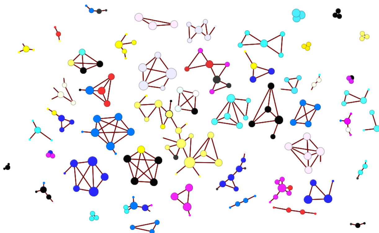
Figure 6.32: Collaborators: 2002-2008
