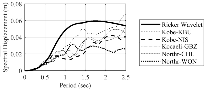
Figure 3.10 Comparison of displacement response spectra
