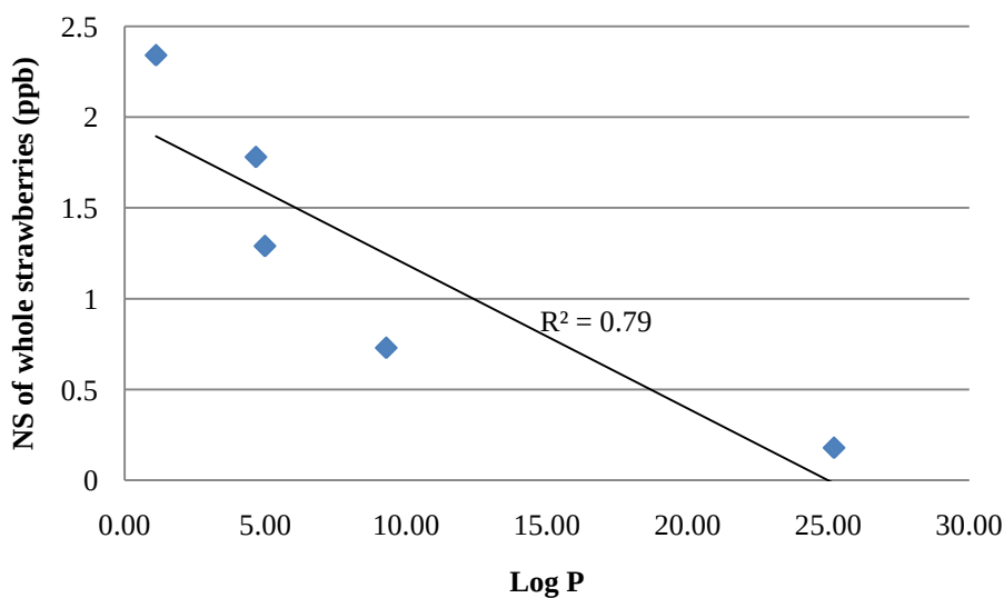
Figure 17. Relationship between Log P values and nosespace (NS) concentrations of selected volatiles of whole strawberries
