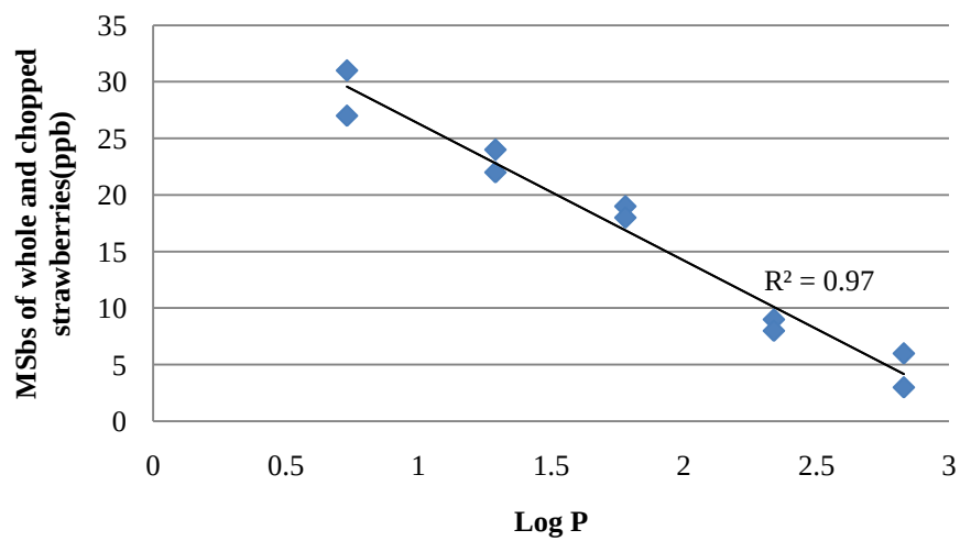
Figure 10. Relationship between Log P values and mouthspace (MSBs) concentrations of selected volatiles of whole and chopped strawberries
