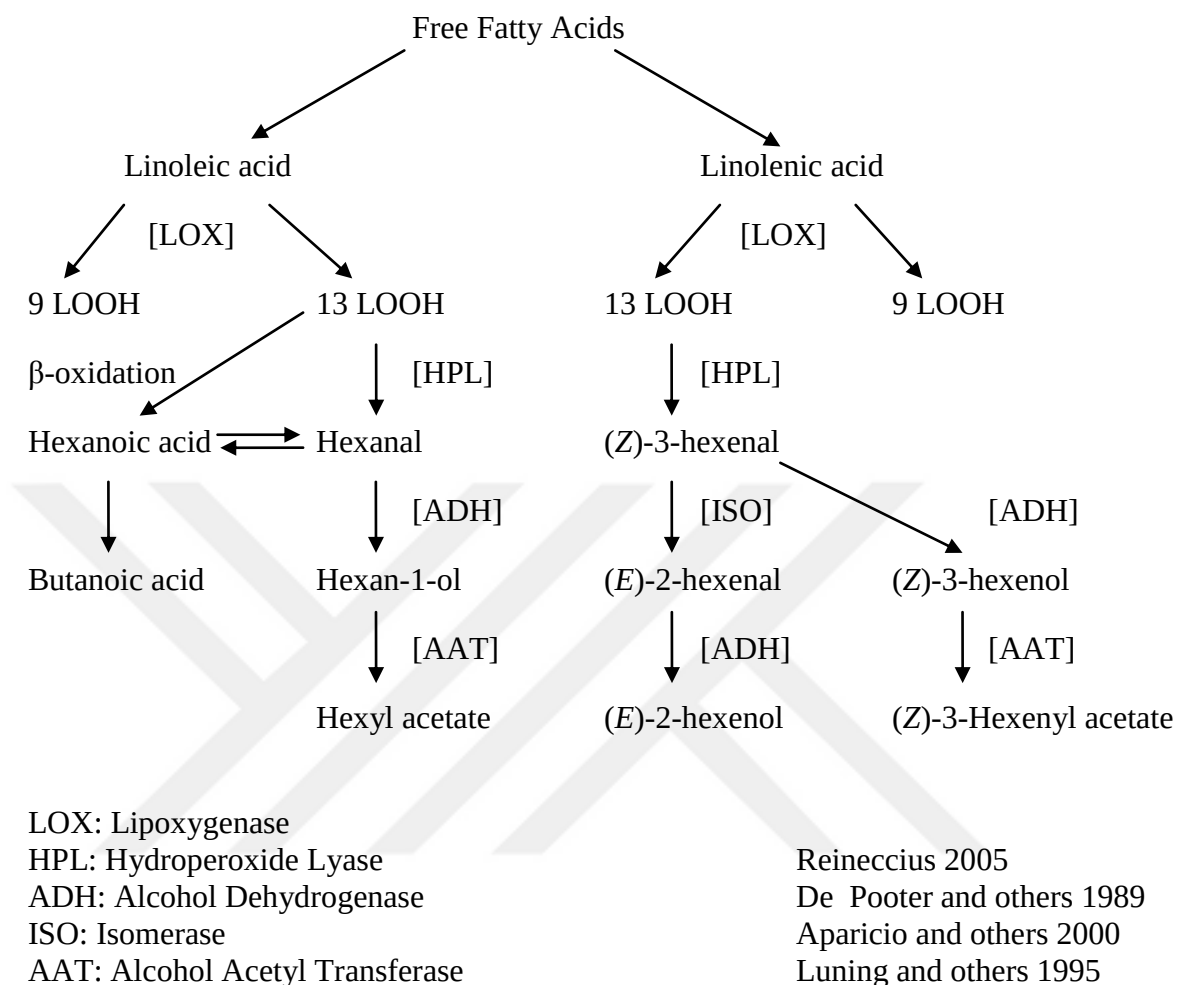
Figure 2 Volatile organic compound formation by lipoxygenase pathway
