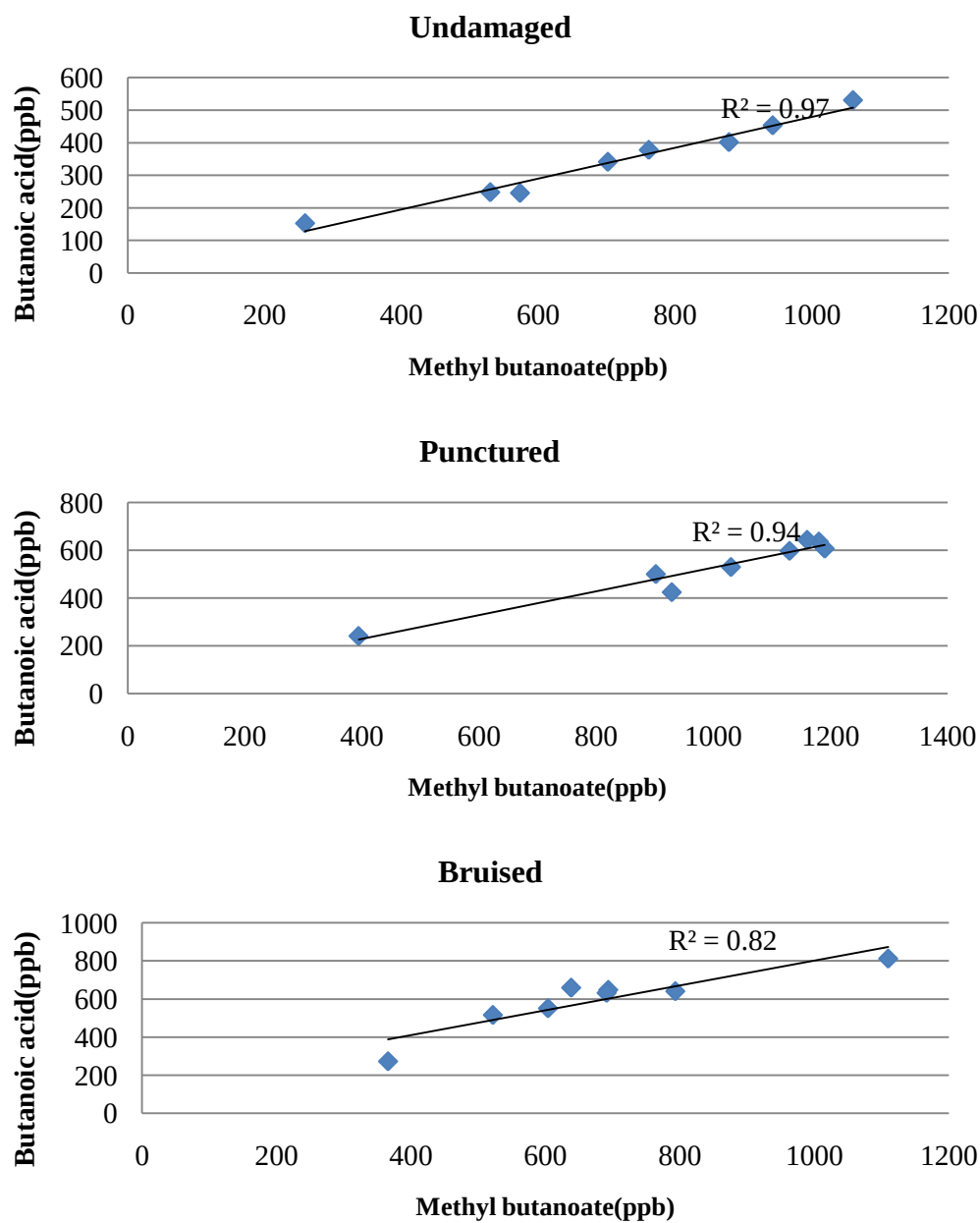
Figure 15. Correlation of butanoic acid and methyl butanoate
