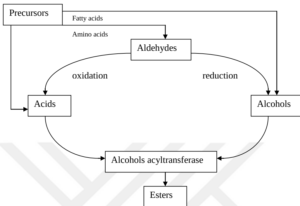
Figure 3. Biological pathway of volatile ester formation (Figure modified from Olias and others 1995)
