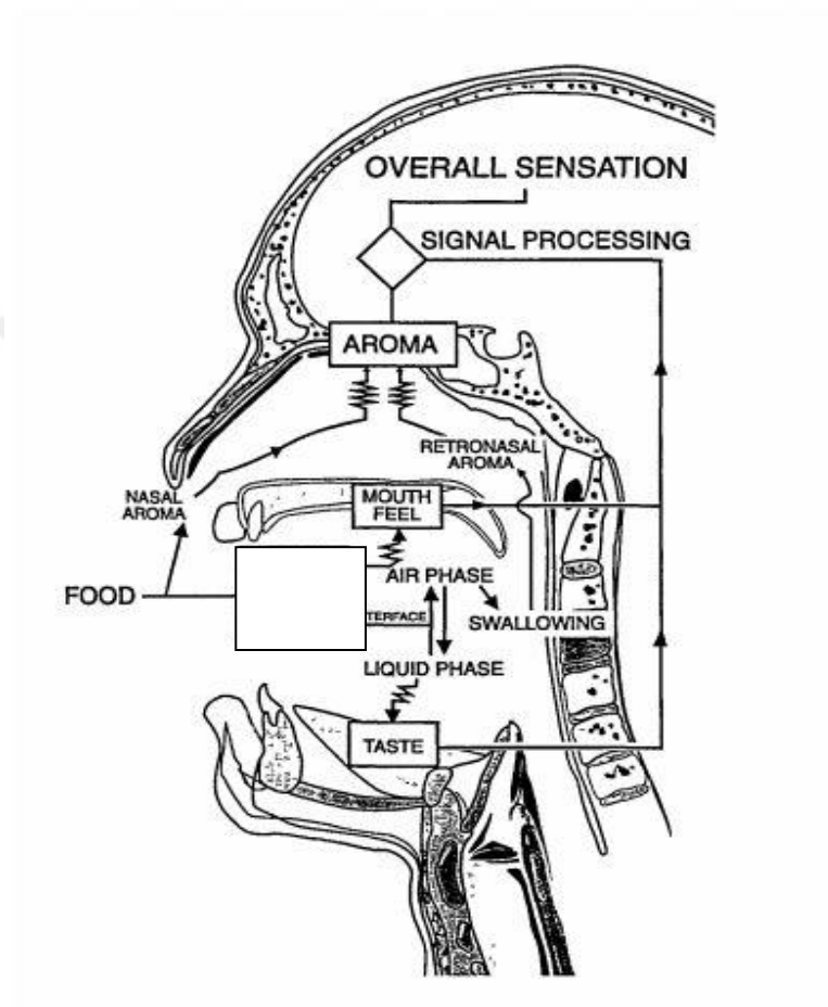
Figure 1 Flavor stimulation and perception locations in the brain (Figure modified from Taylor 1996)
