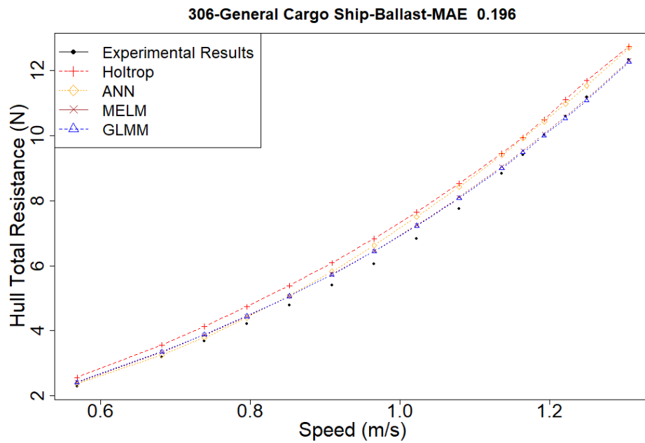
Figure D.12. Resistance Estimation of Model No: 306, General Cargo Ship, Loading Condition: Ballast
