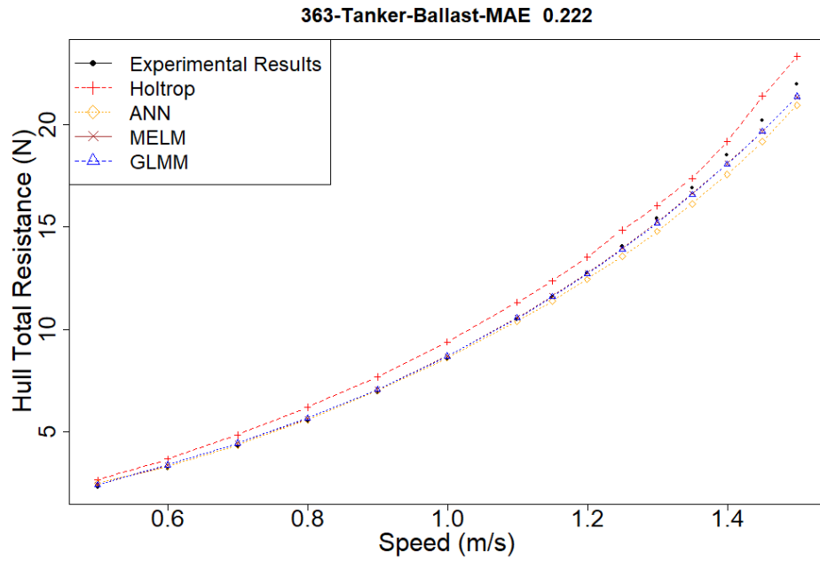
Figure 6.9. Resistance Estimation of Model No: 363, Tanker, Loading Condition: Ballast
