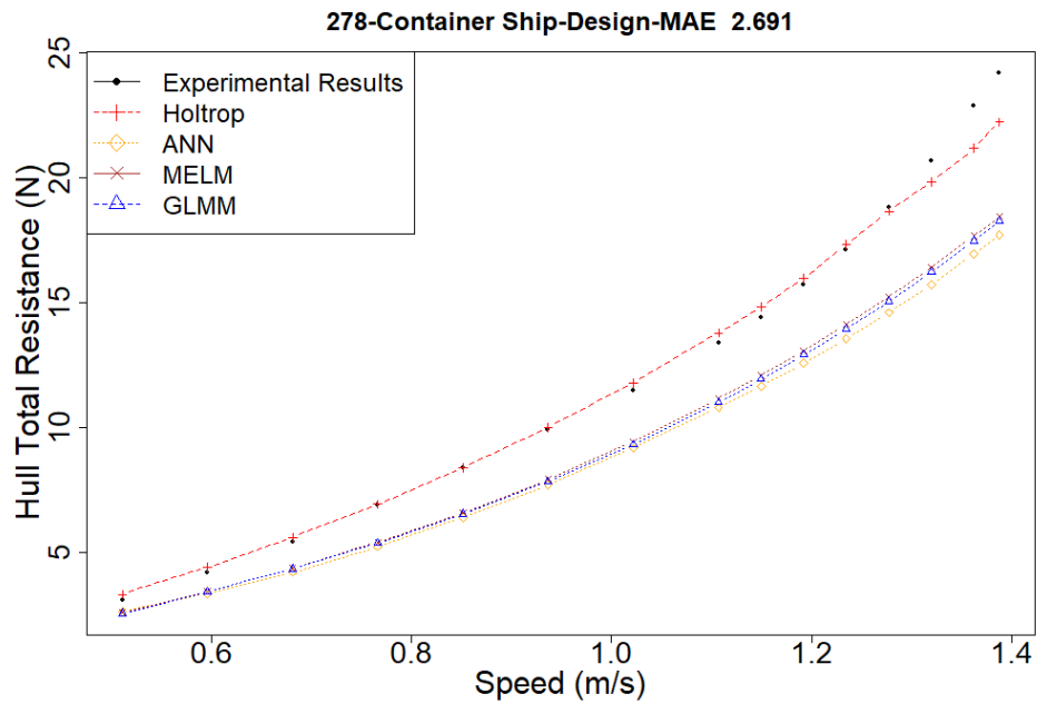
Figure 6.10. Resistance Estimation of Model No: 278, Container Ship, Loading Condition: Design
