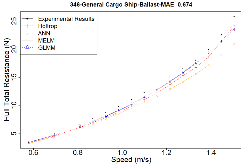
Figure D.24. Resistance Estimation of Model No: 346, General Cargo Ship, Loading Condition: Ballast
