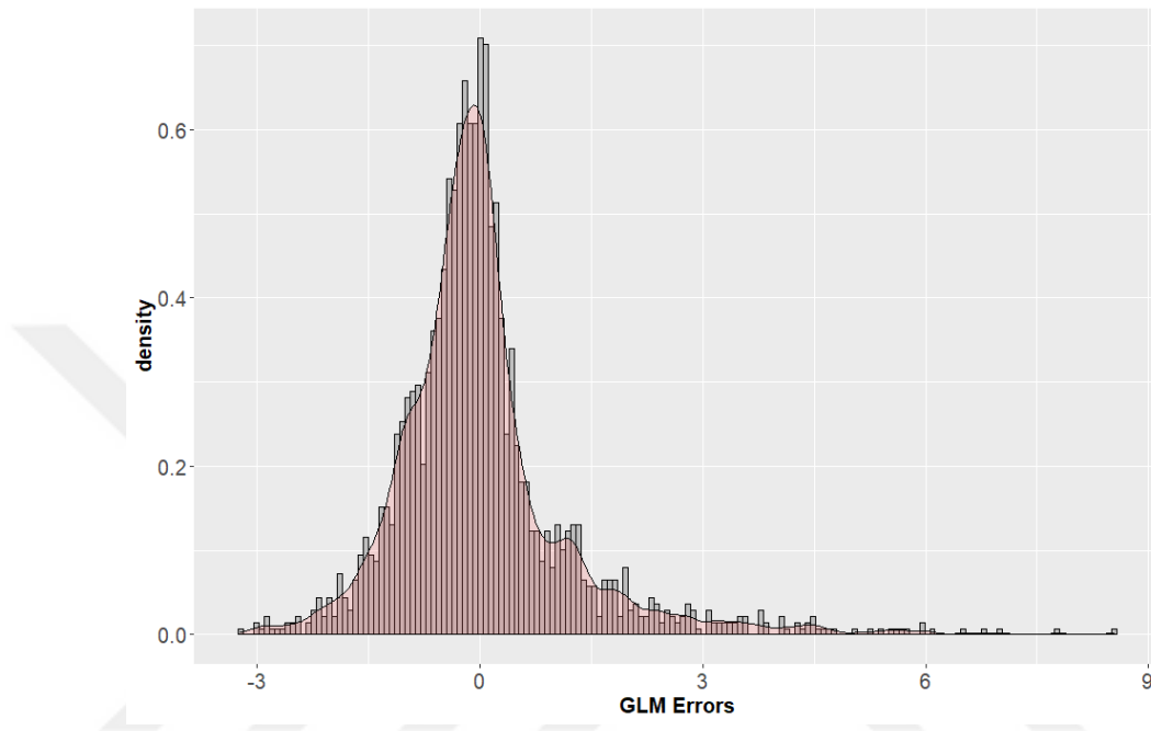
Figure D.1. Histogram of GLM errors
