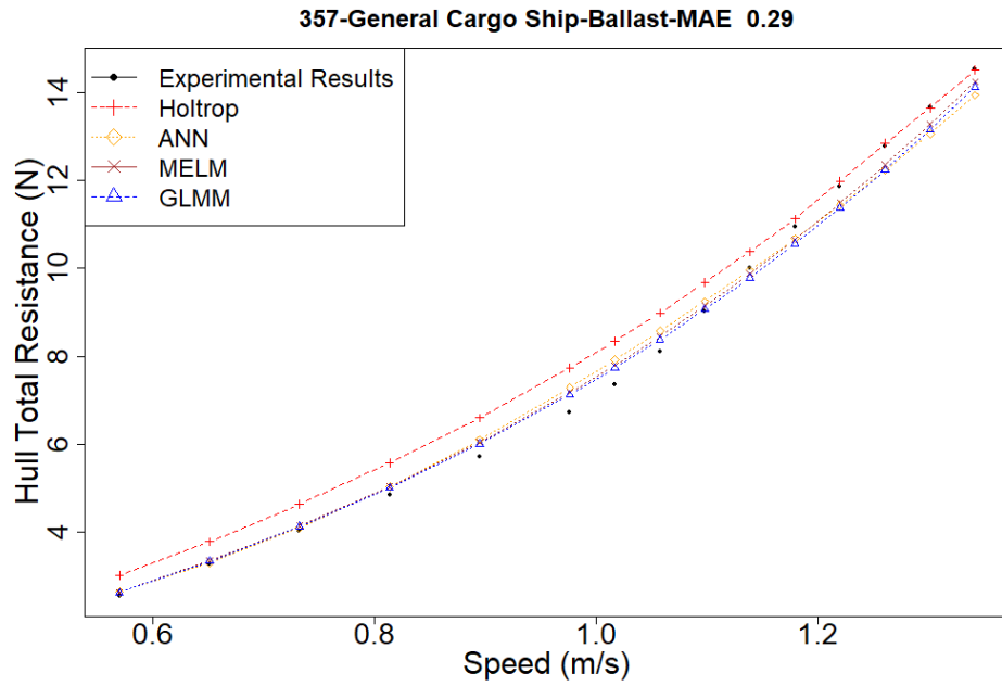
Figure D.28. Resistance Estimation of Model No: 357, General Cargo Ship, Loading Condition: Ballast
