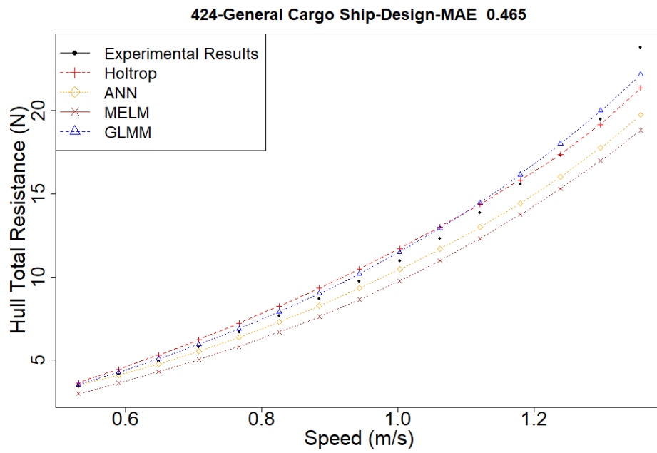
Figure D.38. Resistance Estimation of Model No: 424, General Cargo Ship, Loading Condition: Design
