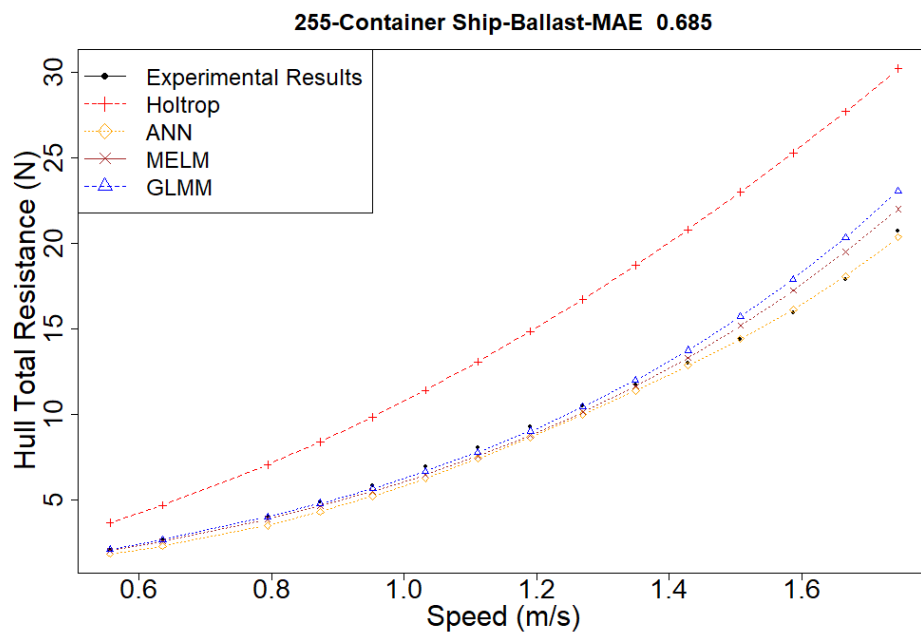
Figure D.39. Resistance Estimation of Model No: 255, Container Ship, Loading Condition: Ballast
