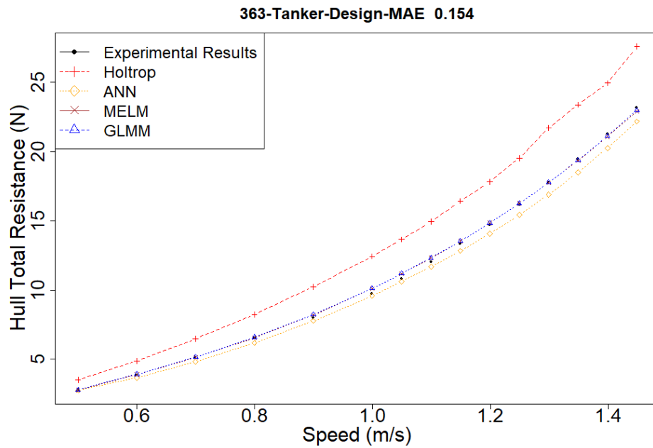
Figure 6.8. Resistance Estimation of Model No: 363, Tanker, Loading Condition: Design
