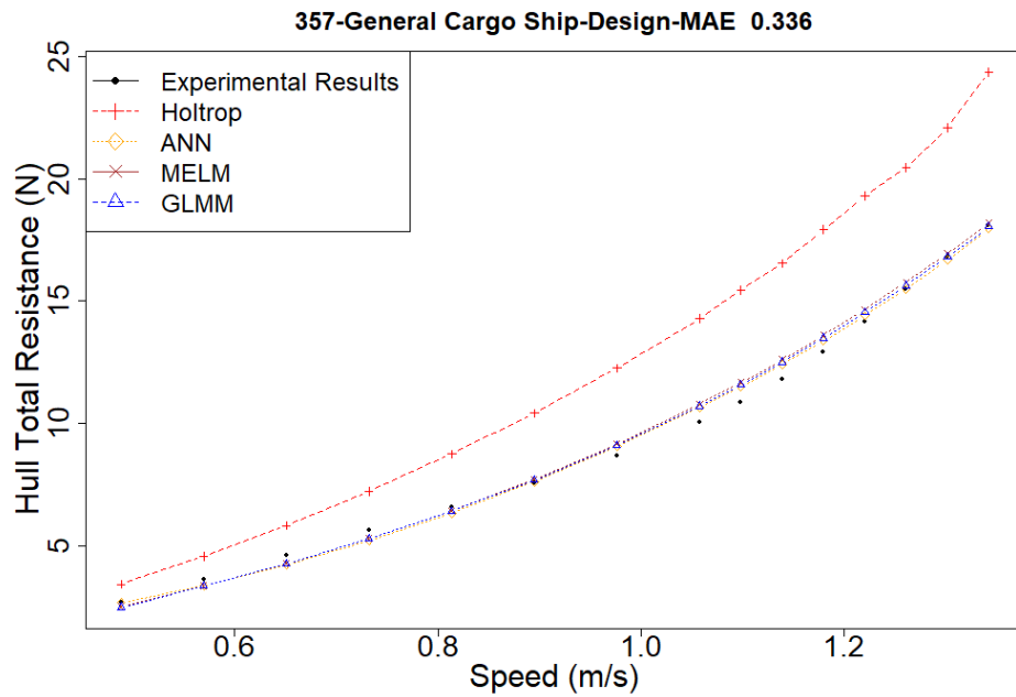
Figure D.29. Resistance Estimation of Model No: 357, General Cargo Ship, Loading Condition: Design
