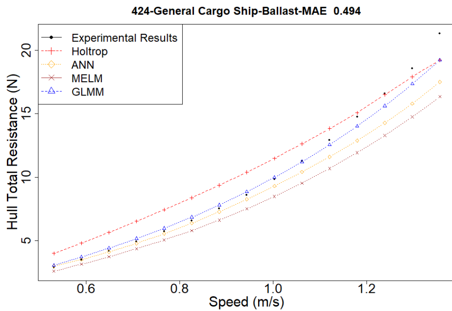
Figure D.37. Resistance Estimation of Model No: 424, General Cargo Ship, Loading Condition: Ballast
