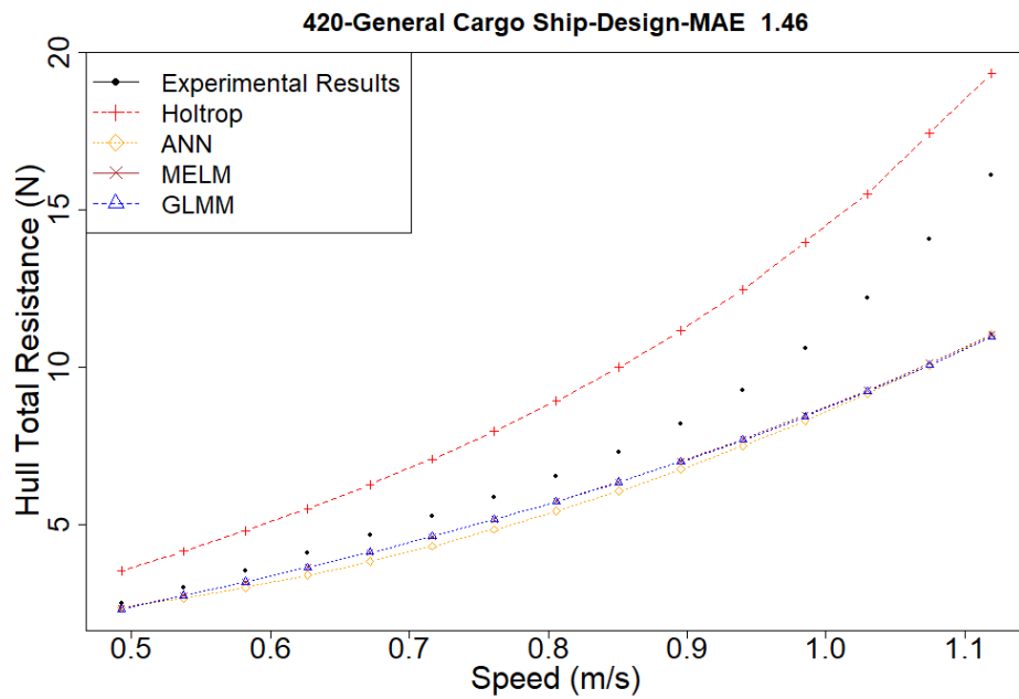
Figure D.36. Resistance Estimation of Model No: 420, General Cargo Ship, Loading Condition: Design
