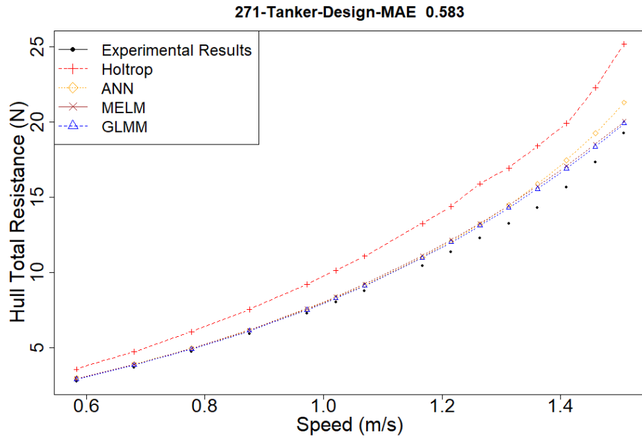
Figure D.54. Resistance Estimation of Model No: 271, Tanker, Loading Condition: Design
