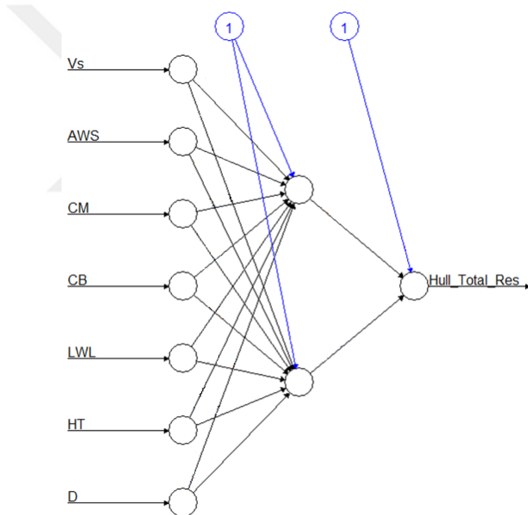
Figure 5.6. Final ANN model
