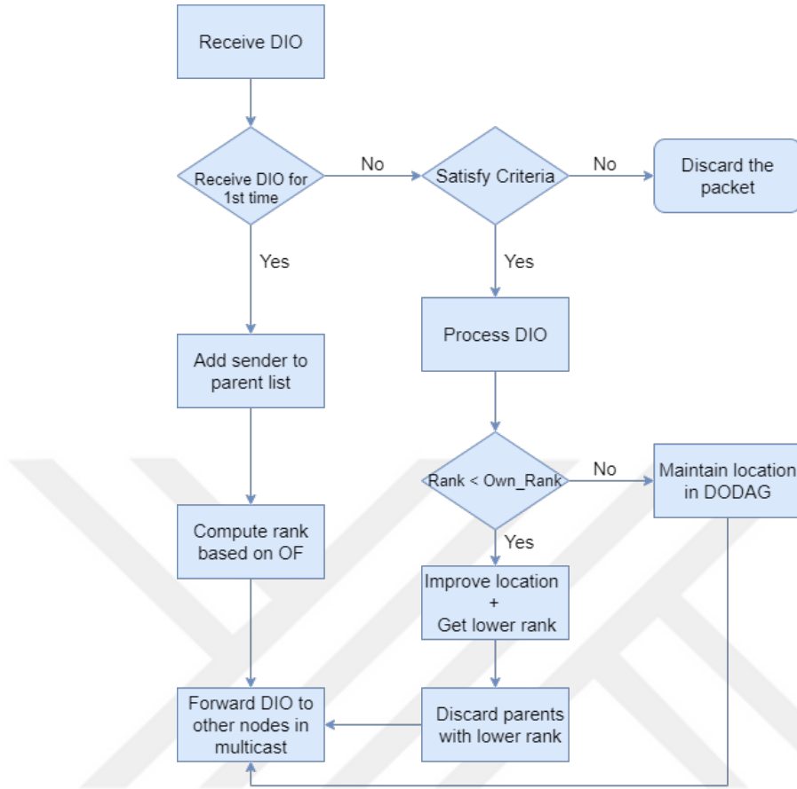
Figure 2.2. Operation of a node in DODAG
