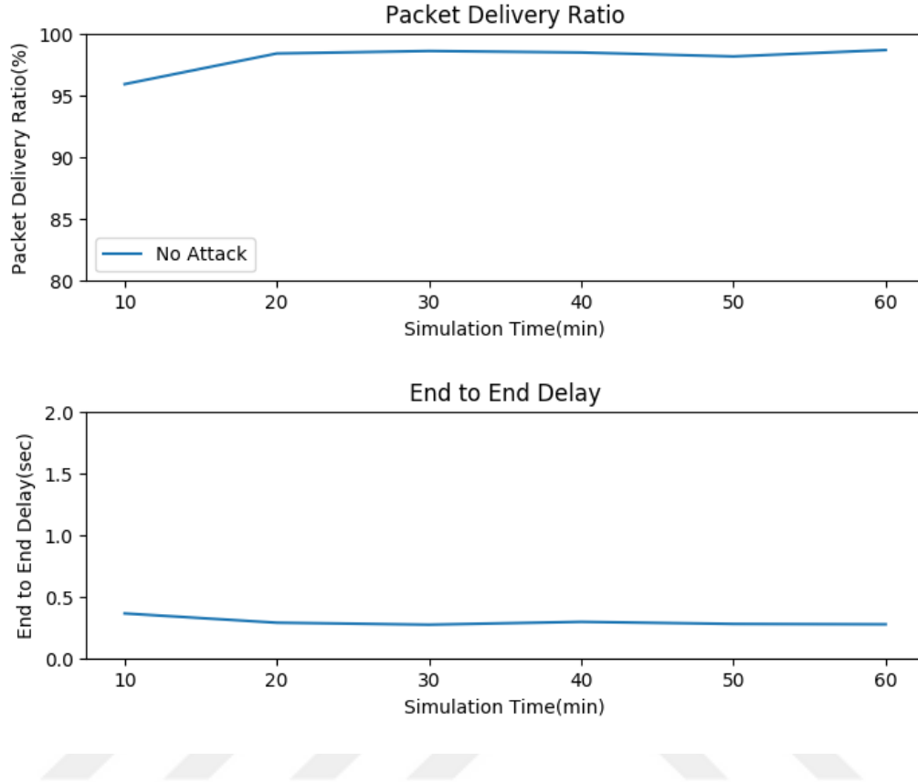
Figure 5.2. PDR and E2E delay metrics of network without attack
