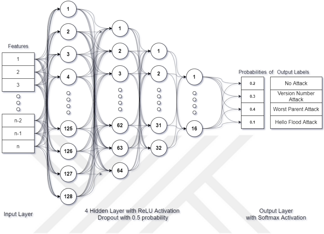
Figure 4.1. Proposed neural network architecture
