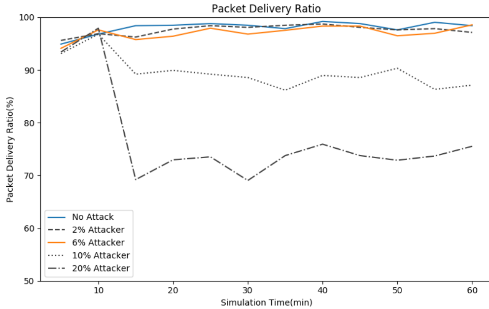
Figure 5.7. PDR for Worst Parent Attack
