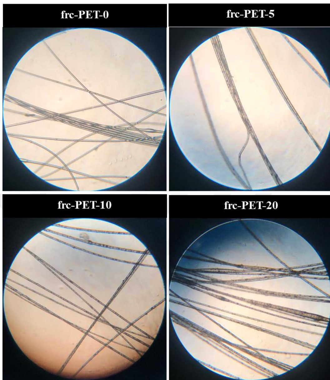
Figure 4.13 Longitudinal views of frc-PET fibers
