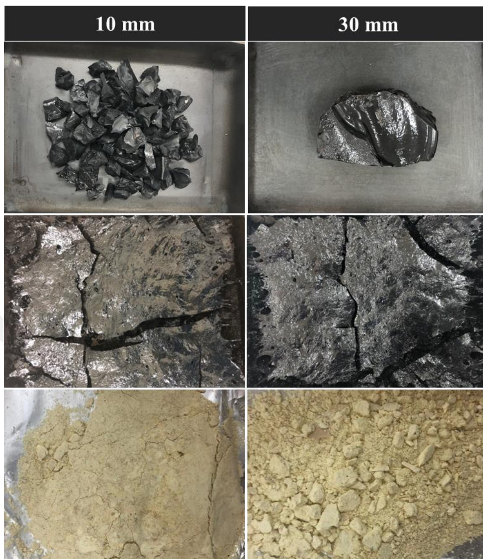
Figure 3.13 Carbonized materials and chemicals obtained from the carbonization of 10 mm and 30 mm d -PET
