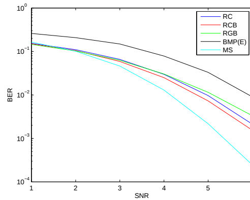
Figure 6-20: The performance of RC, RCB, RGB, MS, and BMP-E on AWGN+EC with p_1 = 0.1 with (96,48) LDPC code
