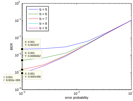
Figure 6-11: BER performance of the complete EED with different separation bounds on BSEEC with p_1 = 0.1 using (15,6,5) LDPC code
