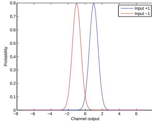
Figure 2-4: The probability distribution of AWGN channel output
