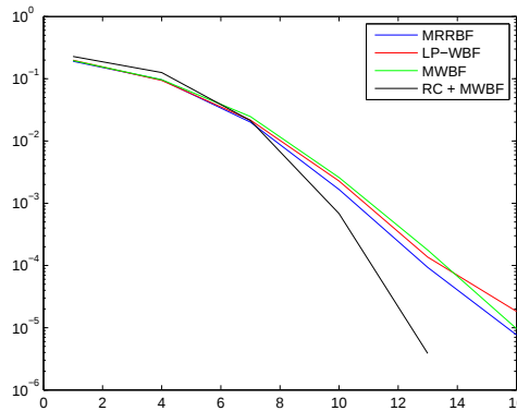
Figure 6-23: The performance of MRRBF, LP-WBF, MWBF, and MWBF+RC (ED) on AWGN channel with Rayleigh fading using (n = 96, k = 48, d_c = 3) LDPC code
