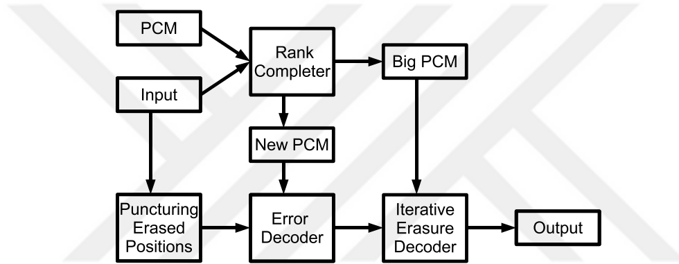
Figure 6-14: Block diagram for the complete EED with stopping set prevention
