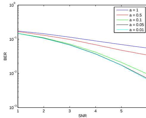
Figure 6-5: The BER performance comparison of RG with different a values on AWGN+EC with p_1 = 0.1
