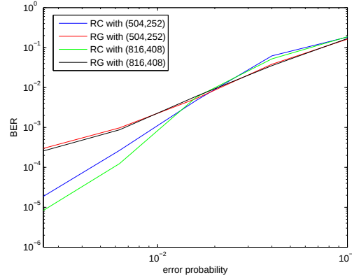
Figure 6-18: The performance of RC and RG on BSEEC with p_1 = 0.1 with (504,252) and (816,408) LDPC codes
