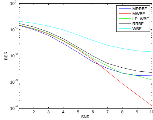
Figure 6-6: The BER performance comparison of RG with different decoders using (96,48,3) on AWGN+EC with p_1 = 0.1
