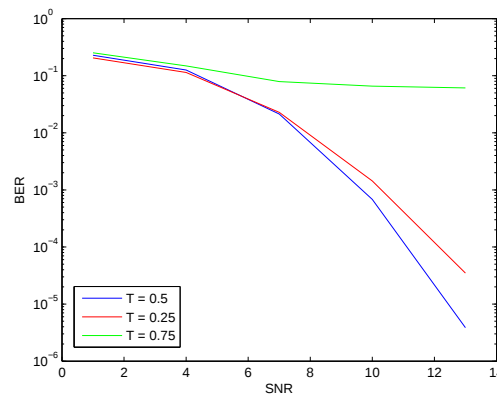
Figure 6-25: The performance of MWBF+RC (ED) on AWGN channel with Rayleigh fading using (n = 96, k = 48, d_c = 3) LDPC code with different T values
