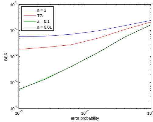
Figure 6-3: The BER performance comparison of RG, simple guessing, and trial guessing for (204,102) code on BSEEC with p_1 = 0.1
