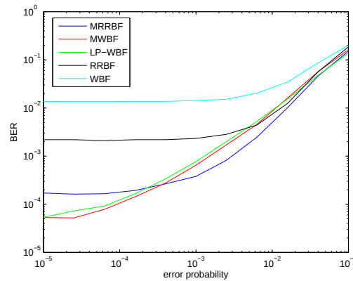
Figure 6-4: The BER performance comparison of RG with different decoders on BSEEC with erasure probability 0.1
