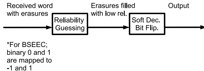
Figure 6-1: Block diagram of a simple decoder using the reliability guessing method
