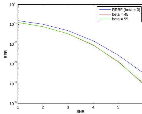
Figure 4-4: The BER performance of RRBf and MRRBF with (n = 96, k = 48, d_c = 4) LDPC code
