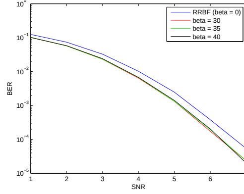
Figure 4-3: The BER performance of the modified reliability ratio algorithm with different \beta values using (n = 96, k = 48, d_c = 3) LDPC code
