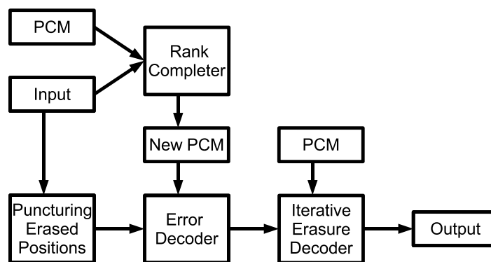
Figure 6-10: Block diagram for the complete EED with RC
