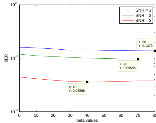
Figure 4-7: The BER performance of the modified reliability ratio algorithm for SNR values 1, 2, and 3 with (816, 408, 5) LDPC code
