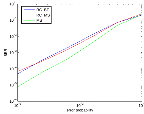
Figure 6-19: The performance of RC+BF, RC+MS, MS on BSEEC with p_1 = 0.1 with (96,48) LDPC code
