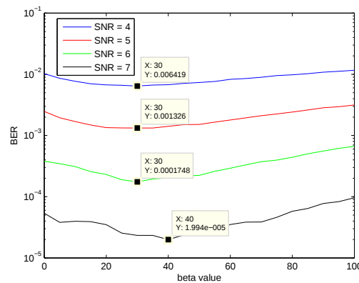
Figure 4-2: The BER performance of the modified reliability ratio algorithm for SNR values 4, 5, 6, and 7 with (n = 96, k = 48, d_c = 3) LDPC code
