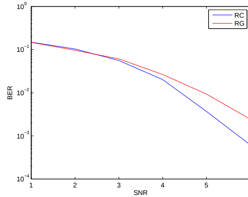
Figure 6-22: The performance of bootstrapped RC and bootstrapped RG on AWGN+EC with p_1 = 0.1 with (816,408) LDPC code
