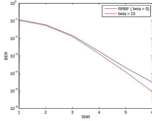
Figure 4-8: The BER performance of RRBF and MRRBF with (816, 408, 3) LDPC code for SNR values 1-6
