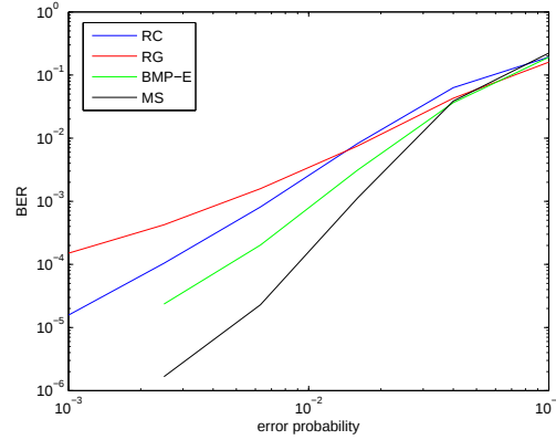
Figure 6-17: The performance of RC, RG, MS, and BMP-E on BSEEC with p_1 = 0.1 with (204,102) LDPC code
