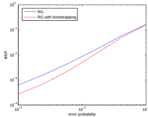
Figure 6-9: The BER performance of RG with and without bootstrapping using (96,48,3) on BSEEC with p_1 = 0.1
