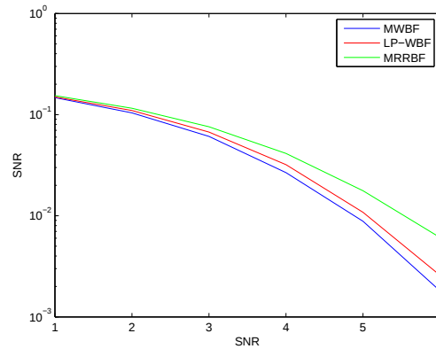
Figure 6-15: The performance of RC with different BF decoders on AWGN+EC with 0.1 erasure probability, using (96,48,3) LDPC code
