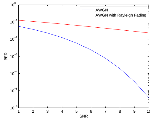
Figure 2-5: The comparison of uncoded AWGN channel to uncoded AWGN with Rayleigh fading channel
