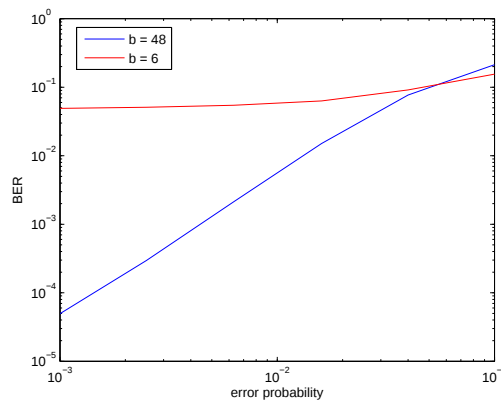
Figure 6-13: BER performance of the complete EED with separation bounds 6 and 48, with (n = 96, k = 48, d = 6) LDPC code on AWGN+EC with p_1 = 0.1
