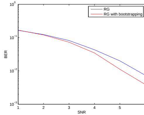
Figure 6-8: The BER performance of RG with and without bootstrapping using (504,252,3) on AWGN+EC with p_1 = 0.1
