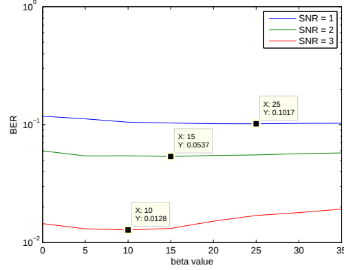
Figure 4-6: The BER performance of the modified reliability ratio algorithm for SNR values 1, 2, and 3 with (816, 408, 3) code
