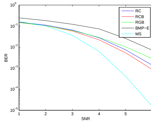
Figure 6-21: The performance of RC, RCB, RGB, MS, and BMP-E on AWGN+EC with p_1 = 0.1 with (204,102) LDPC code
