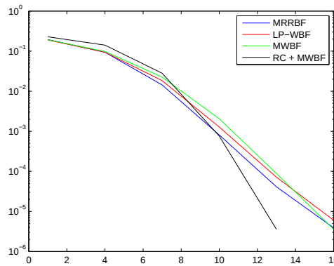
Figure 6-24: The performance of MRRBF, LP-WBF, MWBF, and MWBF+RC (ED) on AWGN channel with Rayleigh fading using (n = 204, k = 102, d_c = 3) LDPC code
