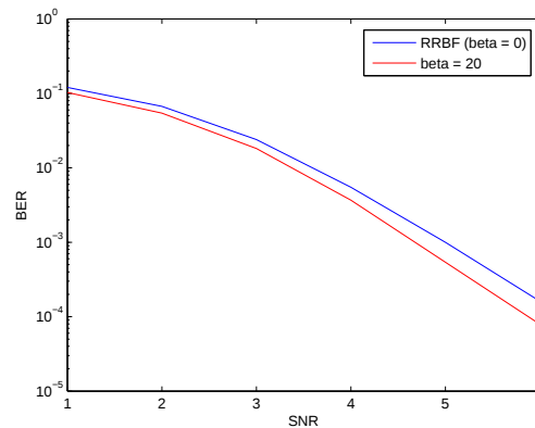
Figure 4-5: The BER performance of RRBf and MRRBF with (n = 204, k = 102, d_c = 3) LDPC code
