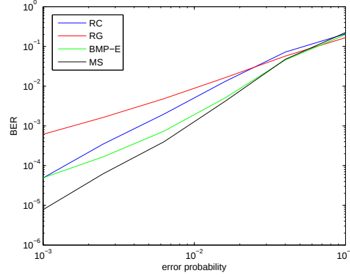
Figure 6-16: The performance of RC, RG, MS, and BMP-E on BSEEC with p_1 = 0.1 with (96,48) LDPC code
