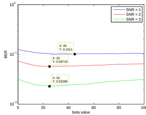
Figure 4-1: The BER performance of the modified reliability ratio algorithm for SNR values 1, 2, and 3 with (n = 96, k = 48, d_c = 3) LDPC code
