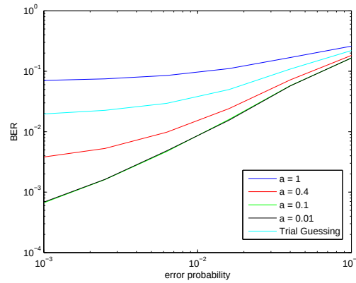
Figure 6-2: The BER performance of RG with different a values for (96,48) and Trial Guessing code on BSEEC with p_1 = 0.1
