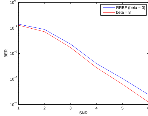
Figure 4-9: The BER performance of RRBF and MRRBF with (2048, 1030) LDPC code
