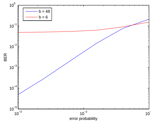
Figure 6-12: BER performance of the complete EED with separation bounds 6 and 48, with (n = 96, k = 48, d = 6) LDPC code on BSEEC with p_1 = 0.1
