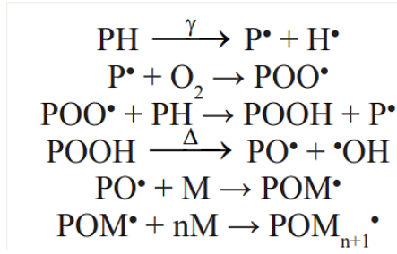
Figure 2.7. The mechanism of the peroxide grafting, where PH, P • , POO • , POOH, PO • , and M represent the polymer substrate, alkyl radicals, peroxide radicals, hydroperoxides, alkoxy radicals, and monomer, respectively [68].
