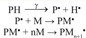
Figure 2.6. The mechanism of the simultaneous grafting, where PH, M, \text{PM}_{n+1}^\bullet represent the polymer substrate, monomer, and macroradicals, respectively [68].
