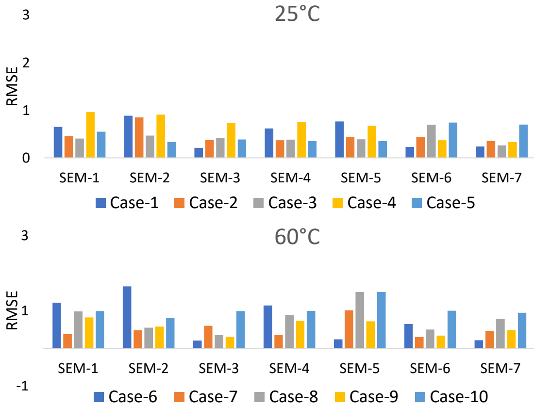
Figure 29. Performance indicators for each Helios NMC case modeling with GA.
