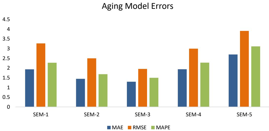
Figure 20. Performance indicators for each LFP dataset modeling with analytical solution.
