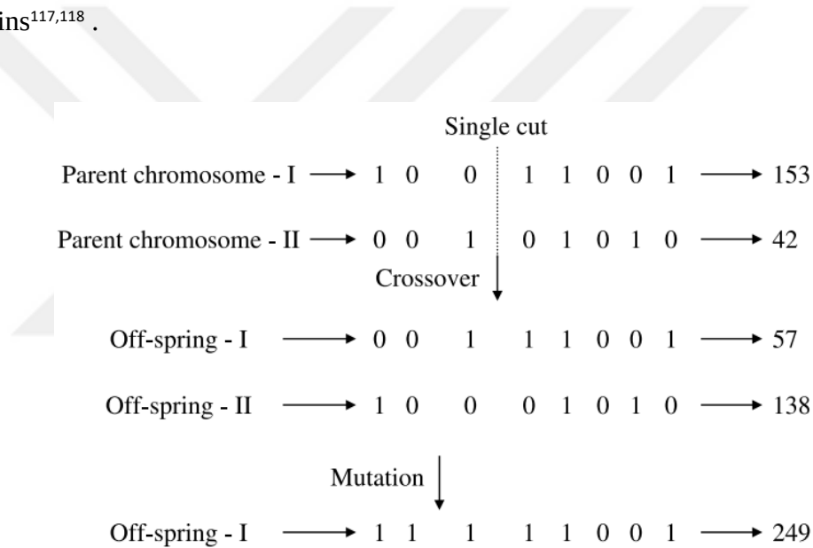
Figure 3. Example for GA process 117,118 .
