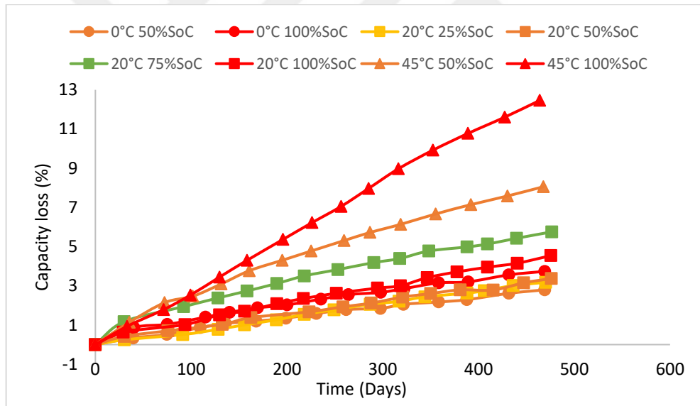
Figure 10. NMC-1 Experimental results for each storage condition.
