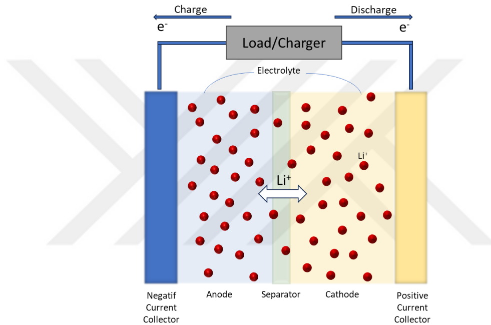
Figure 1 Lithium-ion battery schematic 27 .
