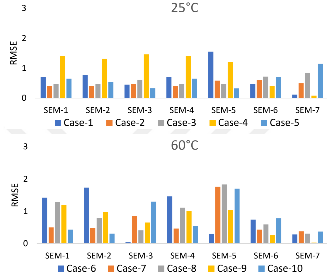
Figure 27. Performance indicators for each Helios NMC prediction case modeling with analytical solution.
