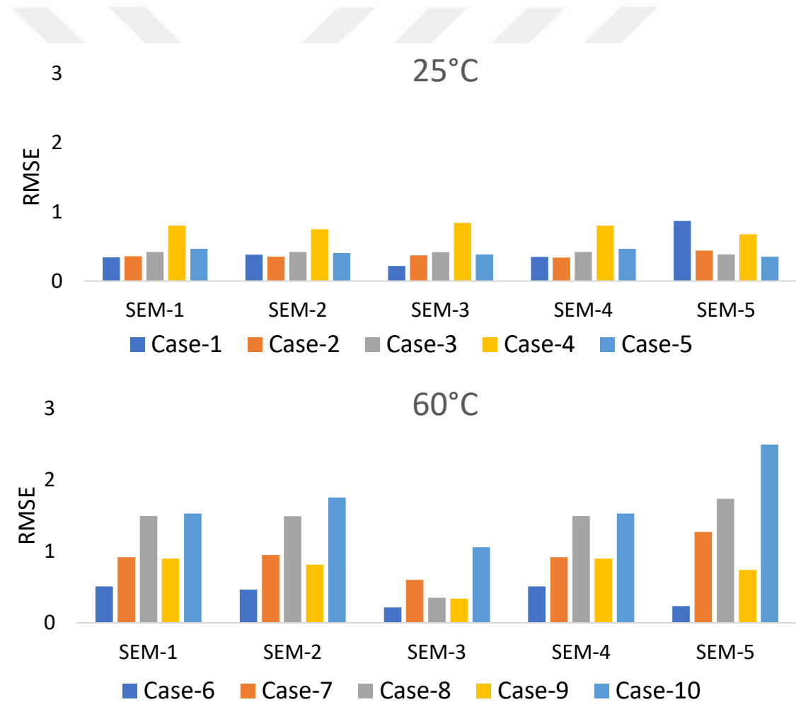
Figure 28. Performance indicators for each Helios NMC case modeling with analytical solution.
