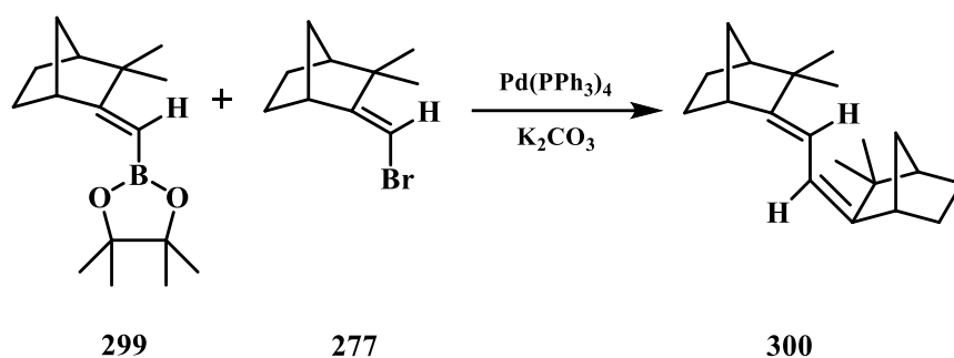
Figure 4.38. Synthesis of compound 300
