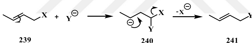
Figure 2.73. Nucleophilic substitution reaction at vinylic position
