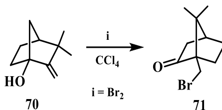
Figure 2.28. Bromination of 1-hydroxy camphene under electrophilic condition
