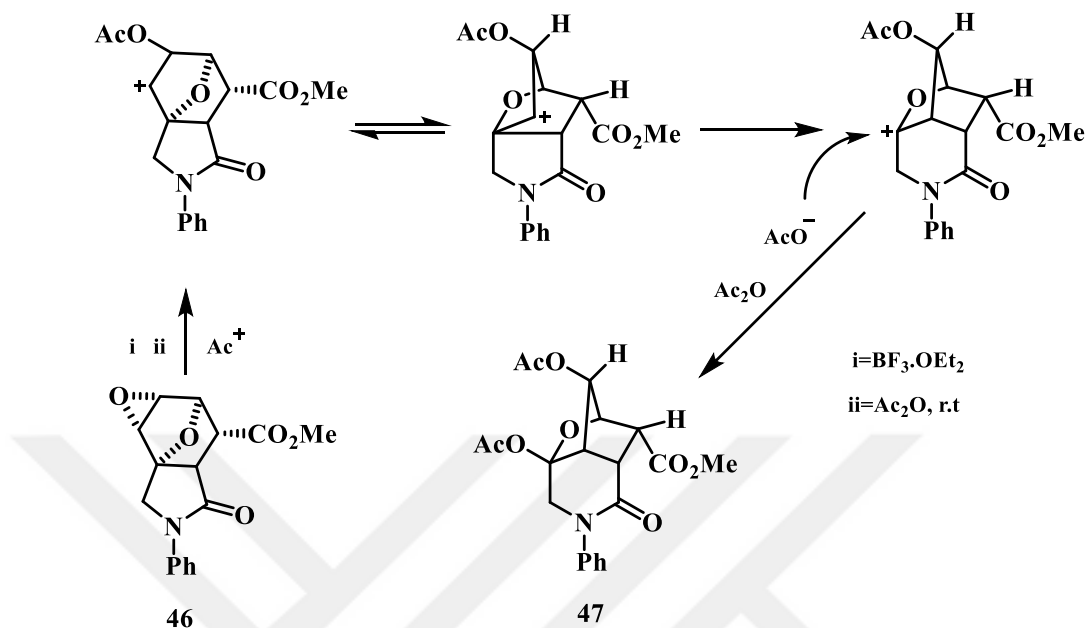
Figure 2.16. Wagner-Meerwein rearrangement (type 1) of oxirane ring of diepoxide (46)
