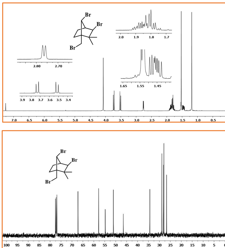
Figure 4.12. ^1\text{H} NMR and ^{13}\text{C} NMR of compound 280
