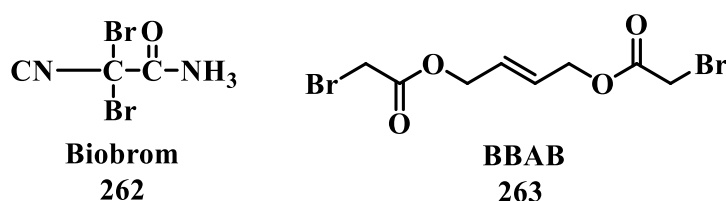
Figure 2.84. Disinfecting agents
