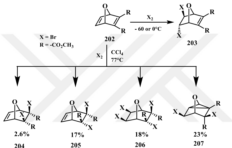
Figure 2.62. Heteroatom effects on the bicyclic systems
