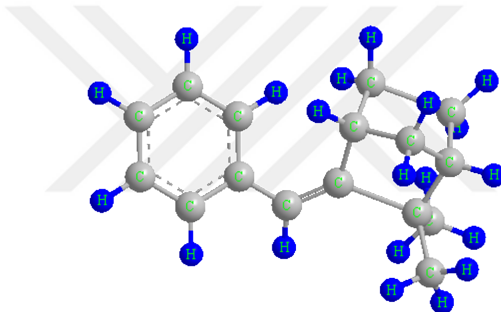
Figure 5.22. Structure of compound 288 drawn at 10° angle
