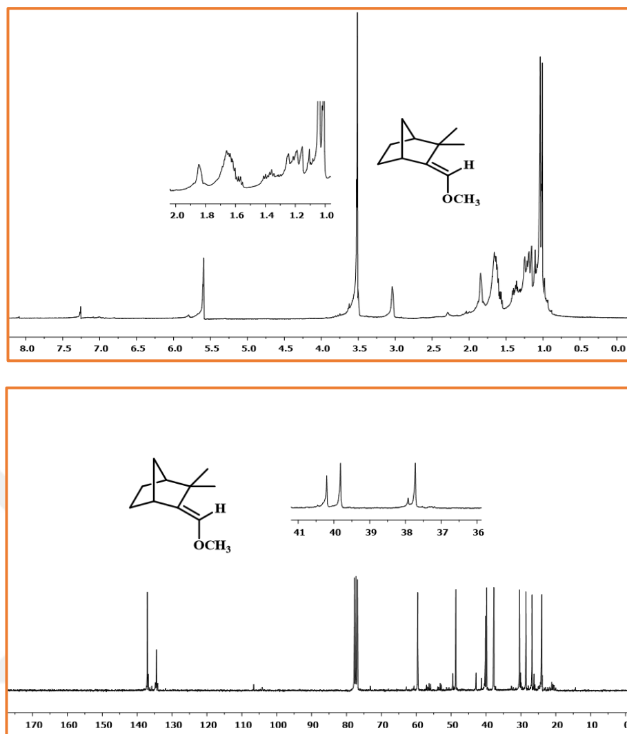
Figure 4.33. ^1\text{H} NMR and ^{13}\text{C} NMR of compound 297
