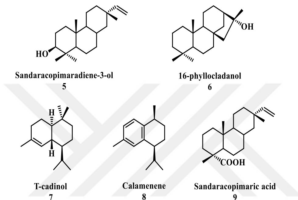
Figure 2.2. Bioactive sesqui- and di-terpenes
