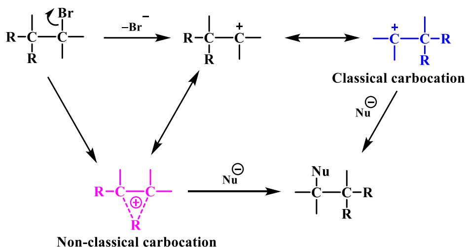
Figure 2.11. Formation of classical and non-classical carbocation in a reaction
