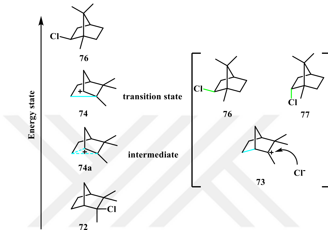
Figure 2.31. Energy diagram for the chlorination of camphene
