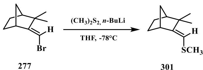
Figure 4.40. Synthesis of compound 301
