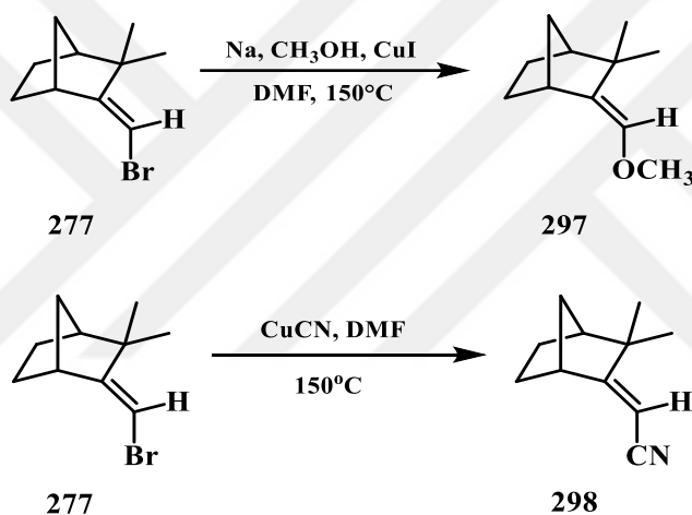
Figure 5.11. Nucleophilic substitution reaction of monobrominated camphene compound (277)
