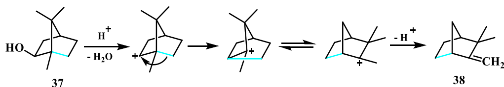
Figure 2.12. Wagner-Meerwein rearrangement in the bicyclic norborneol
