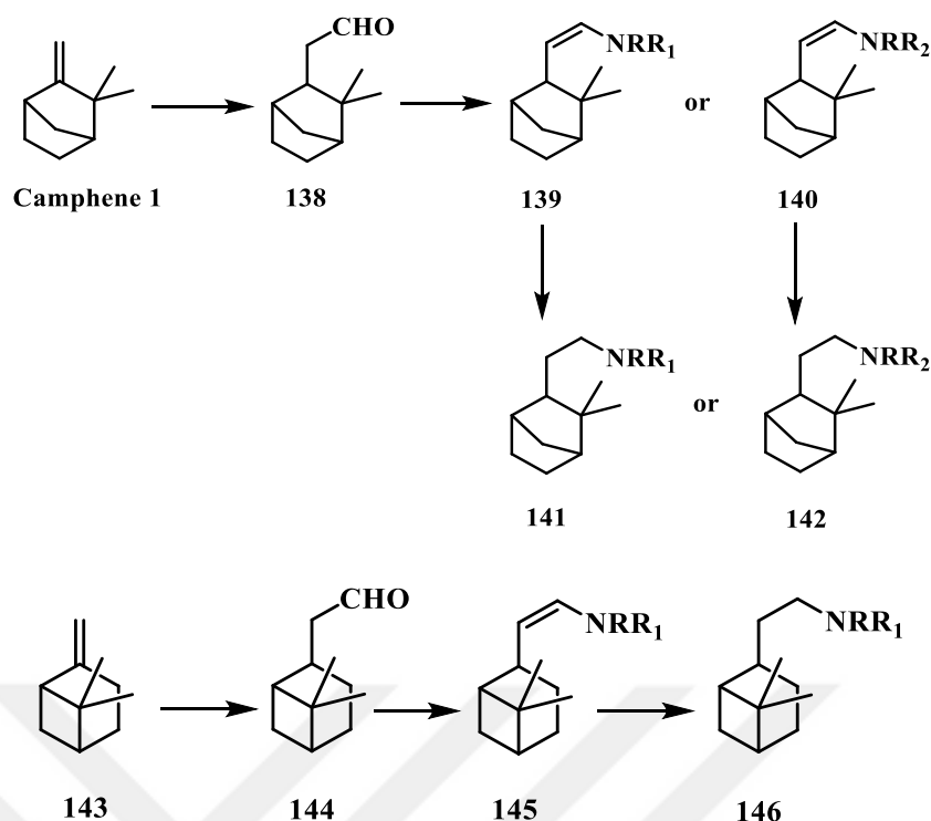
Figure 2.46. Hydroaminomethylation of camphene (1) and β-pinene (143)
