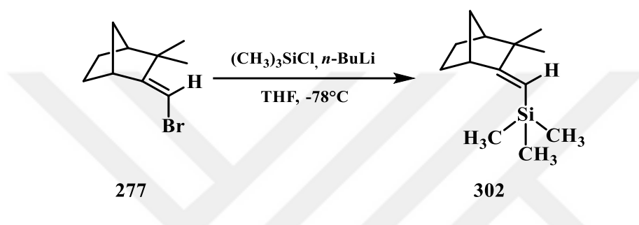
Figure 4.42. Synthesis of compound 302
