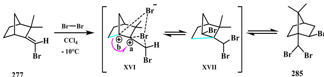
Figure 5.9. Formation mechanism of compound 285
