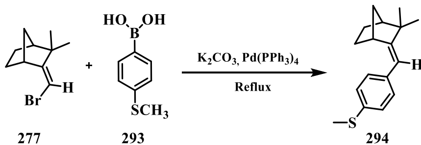
Figure 4.28. Synthesis of compound 294
