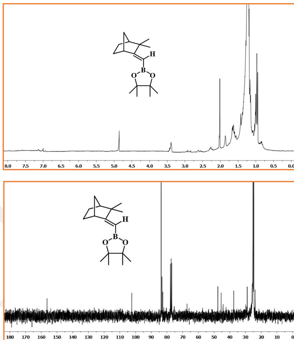
Figure 4.37. ^1\text{H} NMR and ^{13}\text{C} NMR of compound 299
