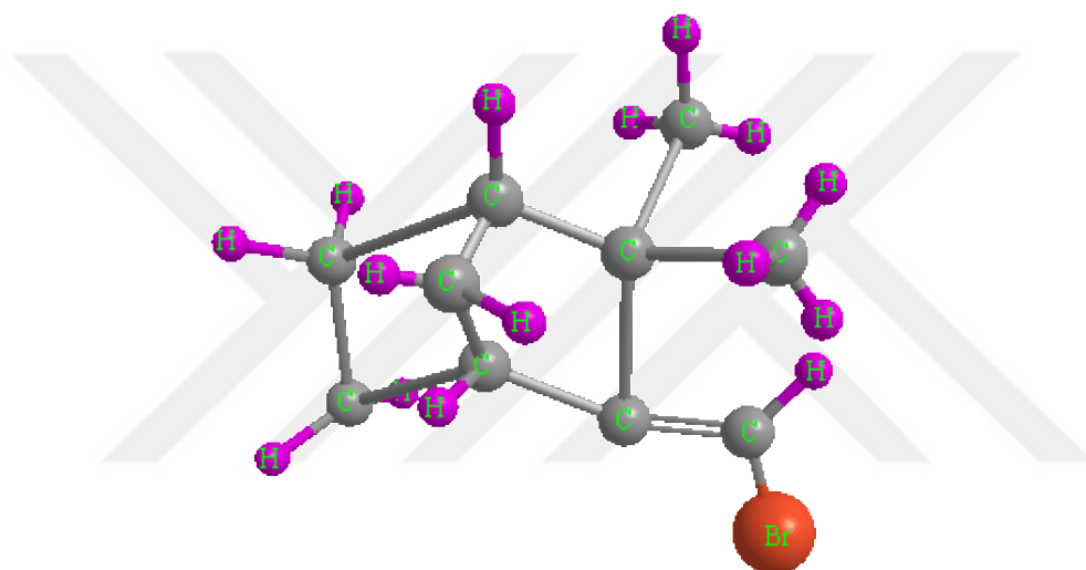
Figure 5.19. Structure of compound 277 drawn at 7° angle
