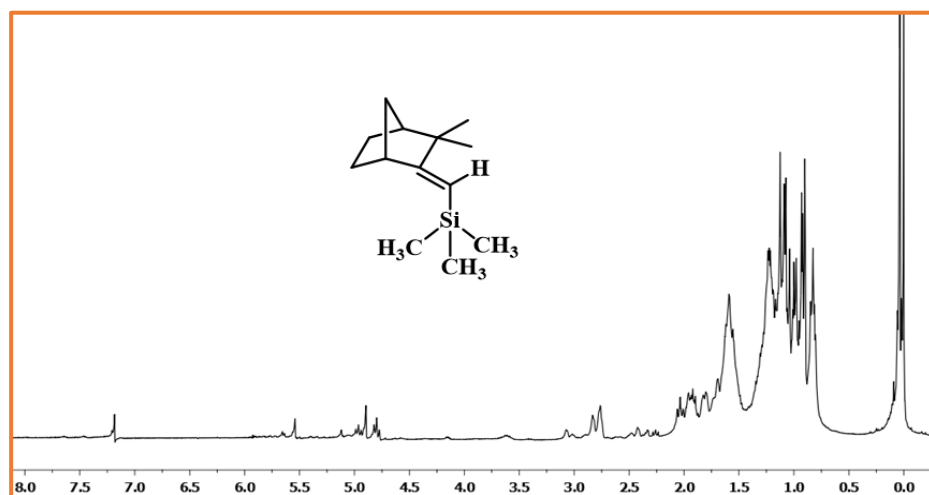
Figure 4.43. 1 H NMR of compound 302
