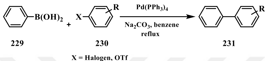
Figure 2.68. Synthesis of compound 231 via Suzuki coupling reaction
