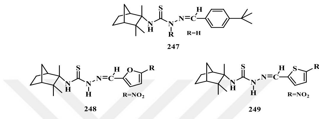
Figure 2.78. Anti-tuberculosis agents
