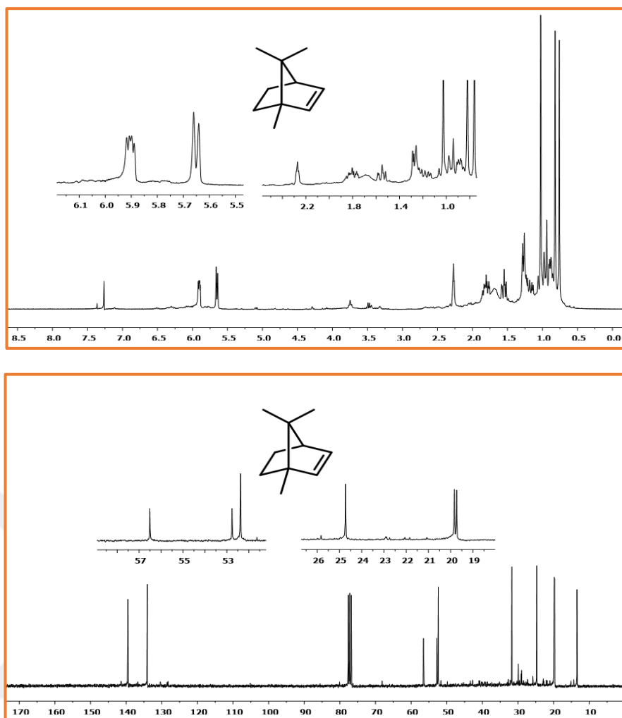
Figure 4.21. ^1\text{H} NMR and ^{13}\text{C} NMR of compound 286
