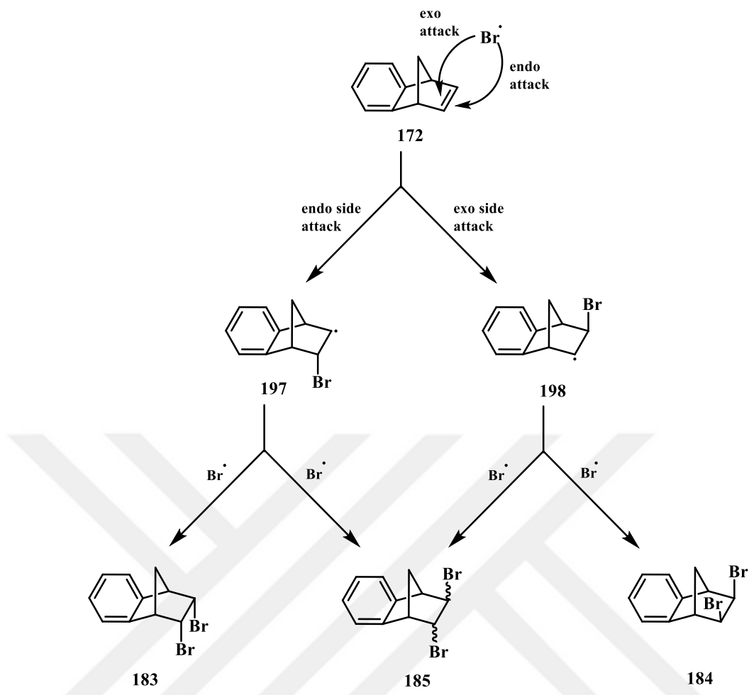
Figure 2.60. Radical mechanism in the bicyclic system
