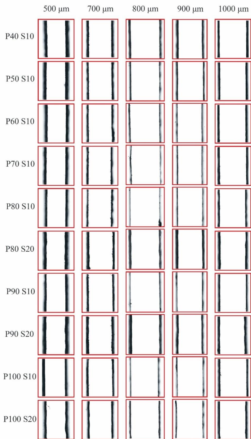
Figure 3.2. Microscopic images of obtained microfluidic channels by ten parameters used in vector mode operation.
