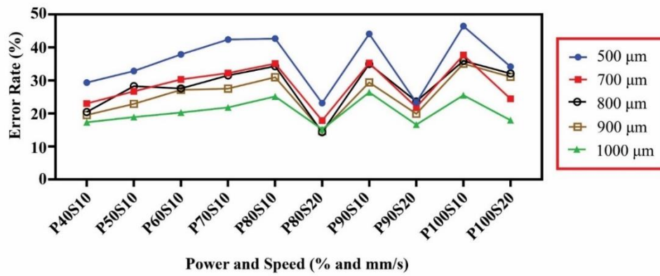
Figure 3.3. Error rates for ten different P-S combinations in vector operation mode. Each data point represents the percentage difference between obtained width and the theoretical width.
