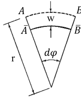
Figure 4.4. Tangential strain due to radial displacement.
