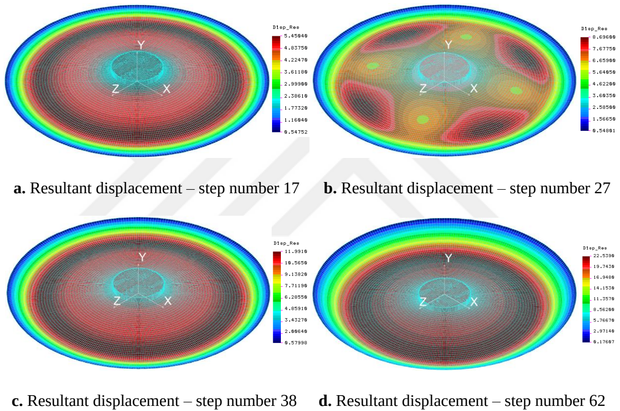
Figure 5.3. Resultant displacement of the simple supported conical shell for \alpha_c=10^\circ , t_{\text{shell}}=1.2 mm.
