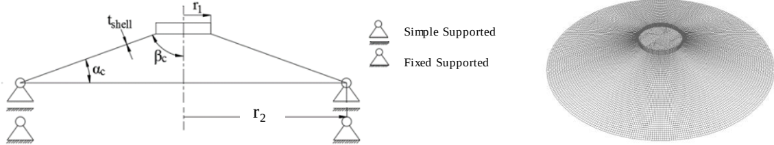
Figure 4.10. Schematic representation and numeric model of extremities.
