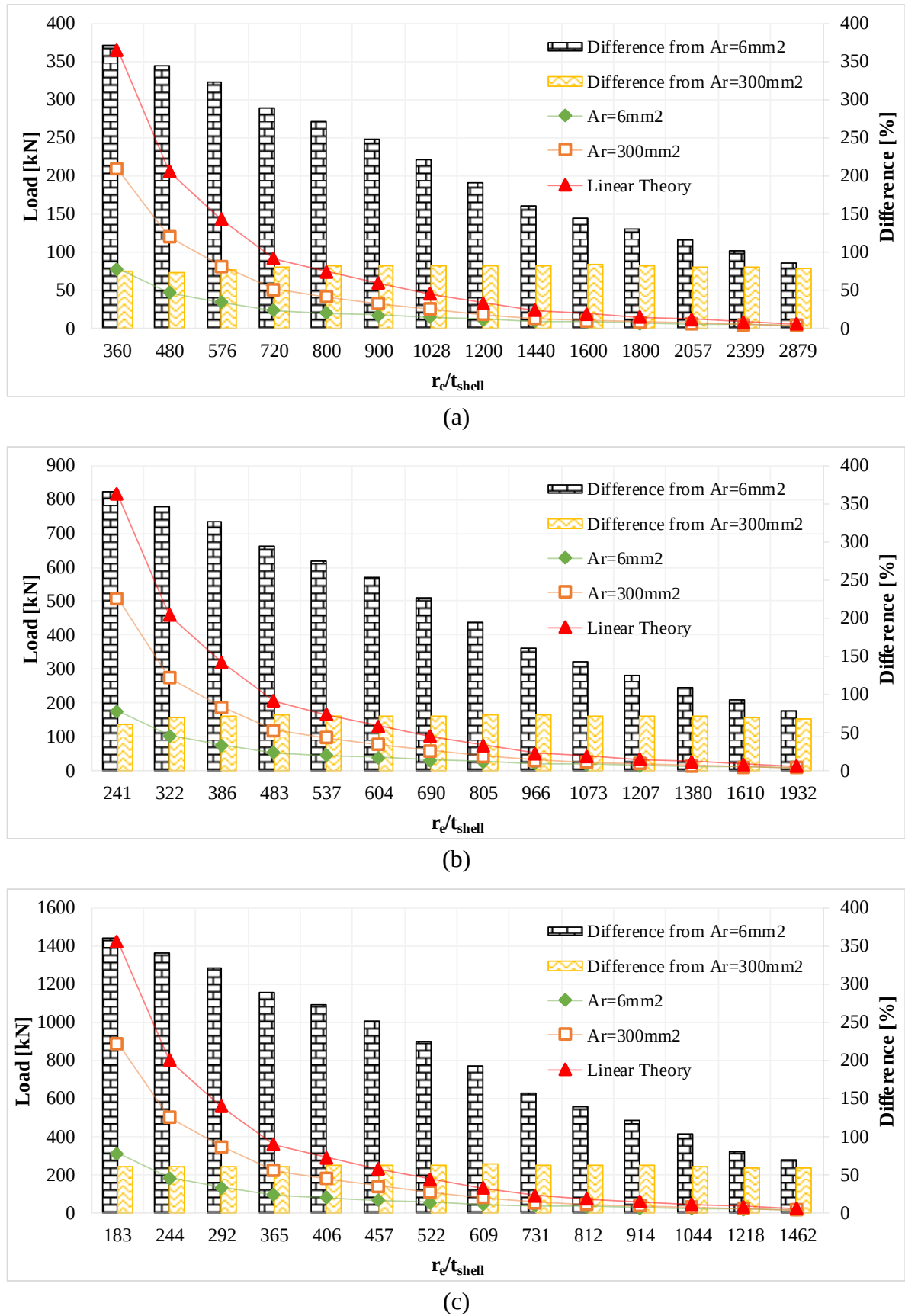
Figure 5.8. Comparison of the theoretical calculation with the limit loads of A_{ring}=6 \text{ mm}^2 and A_{ring}=300 \text{ mm}^2 cases. (a) Base angle 10°, (b) Base angle 15°, (c) Base angle 20°.
