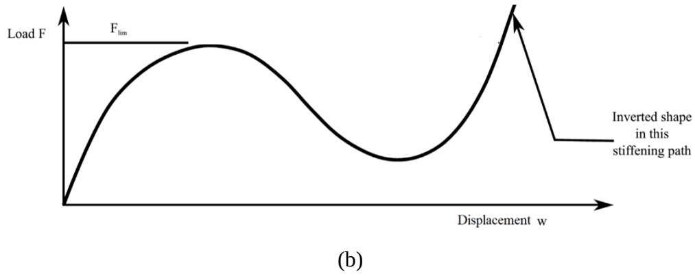
Figure 2.1. (a) Changing geometry of the structure, (b) Load-displacement response [5].
