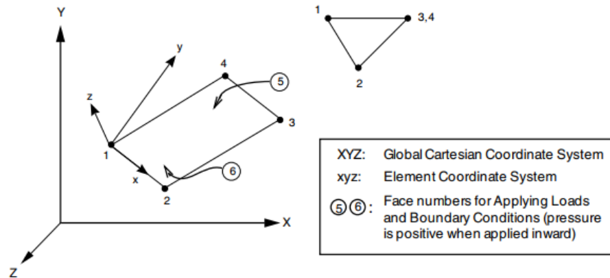
Figure 4.11. The nodal input pattern for a SHELL4T element [41].
