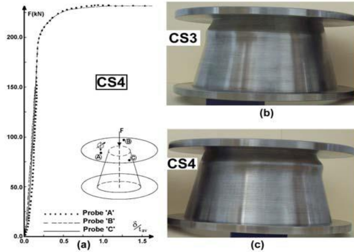
Figure 3.8. Tested conical shells after axial loading [30].
