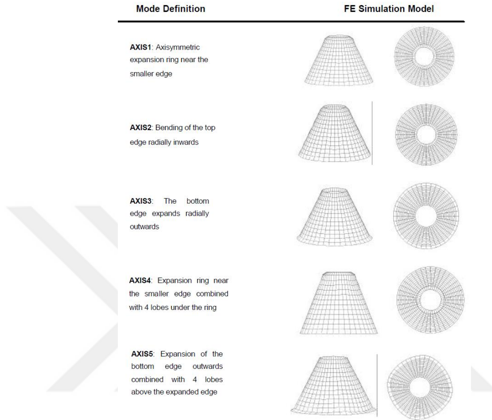
Figure 3.6. Model and definition of the axisymmetric buckling modes of constant [28].
