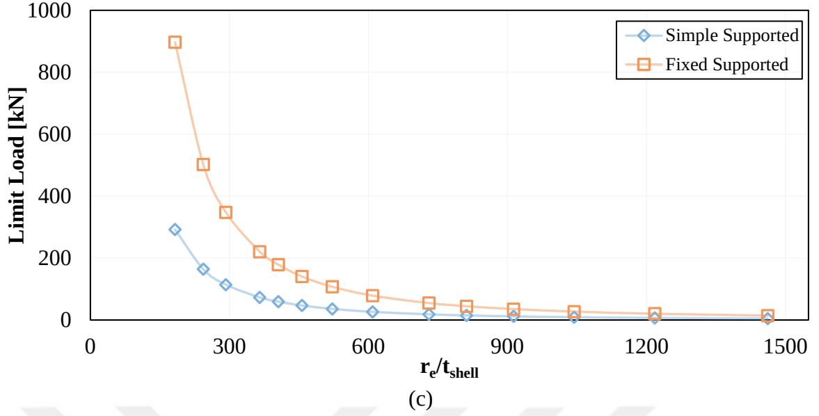
Figure 5.4. Influence of the boundary conditions on the load carrying capacity of the conical shell for different base angles, (a) Base angle 10^\circ , (b) Base angle 15^\circ , (c) Base angle 20^\circ .
