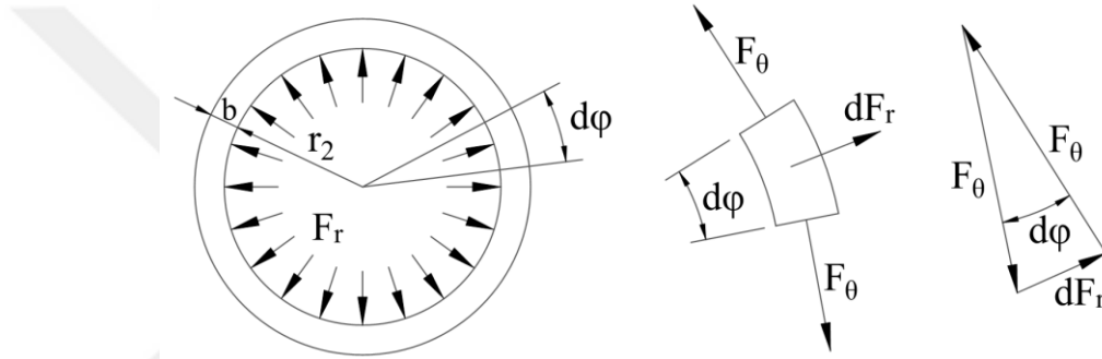
Figure 4.9. Equilibrium state of the forces on the element of the circumferential ring [7].
