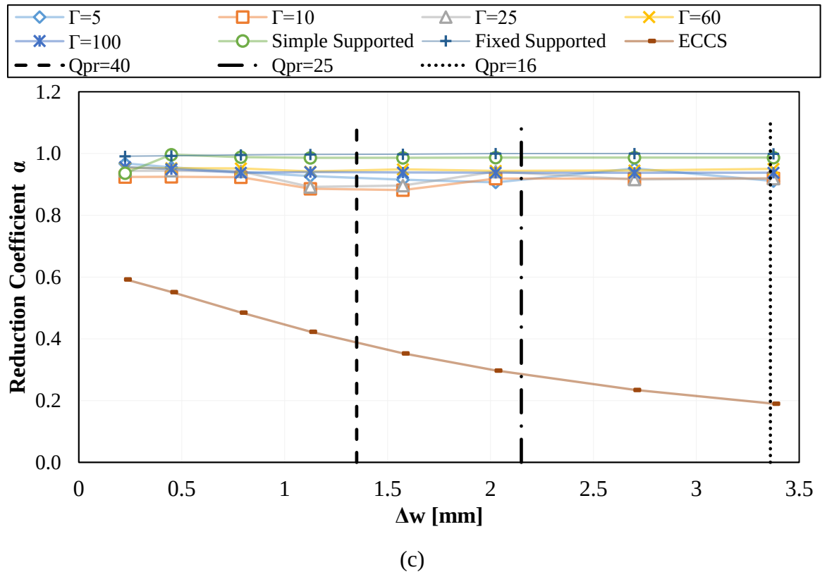
Figure 5.15. Reduction coefficient for different configuration of conical shells with a base angle 15^\circ . (a) t_{\text{shell}} = 0.6 mm, (b) t_{\text{shell}} = 1.4 mm, and (c) t_{\text{shell}} = 3 mm.
