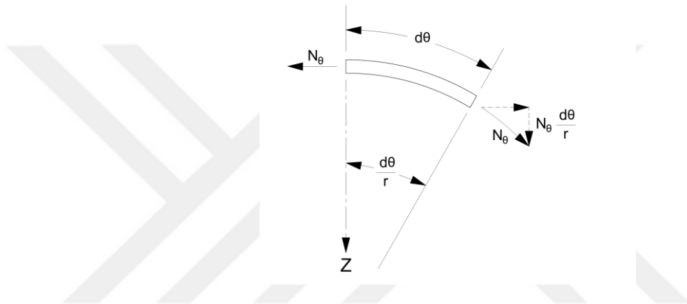
Figure 4.2. The radial component of in-plane forces due to initial curvature.
