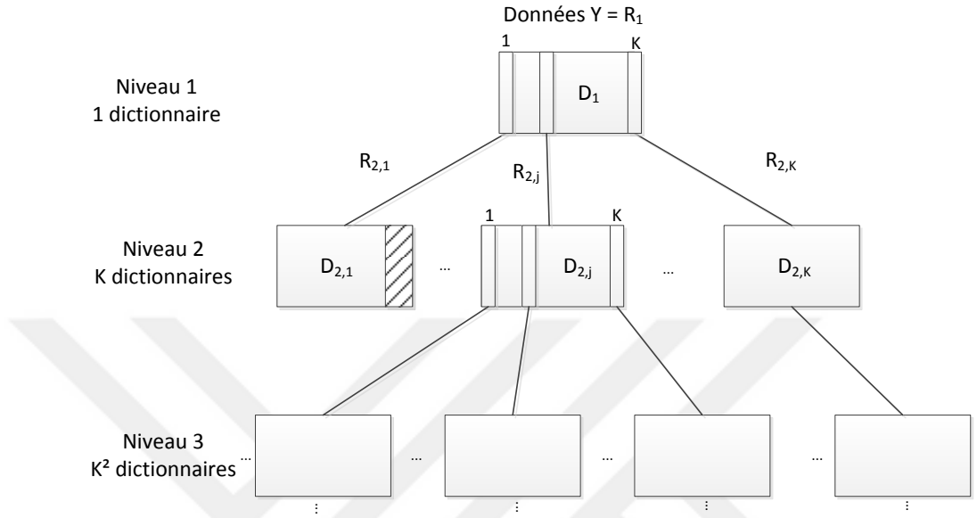
FIGURE 3.1 – La structure arborescente Tree K-SVD.
