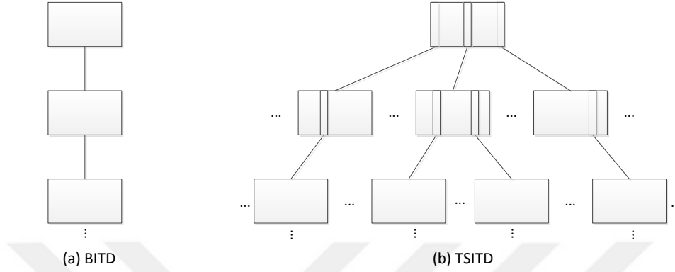
FIGURE 1.4 – Structures BITD (a) et TSITD (b).
