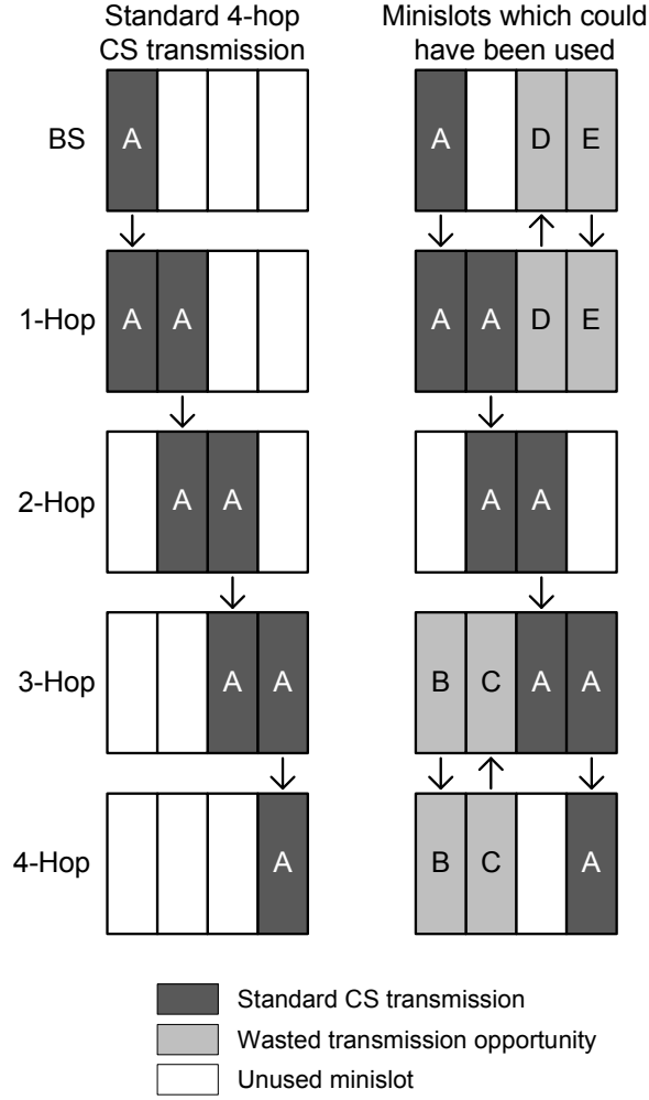
Figure 4.1. Wasted minislots during a standard CS transmission
