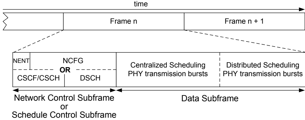
Figure 2.7. Mesh mode OFDM frame structure
