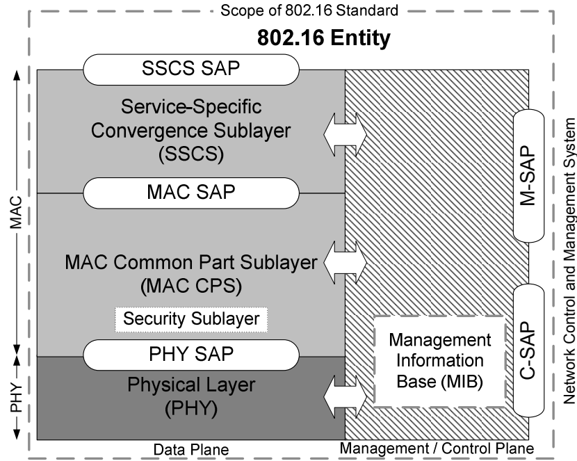
Figure 2.1. Reference model and scope of WiMAX standard [7]
