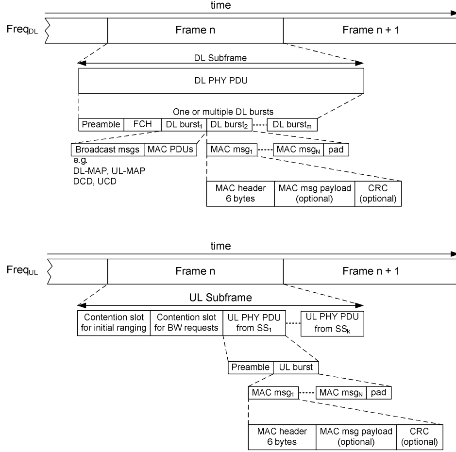
Figure 2.4. PMP mode OFDM frame structure using FDD [3]
