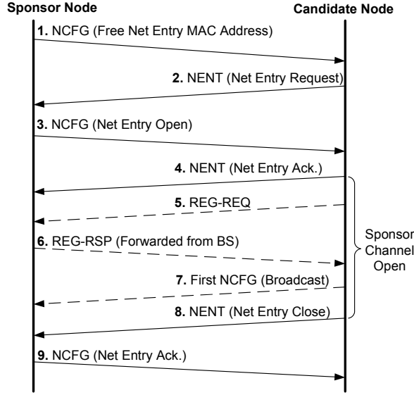
Figure 5.2. Network entry messaging in NEMMS
