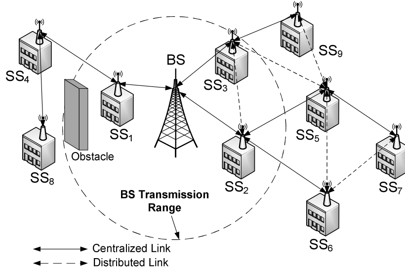
Figure 2.5. Sample WiMAX Mesh mode topology
