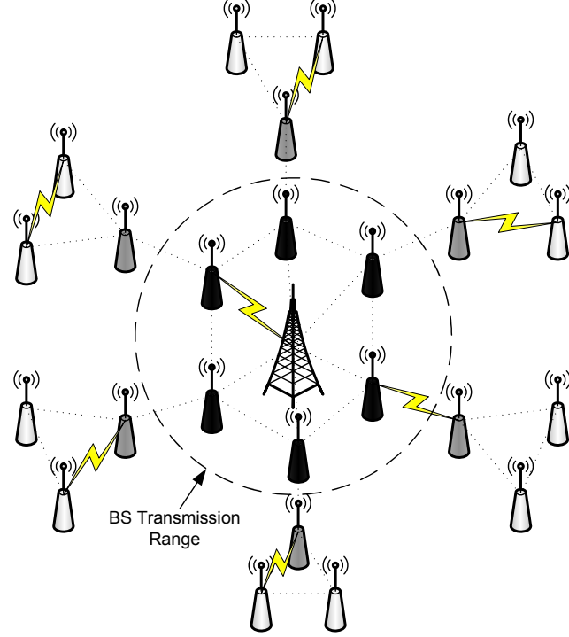
Figure 4.2. HFS concurrent transmissions
