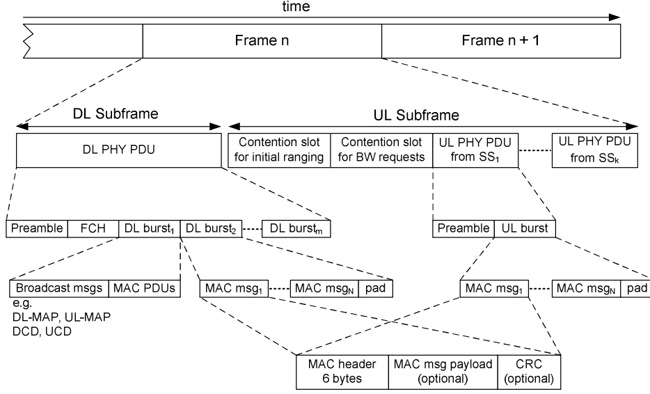
Figure 2.3. PMP mode OFDM frame structure using TDD [3]
