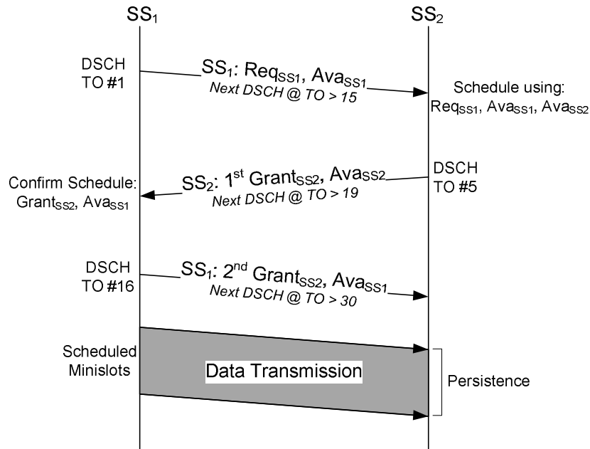
Figure 2.10. DS three-way handshake mechanism
