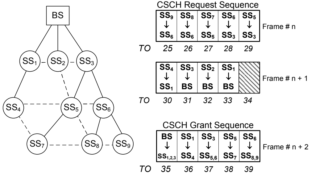
Figure 2.9. CS control message sequence
