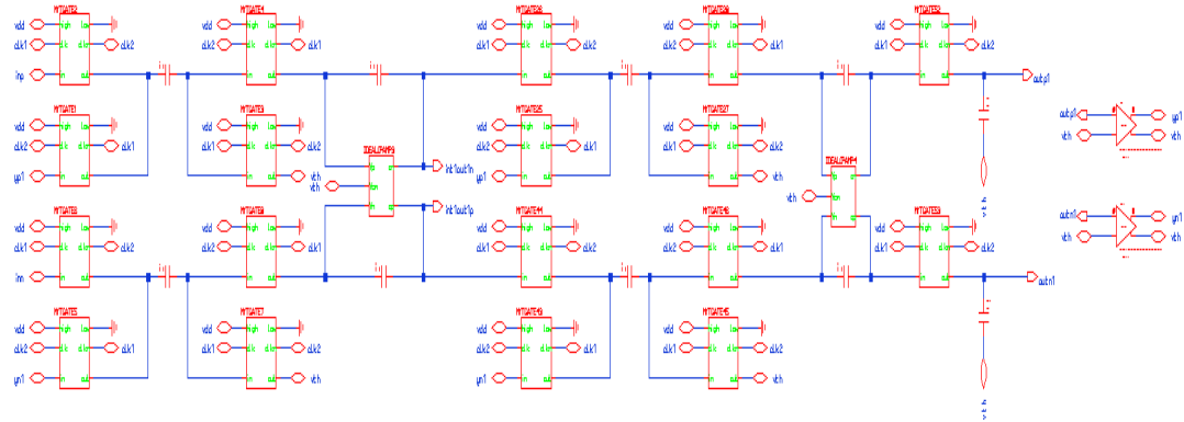
Figure 4.1. Circuit implementation of second order SD modulator with optimum gains by using ideal op-amps
