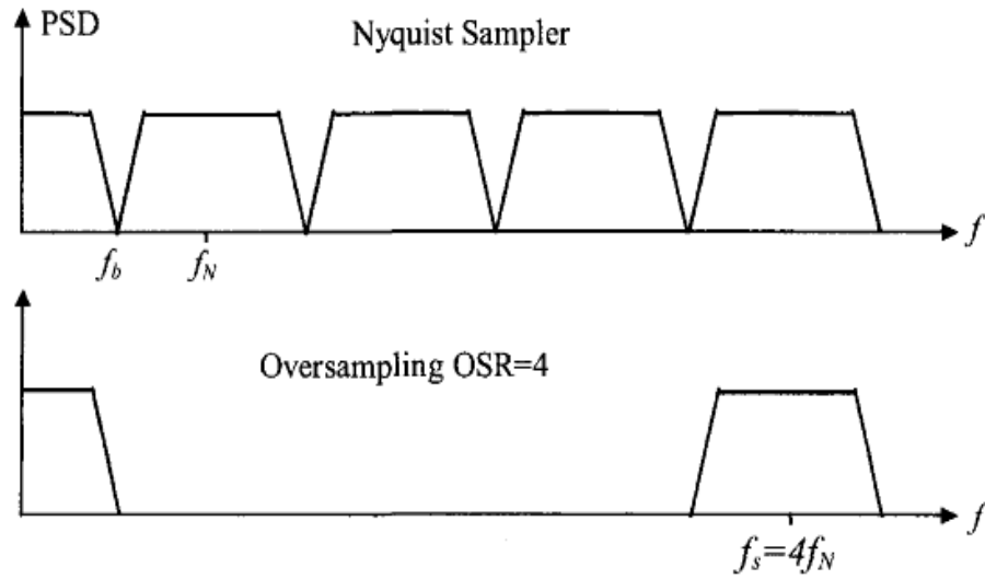
Figure 2.3. Oversampling process [10]
