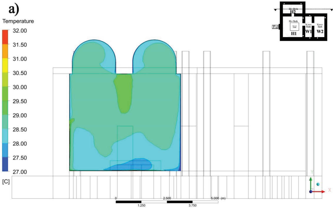
Figure 5.8. The temperature distribution in the the x-y-plane for Scenarios a, b, c and d.
