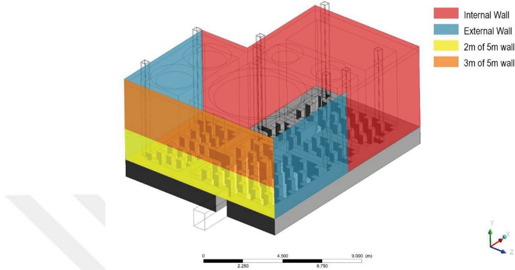
Figure 4.5. Perspective of the hypocaust system and walls of the Alibey Bath.
