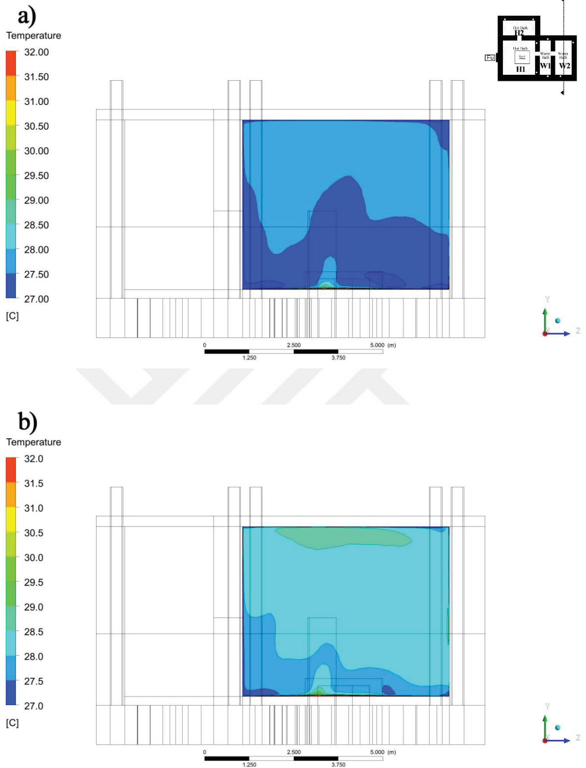
Figure 5.12. The temperature distribution in the y-z-plane for Scenarios a, b, c and d.
