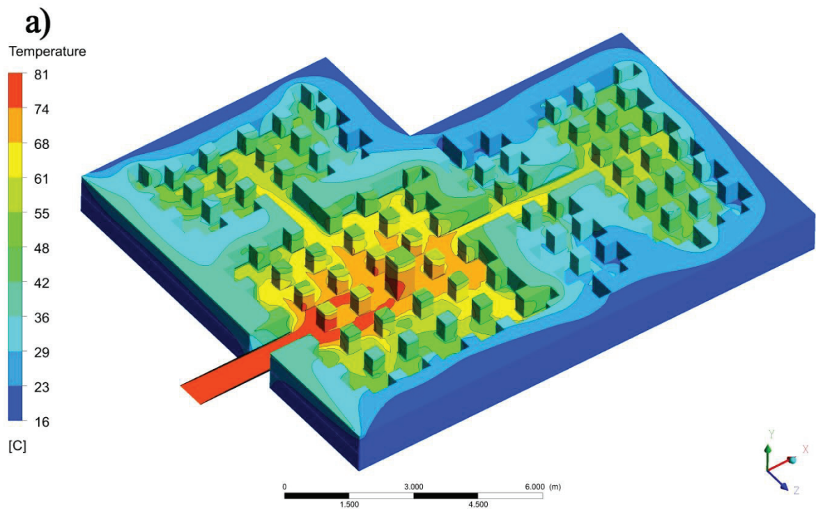
Figure 5.4. The temperature distribution in the hypocaust for Scenarios a, b, c and d.
