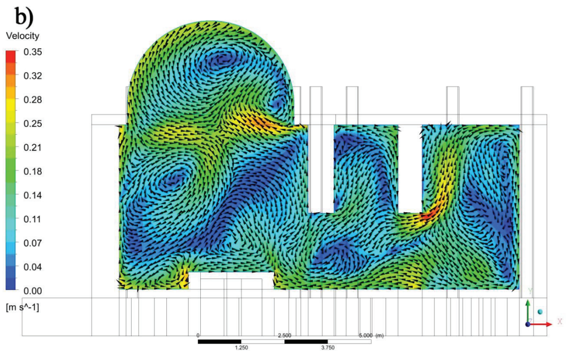
Figure 5.3. The velocity vectors in the x-y-plane for Scenarios a, b, c and d.
