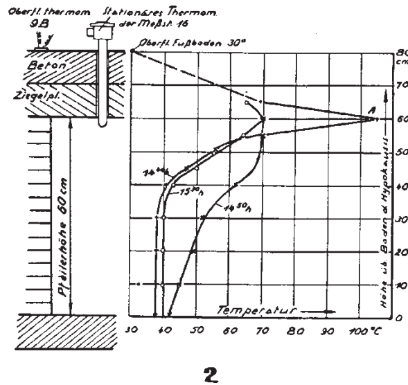
Figure 5.25. Präfurnium Temperature [13].
