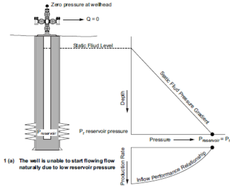
Figure 2.4 The well is unable to natural flow [15]
