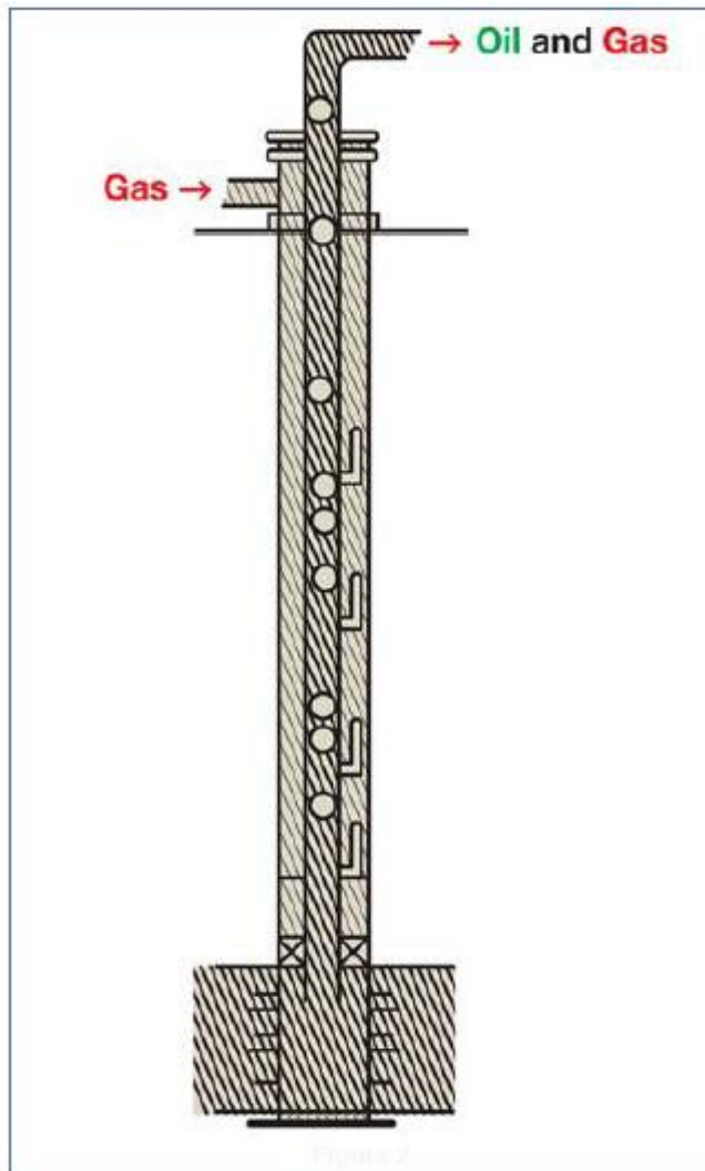
Figure 2.38 Continuous Gas Lift [15]
