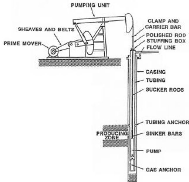
Figure 2.18 Sucker Rod Pump systems
