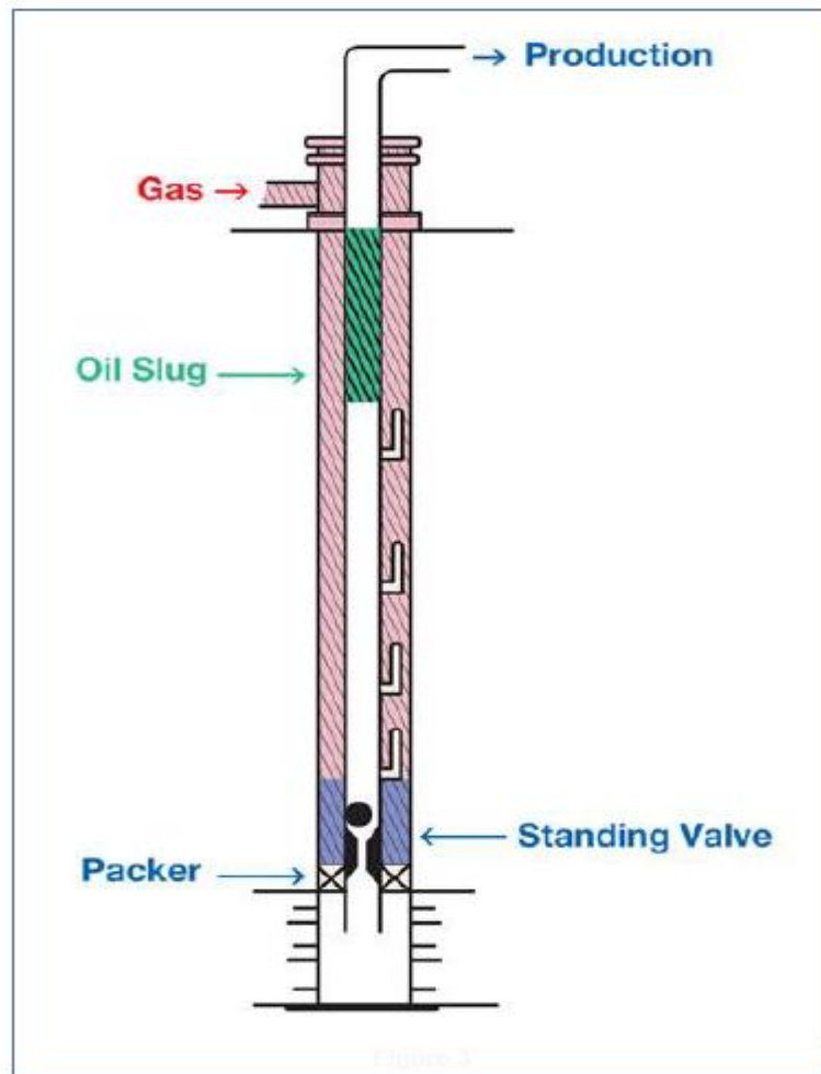
Figure 2.39 Intermittent Gas Lift [15]
