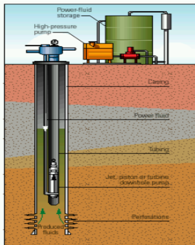
Figure 2.28 Schematic view of Hydraulic Pump [12]
