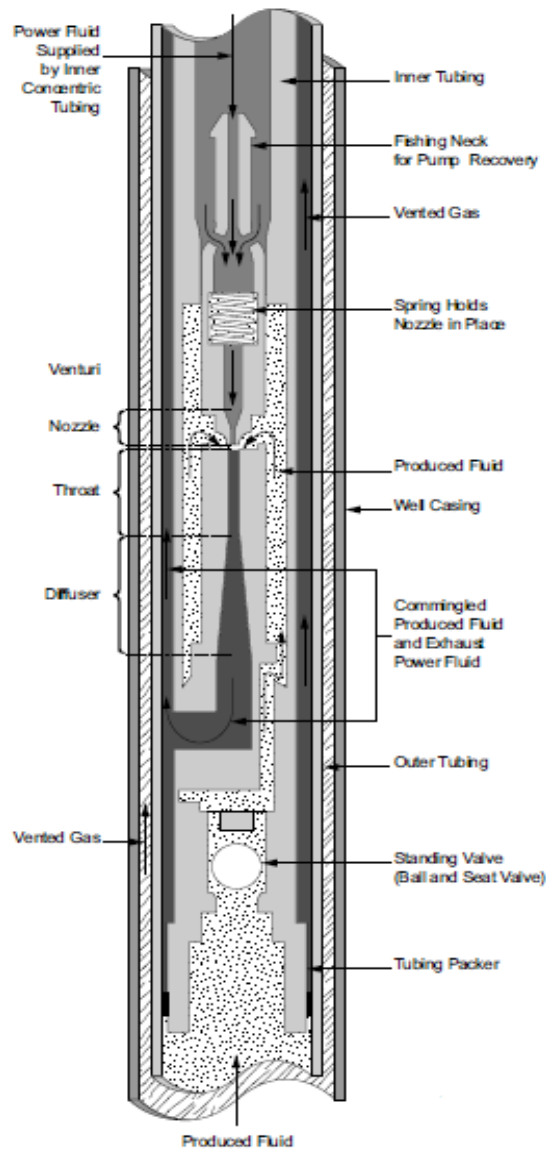
Figure 2.30 Schematic view of Jet pump operation [15]
