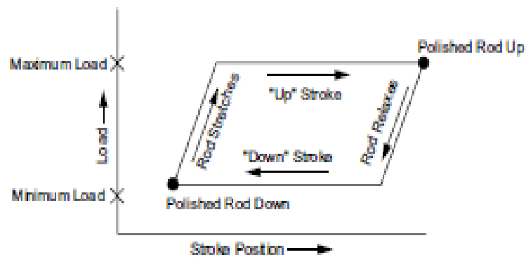
Figure 2.24 Dynamometer in ideal condition
