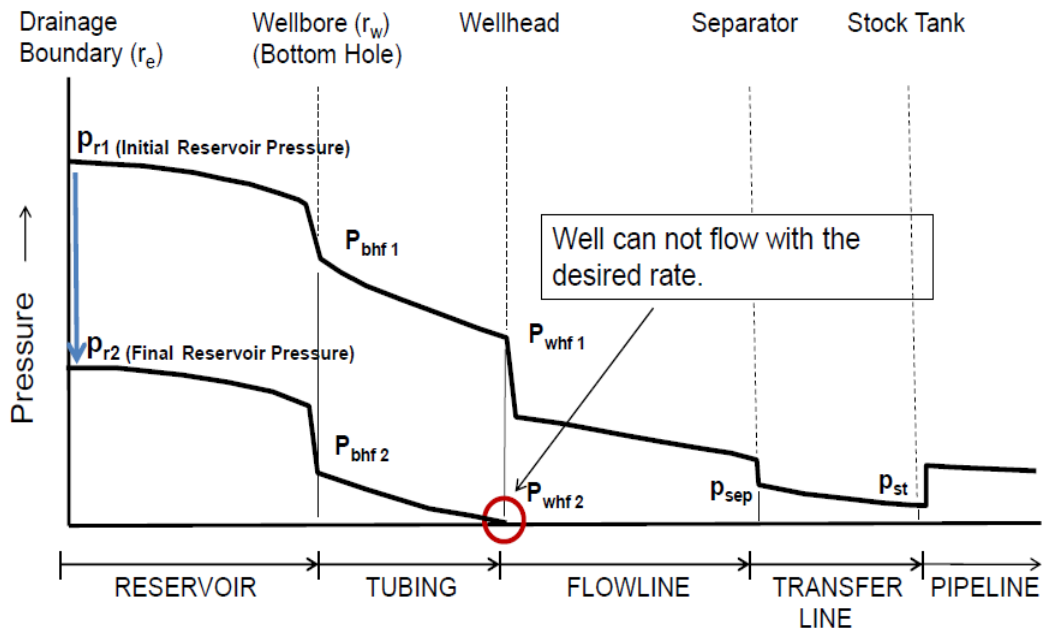
Figure 2.1 Schematic Pressure Profile for Production System [12]
