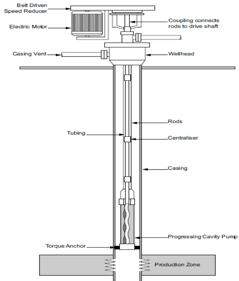
Figure 2.32 Schematic view of PCP system [15]
