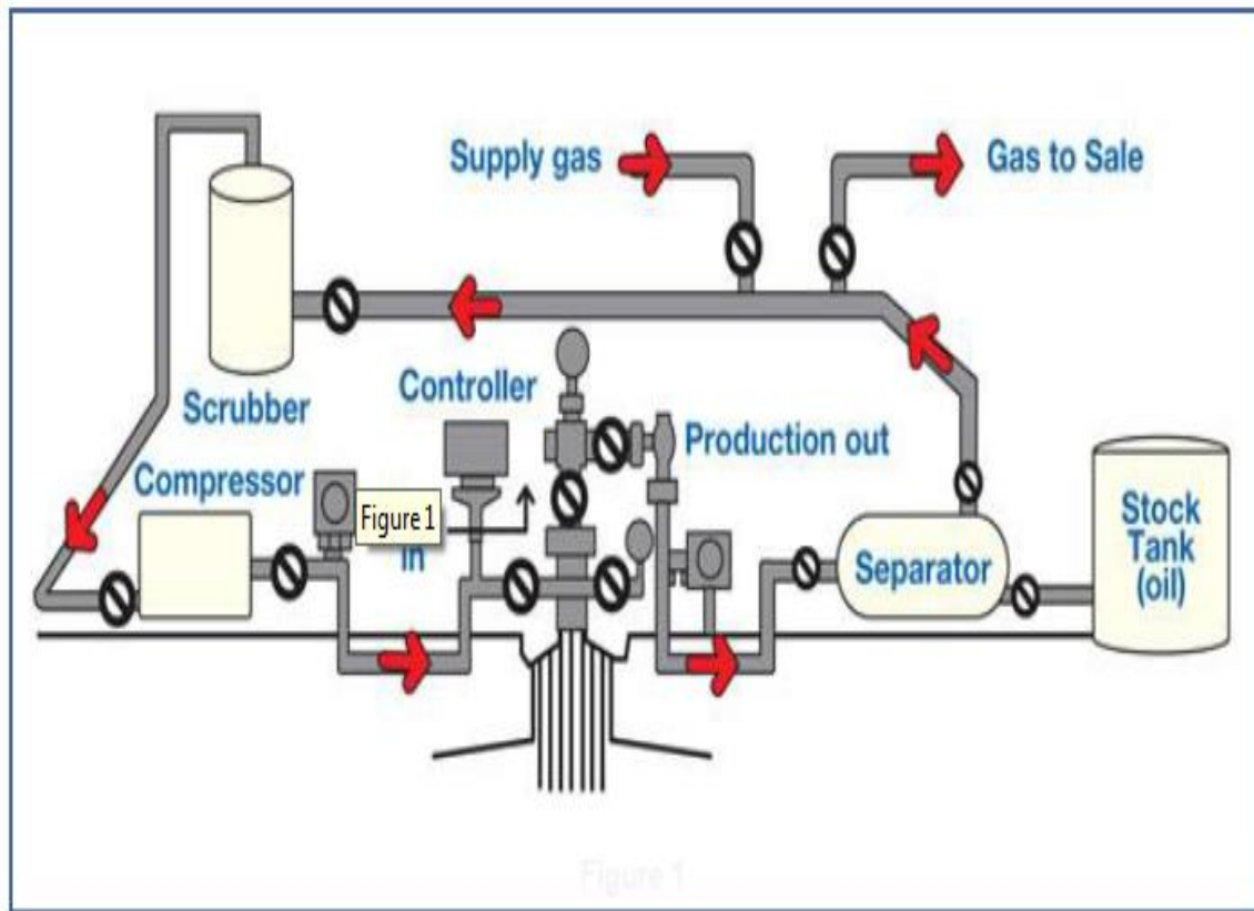
Figure 2.36 Schematic view of Gas Lift system [13]
