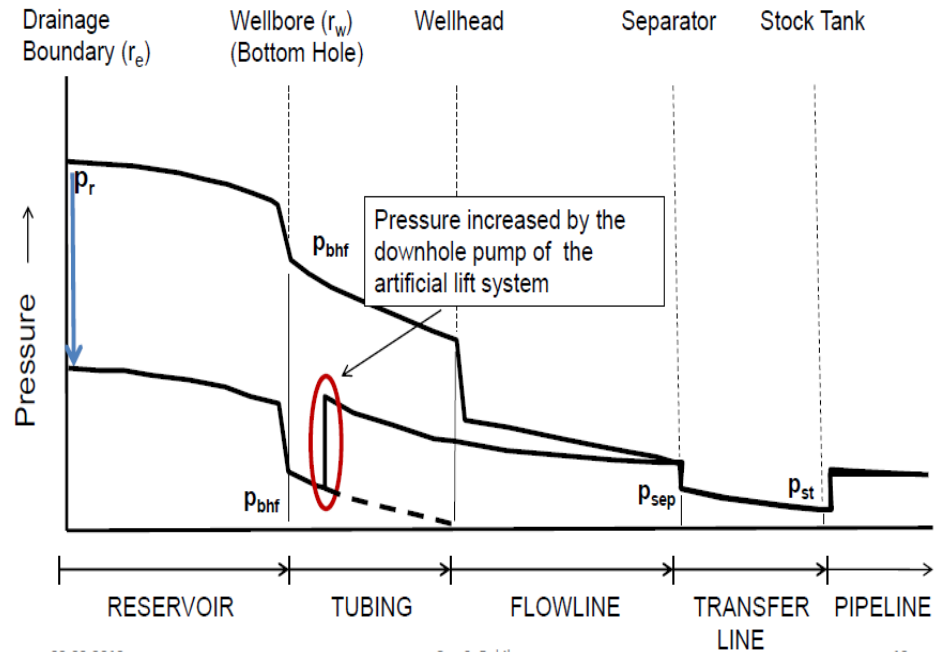
Figure 2.3 Schematic Pressure Profile for Production System [12]
