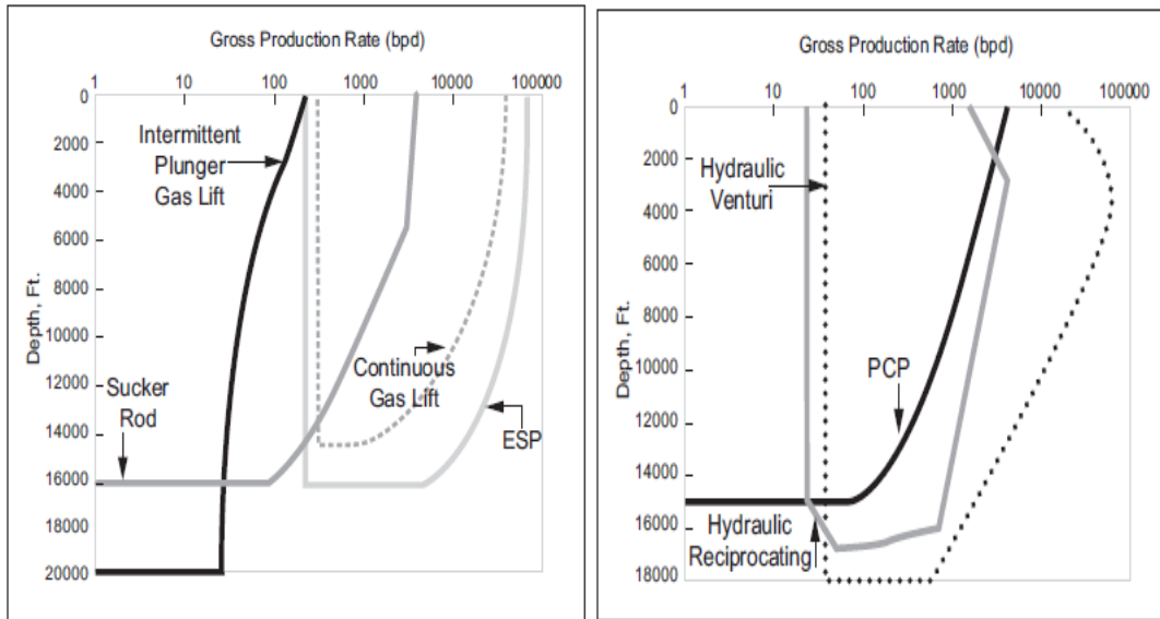
Figure 2.17 Application areas of main artificial lift methods [15]
