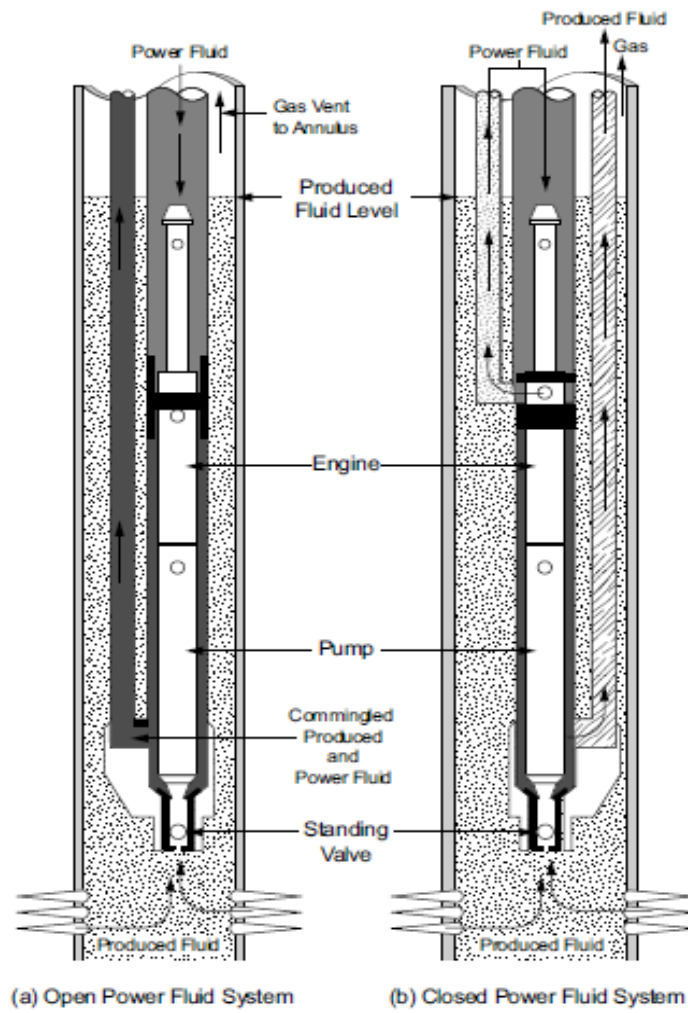
Figure 2.31 Hydraulic pump installation types [15]
