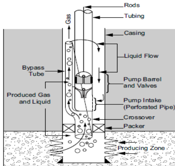
Figure 2.22 Gas anchor set in the well [15]
