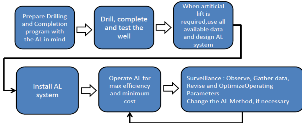
Figure 2.7 Consideration of artificial lift throughout of the well life [12]
