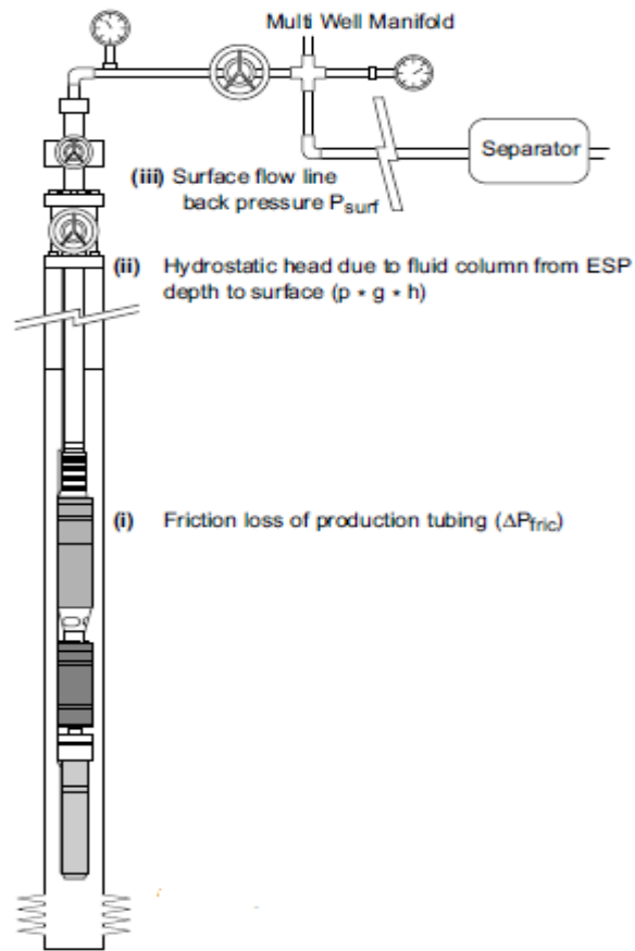
Figure 2.27 Pump TDH requirements [15]
