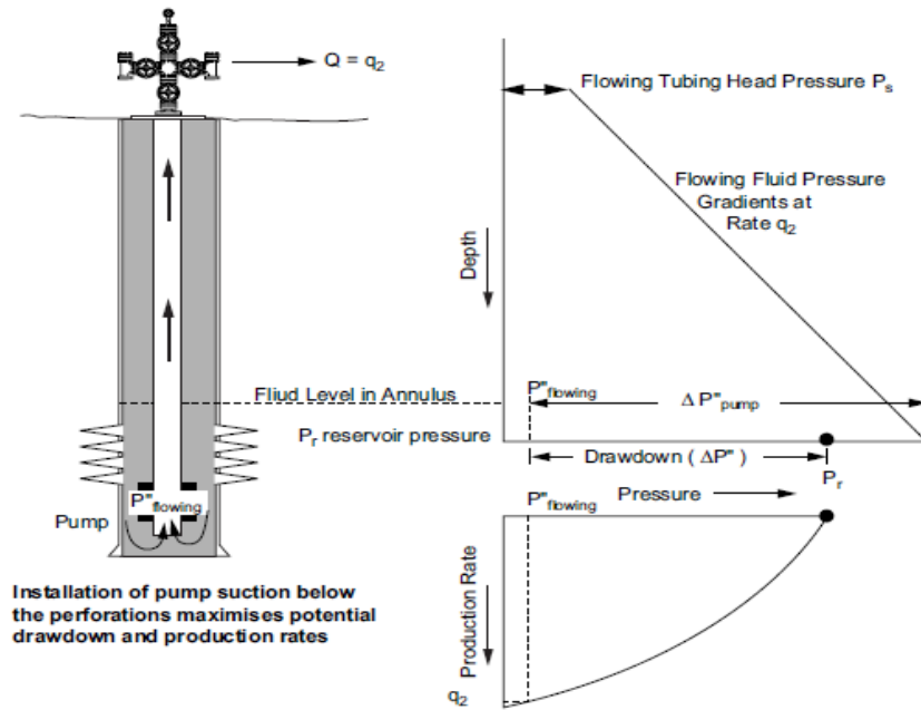
Figure 2.6 Installation of pump suction below perforations increases drawdown and flow rate [15]
