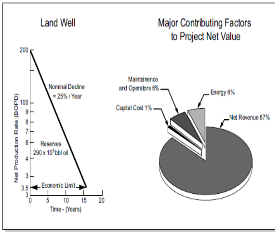
Figure 2.15 Full life cycle economics [15]
