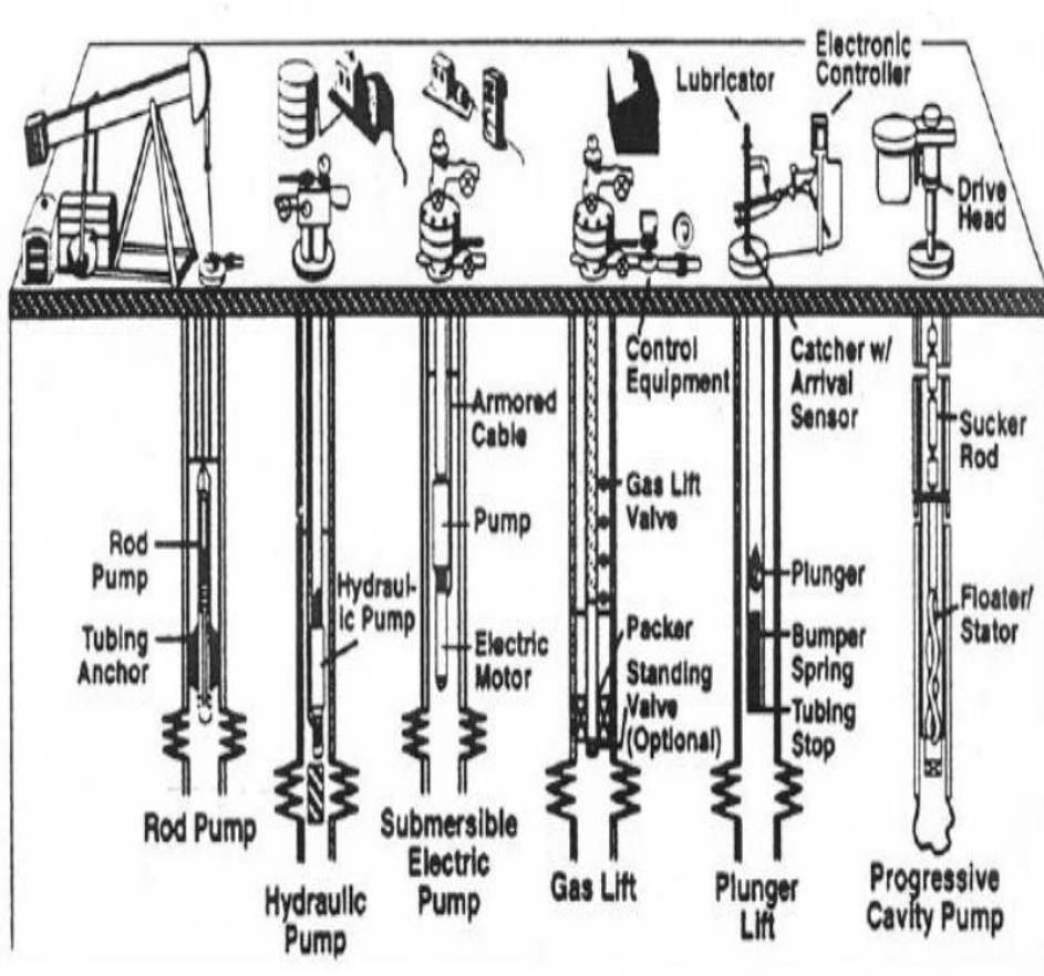
Figure 2.8 Major types of artificial lift techniques
