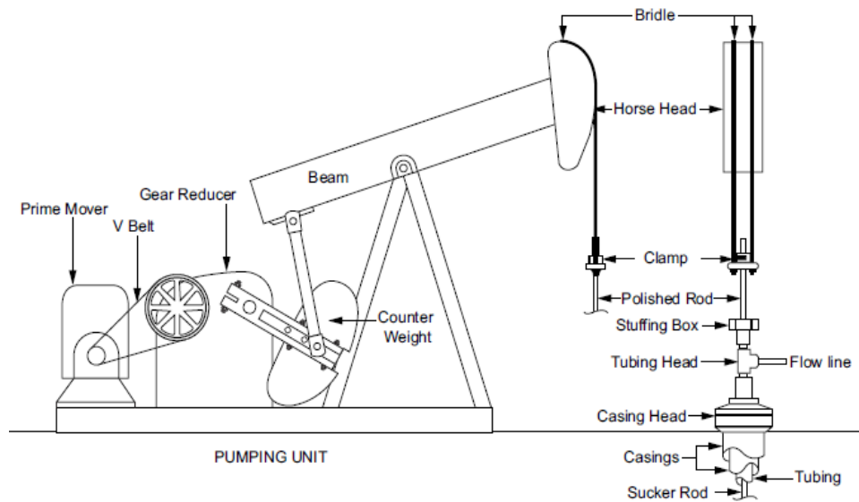
Figure 2.19 Schematic view of Surface equipment [15]
