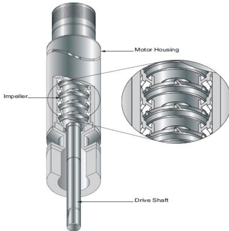
Figure 2.26 Schematic view of ESP pump [15]
