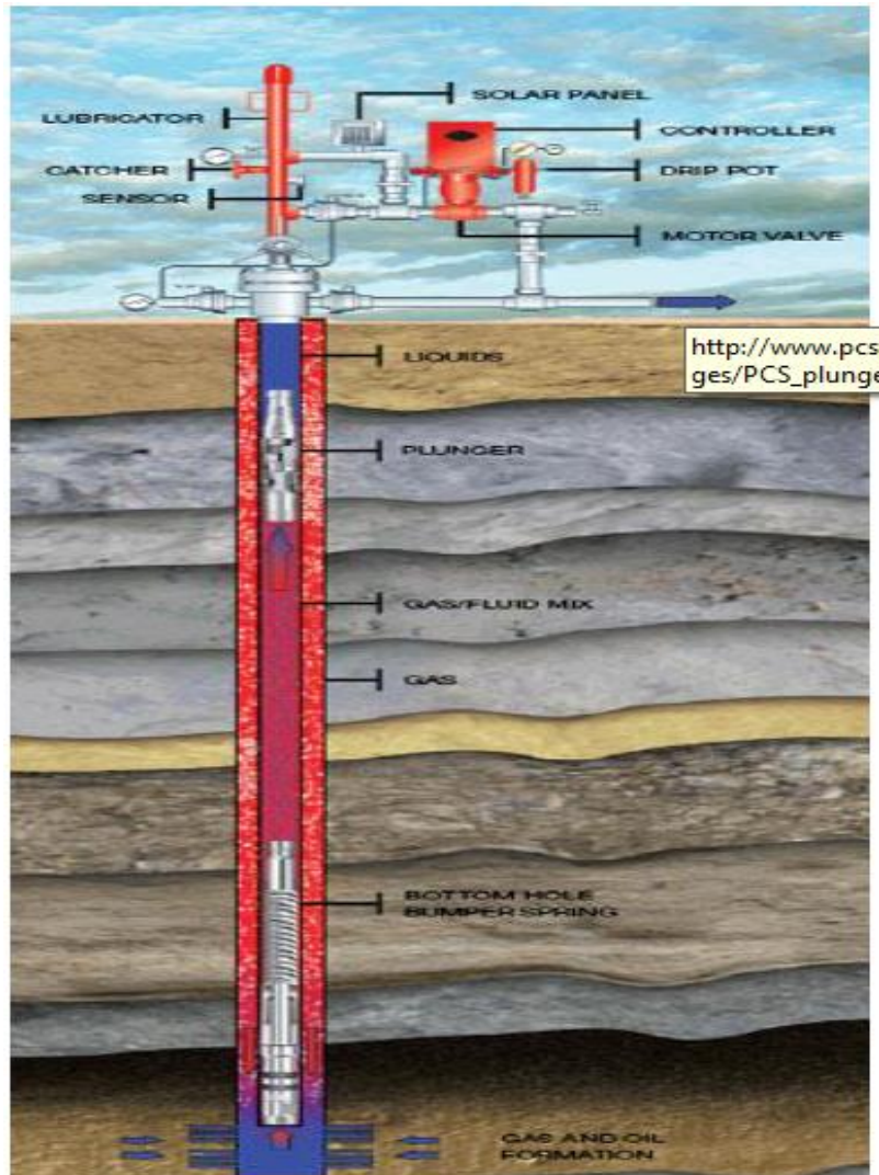
Figure 2.35 Schematic view of Plunger Lift system
