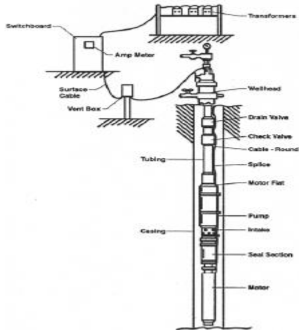
Figure 2.25 Schematic view of ESP
