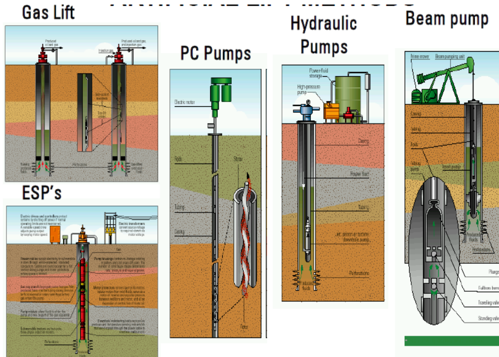
Figure 2.9 Major types of artificial lift techniques [15]
