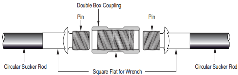
Figure 2.20 Schematic view of Sucker Rod [15]
