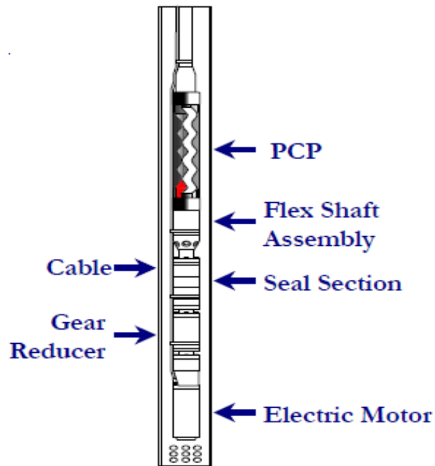
Figure 2.34 Schematic view of ESPCP [8]
