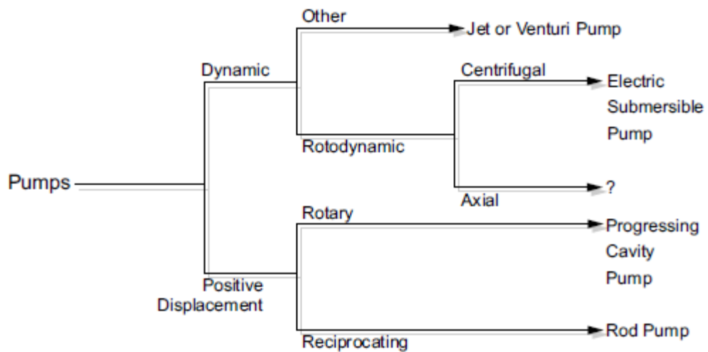
Figure 2.10 Pump classification
