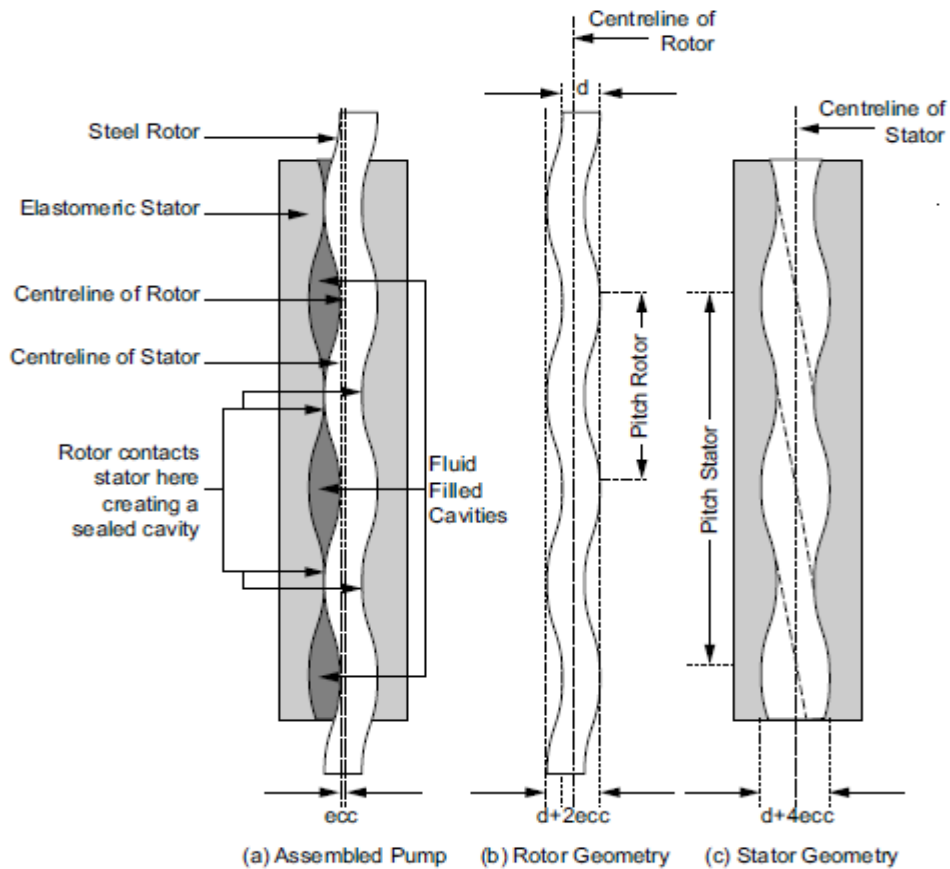
Figure 2.33 Schematic view of PCP and its components [15]
