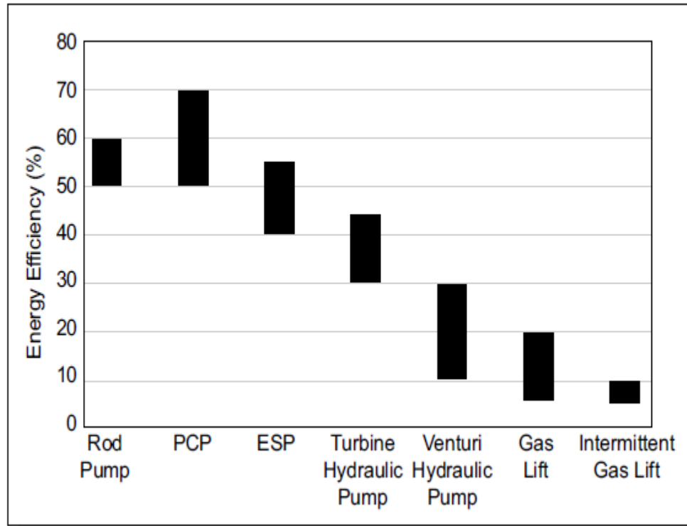
Figure 2.16 Comparison of energy efficiency of different artificial lift types [15]
