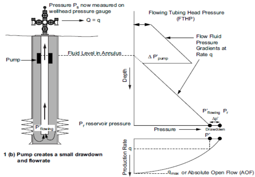
Figure 2.5 Pump creates a small drawdown and flow rate [15]
