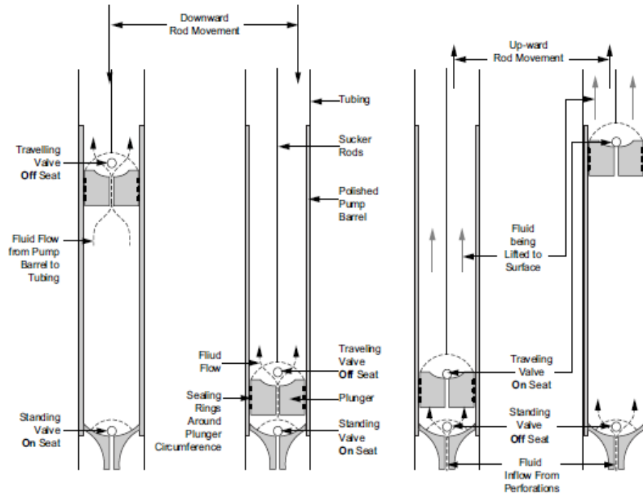
Figure 2.21 Rod Pump operations [15]
