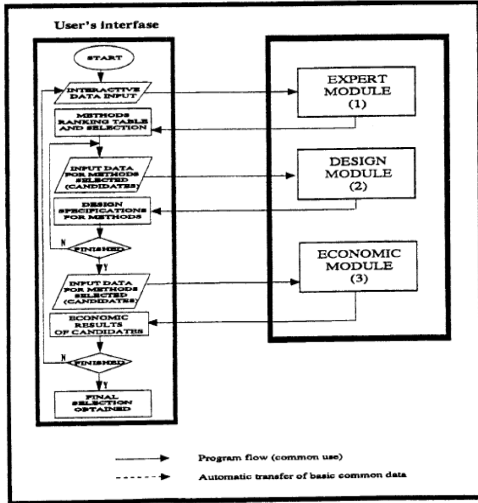
Figure 3.5 ES program flow
