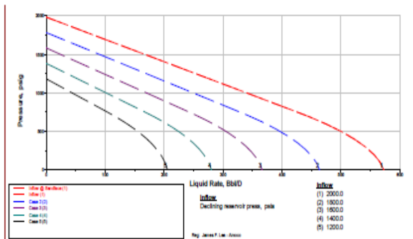
Figure 2.2 IPR curve decreases with time [12]
