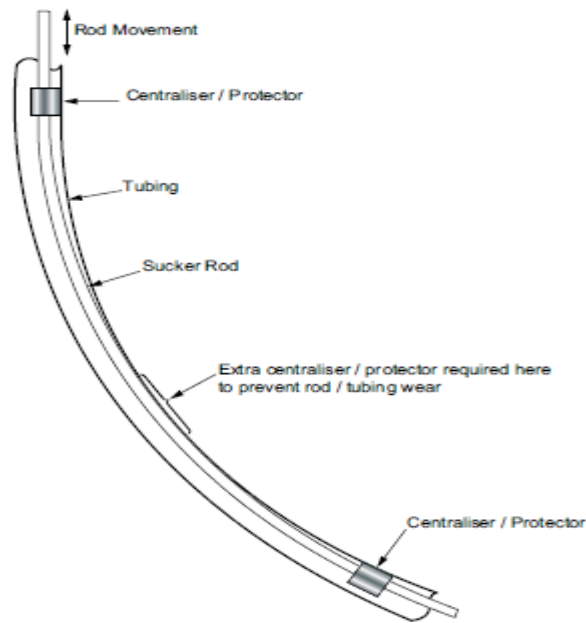
Figure 2.23 Centralizer set in the well [15]
