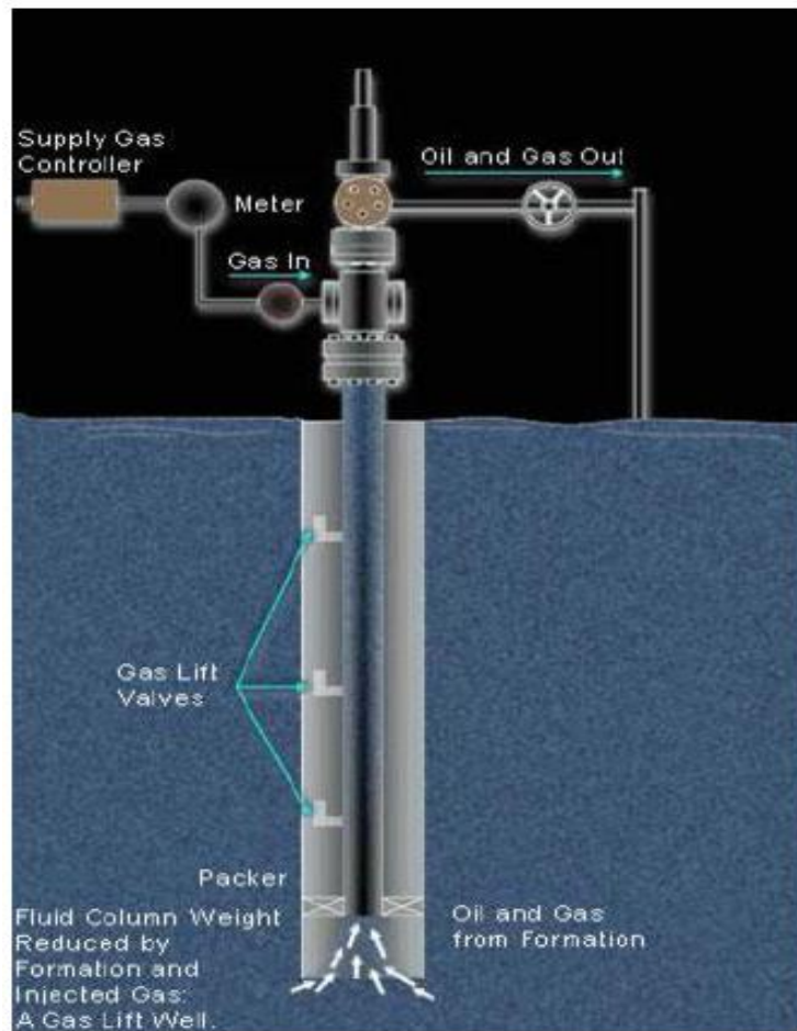
Figure 2.37 Main parts of Gas Lift system [12]
