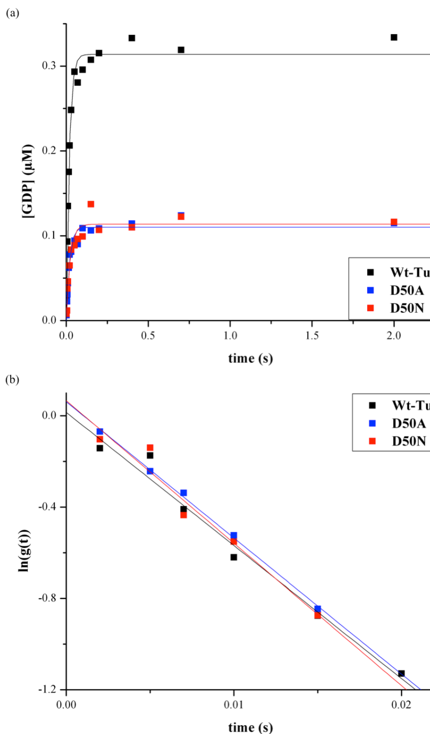
Figure 5.10. Rate of ribosome induced GTP hydrolysis on EF-Tu for wild type and Asp50 mutants in the presence of 80 \mu M Phe-tRNA Phe . (a) The concentration of hydrolyzed GDP ( GDP(t) ) was plotted as a function of time. (b) \ln(g(t)) versus time graph of (a) where the slope gives the k_{GTP} .
