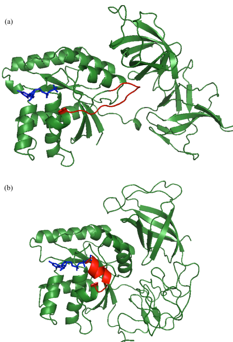
Figure 1.2. Structure of EF-Tu in its GDP (a) and GTP (b) bound states. Switch I region indicated in red and guanine nucleotide in blue color (PDB ID: 1TUI and 2FX3).
