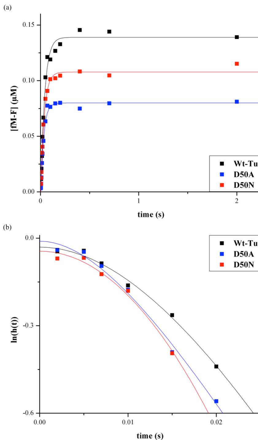
Figure 5.12. The dipeptide formation on ribosomes in the presence of 80 \mu\text{M} tRNA Phe . (a)
