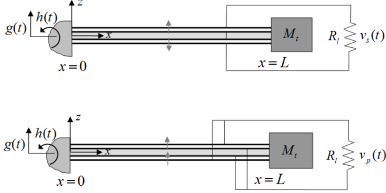
Figure 2.7: Bimorph piezoelectric energy harvesters with a) series connection, b) parallel connection [64].
