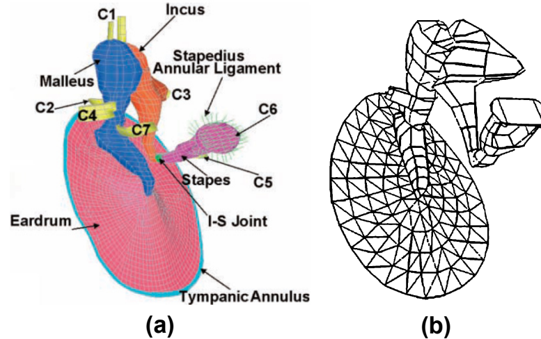
Figure 2.17: FE model of the middle ear for predicting mechanism of ossicular chain a) [127], b) [124].
