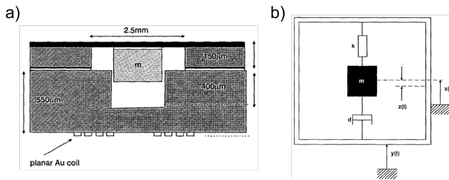
Figure 1.2: a) Schematic view of the microfabricated electromagnetic energy harvester with 0.25 \text{ mm}^3 volume, b) equivalent mass-spring-damper model of the electromagnetic energy harvester [28].
