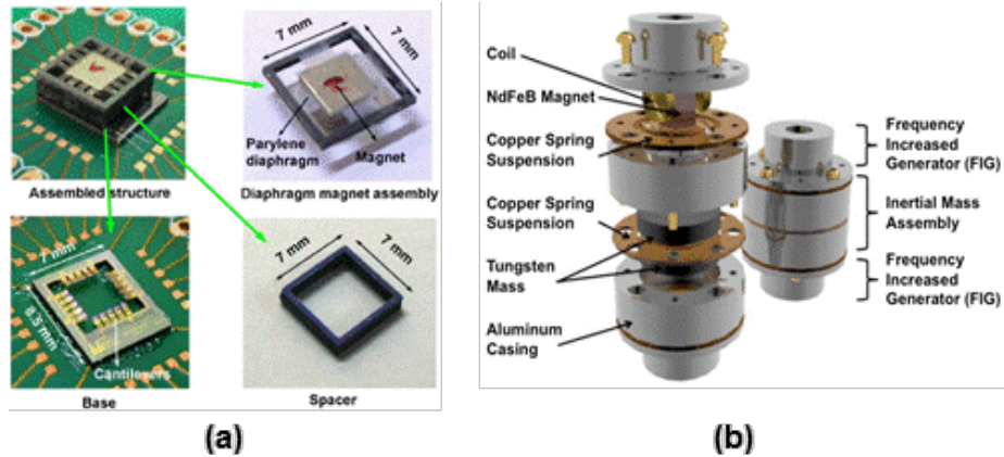
Figure 1.3: Image of the frequency-up converter electromagnetic energy harvester assembly by a) [34] b) [36].
