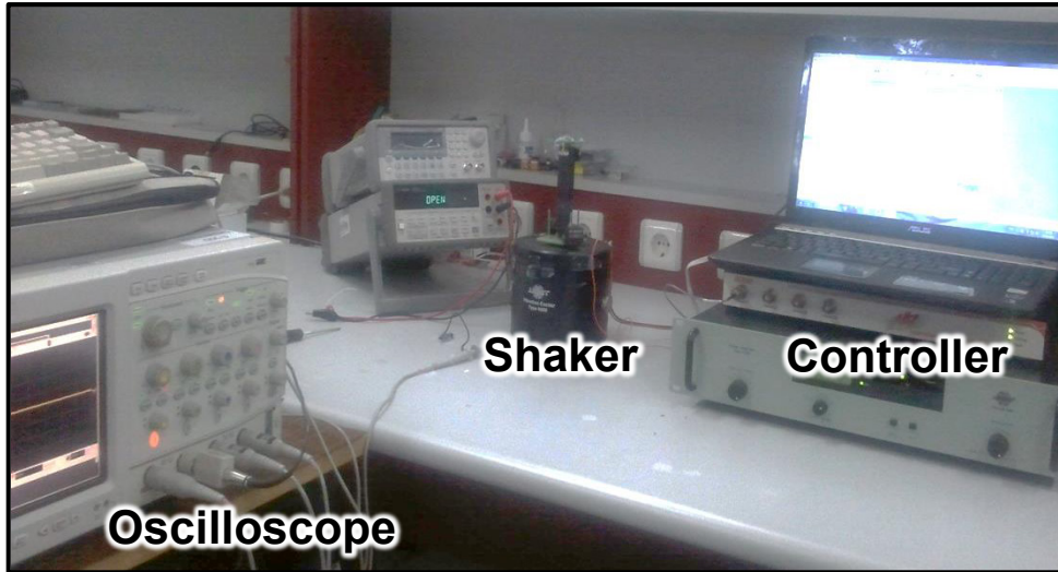
Figure 3.16: Experimental setup for characterization of the harvesters.
