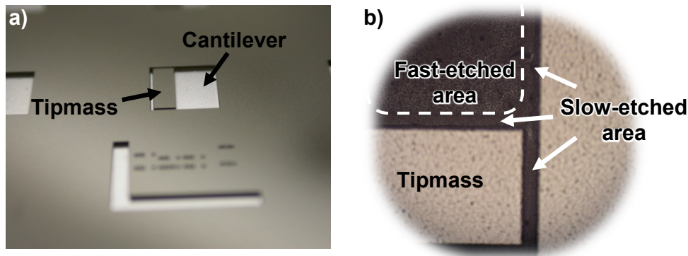
Figure 3.13: Image of the backside of the wafer showing a) tipmass and cantilever structure in the midst of backside DRIE process, b) fast and slow-etched areas.
