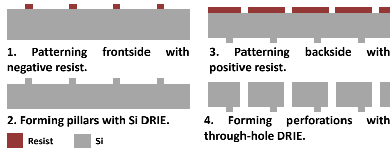
Figure A.4: Fabrication flow of the perforated handling wafer.
