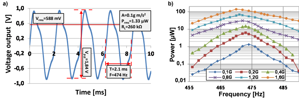
Figure 3.18: a) Generated voltage waveform from the MEMS harvester at its resonance frequency with an input acceleration of 0.1g, b) rms power output at various g levels.
