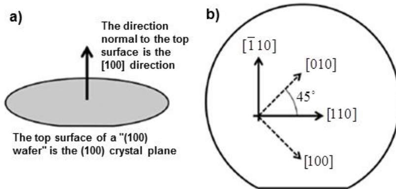
Figure 2.11: Crystal directions of (100) wafer, a) isometric view and [100] direction, b) flat direction and axes [89].
