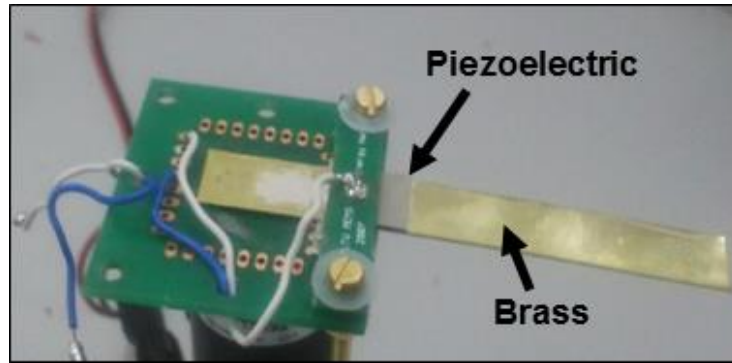
Figure 2.14: Manufactured macro-scale piezoelectric energy harvester prototype [114–116].
