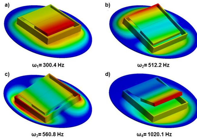
Figure 2.28: First four mode shapes of the coupled structure, which is optimized by using an excitation frequency of 1 kHz.
