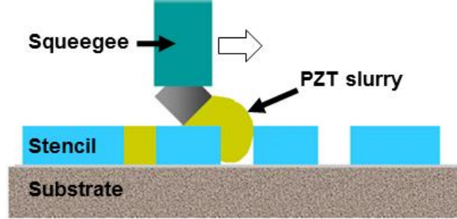
Figure 3.3: Screen printing technique [186].
