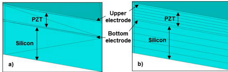
Figure 2.27: View through the thickness of the harvester with a) free meshed structure, a) sweep meshed structure.
