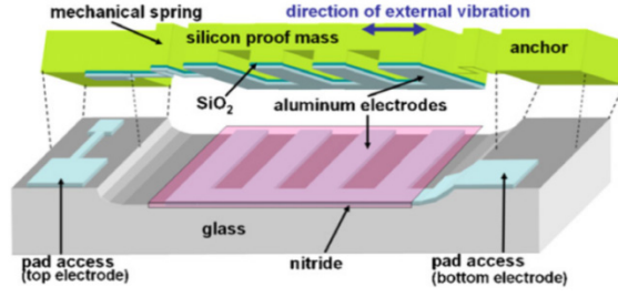
Figure 1.5: 3D schematic view of the electrostatic energy harvester [38].
