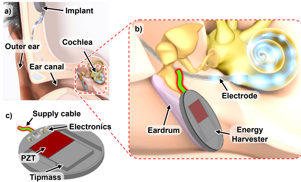
Figure 2.1: The proposed method: converting eardrum vibrations to electricity, a) peripheral auditory system of a cochlear implant user, b) placement of the energy harvester onto the eardrum, c) close-up view of the harvester.
