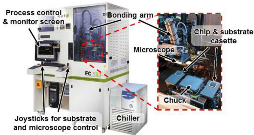
Figure 3.4: SET FC150 flip chip bonder system [193].
