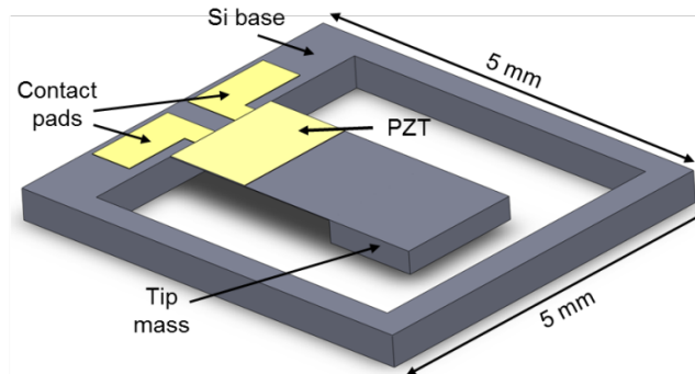
Figure 2.8: Proposed MEMS piezoelectric energy harvester.
