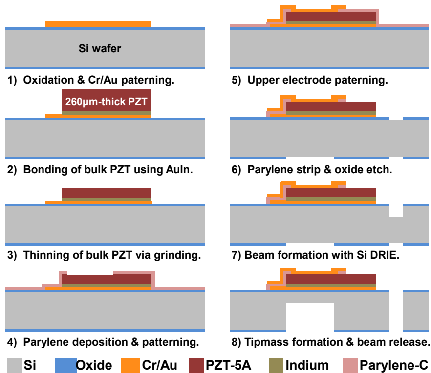
Figure 3.9: Fabrication flow of the MEMS piezoelectric energy harvester [12].
