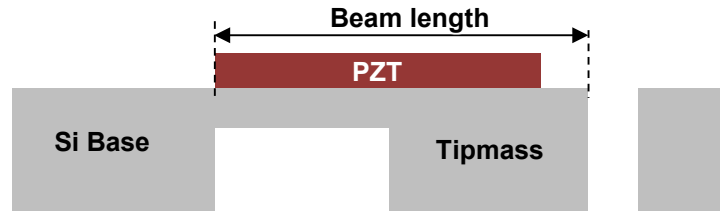
Figure 3.1: Cross-section of MEMS harvester structure.
