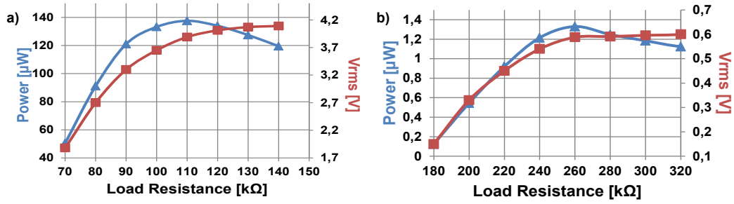
Figure 3.19: Generated rms power and voltage vs. the load resistance at a) 1.6g, b) 0.1g.
