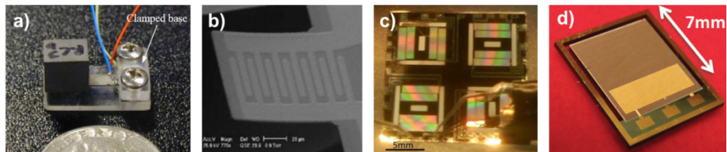
Figure 1.9: a) A macro-scale piezoelectric energy harvester [15], b) microfabricated thin-film PZT energy harvester with interdigitated electrodes [43], c) nonlinear doubly clamped cantilever type wide-bandwidth energy harvester [44], d) piezoelectric energy harvester using bulk piezoceramics [37].
