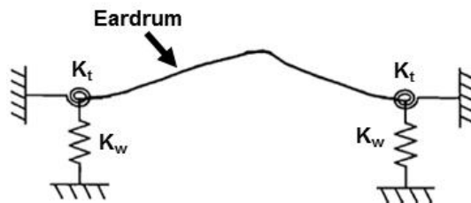
Figure 2.21: Proposed elastic boundary condition models for FE model of eardrum by Wada et al. [124].
