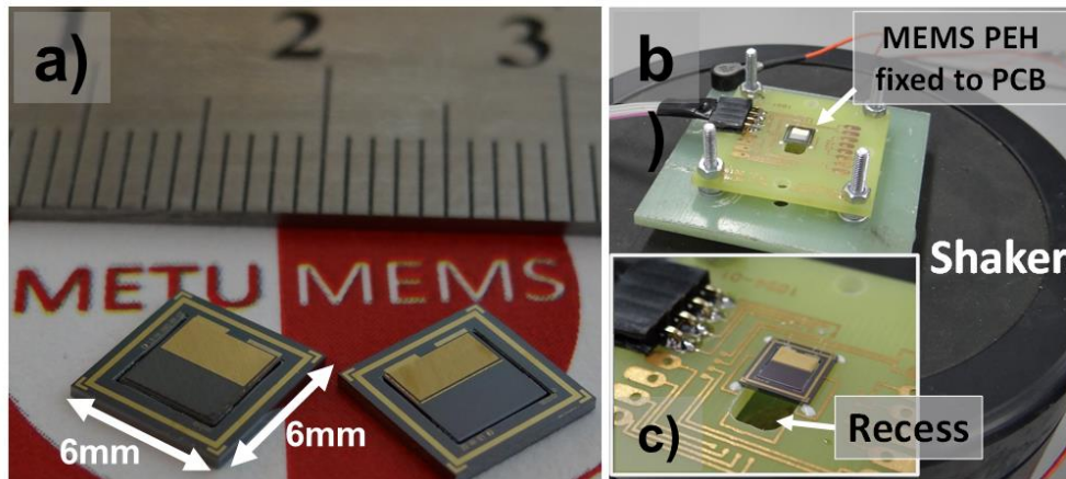
Figure 3.17: a) Fabricated MEMS piezoelectric energy harvesters with 6 \times 6 \text{ mm}^2 footprint and 20 \text{ mm}^3 volume, b) MEMS harvester assembled to PCB and mounted on shaker table, c) close-up view of the MEMS harvester on PCB showing recess below the tipmass.
