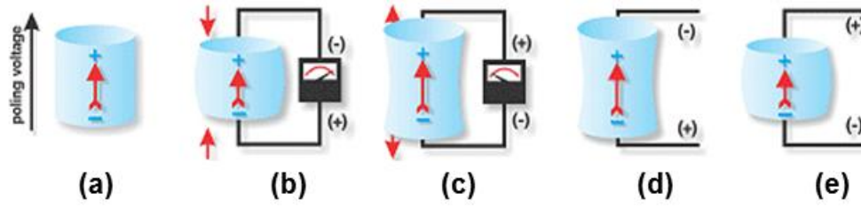
Figure 1.7: Direct and inverse piezoelectric effects, a) poling direction of a disk type piezoceramics, b) disk compressed: generated voltage has same polarity as poling voltage, c) disk stretched: generated voltage has polarity opposite that of poling voltage, d) applied voltage has same polarity as poling voltage: disk lengthens, e) applied voltage has polarity opposite that of poling voltage: disk shortens [39].
