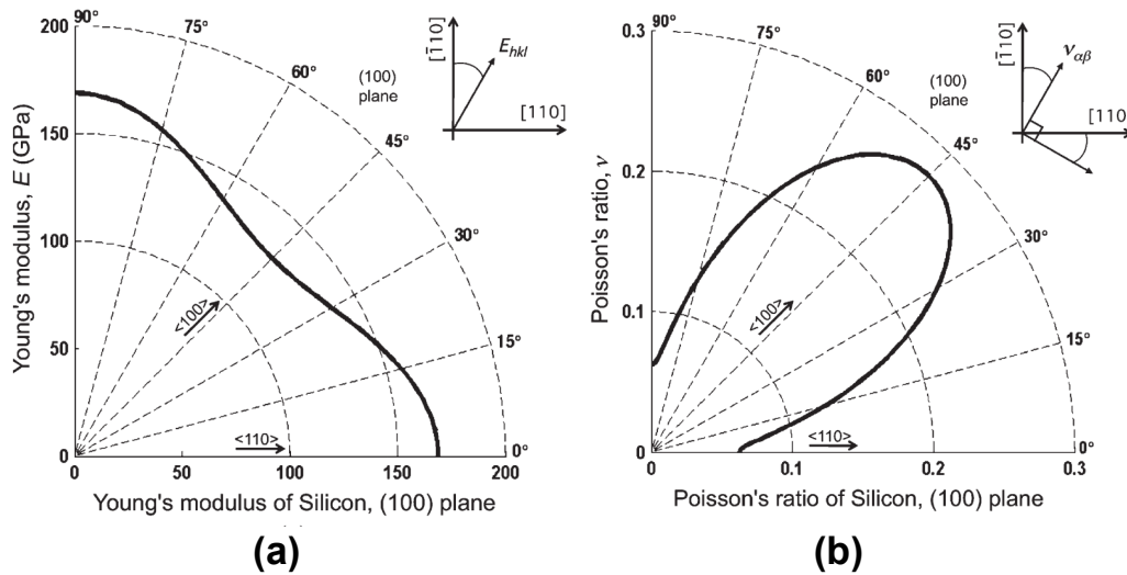
Figure 2.12: a) Young's Modulus, b) Poisson's ratio value with respect to wafer's crystal directions [89], [104–107].
