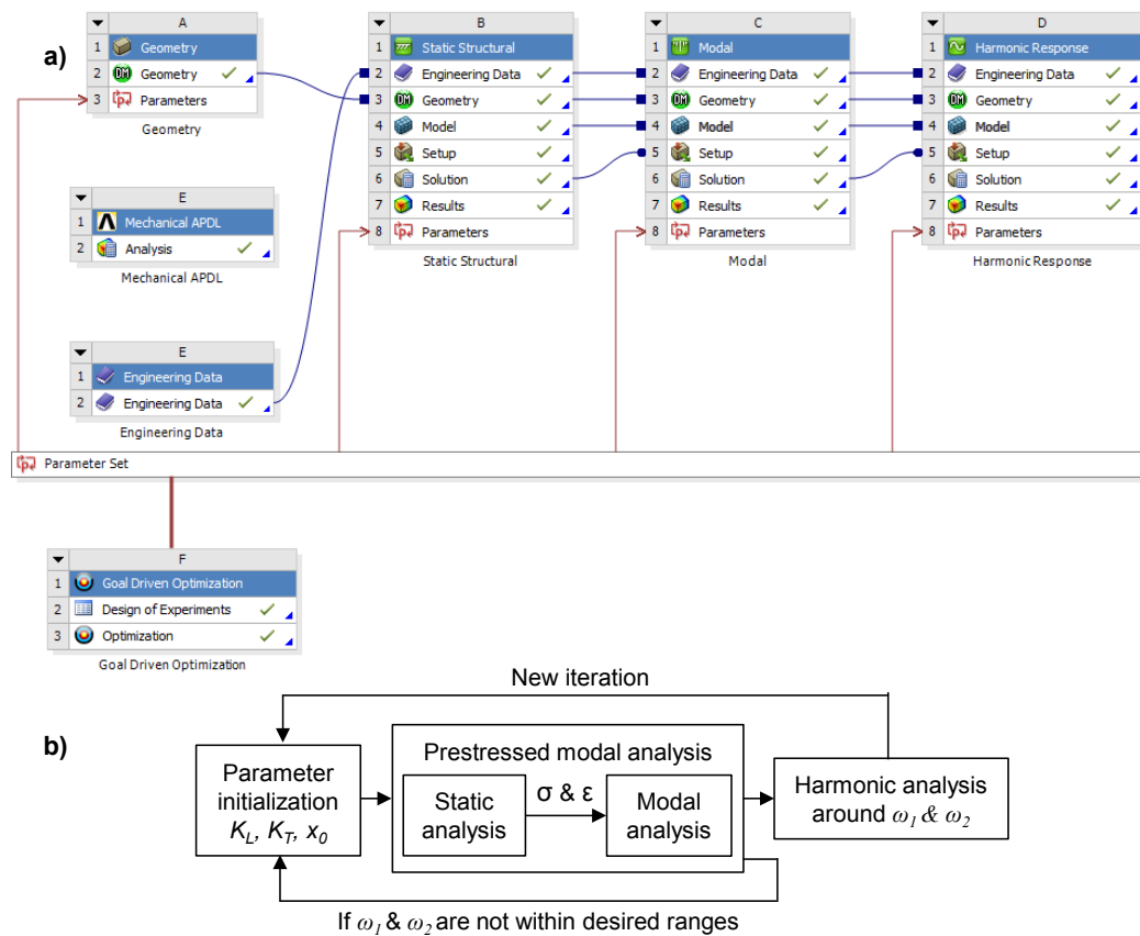
Figure 2.22: a) User interface of the ANSYS Workbench module for the developed optimization routine, b) conditional representation of the developed optimization routine.
