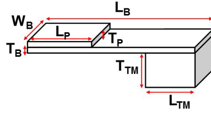
Figure 2.9: Dimensions of the MEMS piezoelectric energy harvester.
