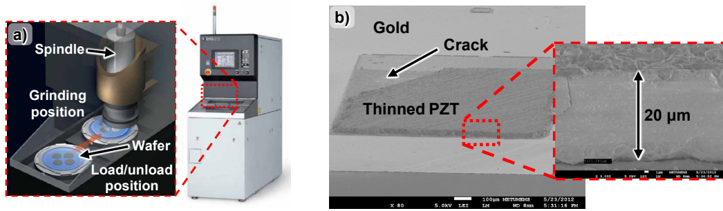
Figure 3.8: a) Disco DAG810 grinder machine [208], b) PZT sample thinned to 20 \mu\text{m} on gold surface.
