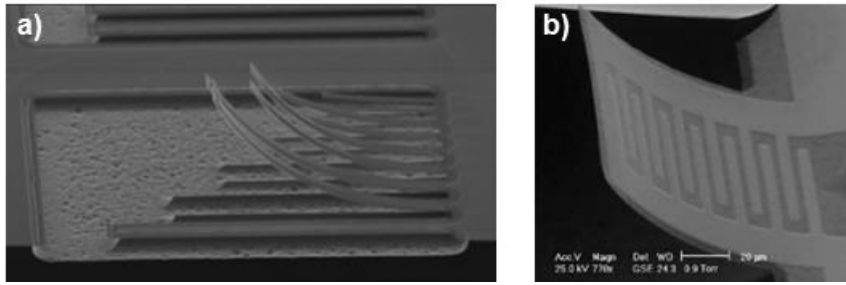
Figure 3.2: SEM images of curled beams fabricated via sol-gel PZT coating method, a) array of cantilevers [177], b) piezoelectric beam with interdigitated electrodes [43].
