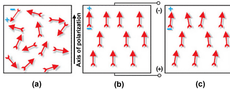
Figure 1.6: Poling a piezoelectric ceramic, a) random orientation of polar domains before polarization, b) polarization in DC field, c) remanent polarization after electric field removed [39].
