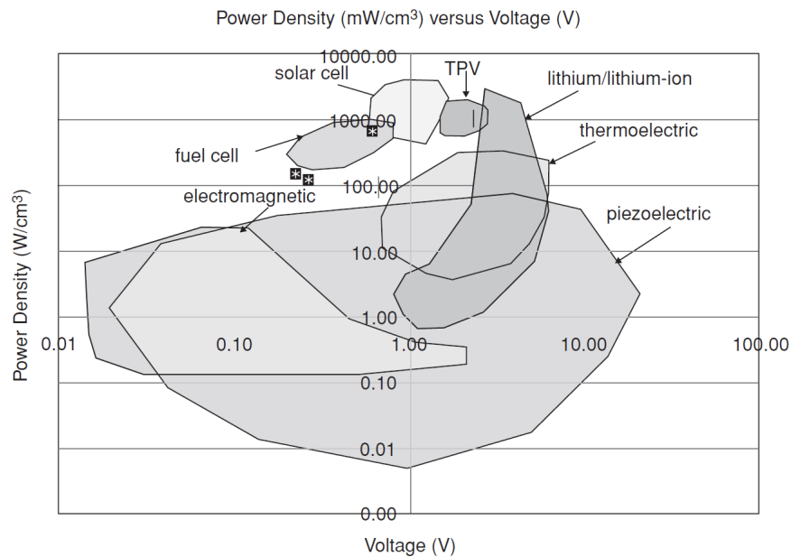
Figure 1.1: Power density versus voltage plot for various transduction mechanisms and lithium-based supplies [20].
