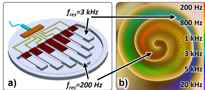
Figure 4.7: a) Proposed multi-frequency MEMS harvester that natural frequency of each cantilever corresponds to a frequency band in cochlea, similar to a frequency discretized cochlea model, b) frequency range of cochlea [217].
