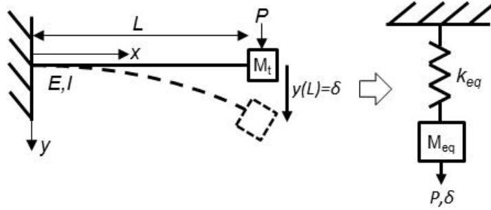
Figure 2.6: Fixed-free type cantilever beam with a tip mass and its lumped model.
