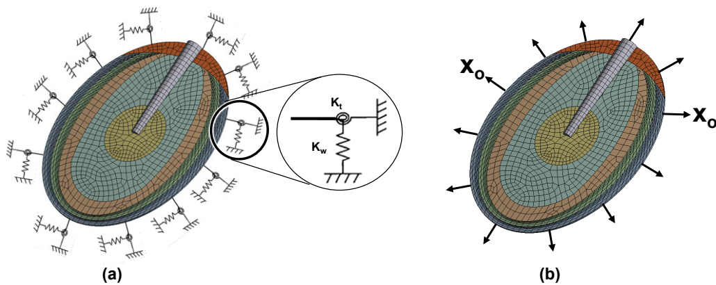
Figure 2.23: FE model of eardrum a) where linear and torsional springs attached to the nodes located at the boundary, b) where a predetermined displacement, x_0 , is applied normal to the boundary.
