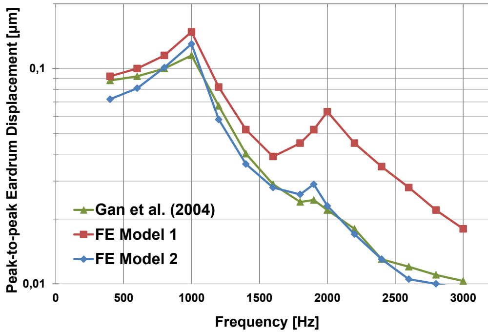
Figure 2.24: Comparison of the developed eardrum FE models with the measured eardrum frequency response curve at 90 dB SPL [129]. (FE Model 1: springs are attached to the boundary, FE Model 2: stretching displacement is applied to the boundary).
