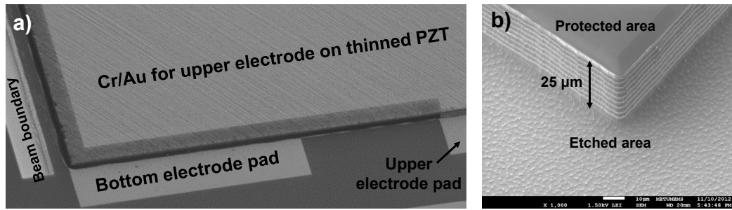
Figure 3.12: SEM image of the harvester showing a) PZT, contact pads, and Si-etched region, b) close-up view from the corner of the cantilever after frontside DRIE.
