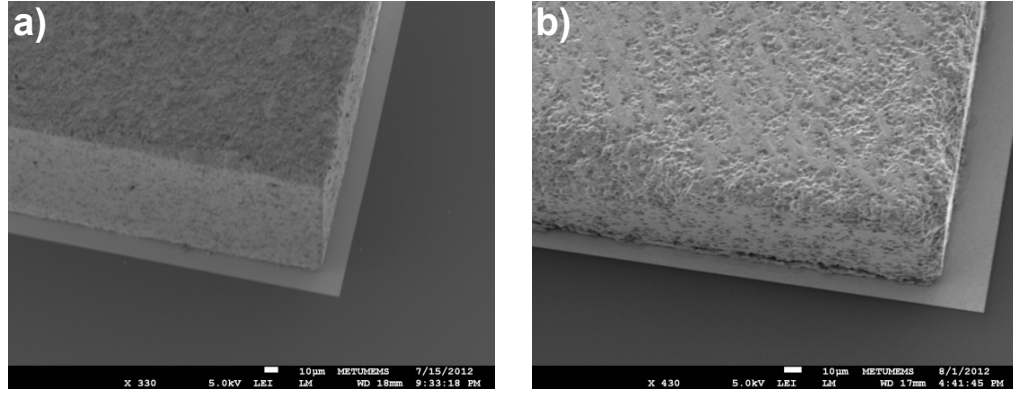
Figure 3.10: Bonded PZT sample a) before thinning, b) after thinning.
