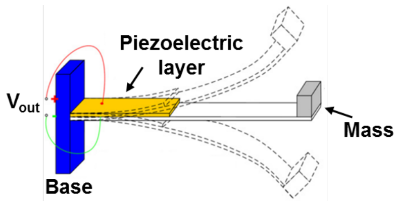
Figure 2.3: Conventional piezoelectric energy harvester design, a fixed-free cantilever beam with tip mass [58].
