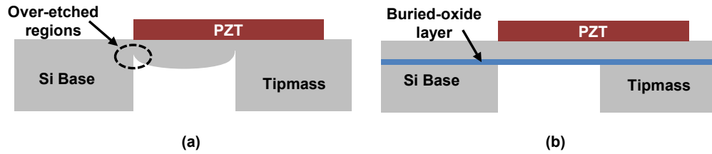
Figure 3.15: Cross-sectional view of a) the fabricated harvester showing over-etched regions around sidewalls, b) the harvester fabricated using SOI wafer.
