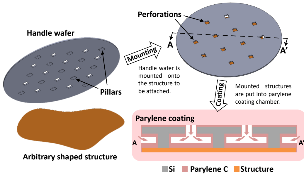
Figure A.1: a) Handling of thin structures using parylene coating, b) cross section of A-A'.
