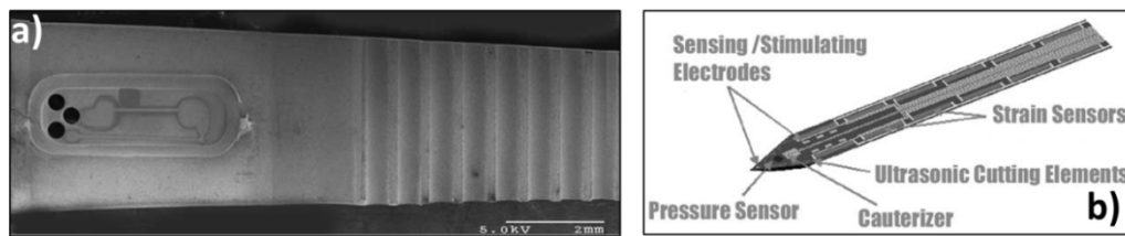
Figure 1.10: a) Embedded strain gauges and temperature sensors on a micro gripper, b) the data knife smart scalpel developed by Verimetra, Inc. [47].
