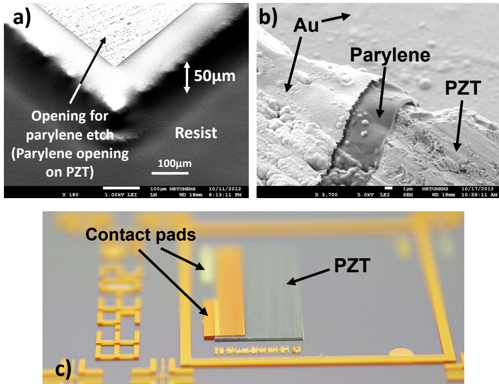
Figure 3.11: a) SEM image of lithography process on a 50 \mu\text{m} -thick PZT on Si, b) close-up view of the upper electrode through PZT edge, c) side view of the harvester after metal patterning.
