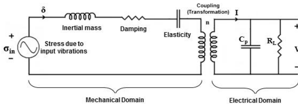
Figure 2.4: Representation of piezoelectric energy harvester with lumped electrical elements [15].
