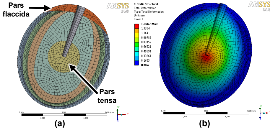
Figure 2.20: a) Meshed FE model of the eardrum showing six different sections of the eardrum including pars flaccida and pars tensa with 6781 nodes, b) static analysis results showing the depth of the central region.
