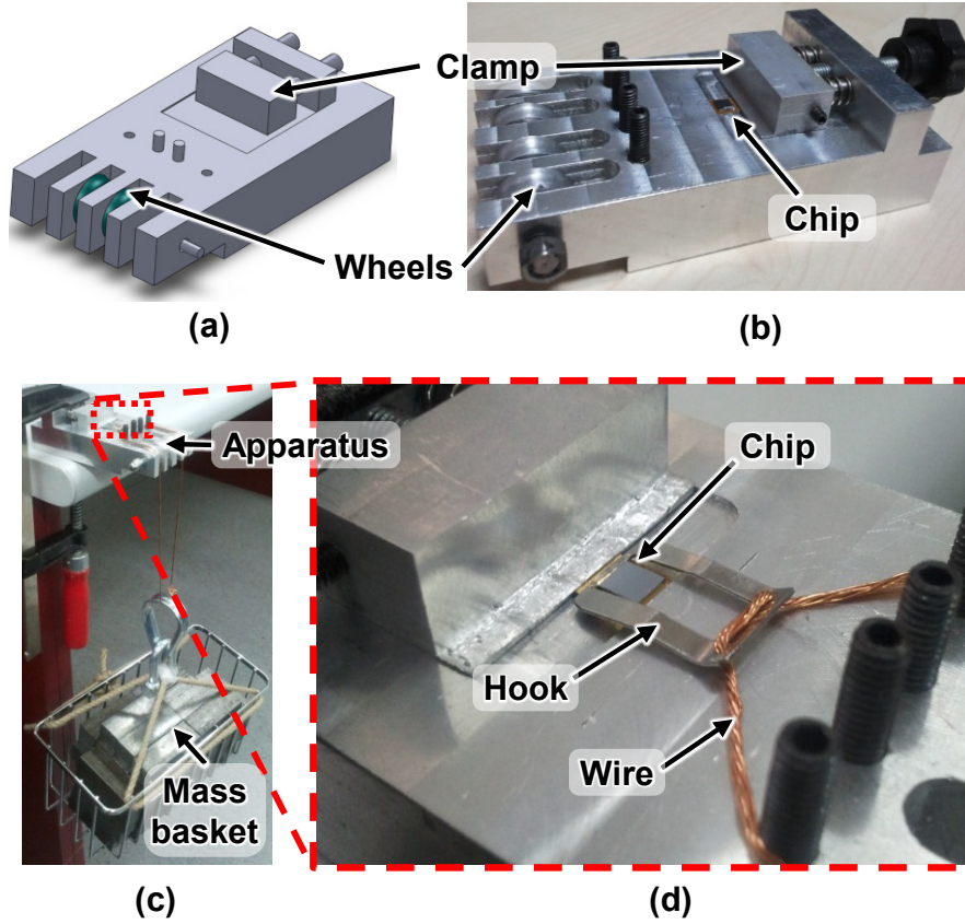
Figure 3.5: a) CAD model of the designed shear test apparatus, b) manufactured apparatus, c-d) experimental setup for the shear test measurement of gold thermocompression-bonded samples.
