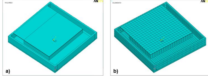
Figure 2.13: Developed parametric MEMS piezoelectric energy harvester model using FEM program, a) unmeshed, b) meshed.
