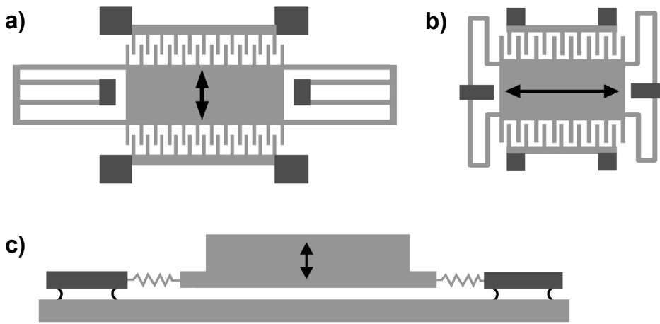
Figure 1.4: Typical electrostatic energy harvester designs, a) in-plane overlap, b) in-plane gap closing, c) out-of-plane gap closing converter.
