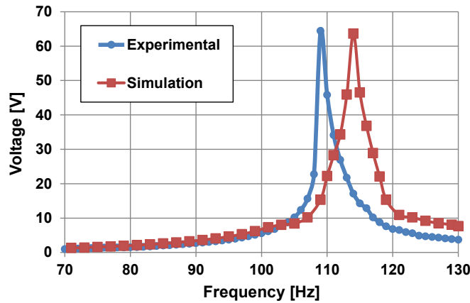
Figure 2.15: Comparison of voltage output versus frequency plot of the experimental results and simulations.
