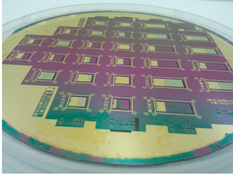
Figure 3.14: Final image of the frontside of the process wafer.
