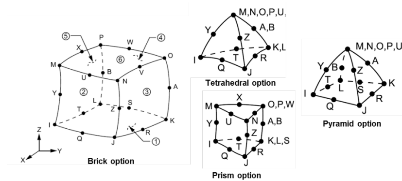
Figure 2.10: SOLID186 structural solid and SOLID226 coupled-field solid geometry with various shape options [100].
