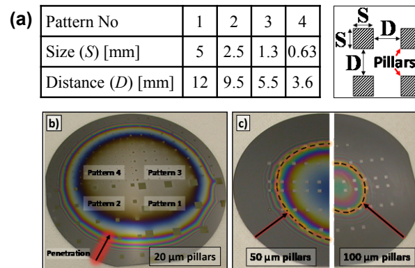
Figure A.3: a) Pillar patterns b) wafer with various patterns c) wafers with pattern similar to Pattern 2 and pillars with height of 50 \mu\text{m} and 100 \mu\text{m} .
