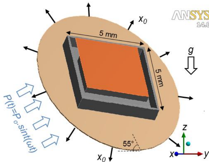
Figure 2.25: FE model of the energy harvester mounted on the eardrum showing the boundary conditions and orientation of the eardrum. Eardrum is oriented at an angle of 55^\circ to the horizontal axis (y-axis), and gravitational acceleration is applied along vertical axis (z-axis). Pressure, P(t) , is applied normal to the membrane surface.
