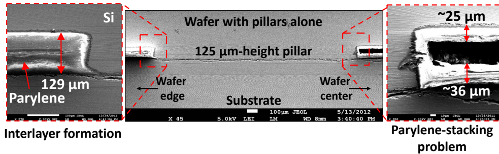
Figure A.2: Cross sectional SEM image around a) fully filled side, b) pillar, c) partially filled side.
