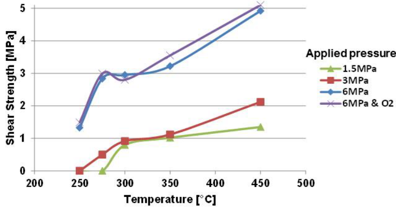
Figure 3.7: Experimental results of the bonded samples with gold thermocompression method.
