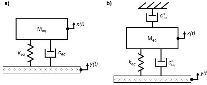
Figure 2.5: Lumped parameter model of the base excitation problem used for representation of vibration-based energy harvesters a) widely referred lumped model, b) modified model representing more precise model of air damping mechanism proposed by Erturk et al. [64].
