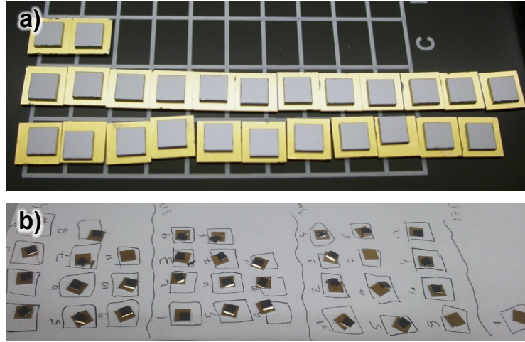
Figure 3.6: Gold thermocompression bonding a) samples before shear test, b) cracked samples after shear test.
