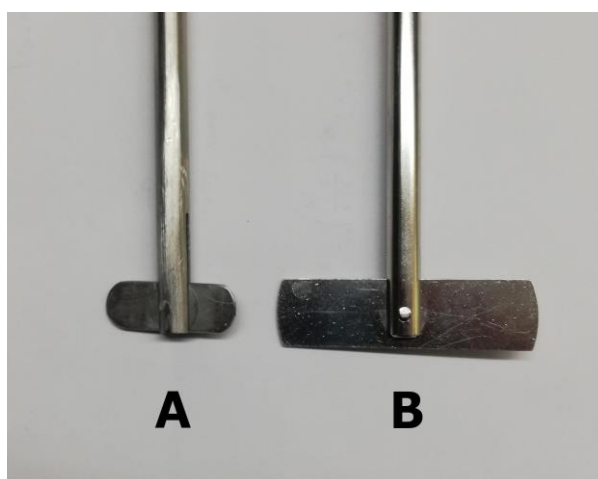
Figure 3.16. Rotors: Rotor A (1x3.1 cm), Rotor B (1.5x5.8 cm)
