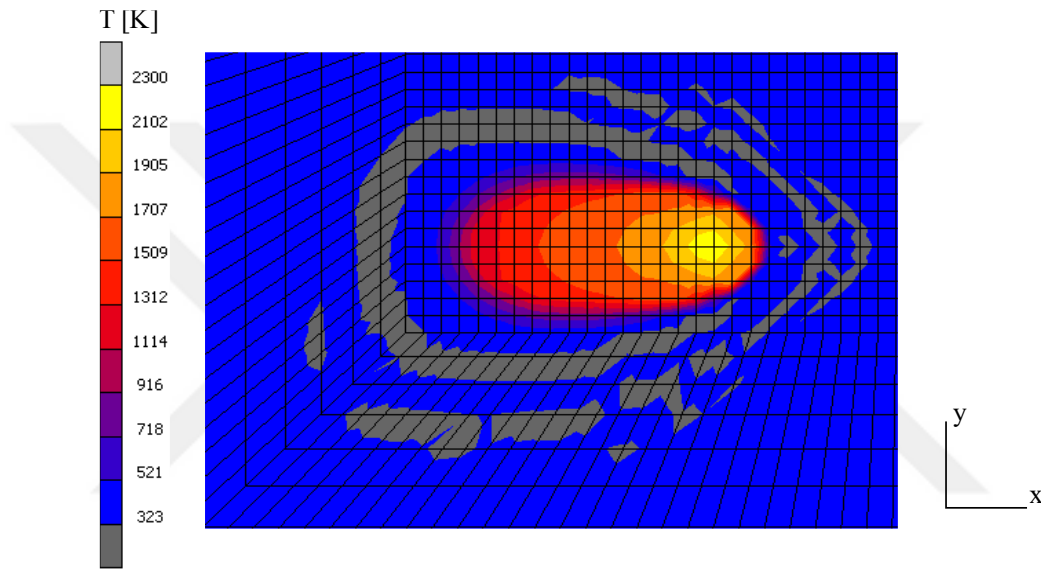
Figure 3-9: Heat affected zone with a mesh refinement of %50.
