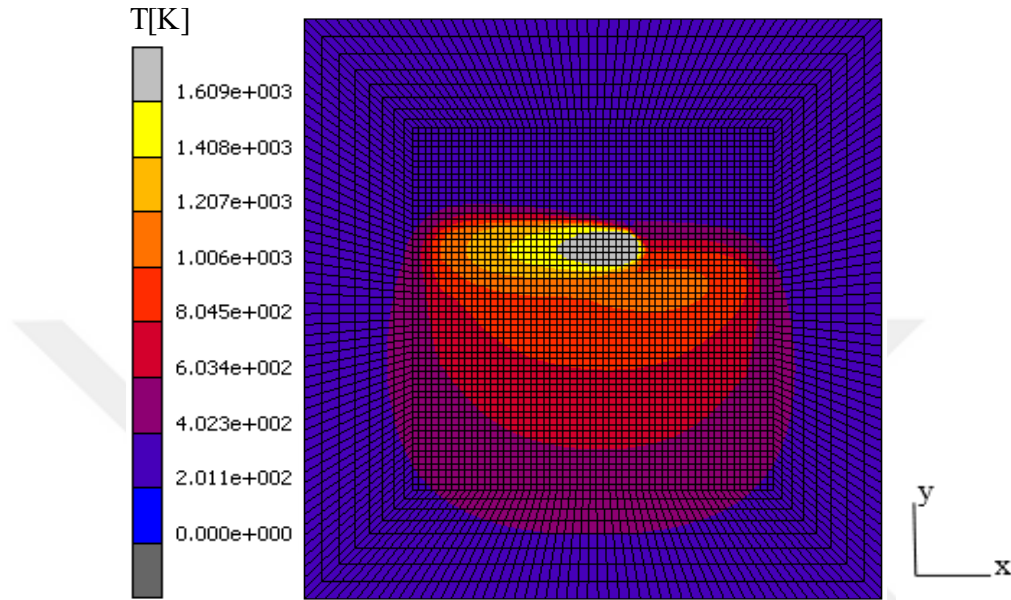
Figure 5-1: Temperature distribution at t=0.00899 s.
