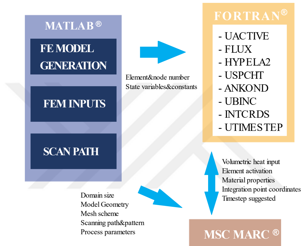
Figure 3-5: Block diagram for the model generation and FE analysis.
