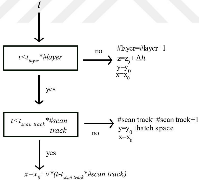
Figure 3-11: Scan path algorithm.
