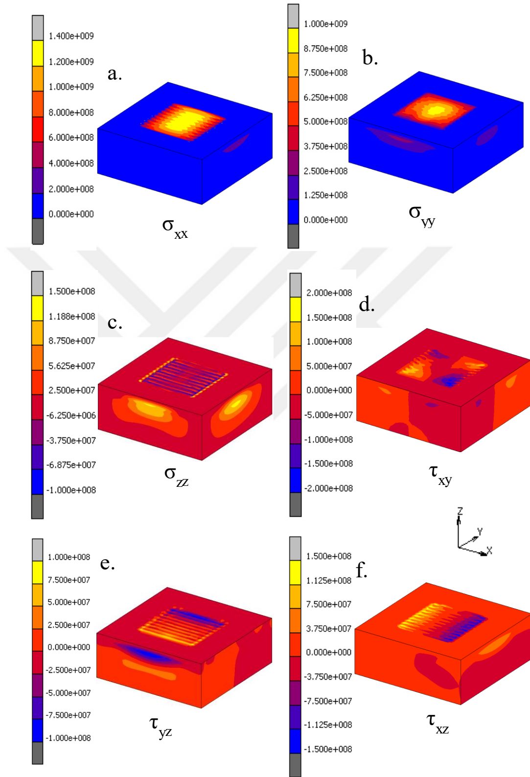
Figure 5-11: Stresses after the deposition of the first layer a. \sigma_{xx} [MPa] b. \sigma_{yy} [MPa] c. \sigma_{zz} [MPa], d. \tau_{xy} [MPa] e. \tau_{yz} [MPa] f. \tau_{xz} [MPa].
