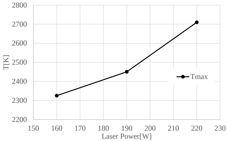
Figure 5-4: Maximum achieved temperature during deposition against varying laser power.
