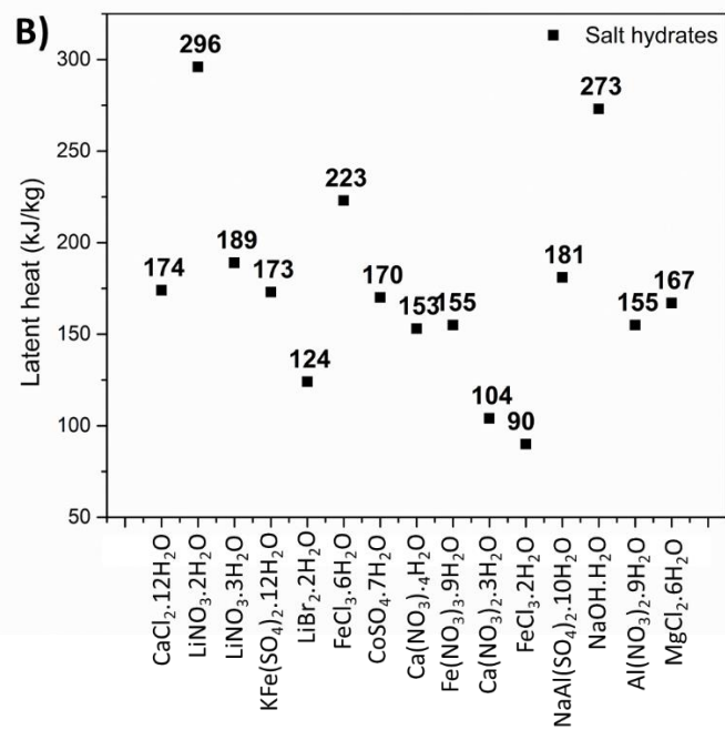
Figure 7. (A) Melting temperatures and (B) latent heat of fusion values of salt hydrate type PCMs.
