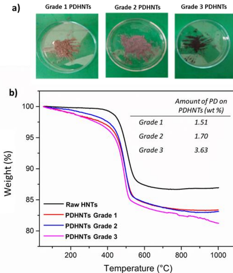
Figure 26. a) Photographs of grade 1, grade 2 and grade 3 PDHNTs, b) TGA analysis of separated PDHNTs.
