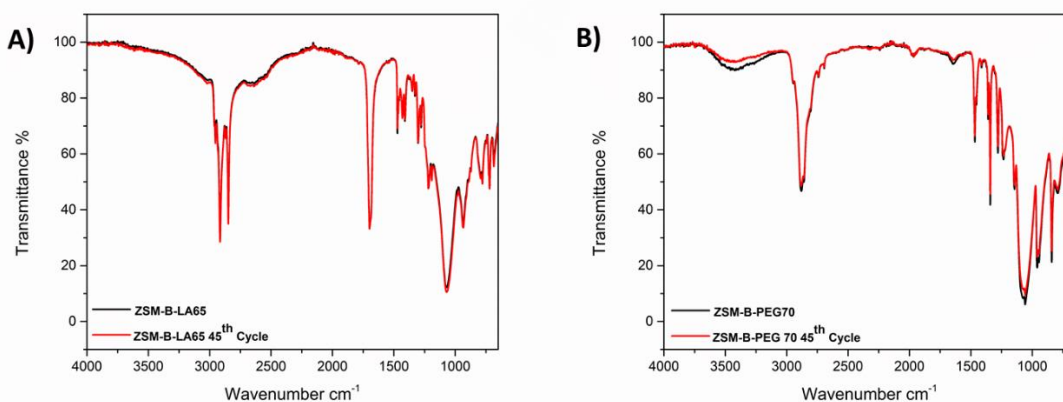
Figure 50. FT-IR analysis of accelerated thermal cycles for (A) ZSM-B-LA65 and ZSM-B-PEG70 (B) end of 45 cycles.
