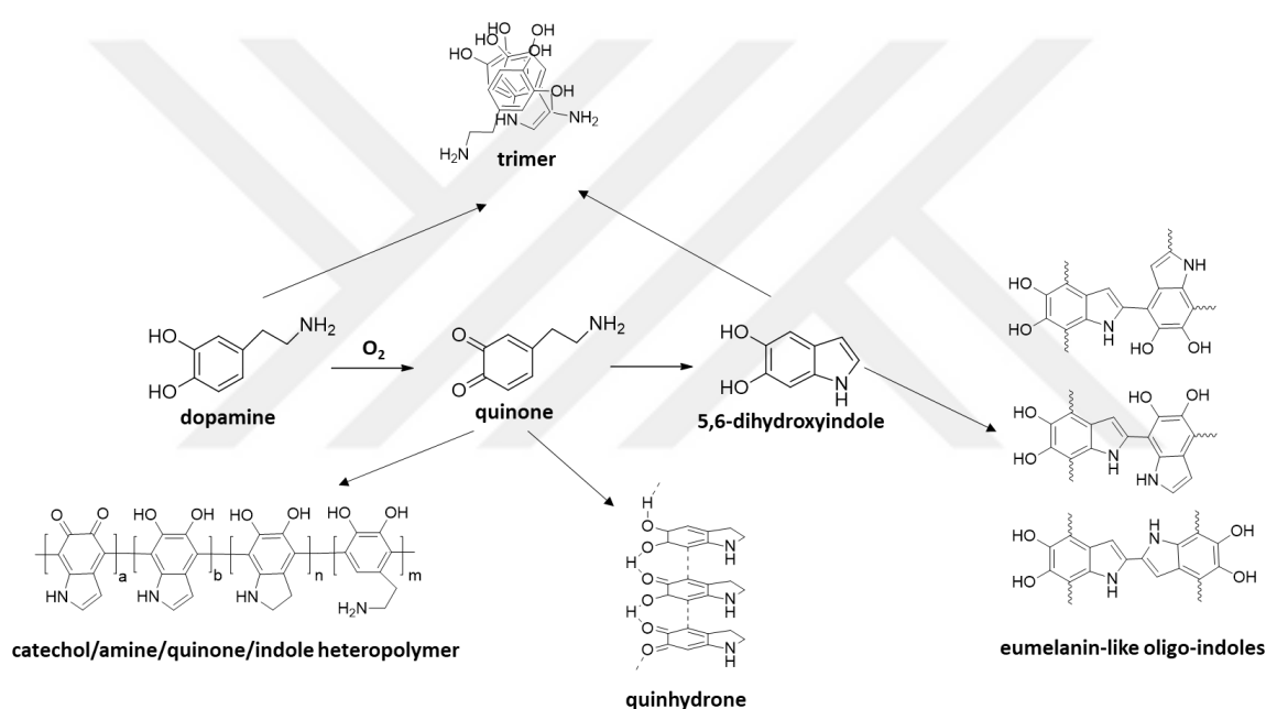
Figure 2. Theories on PDA structure and formation.
