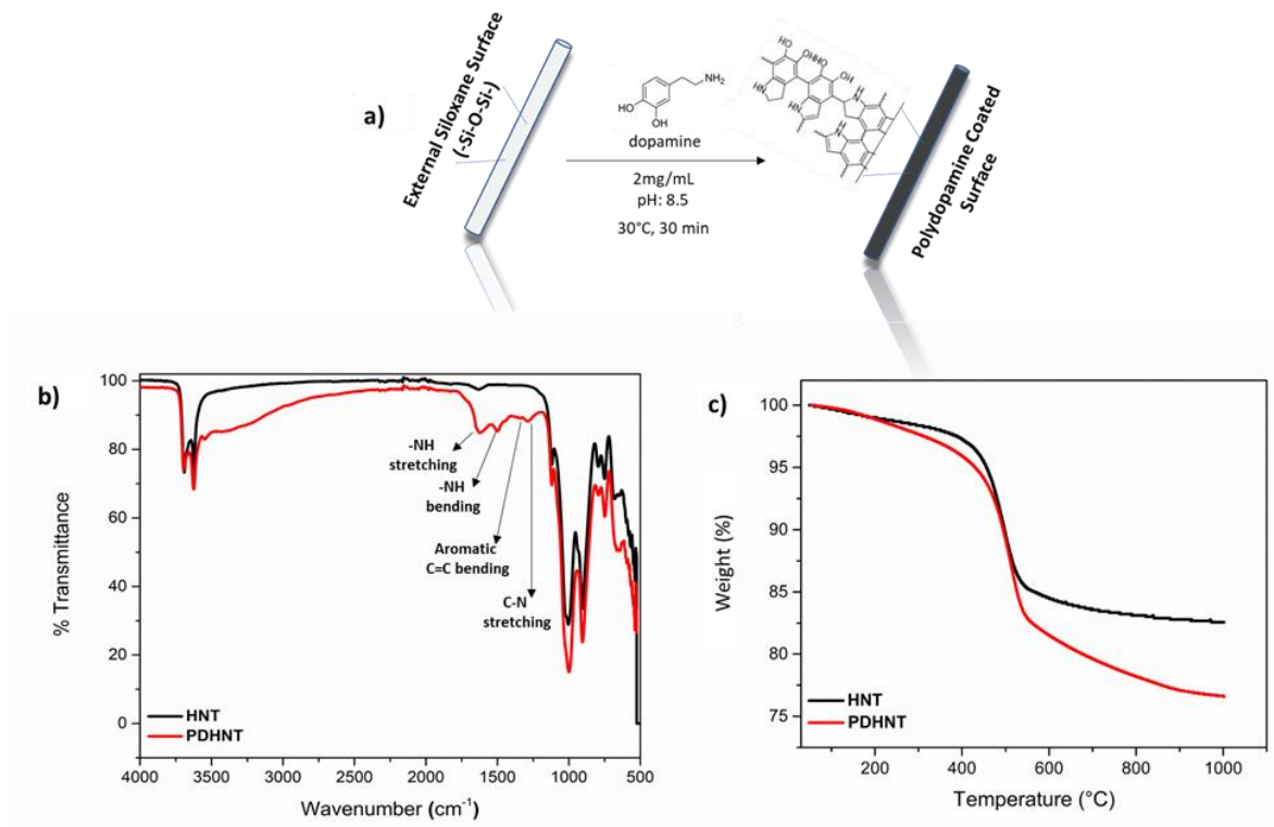
Figure 23. Coating of HNTs with polydopamine (a), FT-IR (b) and TGA (c) analysis of raw HNTs and PDHNTs.
