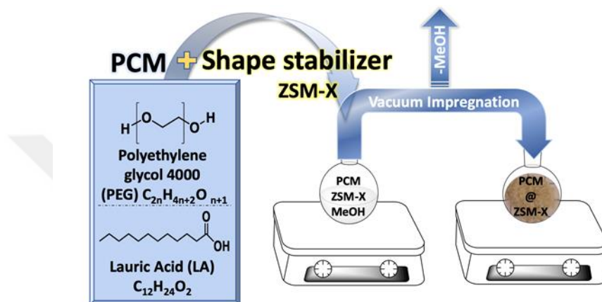
Figure 45. Schematic representation of the composite preparation.
