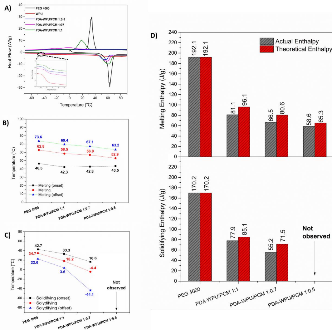
Figure 60. DSC curves (A), melting (B) and solidifying (C) temperatures with onset, peak and offset points, and melting/solidifying enthalpies (D) of PEG4000 and PDA-WPU/PCM film composites.
