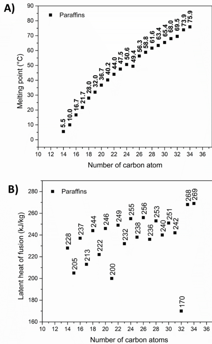
Figure 4. (A) Melting temperatures and (B) latent heat of fusion values of paraffin type PCMs.
