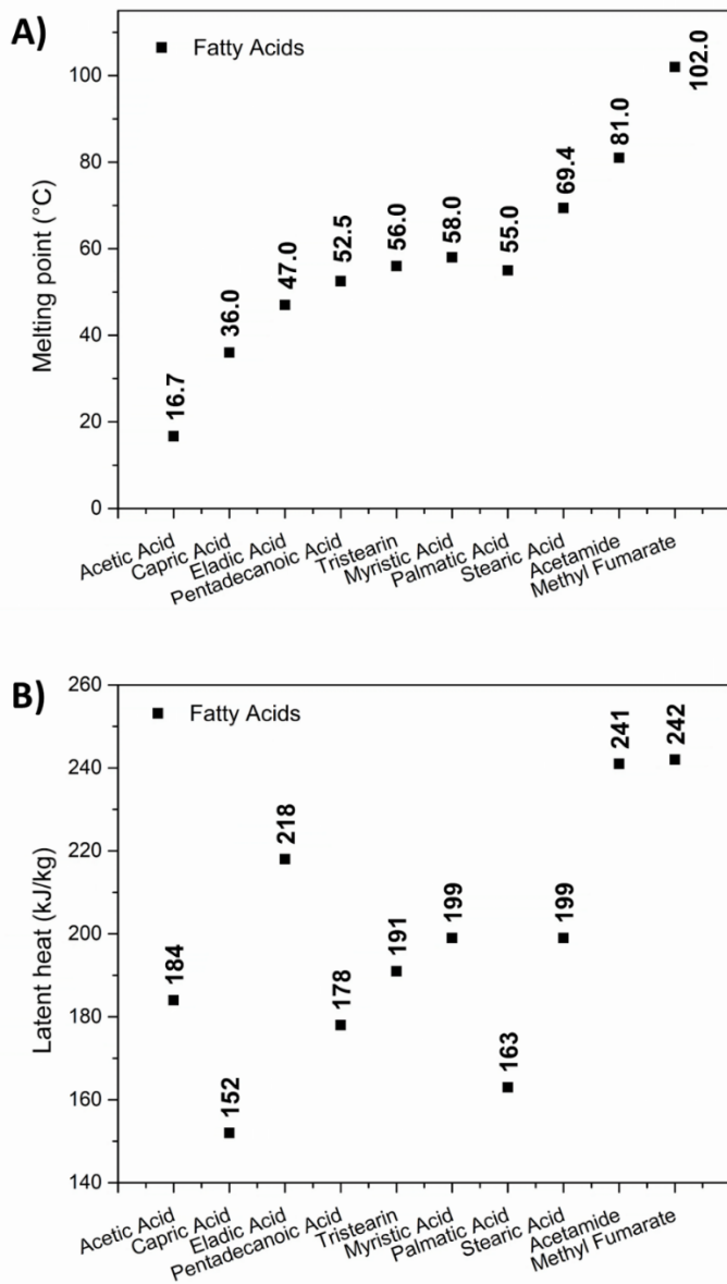
Figure 6. (A) Melting temperatures and (B) latent heat of fusion values of fatty acid type PCMs.
