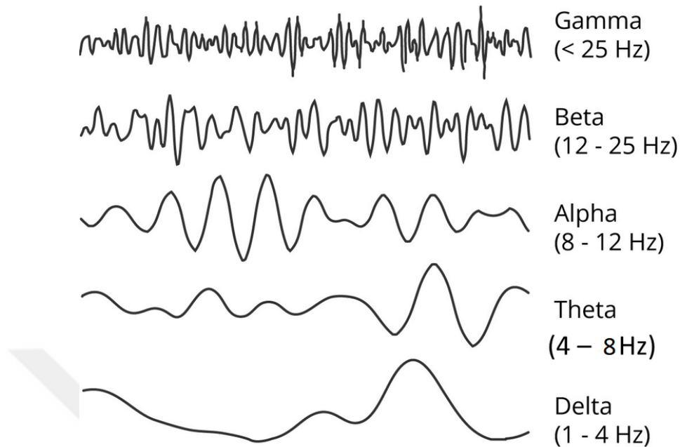
FIGURE 2.4. Frequency Band of EEG Signals
