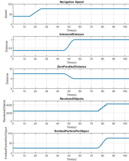
FIGURE 3.8. Time-dependent changes in the cue parameters of the control 2 session
