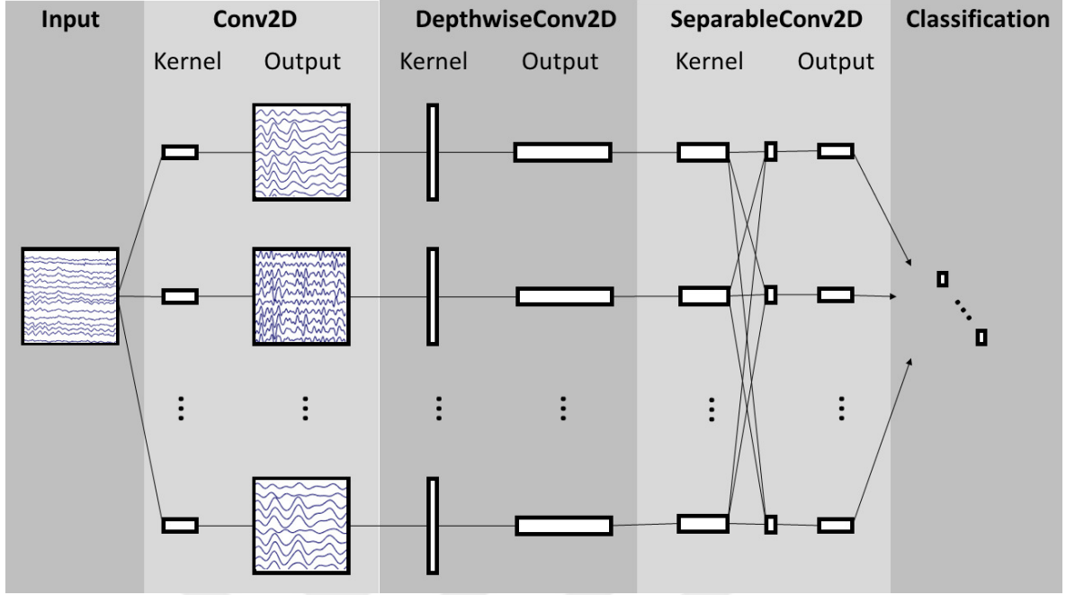
FIGURE 3.15. The architecture of EEGNet algorithm. Adapted from [4]
