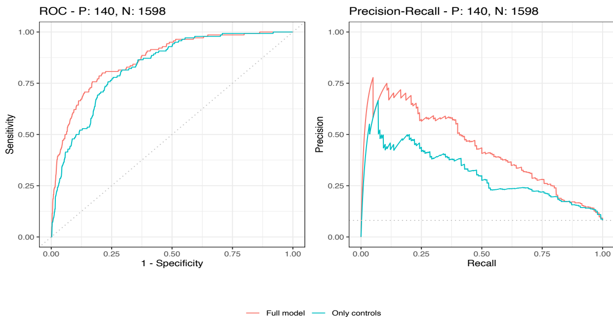
Figure 2.6: ROC and PR curves
