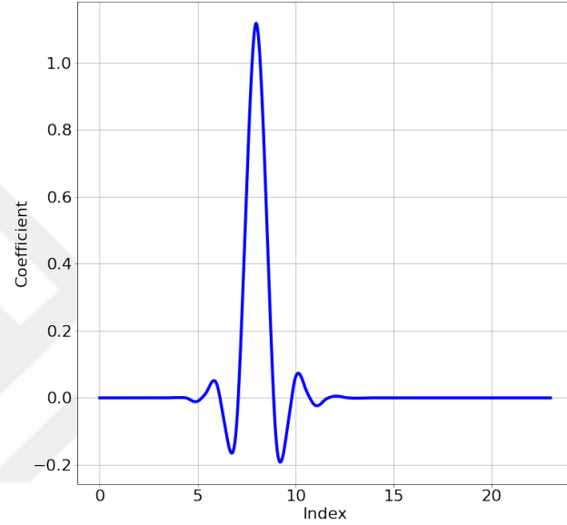
Figure 5.20. Coiflet 4 wavelet.
