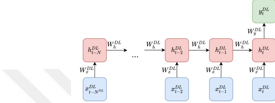
Figure 4.5. Architecture of RNN. Adapted from [50].
