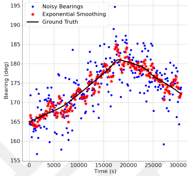
Figure 4.4. Exponential smoothing results.
