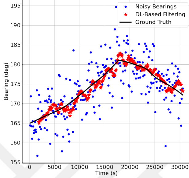
Figure 4.8. DL-based filtering results.
