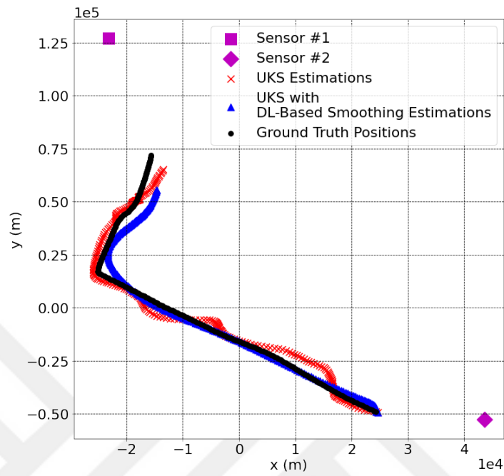
Figure 5.27. Estimated trajectory by UKS with DL-Based Smoothing.
