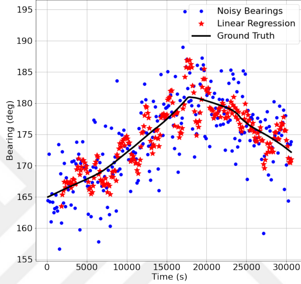
Figure 4.2. Linear regression results.
