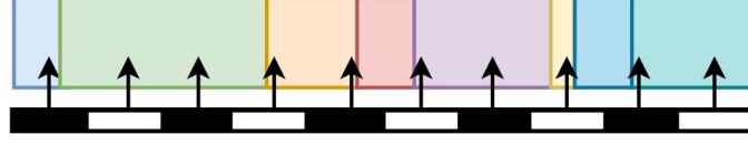
Figure 3.1. Visualization of systematic resampling method. Adapted from [30].
