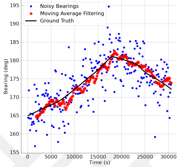
Figure 4.3. Moving average filtering results.
