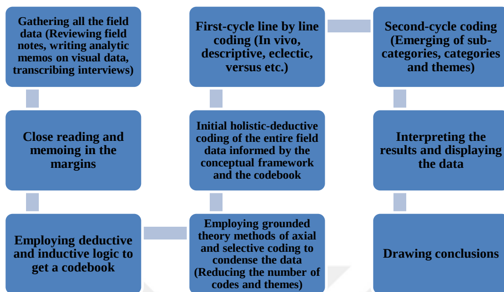
Figure 6. Data Analysis Procedure of the Study
