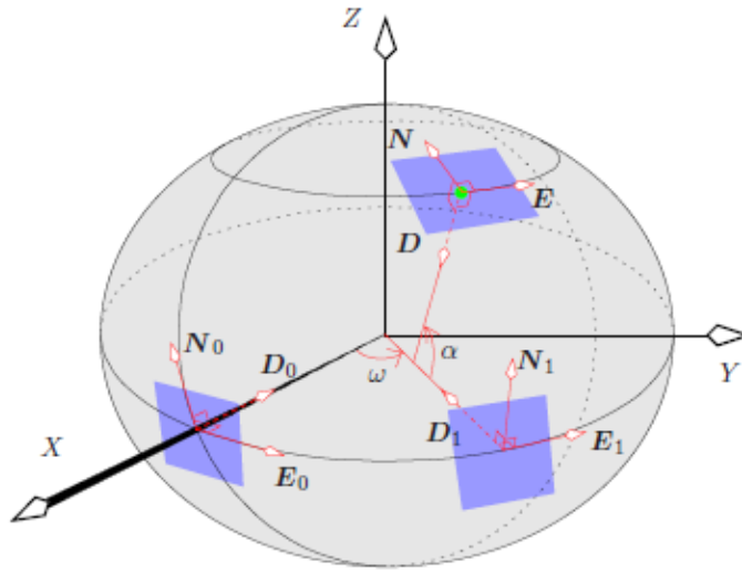
Figure 1-14: Local NED coordinate frames at different locations [18]
