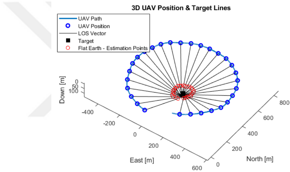
Figure 6-8: Flight Test 1 UAV position, target lines, and target position.
