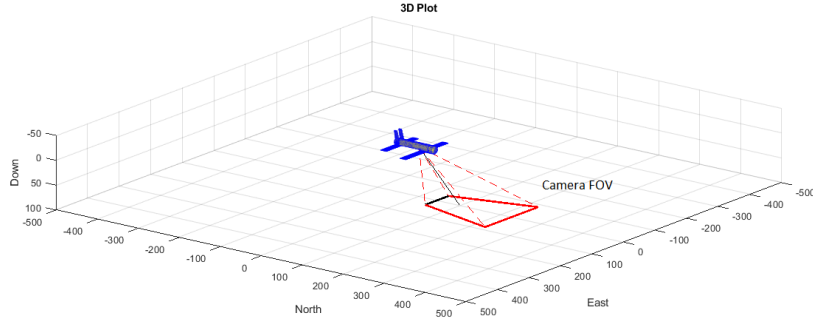
Figure 1-17: Top diagonal view of UAV with a -45-degrees gimbal elevation angle
