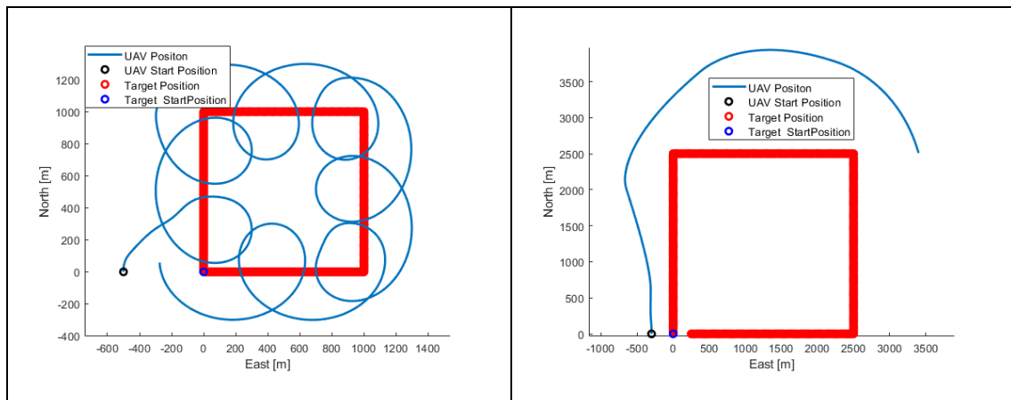
Figure 5-8: 2D position graph for moving and turning target with 5 m/s and 25 m/s speeds.
