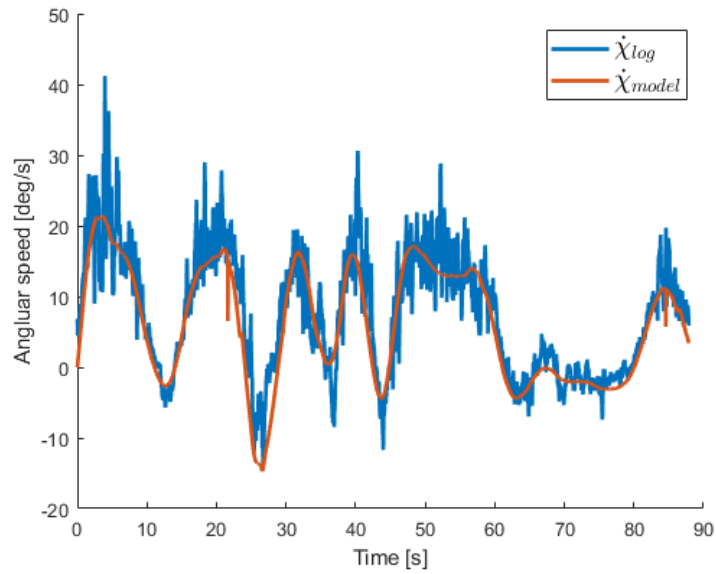
Figure 3-10: Model and flight track angle rates
