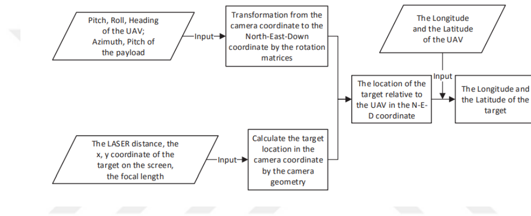
Figure 2-2: Single eye localization work flow [26]
