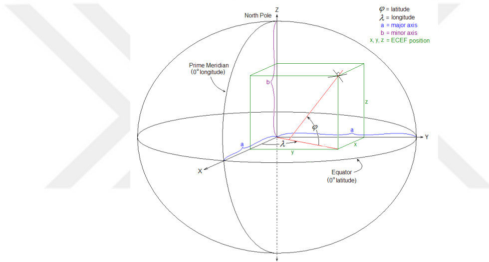
Figure 1-12: ECEF and NED frames
