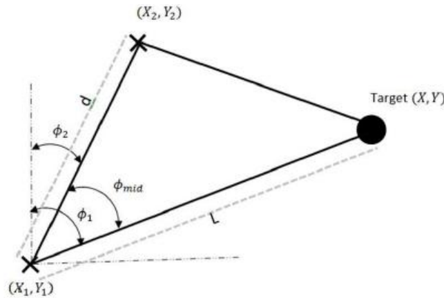
Figure 2-1: Object triangulation [27]
