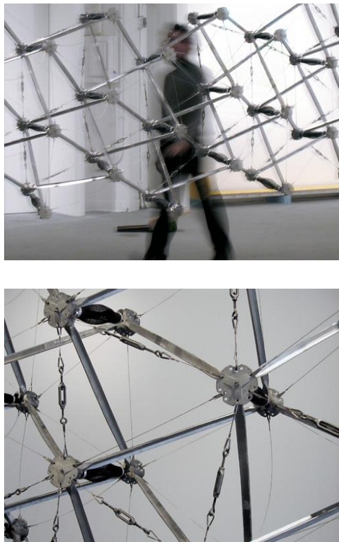
Figure 3.44. Actuated tensegrity prototypes. (Source: Orambra, 2012)
