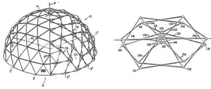
Figure 3.9. Zeigler's partial spherical dome (Source: Gantes, 2001)
