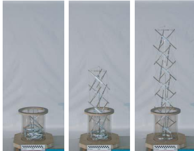
Figure 3- 41 Physical model of Pellegrino's folding mast at different stages of folding process (Source: Tibert & Pellegrino, 2003)
