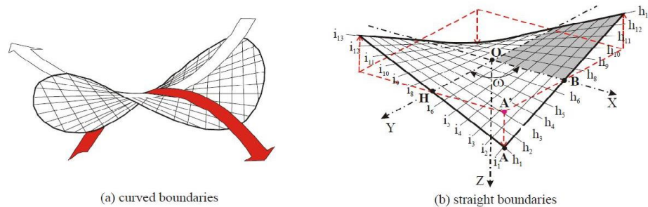
Figure 4.17. The boundaries, or edges, of the hyperbolic paraboloid can be straight or curved (Source: Pottmann, 2007)
