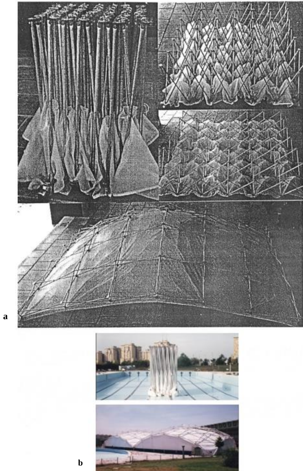
Figure 3.12. a) Model of a Selffolding roof hanging fabric (Source: Escrig et al., 1996) b) The Photo of the deployable roof for San Pablo Swimming Pool (Source: Escrig ,2013)
