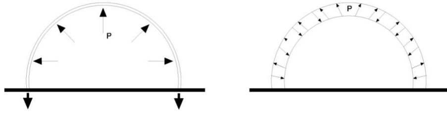
Figure 3.36. Principles of Air Supported and Air Inflated Membrane (Source: Gantes, 2001)
