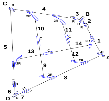
Figure 5.20 Kinematic diagram with intermediate links (Korkmaz, Susam & Akgün, 2013)
