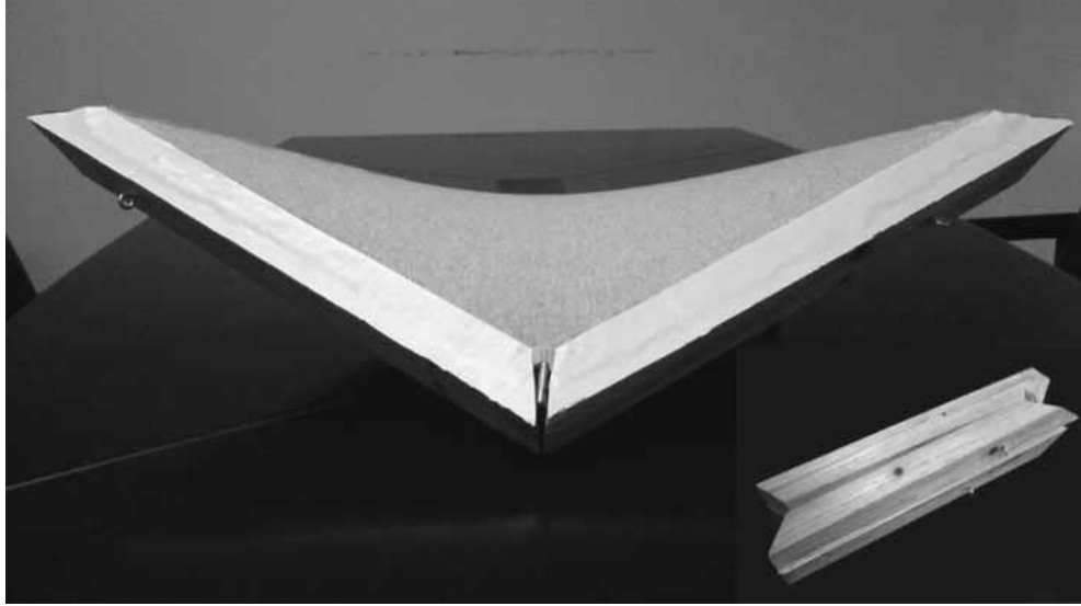
Figure 5.15. A deployable membrane structure in the folded and unfolded configurations (Source: Yu, Luo, & Li, 2007)
