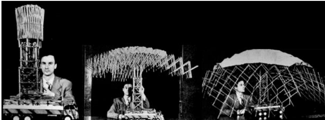
Figure 3.8. Pinero's deployable structure (Source: Robbin, 1996)
