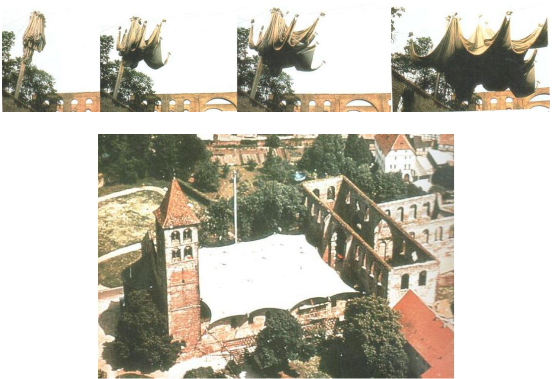
Figure 3.31. Frei Otto's convertible roof design for Bad Hersfeld in 1968 (Source: Otto & Rasch,1995)
