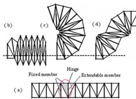
Figure 3.59. Transformation of beam shape using VGT (Source: Inoue, 2008)
