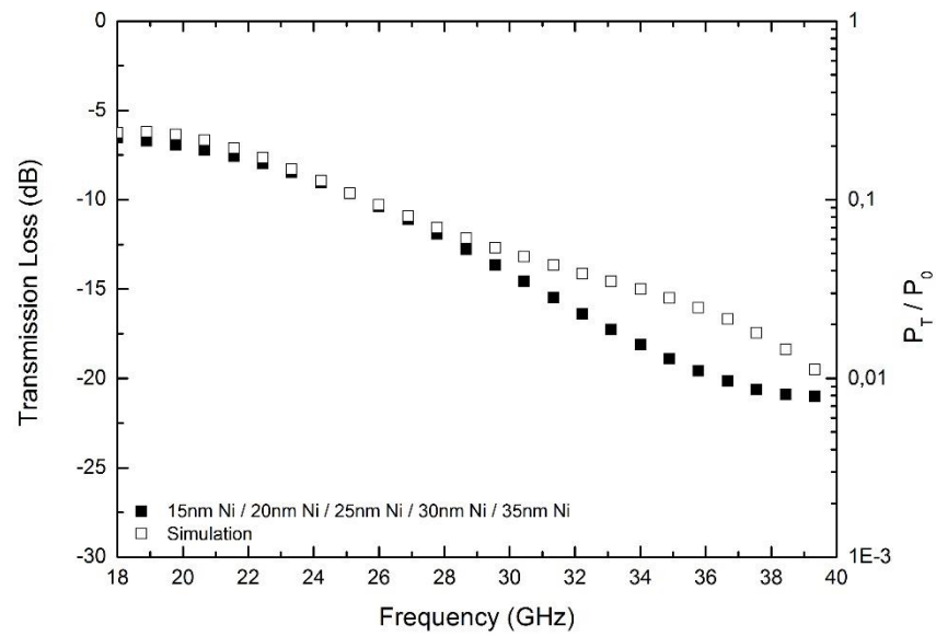
Figure A.32 EM wave transmission loss comparison of five layer nickel surface modified aramid fiber structure and its simulation.
