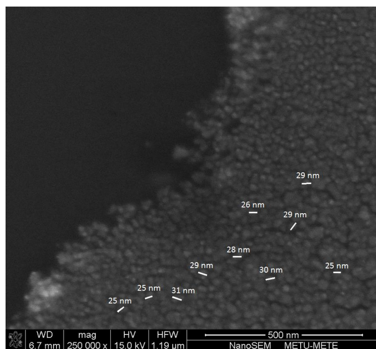
Figure 4.7 Edge morphology of 25 nm Au thin film on silicon wafer, photo taken by FESEM under x240000 magnification.
