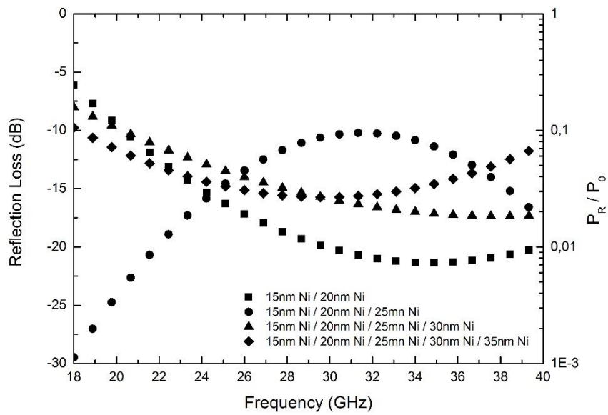
Figure 4.49 EM wave reflection loss varying with frequency in nickel surface modified multilayered aramid fiber woven fabrics.
