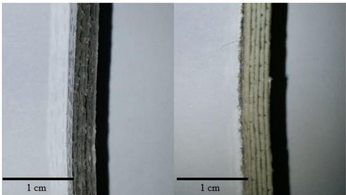
Figure 3.5 Cross-sections of composite structures without surface modifications.
