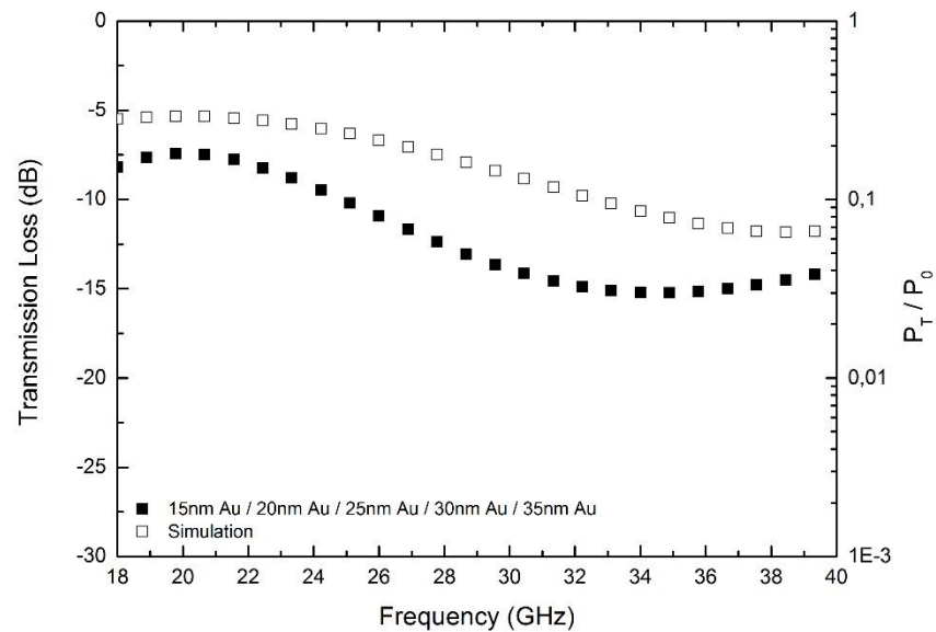
Figure 4.75 Comparison of measured and simulated EM wave transmission loss of gold surface modified 5-layered glass fiber woven fabric structure.
