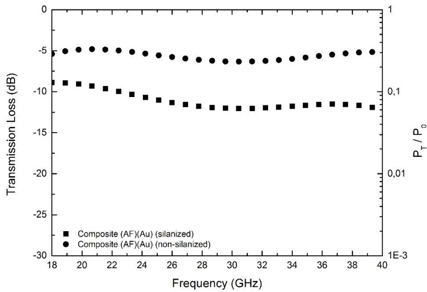
Figure 4.67 EM wave transmission loss varying with frequency in silanized and non-silanized composites containing gold surface modified multilayered aramid fiber woven fabrics.
