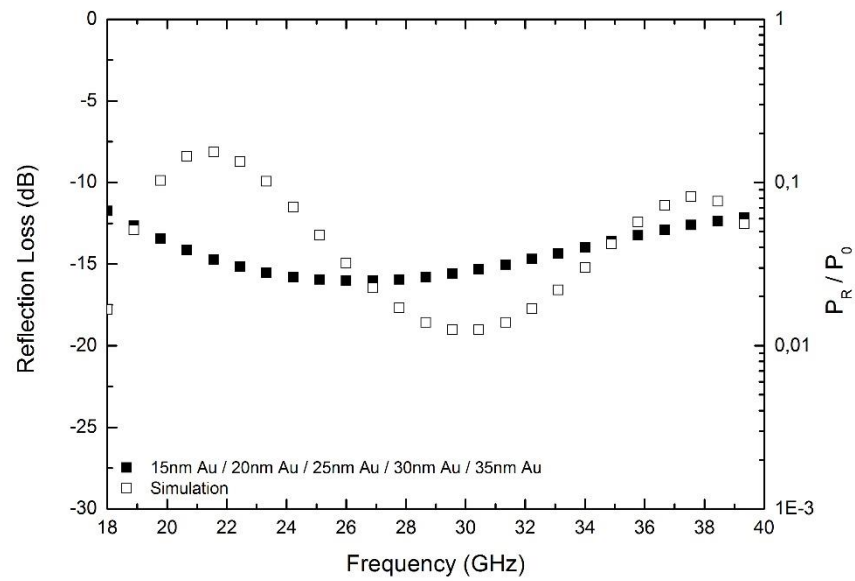
Figure A.28 EM wave reflection loss comparison of five layer gold surface modified aramid fiber structure and its simulation.
