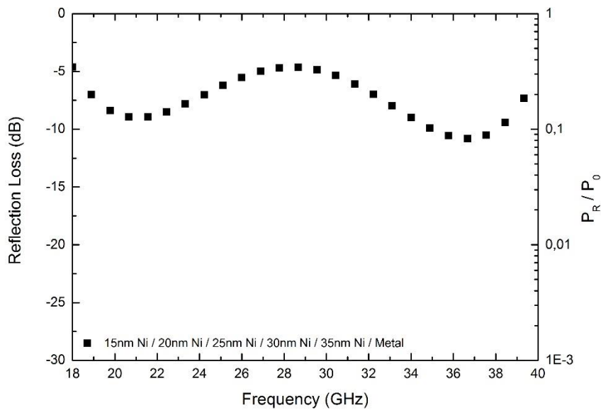
Figure 4.52 EM wave reflection loss varying with frequency in nickel surface modified 5-layered aramid fiber woven fabrics with metallic backing plate.
