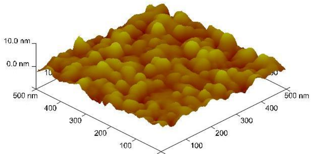
Figure 4.10 3D microstructure photo taken using AFM of 25 nm thick Au film on silicon wafer (500 nm x 500 nm area).
