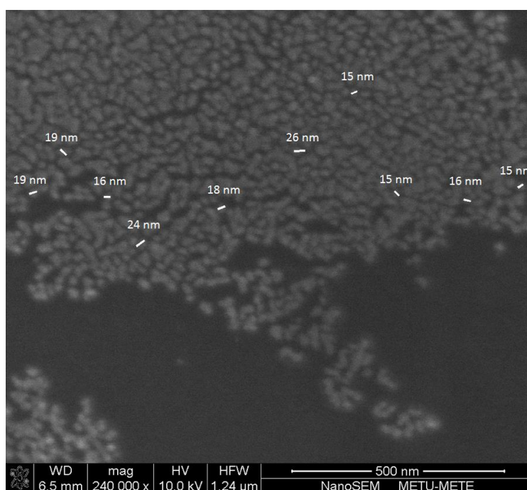
Figure 4.5 Edge morphology of 15 nm Au thin film on silicon wafer, photo taken by FESEM under x240000 magnification.
