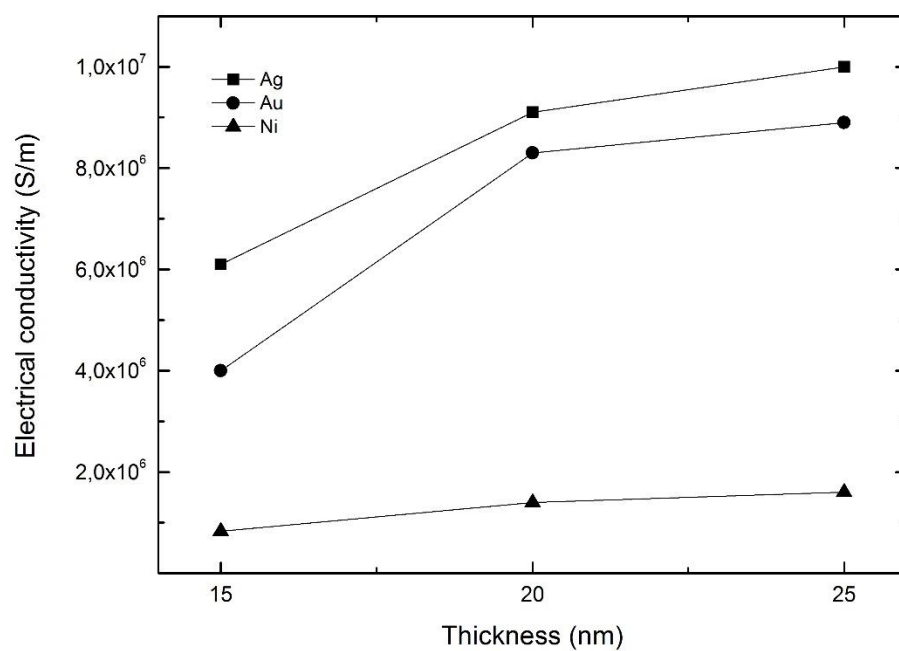
Figure 4.1 Electrical conductivity of Ag, Au, Ni thin films with changing film thickness.
