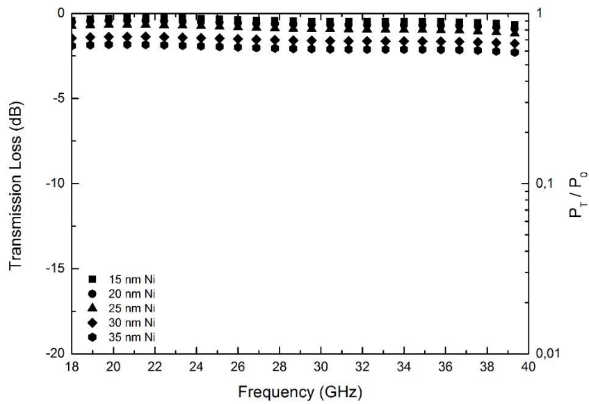
Figure A.20 EM wave transmission loss varying with frequency in silanized nickel surface modified single layer aramid fiber woven fabrics.
