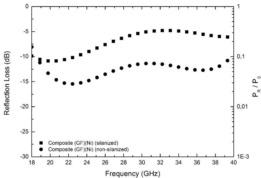
Figure 4.65 EM wave reflection loss varying with frequency in silanized and non-silanized composites containing nickel surface modified multilayered glass fiber woven fabrics under the presence of a metallic backing plate.
