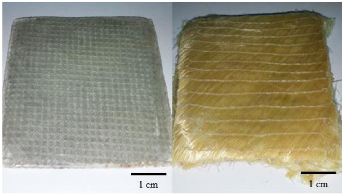
Figure 3.4 Photographs of fabricated composites without surface modifications.
