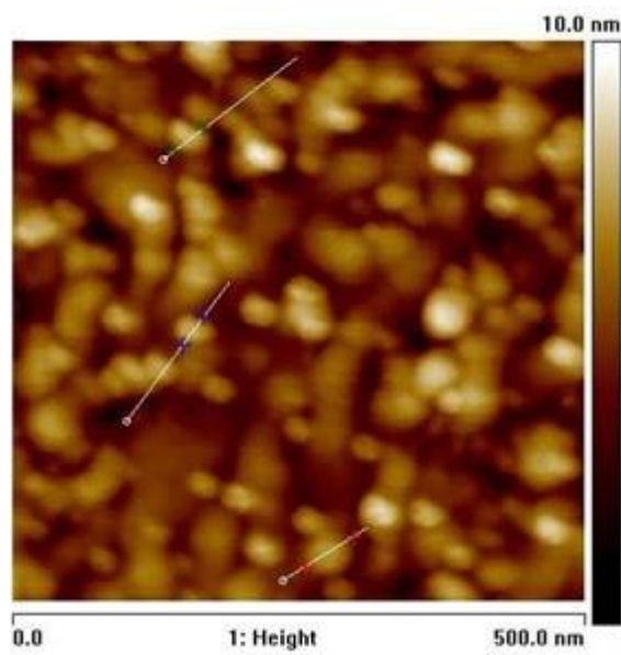
Figure 4.11 2D microstructure photo taken using AFM of 25 nm thick Au film on silicon wafer (500 nm x 500 nm area) and nuclei size determination.
