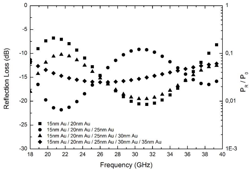
Figure 4.30 EM wave reflection loss varying with frequency in gold surface modified multilayered glass fiber woven fabrics.
