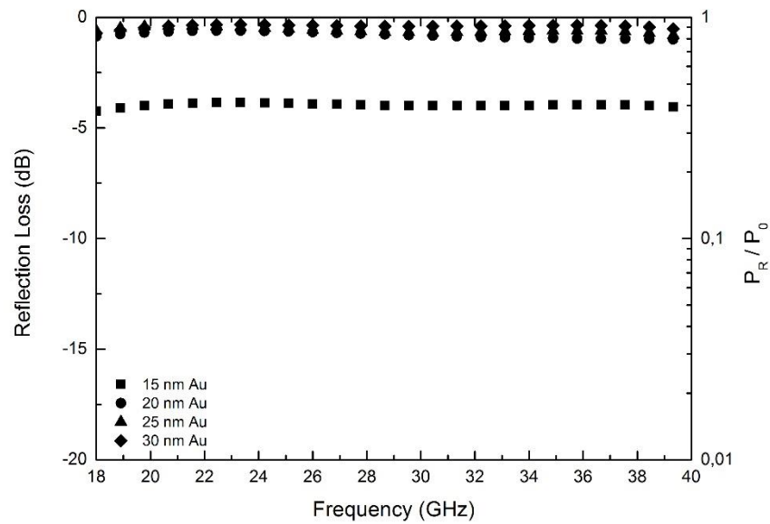
Figure 4.53 EM wave reflection loss varying with frequency in gold surface modified single layer PET sheets.
