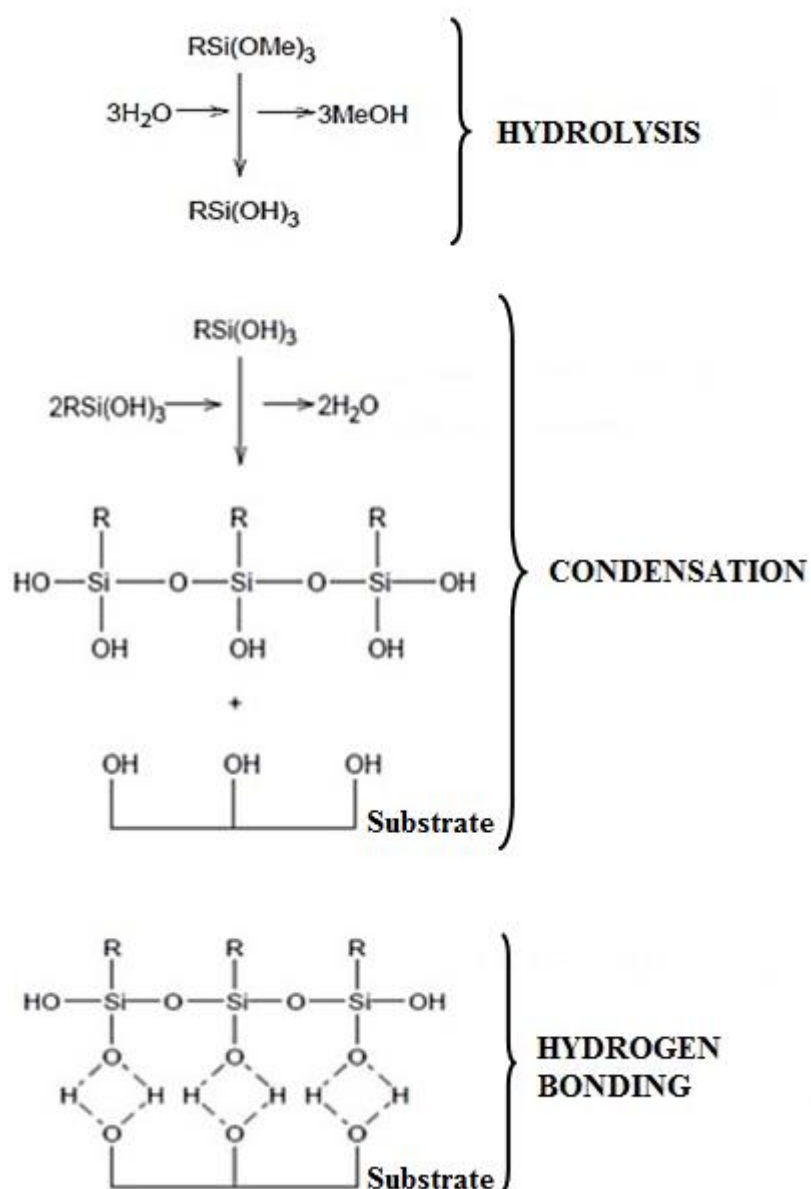
Figure 3.2 Schematics of chemical reactions taking place during silane treatment.
