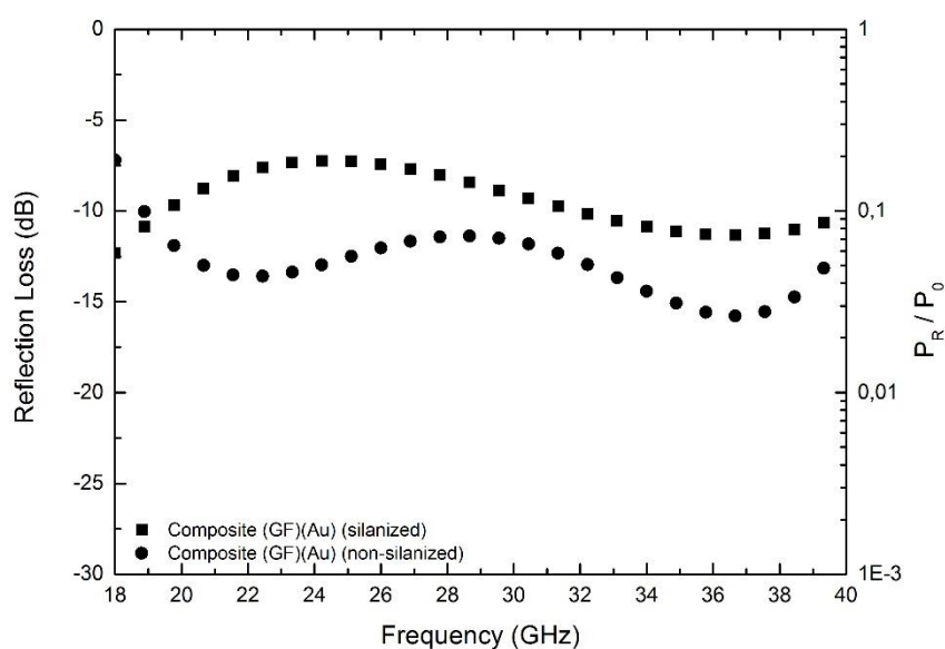
Figure 4.58 EM wave reflection loss varying with frequency in silanized and non-silanized composites containing gold surface modified multilayered glass fiber woven fabrics.
