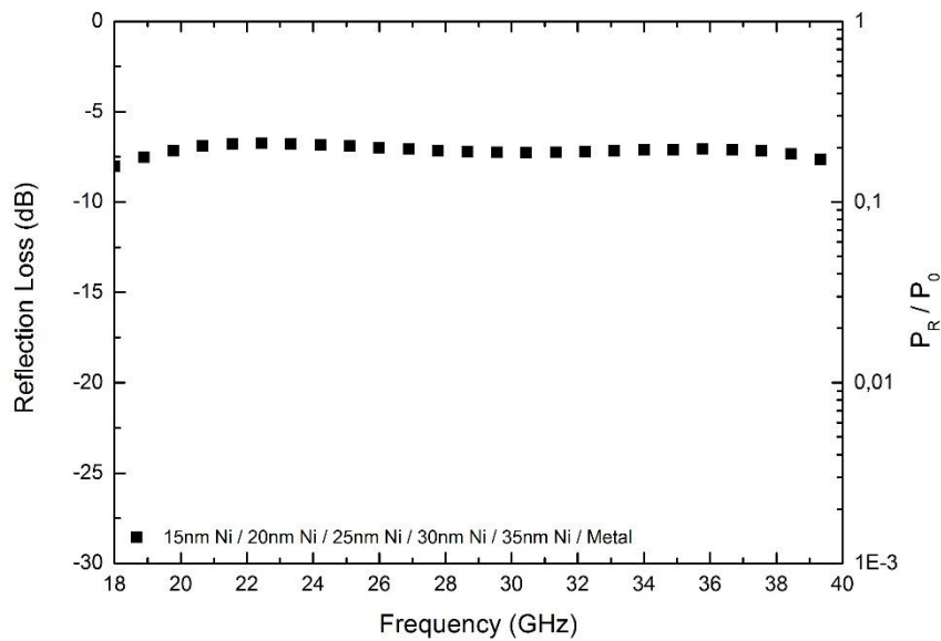
Figure 4.39 EM wave reflection loss varying with frequency in nickel surface modified 5-layered glass fiber woven fabrics with metallic backing plate.
