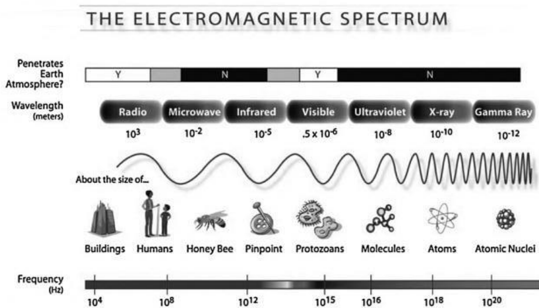
Figure 2.1 Electromagnetic spectrum [6].
