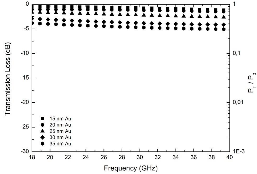
Figure 4.41 EM wave transmission loss varying with frequency in gold surface modified single layer aramid fiber woven fabrics.
