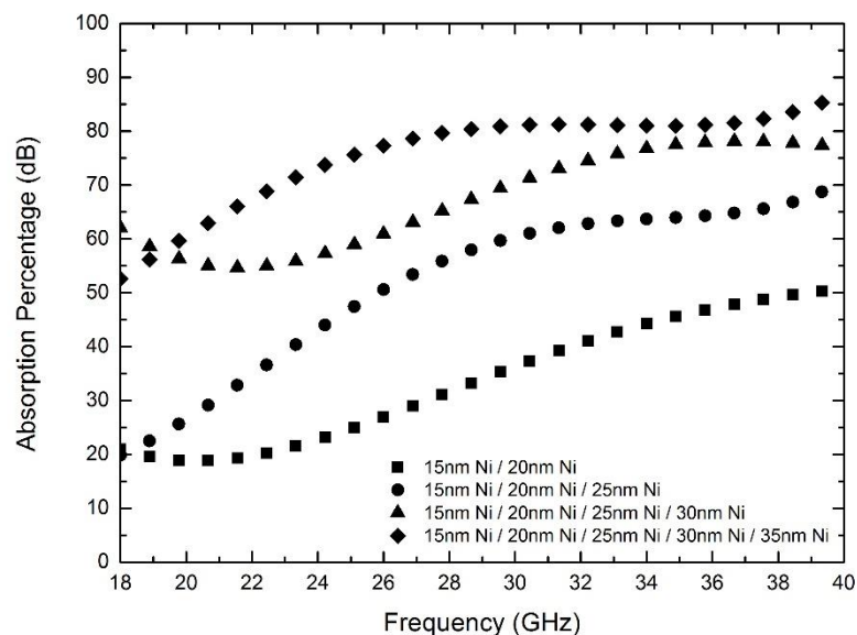
Figure 4.38 EM wave absorption percentages varying with frequency in nickel surface modified multilayered glass fiber woven fabrics.
