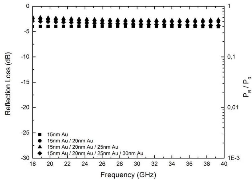
Figure 4.55 EM wave reflection loss varying with frequency in gold surface modified multilayered PET sheets.
