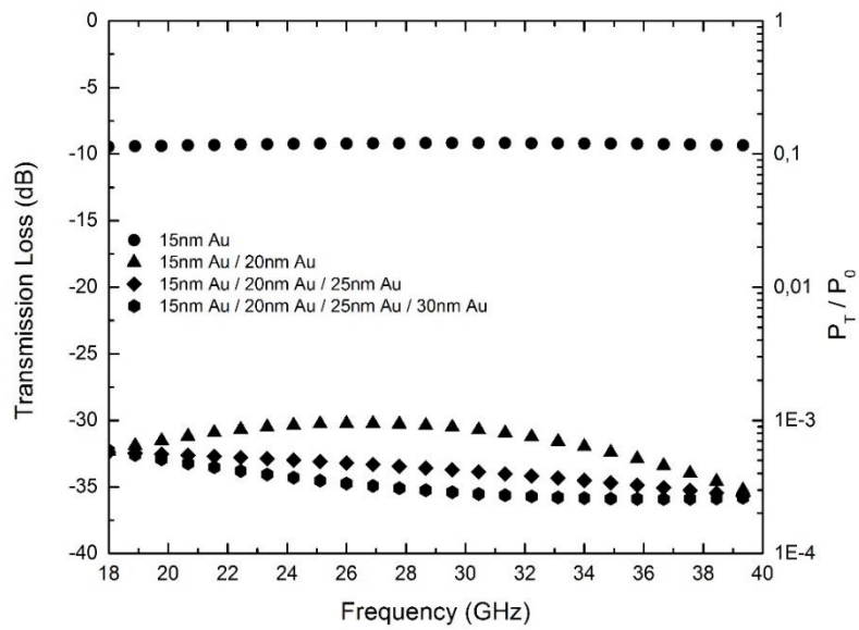
Figure 4.56 EM wave transmission loss varying with frequency in gold surface modified multilayered PET sheets.
