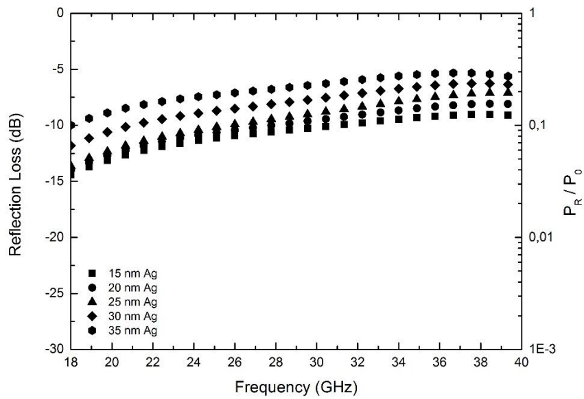
Figure 4.16 EM wave reflection loss varying with frequency in silver surface modified single layered glass fiber woven fabrics.
