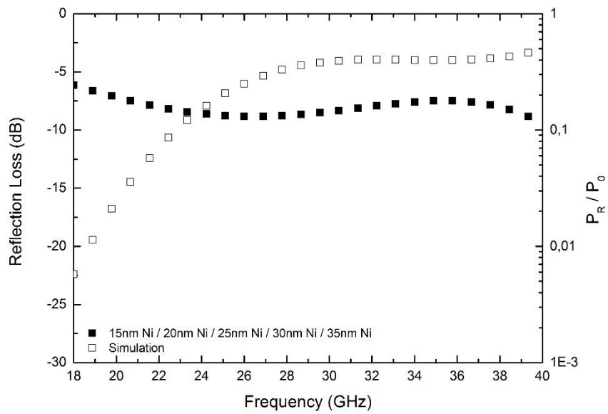
Figure A.31 EM wave reflection loss comparison of five layer nickel surface modified aramid fiber structure and its simulation.
