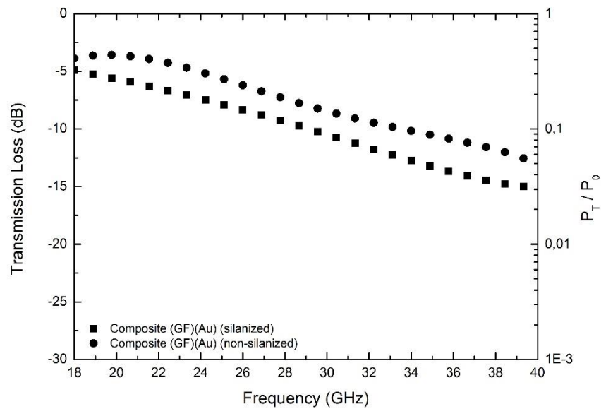
Figure 4.59 EM wave transmisson loss varying with frequency in silanized and non-silanized composites containing gold surface modified multilayered glass fiber woven fabrics.
