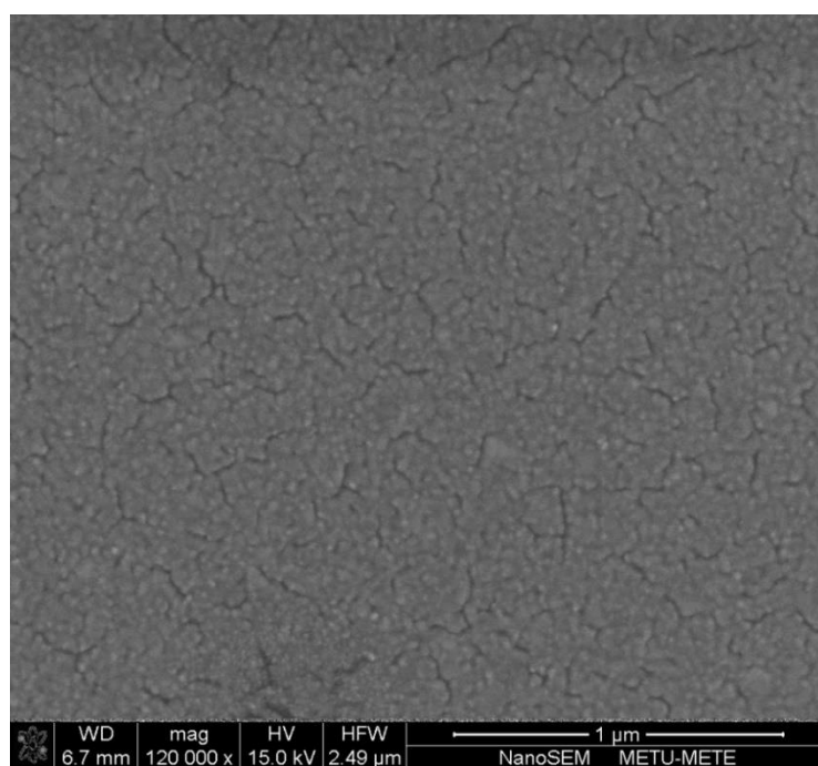
Figure 4.4 Surface morphology of 25 nm Au thin film on silicon wafer, photo taken by FESEM under x120000 magnification.
