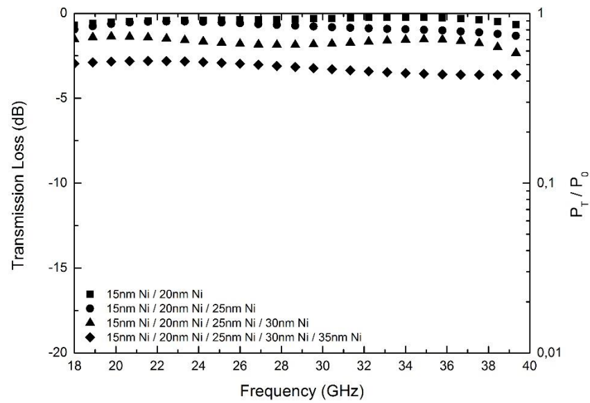
Figure A.22 EM wave transmission loss varying with frequency in silanized nickel surface modified multilayered aramid fiber woven fabrics.
