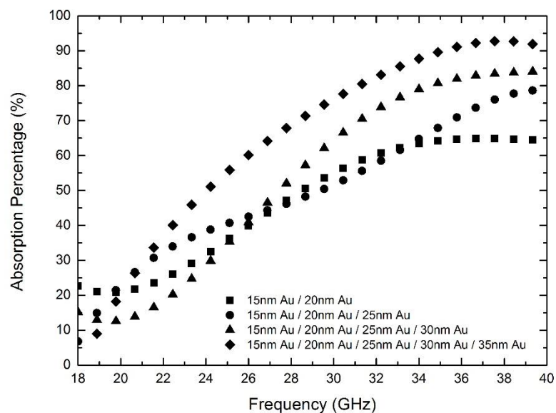
Figure A.5 EM wave absorption percentage varying with frequency in silanized gold surface modified multilayered glass fiber woven fabrics.
