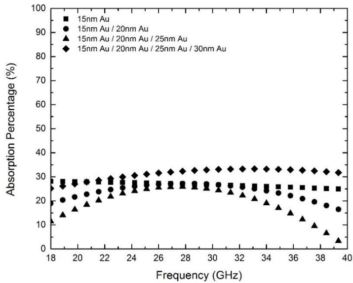
Figure 4.57 EM wave absorption percentage varying with frequency in gold surface modified multilayered PET sheets.
