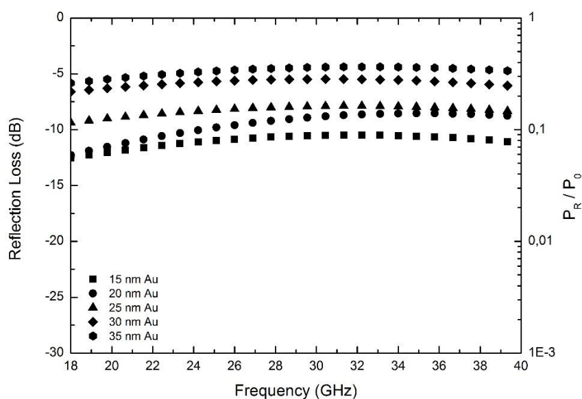
Figure 4.40 EM wave reflection loss varying with frequency in gold surface modified single layer aramid fiber woven fabrics.
