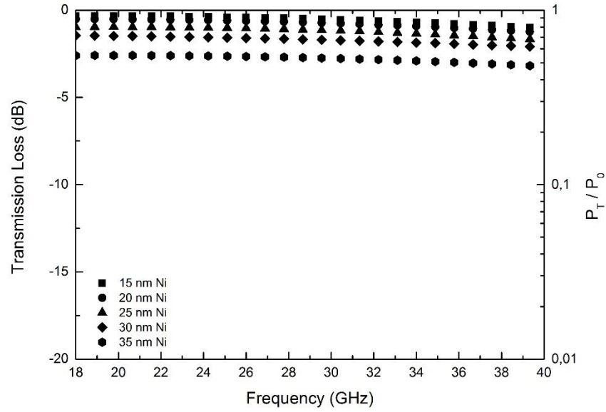
Figure 4.48 EM wave transmission loss varying with frequency in nickel surface modified single layer aramid fiber woven fabrics.
