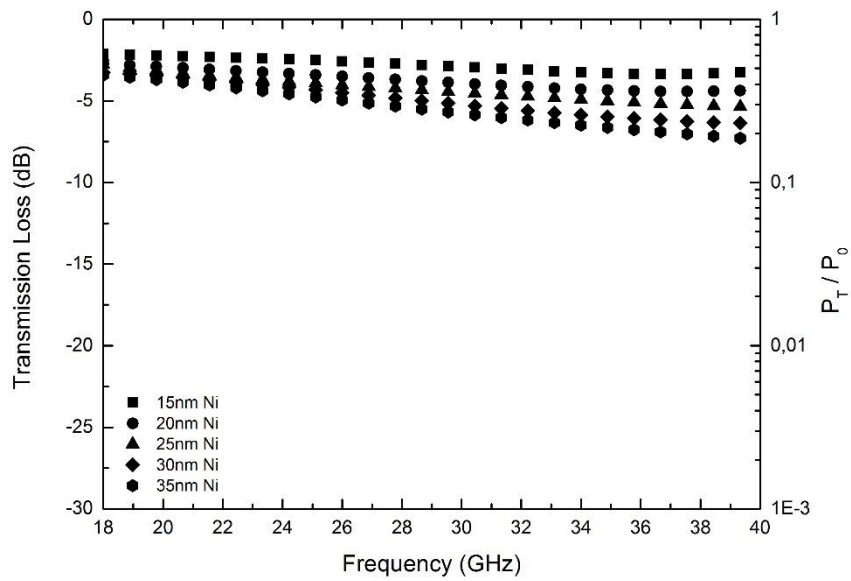
Figure A.8 EM wave transmission loss varying with frequency in silanized nickel surface modified single layer glass fiber woven fabrics.
