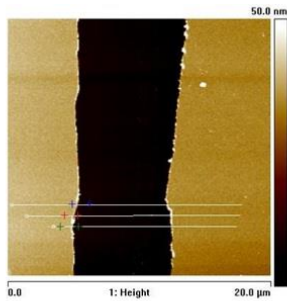
Figure 4.15 2D microstructure of the scratch, photo taken using AFM on the 25 nm thick Au film on silicon wafer (20 μm x 20 μm area) and thickness measurement.
