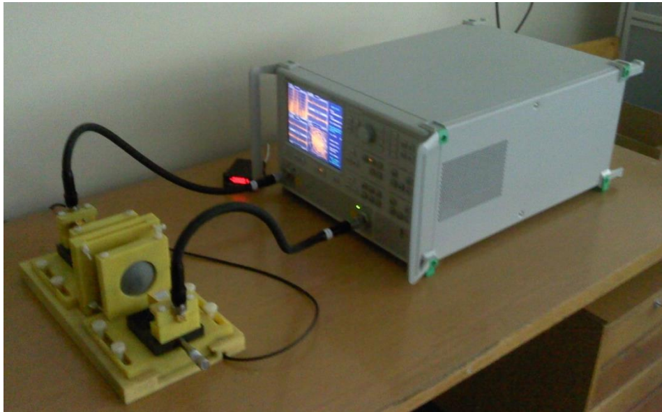
Figure 3.11 Custom-designed and built free-space measurement system and the utilized network analyzer.
