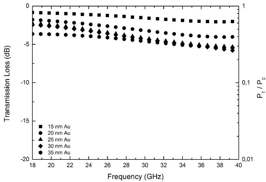
Figure A.2 EM wave transmission loss varying with frequency in silanized gold surface modified single layer glass fiber woven fabrics.
