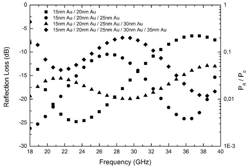
Figure A.15 EM wave reflection loss varying with frequency in silanized gold surface modified multilayered aramid fiber woven fabrics.
