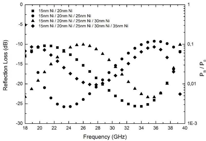
Figure A.21 EM wave reflection loss varying with frequency in silanized nickel surface modified multilayered aramid fiber woven fabrics.
