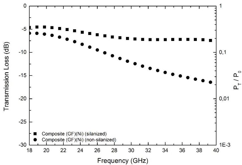
Figure 4.63 EM wave transmission loss varying with frequency in silanized and non-silanized composites containing nickel surface modified multilayered glass fiber woven fabrics.
