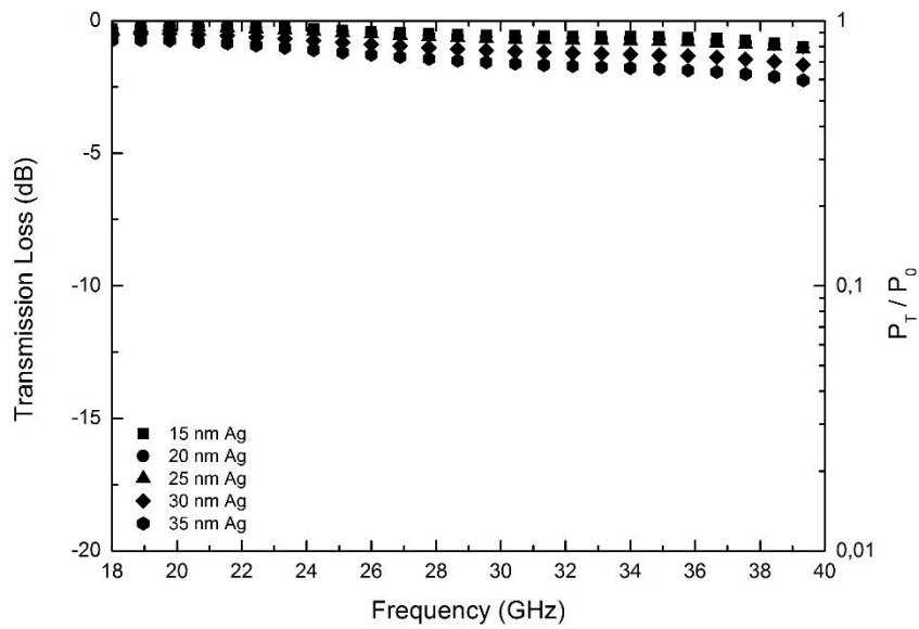
Figure 4.17 EM wave transmission loss varying with frequency in silver surface modified single layered glass fiber woven fabrics.
