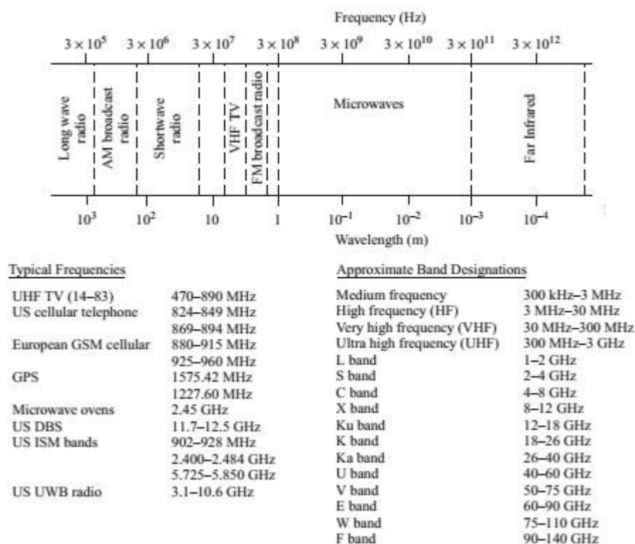
Figure 2.3 Microwave frequency applications and frequency bands [8].
