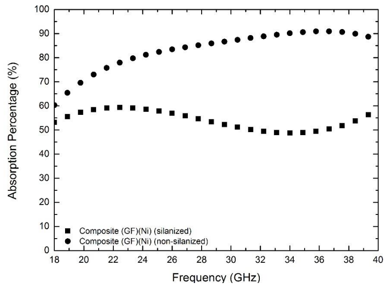
Figure 4.64 EM wave absorption percentage varying with frequency in silanized and non-silanized composites containing nickel surface modified multilayered glass fiber woven fabrics.
