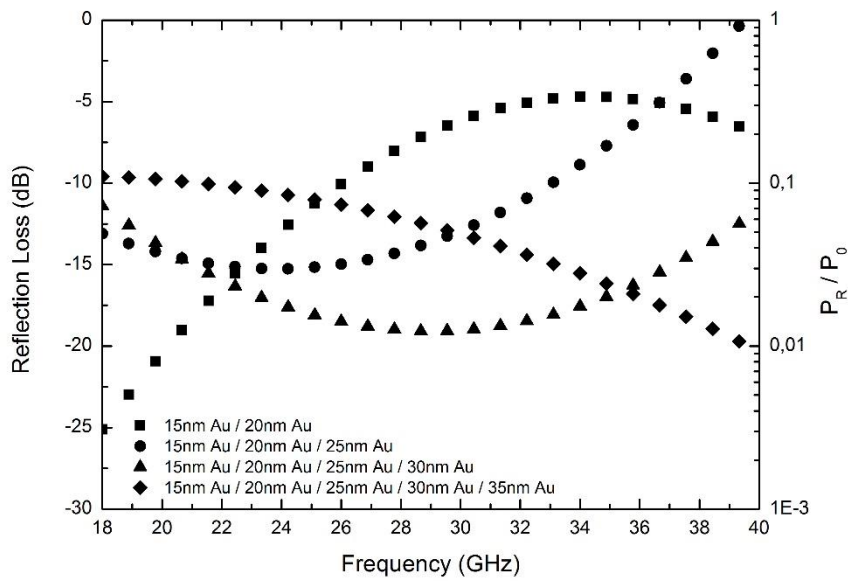
Figure 4.42 EM wave reflection loss varying with frequency in gold surface modified multilayered aramid fiber woven fabrics.
