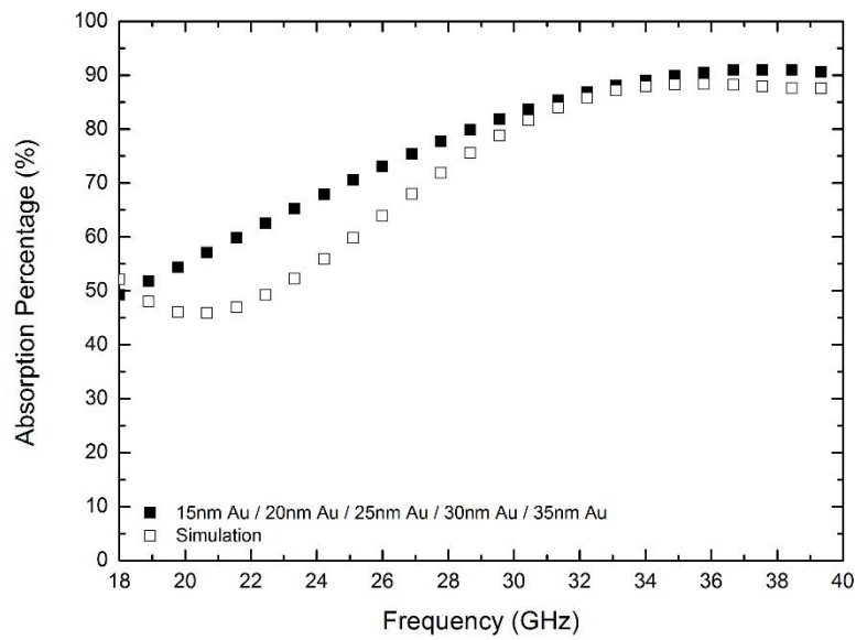
Figure A.30 EM wave absorption percentage comparison of five layer gold surface modified aramid fiber structure and its simulation.
