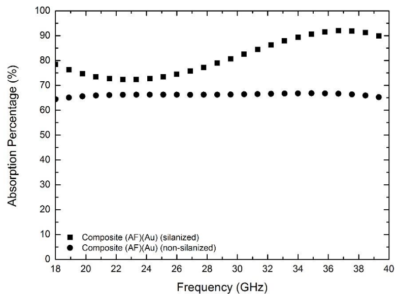
Figure 4.68 EM wave absorption percentage varying with frequency in silanized and non-silanized composites containing gold surface modified multilayered aramid fiber woven fabrics.
