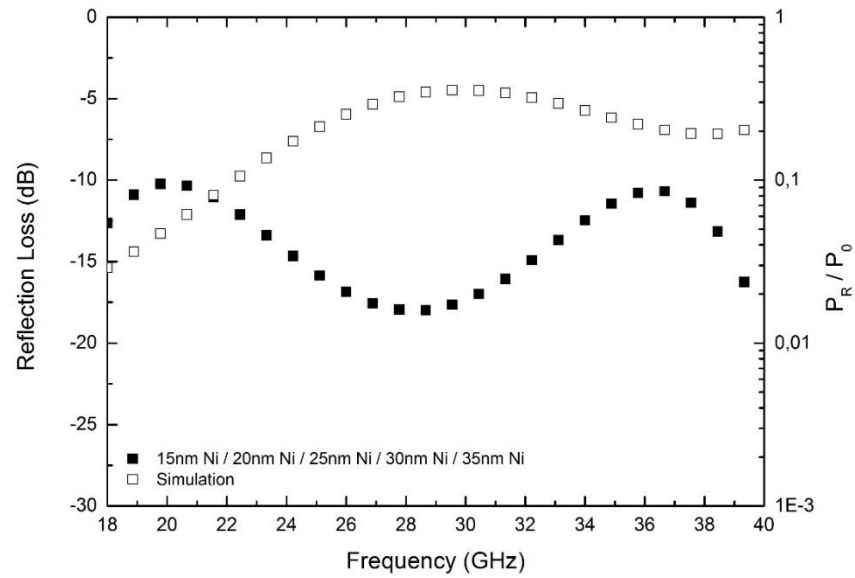
Figure A.25 EM wave reflection loss comparison of five layer nickel surface modified glass fiber structure and its simulation.
