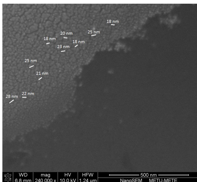
Figure 4.6 Edge morphology of 20 nm Au thin film on silicon wafer, photo taken by FESEM under x240000 magnification.
