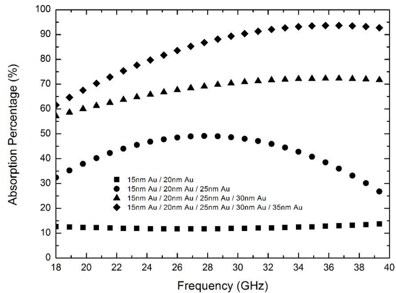
Figure 4.44 EM wave absorption percentage varying with frequency in gold surface modified multilayered aramid fiber woven fabrics.
