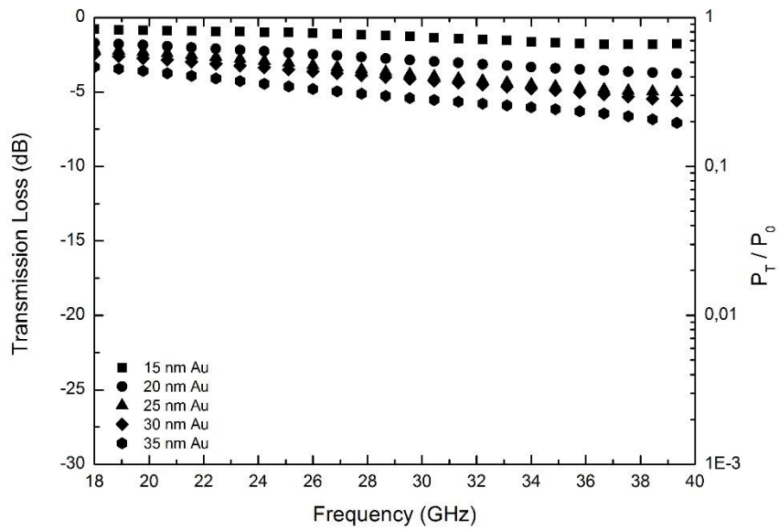
Figure 4.29 EM wave transmission loss varying with frequency in gold surface modified single layer glass fiber woven fabrics.
