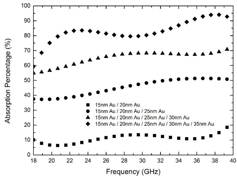
Figure A.17 EM wave absorption percentage varying with frequency in silanized gold surface modified single layer aramid fiber woven fabrics.
