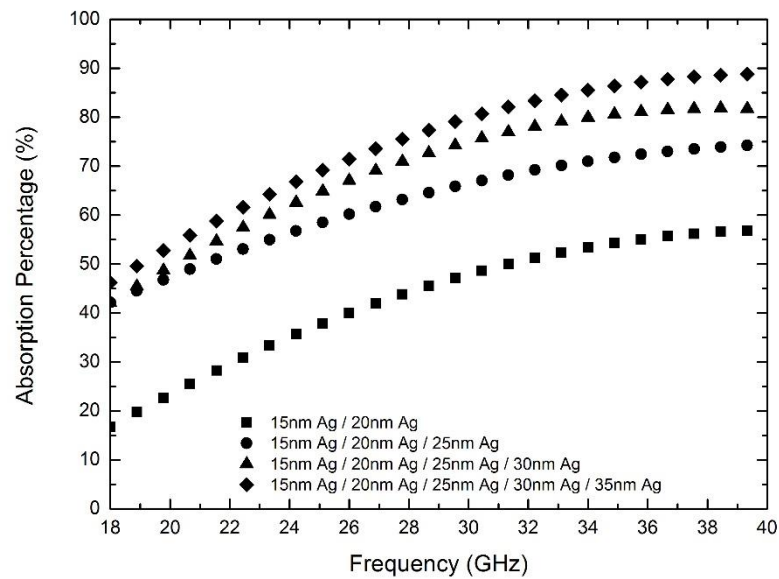
Figure 4.20 EM wave absorption varying with frequency in silver surface modified multilayered glass fiber woven fabrics.
