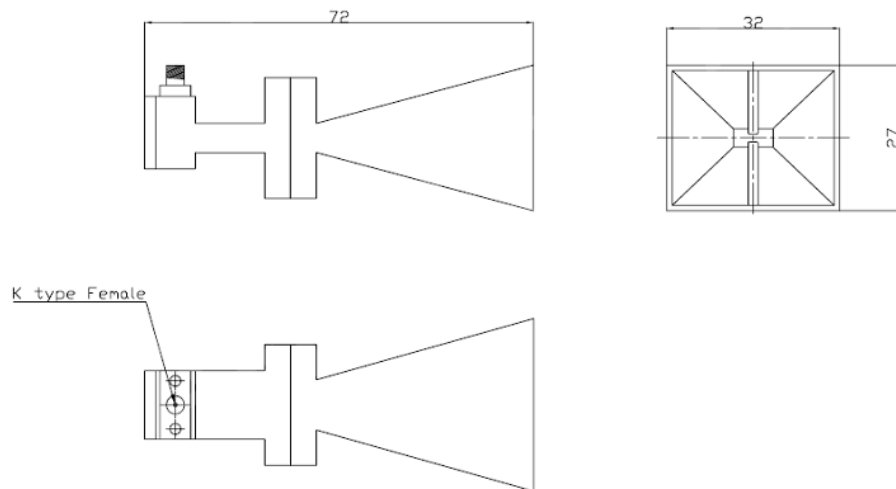
Figure 3.7 Schematic view of horn antennas used in free-space measurement system with their dimensions (dimensions are in unit of mm).
