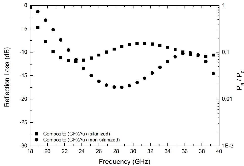
Figure 4.61 EM wave reflection loss varying with frequency in silanized and non-silanized composites containing gold surface modified multilayered glass fiber woven fabrics under the presence of a metallic backing plate.
