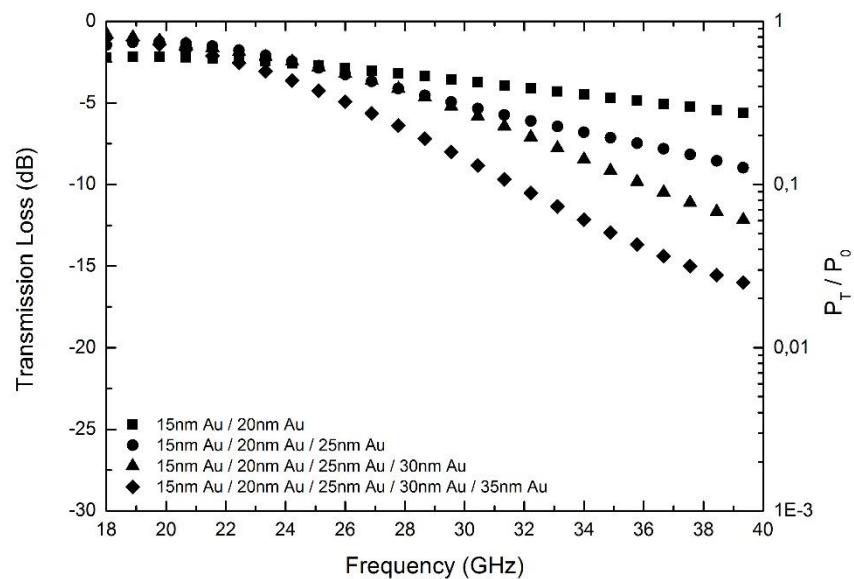
Figure A.4 EM wave transmission loss varying with frequency in silanized gold surface modified multilayered glass fiber woven fabrics.
