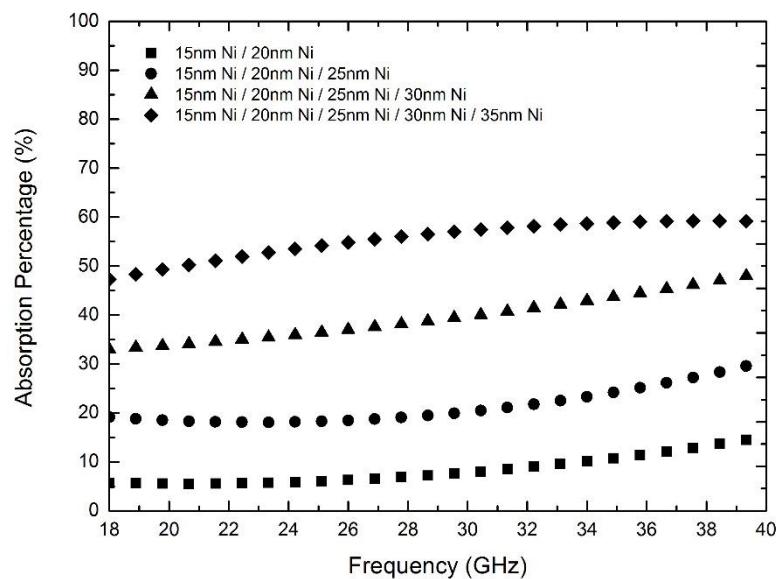
Figure 4.51 EM wave absorption percentage varying with frequency in nickel surface modified multilayered aramid fiber woven fabrics.
