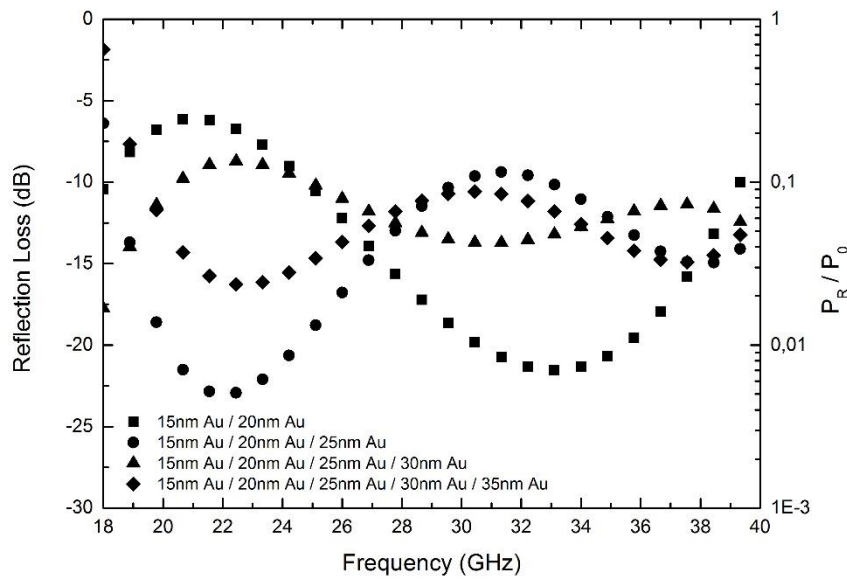
Figure A.3 EM wave reflection loss varying with frequency in silanized gold surface modified multilayered glass fiber woven fabrics.
