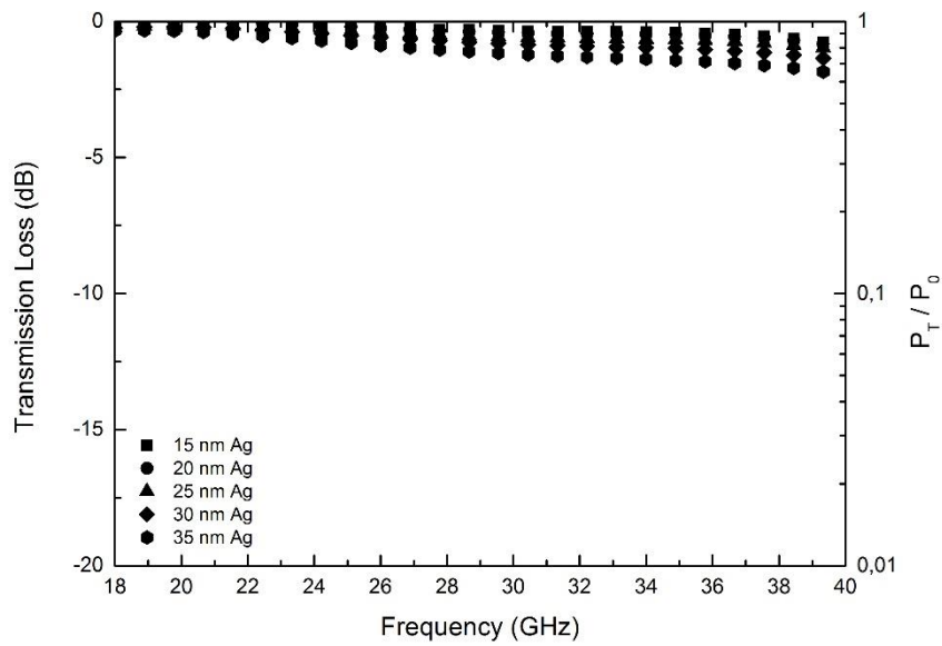
Figure 4.23 EM wave transmission loss varying with frequency in oxidized silver surface modified single layered glass fiber woven fabrics.
