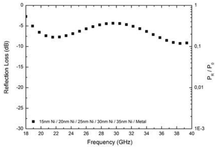
Figure A.24 EM wave reflection loss varying with frequency in silanized nickel surface modified multilayered aramid fiber woven fabrics with backing metallic plate.
