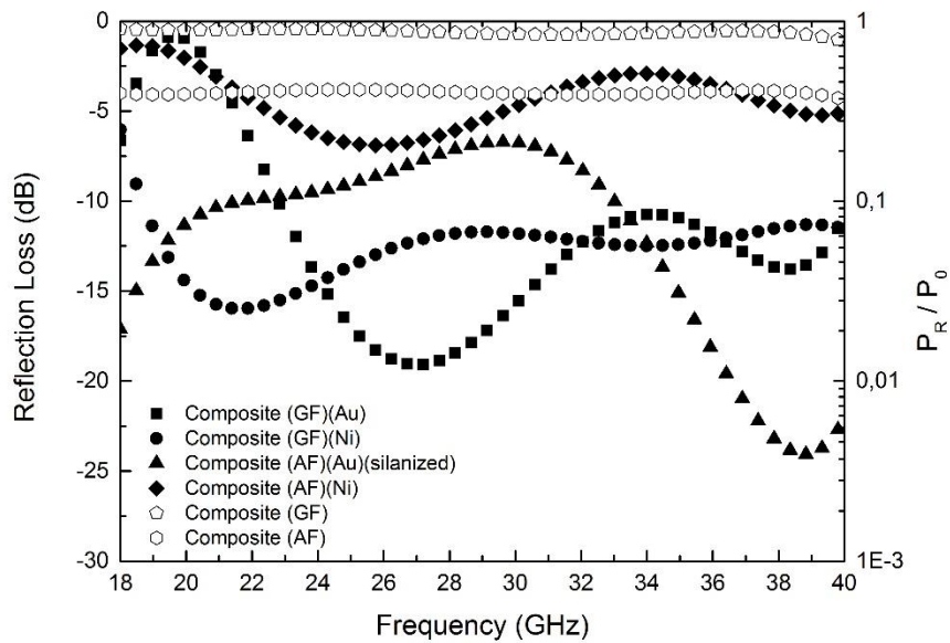
Figure 4.84 EM wave reflection loss of selected composites varying with frequency.
