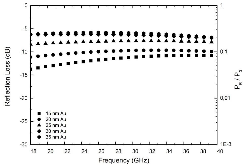
Figure A.13 EM wave reflection loss varying with frequency in silanized gold surface modified single layer aramid fiber woven fabrics.
