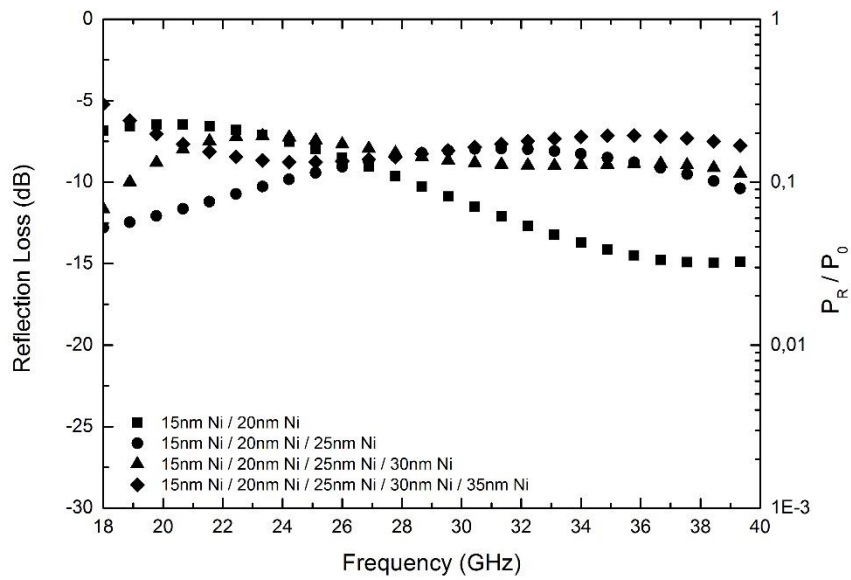
Figure A.9 EM wave reflection loss varying with frequency in silanized nickel surface modified multilayered glass fiber woven fabrics.
