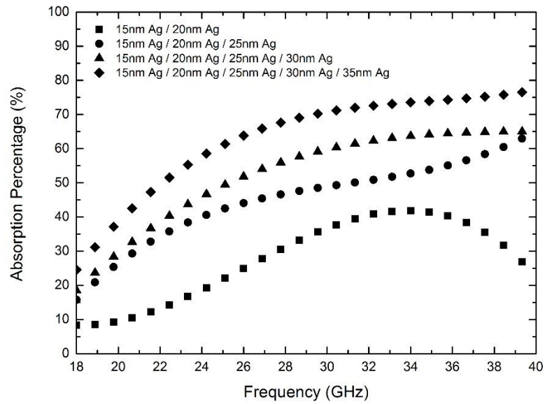
Figure 4.26 EM wave absorption percentage varying with frequency in oxidized silver surface modified multilayered glass fiber woven fabrics.
