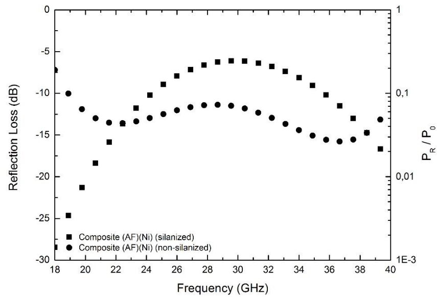
Figure 4.70 EM wave reflection loss varying with frequency in silanized and non-silanized composites containing nickel surface modified multilayered aramid fiber woven fabrics.
