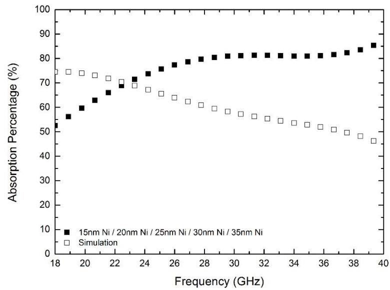
Figure A.33 EM wave absorption percentage comparison of five layer nickel surface modified aramid fiber structure and its simulation.
