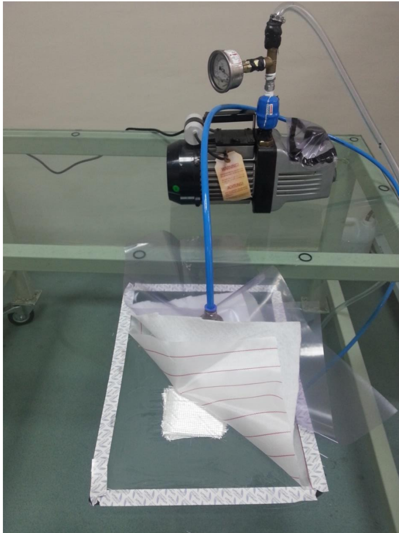
Figure 3.3 Constructed vacuum bagging system.
