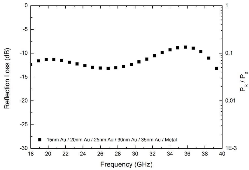
Figure A.18 EM wave reflection loss varying with frequency in silanized gold surface modified multilayered aramid fiber woven fabrics with backing metallic plate.
