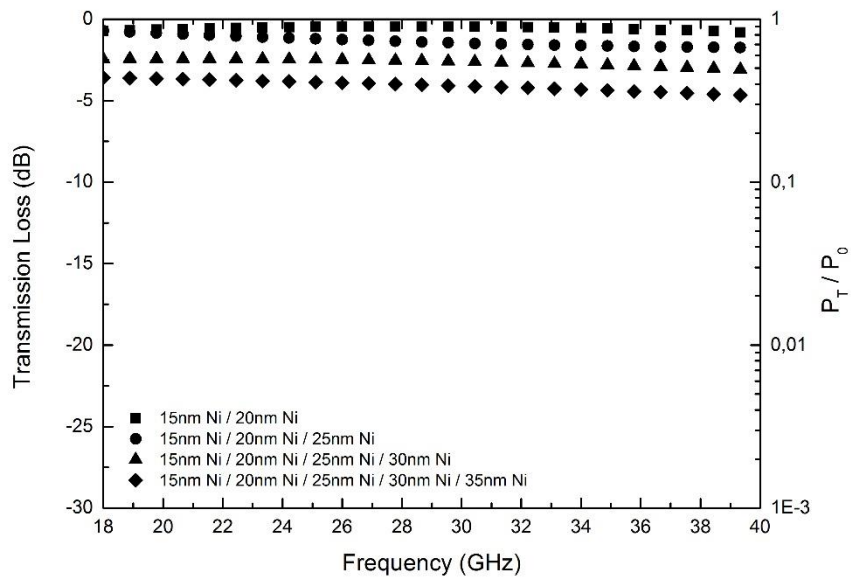
Figure 4.50 EM wave transmission loss varying with frequency in nickel surface modified multilayered aramid fiber woven fabrics.
