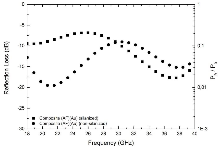
Figure 4.66 EM wave reflection loss varying with frequency in silanized and non-silanized composites containing gold surface modified multilayered aramid fiber woven fabrics.
