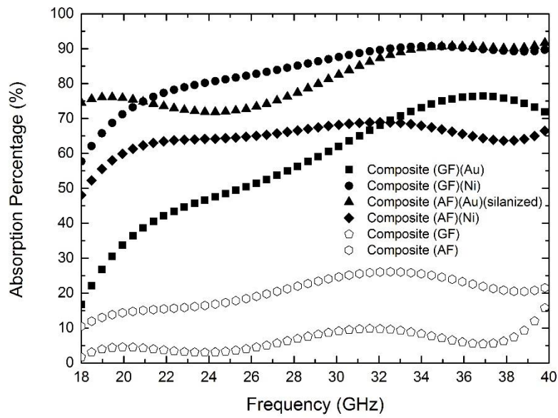
Figure 4.83 EM wave absorption percentage of the selected composites varying with frequency.
