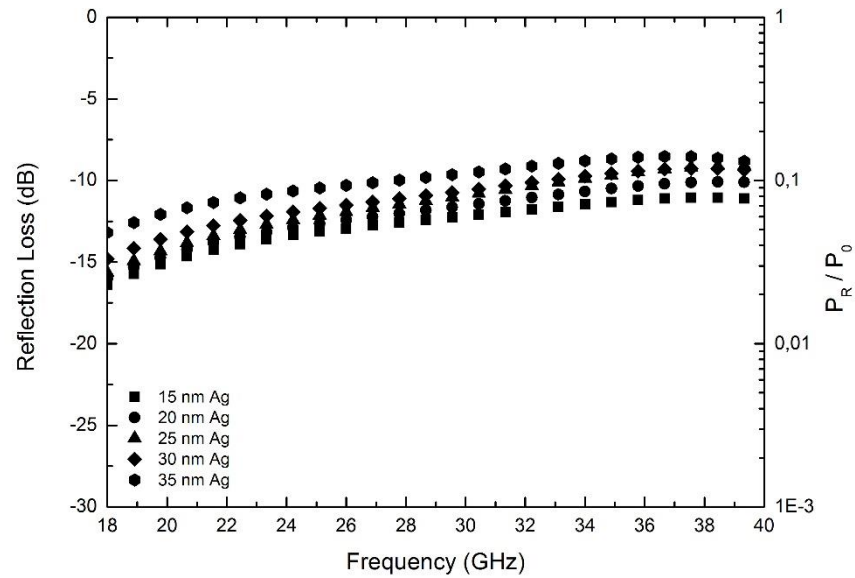
Figure 4.22 EM wave reflection loss varying with frequency in oxidized silver surface modified single layered glass fiber woven fabrics.
