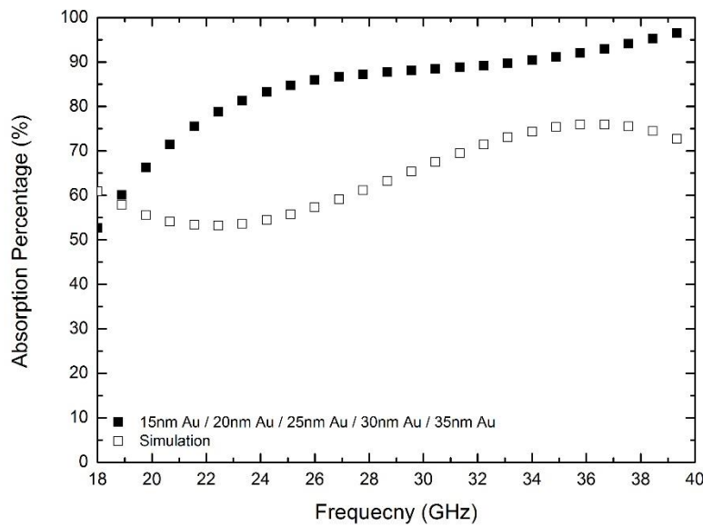
Figure 4.76 Comparison of measured and simulated EM wave absorption percentage of gold surface modified 5-layered glass fiber woven fabric structure.
