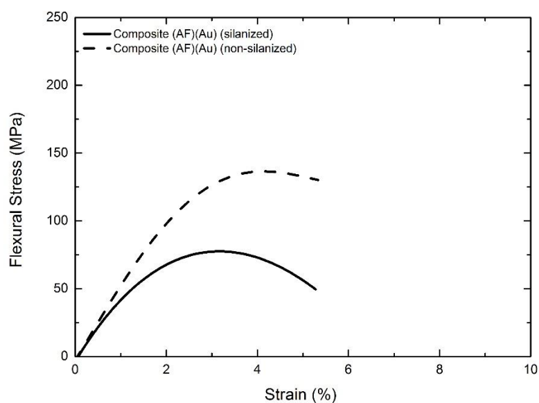
Figure 4.81 Three-point bending test results of prototype composites containing silanized and non-silanized gold surface modified aramid fiber woven fabrics.
