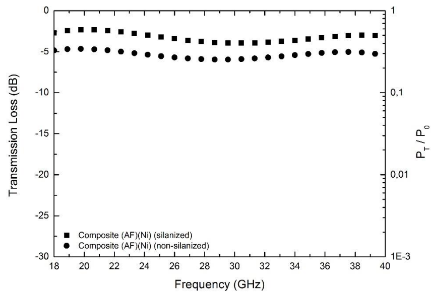
Figure 4.71 EM wave transmission loss varying with frequency in silanized and non-silanized composites containing nickel surface modified multilayered aramid fiber woven fabrics.
