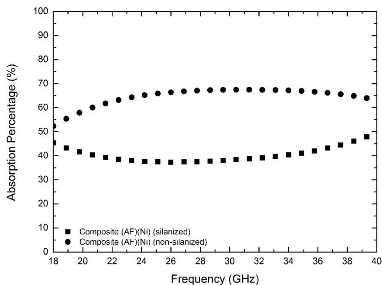
Figure 4.72 EM wave absorption percentage varying with frequency in silanized and non-silanized composites containing nickel surface modified multilayered aramid fiber woven fabrics.
