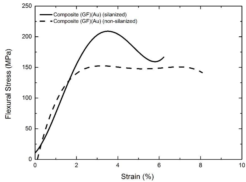
Figure 4.78 Three-point bending test results of prototype composites containing silanized and non-silanized gold surface modified glass fiber woven fabrics.
