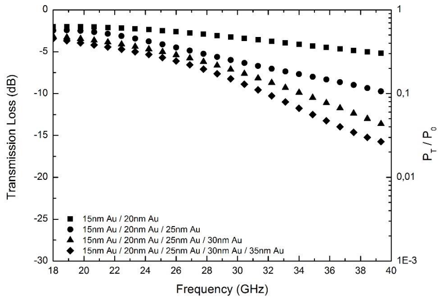
Figure 4.31 EM wave transmission loss varying with frequency in gold surface modified multilayered glass fiber woven fabrics.
