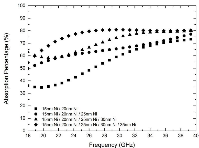
Figure A.11 EM wave absorption percentage varying with frequency in silanized nickel surface modified multilayered glass fiber woven fabrics.
