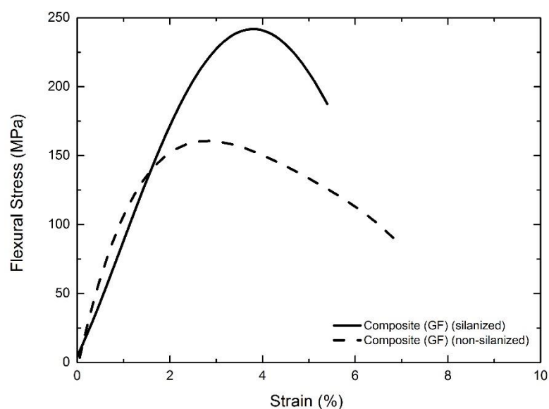
Figure 4.77 Three-point bending test results of prototype composites containing silanized and non-silanized as-received glass fiber woven fabrics.
