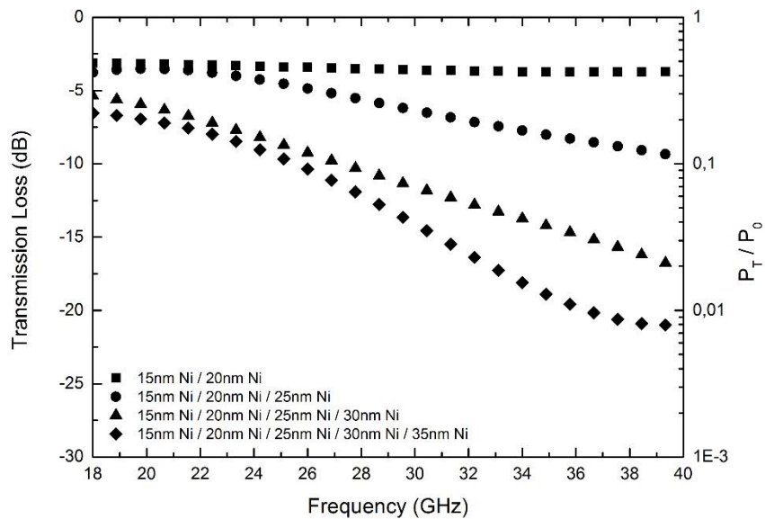
Figure 4.37 EM wave transmission loss varying with frequency in nickel surface modified multilayered glass fiber woven fabrics.
