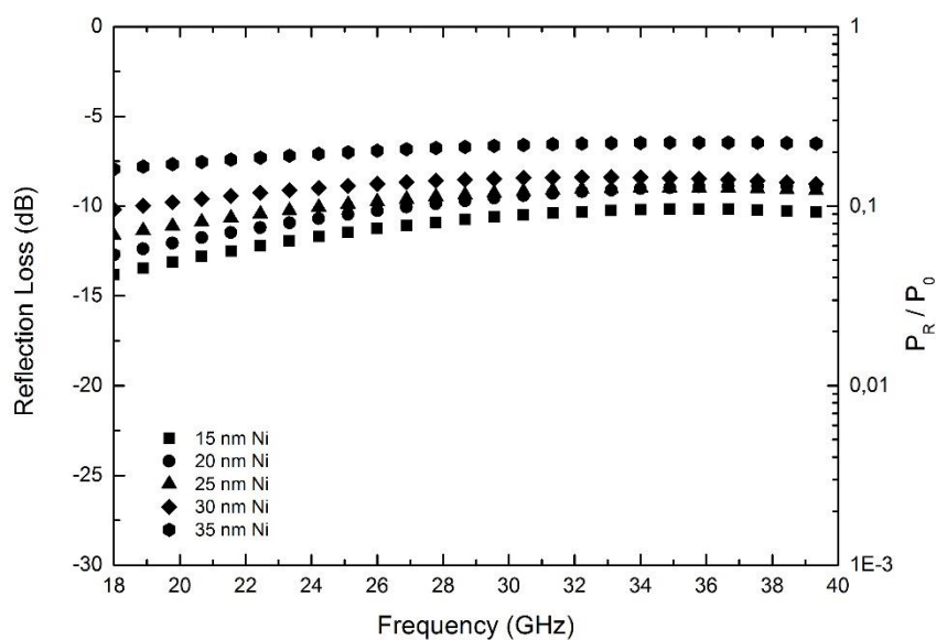
Figure 4.47 EM wave reflection loss varying with frequency in nickel surface modified single layer aramid fiber woven fabrics.
