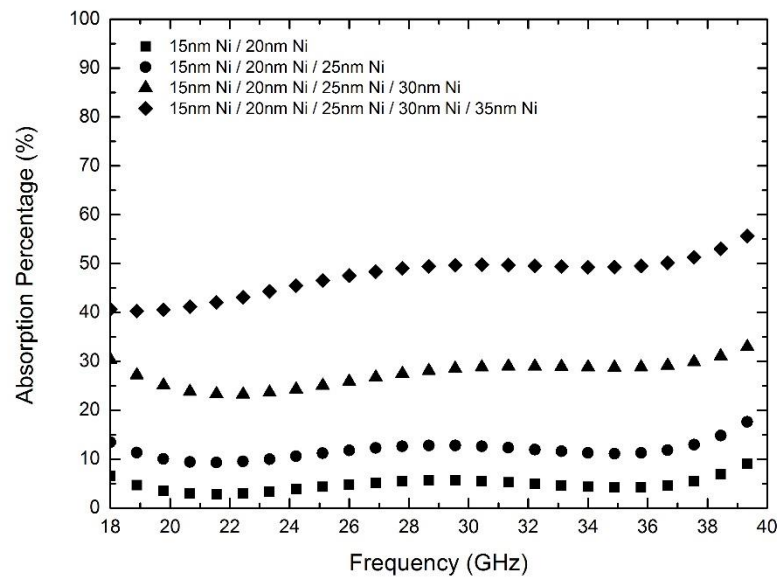
Figure A.23 EM wave absorption percentage varying with frequency in silanized nickel surface modified multilayered aramid fiber woven fabrics.
