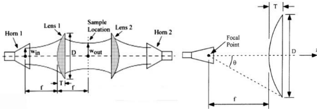
Figure 3.8 Schematic view of layout for free-space method and polymeric lenses with specific dimensions [43].
