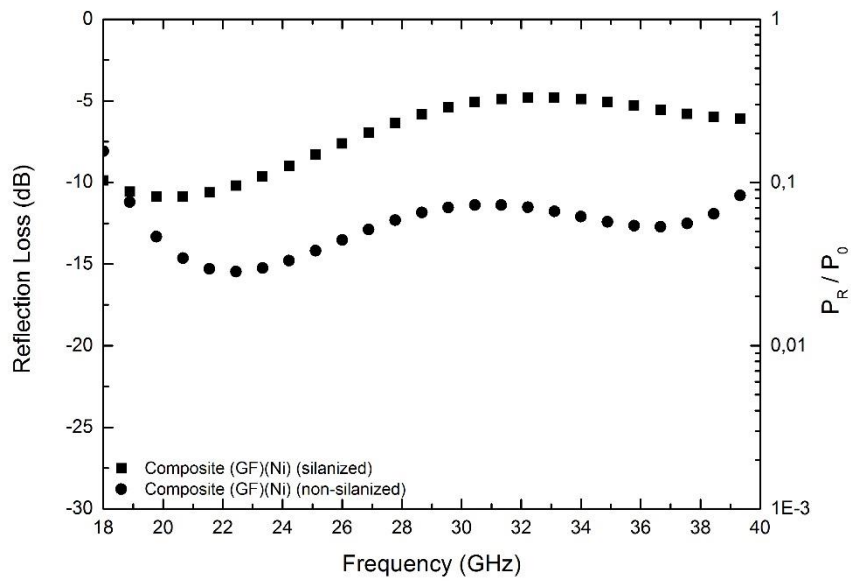
Figure 4.62 EM wave reflection loss varying with frequency in silanized and non-silanized composites containing nickel surface modified multilayered glass fiber woven fabrics.
