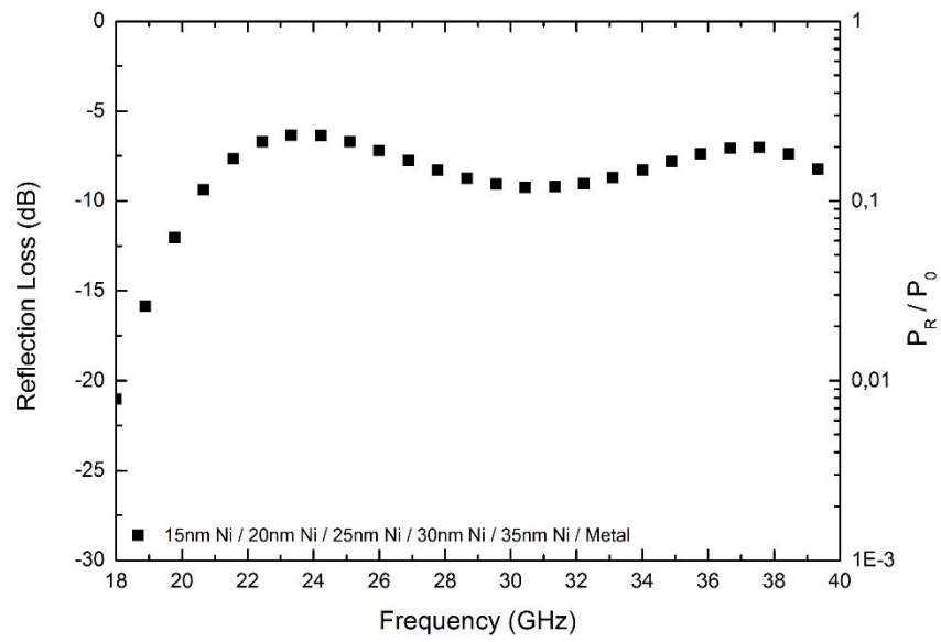
Figure A.12 EM wave reflection loss varying with frequency in silanized nickel surface modified multilayered glass fiber woven fabrics with backing metallic plate.
