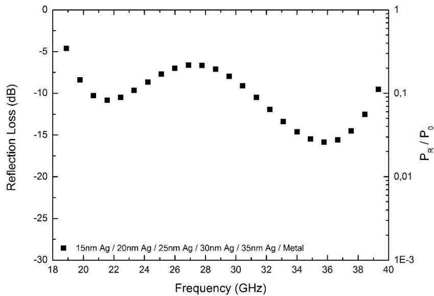
Figure 4.27 EM wave reflection loss varying with frequency in oxidized silver surface modified 5-layered glass fiber woven fabric with metallic backing plate.
