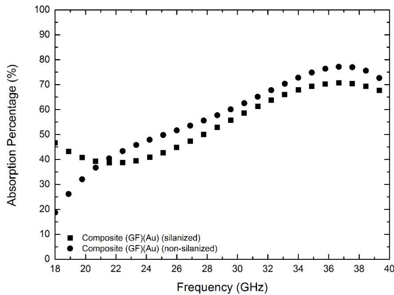
Figure 4.60 EM wave absorption percentage varying with frequency in silanized and non-silanized composites containing gold surface modified multilayered glass fiber woven fabrics.
