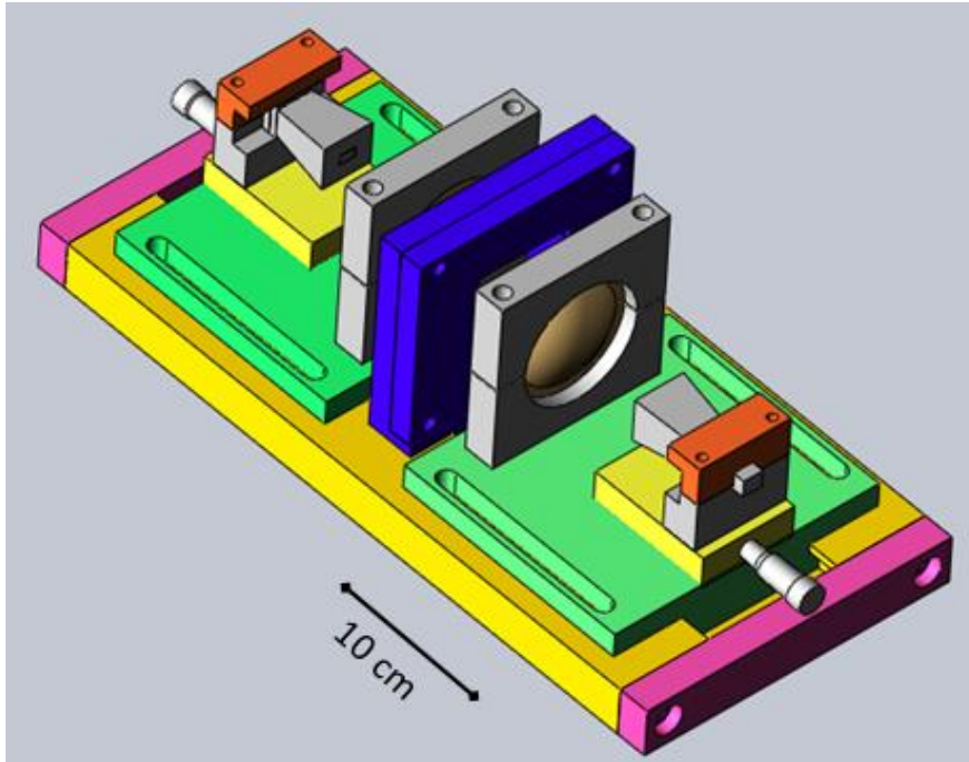
Figure 3.10 Isometric view of designed layout of Free-space method.
