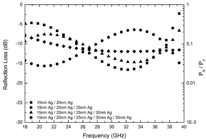
Figure 4.24 EM wave reflection loss varying with frequency in oxidized silver surface modified multilayered glass fiber woven fabrics.
