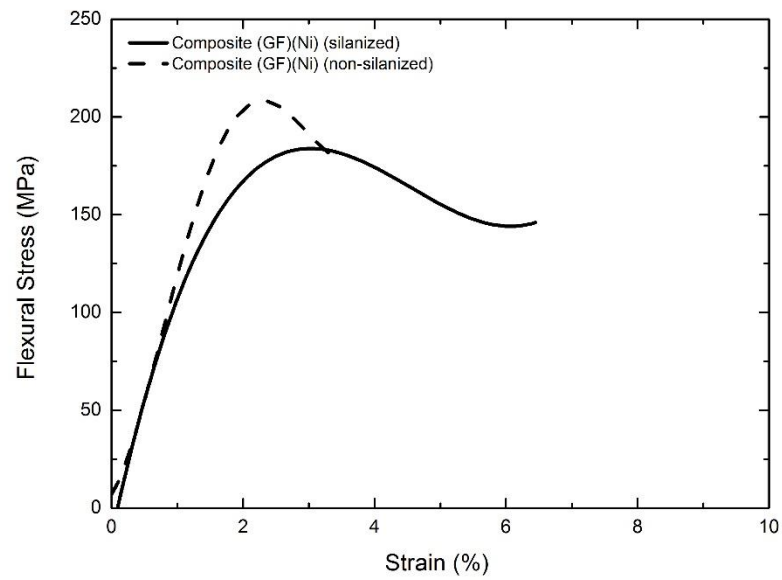
Figure 4.79 Three-point bending test results of prototype composites containing silanized and non-silanized nickel surface modified glass fiber woven fabrics.
