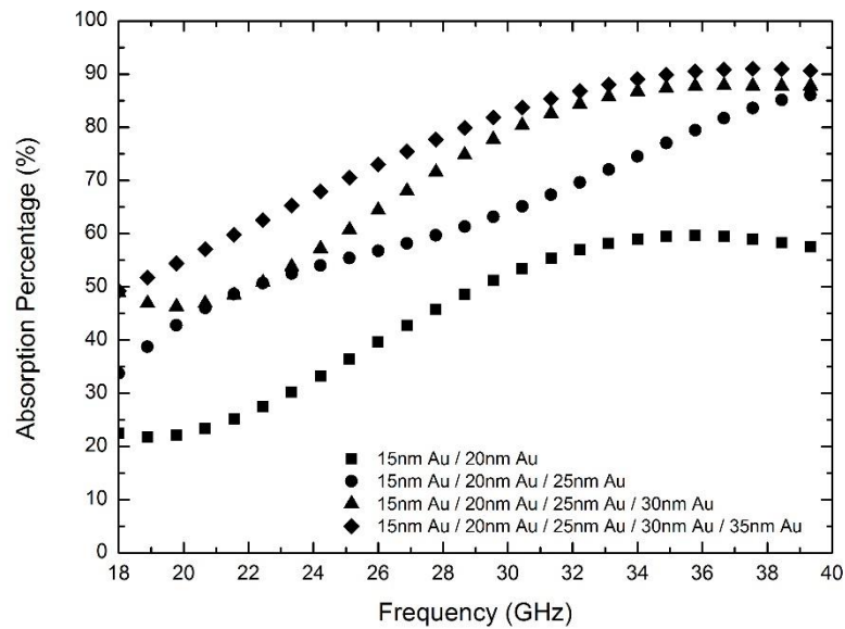
Figure 4.32 EM wave absorption percentage varying with frequency in gold surface modified multilayered glass fiber woven fabrics.
