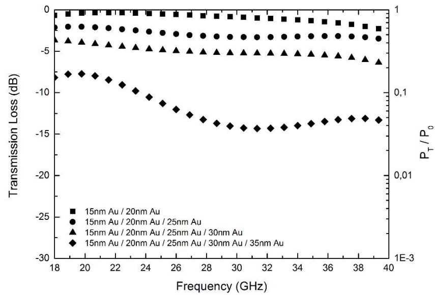
Figure A.16 EM wave transmission loss varying with frequency in silanized gold surface modified multilayered aramid fiber woven fabrics.
