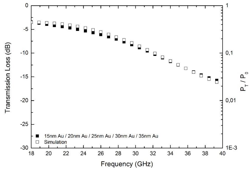
Figure A.29 EM wave transmission loss comparison of five layer gold surface modified aramid fiber structure and its simulation.
