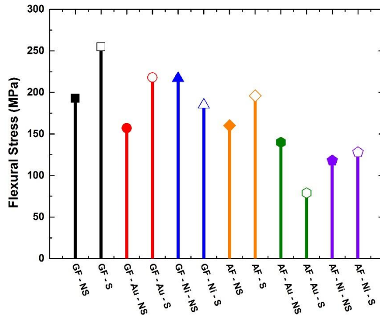
Figure 4.85 Maximum flexural stress values achieved in 12 different composite types.
