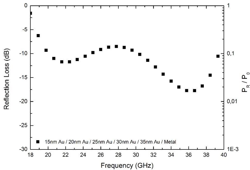
Figure 4.33 EM wave reflection loss varying with frequency in gold surface modified 5-layered glass fiber woven fabrics with metallic backing plate.
