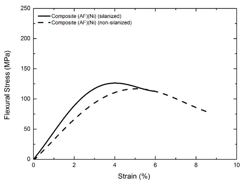
Figure 4.82 Three-point bending test results of prototype composites containing silanized and non-silanized aramid surface modified aramid fiber woven fabrics.
