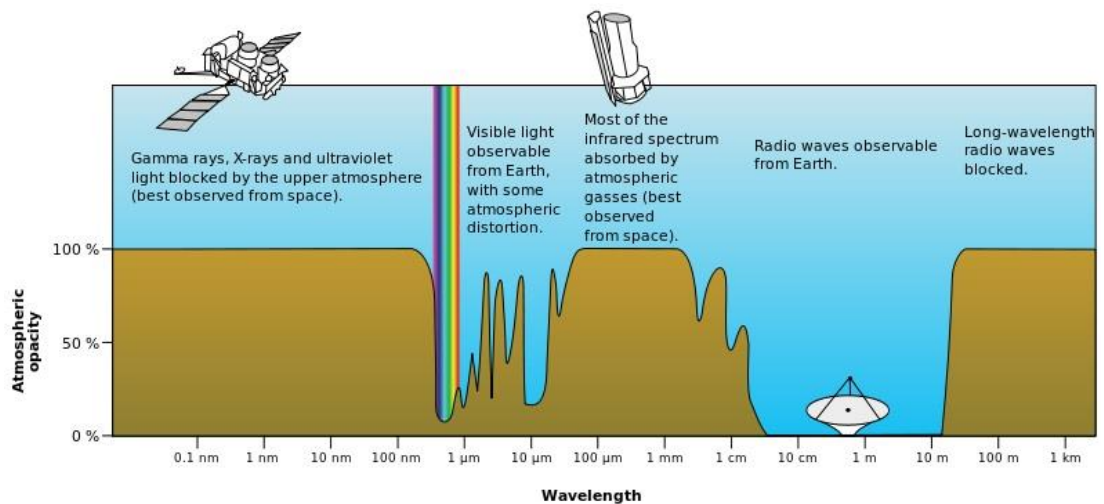
Figure 2.2 Atmospheric opacity [7].
