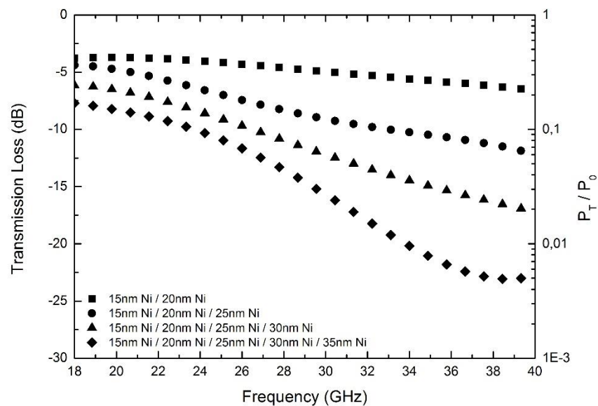
Figure A.10 EM wave transmission loss varying with frequency in silanized nickel surface modified multilayered glass fiber woven fabrics.
