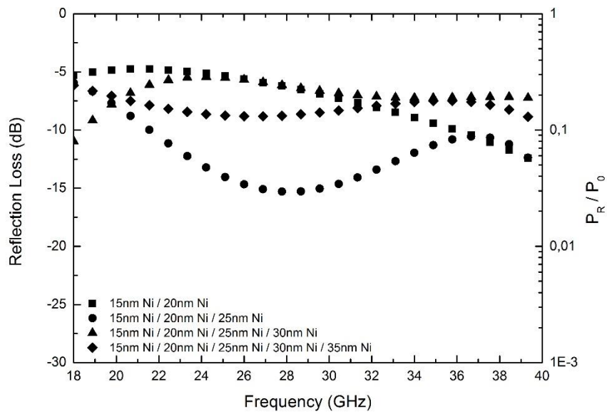
Figure 4.36 EM wave reflection loss varying with frequency in nickel surface modified multilayered glass fiber woven fabrics.
