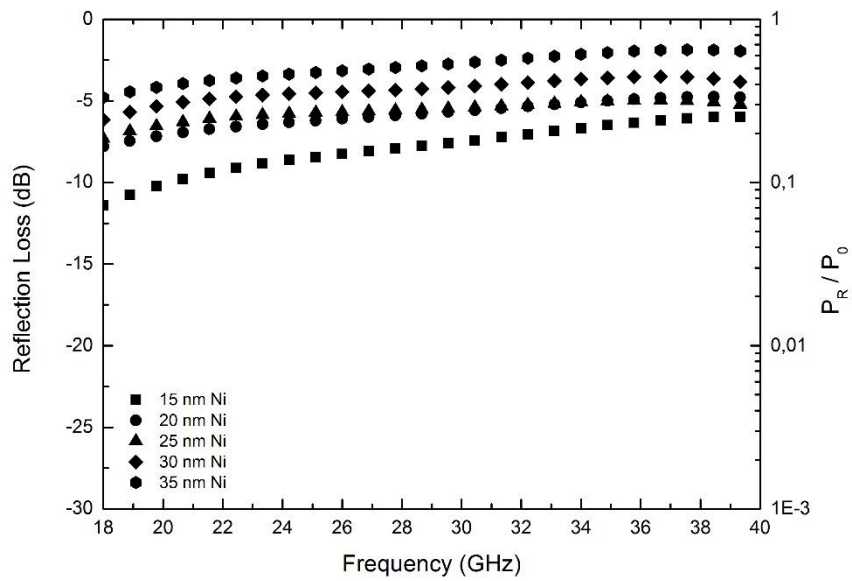
Figure 4.34 EM wave reflection loss varying with frequency in nickel surface modified single layer glass fiber woven fabrics.
