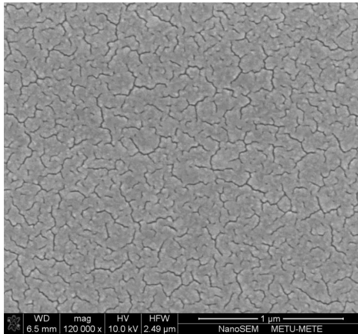
Figure 4.2 Surface morphology of 15 nm Au thin film on silicon wafer, photo taken by FESEM under x120000 magnification.
