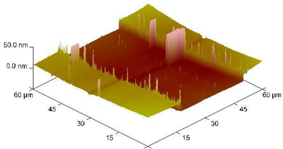
Figure 4.12 3D microstructure of the scratch, photo taken using AFM on the 15 nm thick Au film on silicon wafer (60 μm x 60 μm area).
