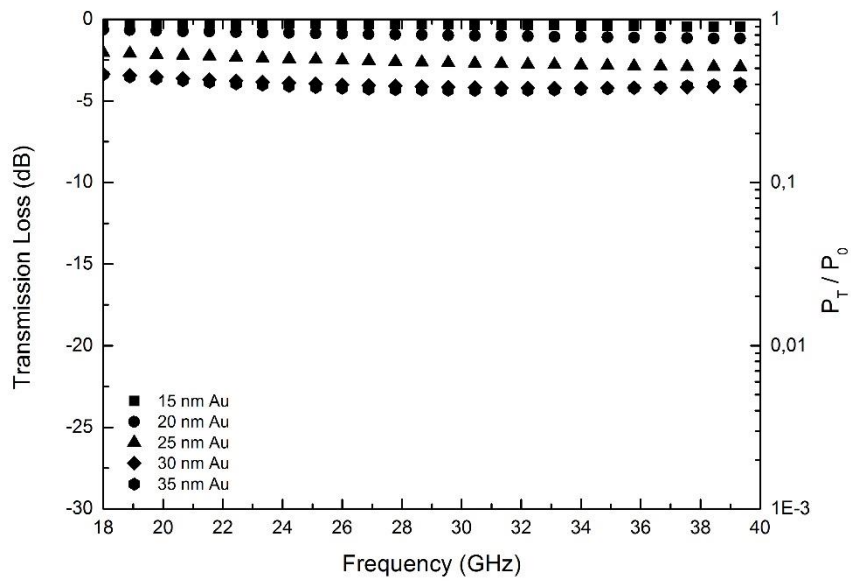
Figure A.14 EM wave transmission loss varying with frequency in silanized gold surface modified single layer aramid fiber woven fabrics.
