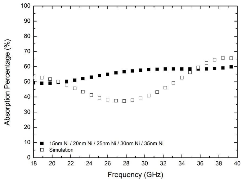
Figure A.27 EM wave absorption percentage comparison of five layer nickel surface modified glass fiber structure and its simulation.
