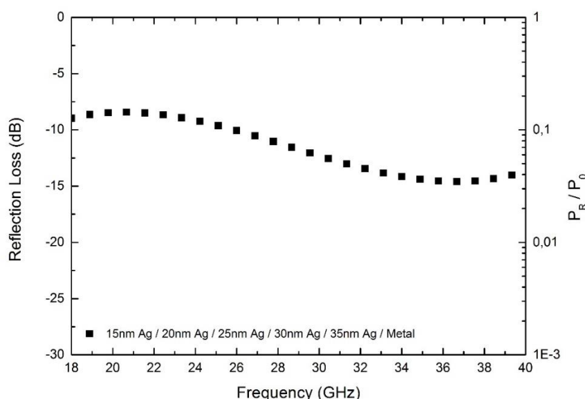
Figure 4.21 EM wave reflection loss varying with frequency in silver surface modified multilayered (5-layered) glass fiber woven fabric with metallic backing plate.
