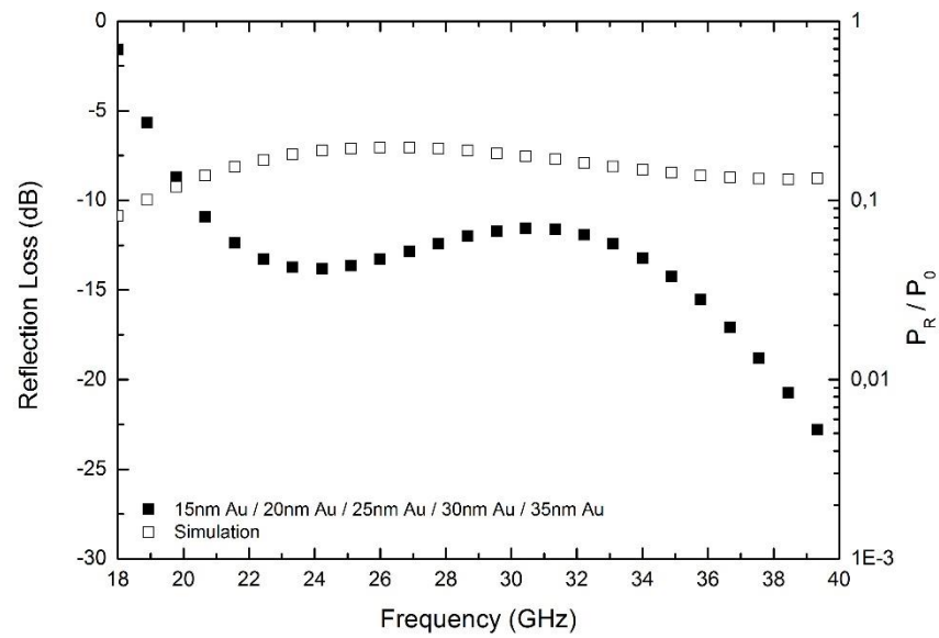
Figure 4.74 Comparison of measured and simulated EM wave reflection loss of gold surface modified 5-layered glass fiber woven fabric structure.
