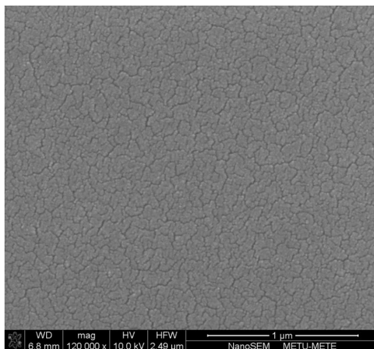
Figure 4.3 Surface morphology of 20 nm Au thin film on silicon wafer, photo taken by FESEM under x120000 magnification.
