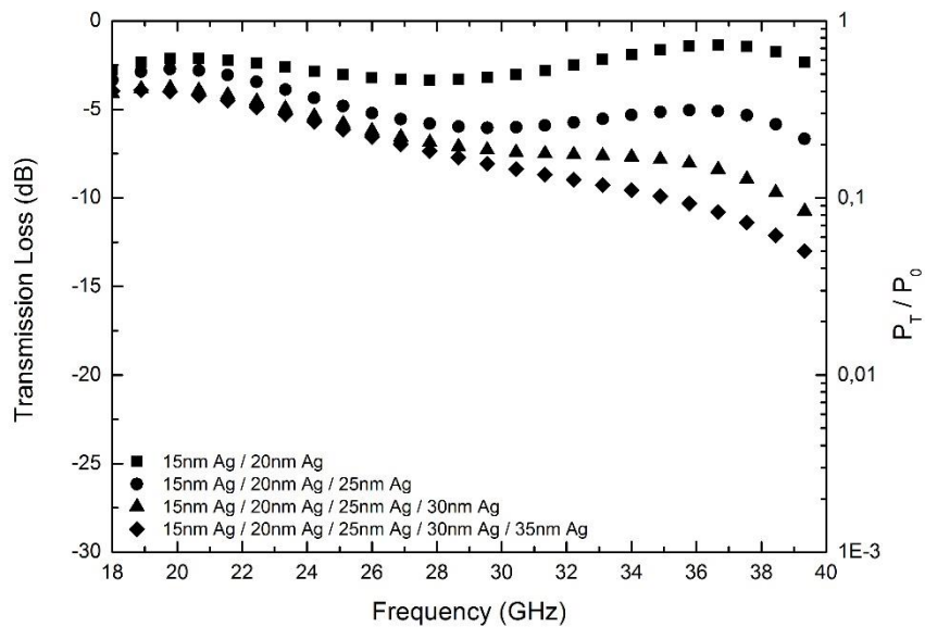
Figure 4.19 EM wave transmission loss varying with frequency in silver surface modified multilayered glass fiber woven fabrics.
