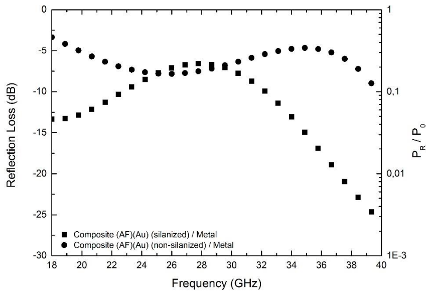
Figure 4.69 EM wave reflection loss varying with frequency in silanized and non-silanized composites containing gold surface modified multilayered aramid fiber woven fabrics under the presence of a metallic backing plate.
