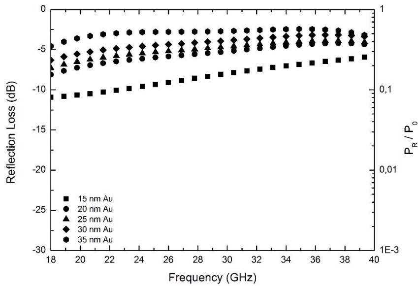
Figure 4.28 EM wave reflection loss varying with frequency in gold surface modified single layer glass fiber woven fabrics.
