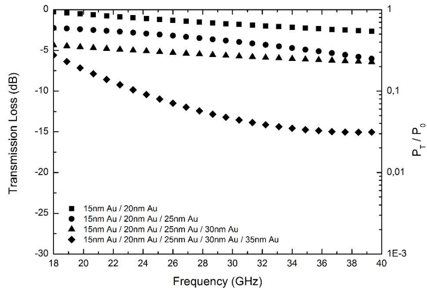
Figure 4.43 EM wave transmission loss varying with frequency in gold surface modified multilayered aramid fiber woven fabrics.
