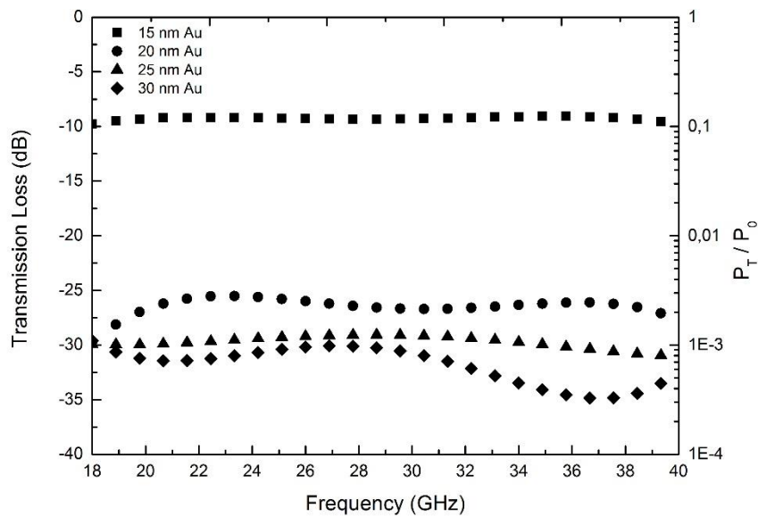
Figure 4.54 EM wave transmission loss varying with frequency in gold surface modified single layer PET sheets.
