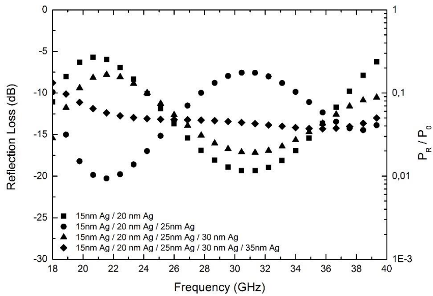
Figure 4.18 EM wave reflection loss varying with frequency in silver surface modified multilayered glass fiber woven fabrics.
