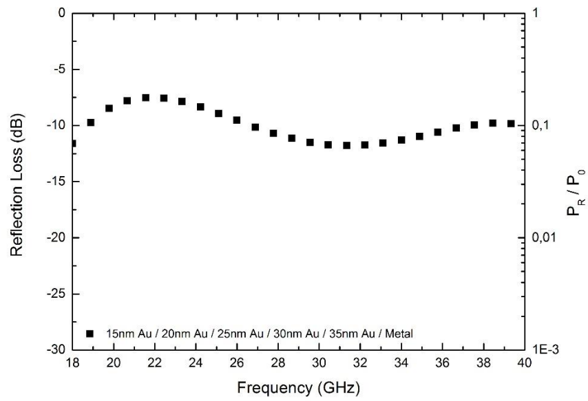
Figure A.6 EM wave reflection loss varying with frequency in silanized gold surface modified multilayered glass fiber woven fabrics with backing metallic plate.
