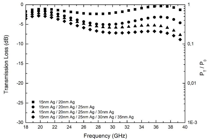
Figure 4.25 EM wave transmission loss varying with frequency in oxidized silver surface modified multilayered glass fiber woven fabrics.
