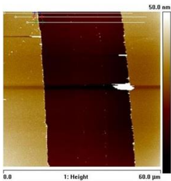
Figure 4.13 2D microstructure of the scratch, photo taken using AFM on the 15 nm thick Au film on silicon wafer (60 μm x 60 μm area) and thickness measurement.
