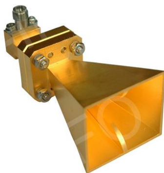
Figure 3.6 Horn antenna used in free-space measurement system.
