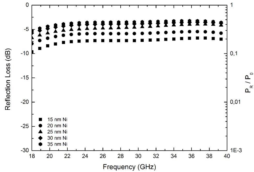
Figure A.7 EM wave reflection loss varying with frequency in silanized nickel surface modified single layer glass fiber woven fabrics.
