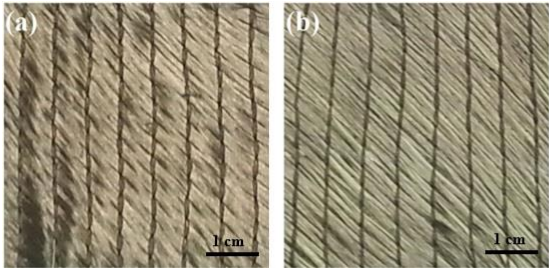
Figure 4.46. Aramid fiber woven fabrics with gold surface modification as (a) non-silanized and (b) silanized.
