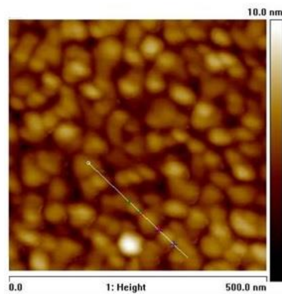
Figure 4.9 2D microstructure photo taken using AFM of 15 nm thick Au film on silicon wafer (500 nm x 500 nm area) and nuclei size determination.
