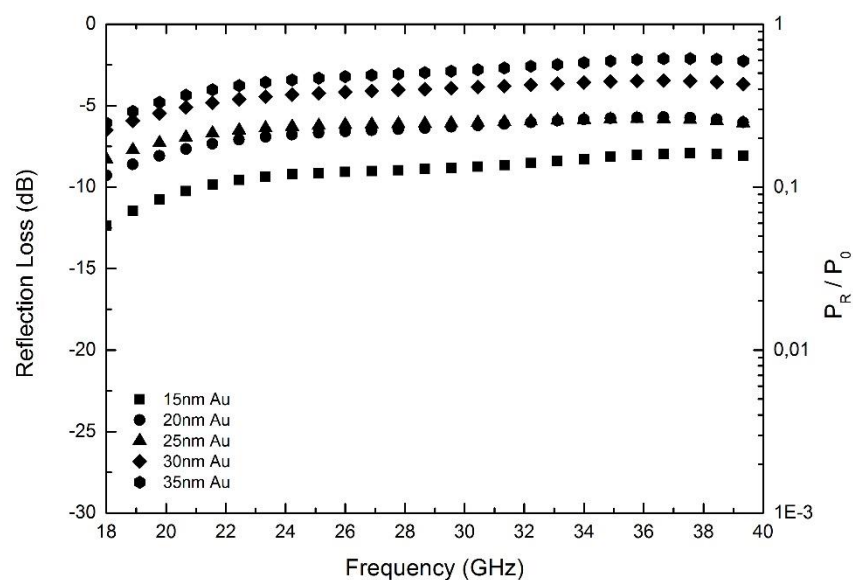
Figure A.1 EM wave reflection loss varying with frequency in silanized gold surface modified single layer glass fiber woven fabrics.
