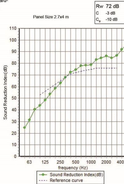
Figure E.42 Estimated data of Gw' proposal of Original Wall 4.
