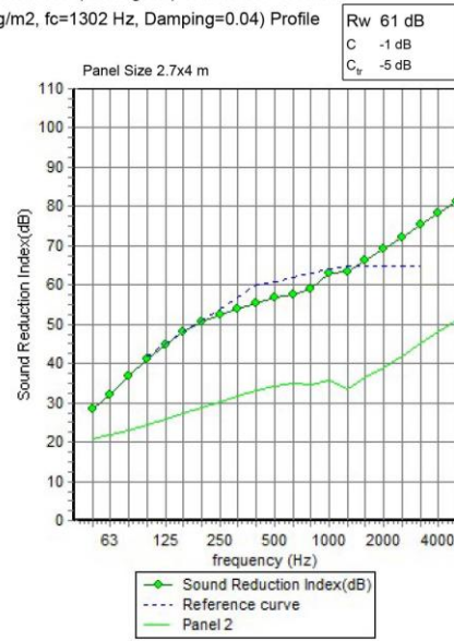
Figure F.17 Estimated data of II F -E proposal of Semi-Repaired-Floor 2/3.
