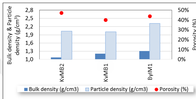
Figure 4.22 Bulk density, particle density and porosity values of the samples.
