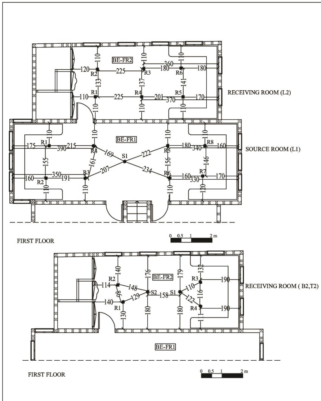
Figure B.1 Measurement of airborne sound transmission through Reconstructed-Wall 1(W1-BE-FR1/R2).
