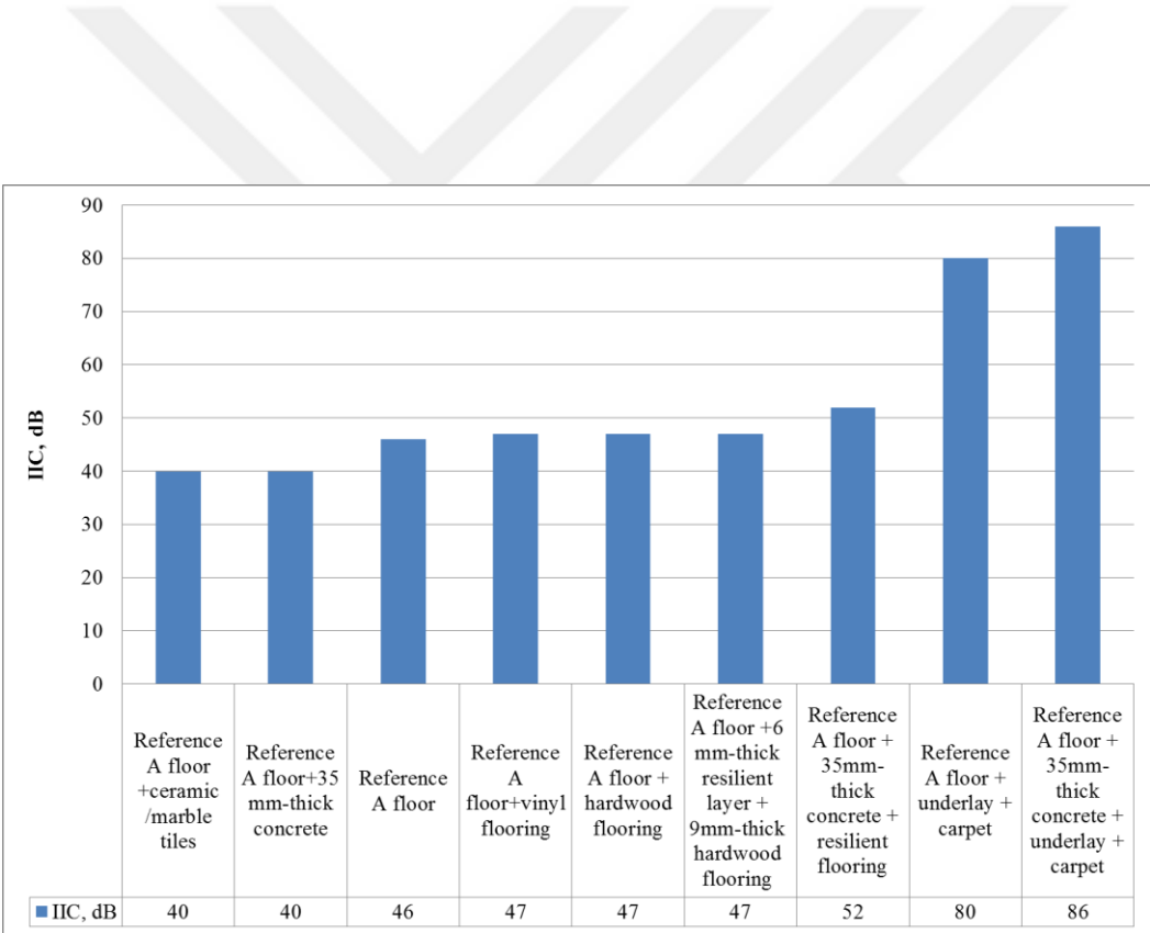
Figure 2.9 IIC values of Reference A floor with different toppings.
