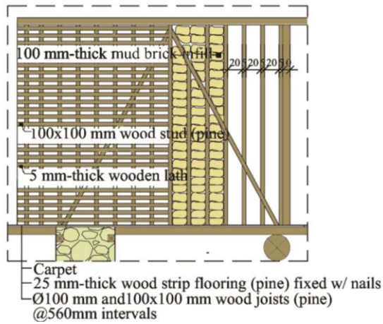
Figure 3.25 Elevations of Original-Wall 4 & sections of Original-Floor 4 in 1/50 scale (Drawn by author).
