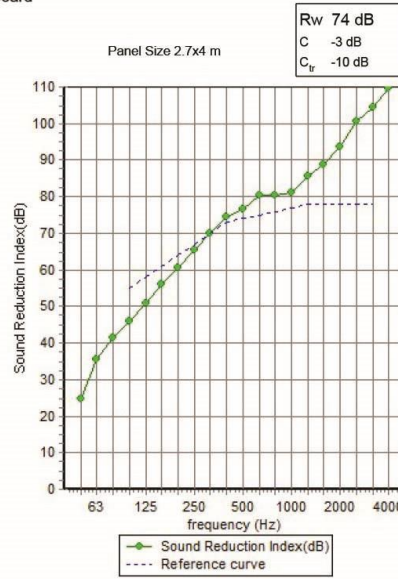
Figure E.41 Estimated data of Hw proposal of Original Wall 4.
