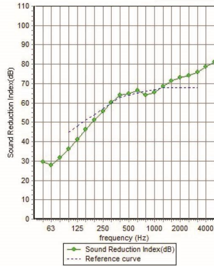
Figure E.37 Estimated data of Cw' proposal of Original Wall 4.
