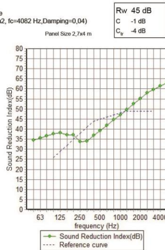
Figure D.2 Estimated data of Semi-Repaired-Wall 2/3.
