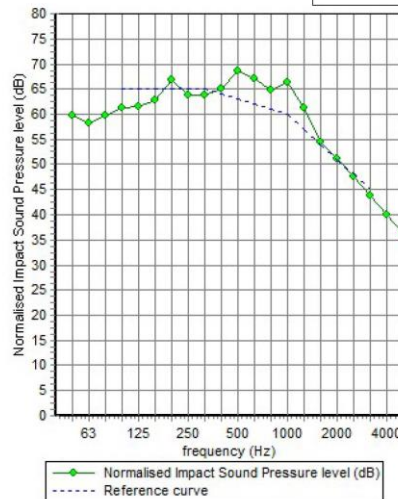
Figure F.6 Estimated data of IF-C proposal of Reconstructed-Floor 1.
