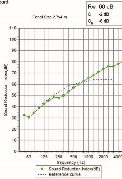
Figure E.21 Estimated data of Cw proposal of Semi-Repaired-Wall2/3.
