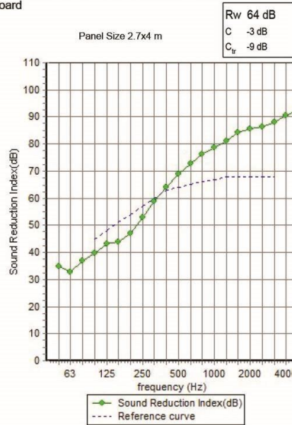
Figure E.11 Estimated data of Ew proposal of Reconstructed-Wall 1.
