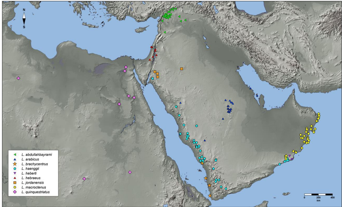
Figure 1.6 Distribution of Leirus species, focusing on Arabian Peninsula, northeastern Africa and Middle East. (Lowe et al. 2014)
