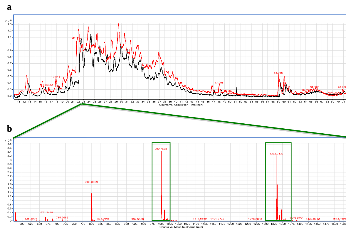
Figure C.2 (a) Mass chromatogram of Leiurus abdullahbayrami venom peptide fraction from second 11 to 70. (b) Zoomed chromatogram at 22.56 th second, observed peaks are marked in green. m/z ratios of the same mass (3996 Da) in different charges can be seen at the top.
