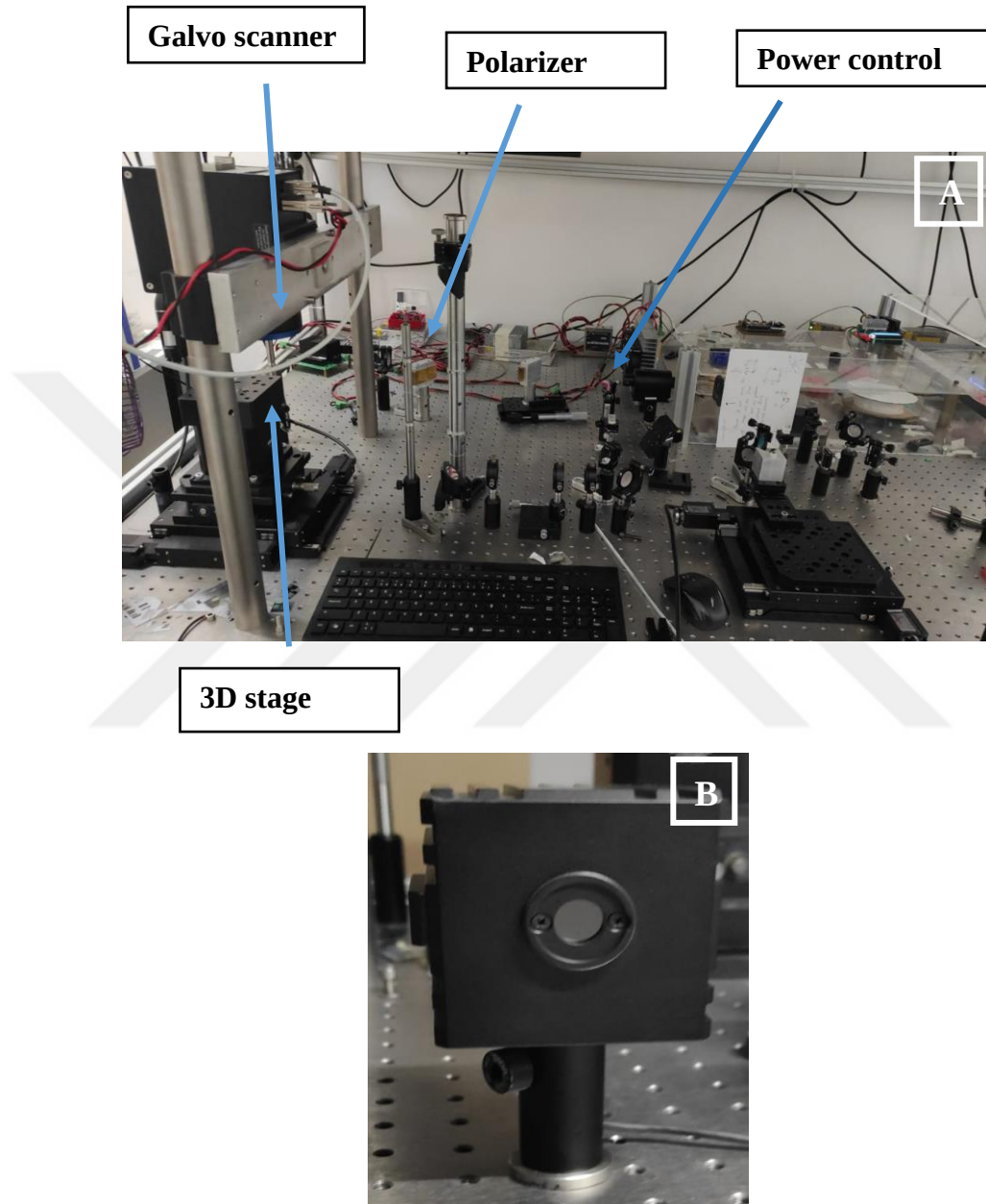
Figure 2.2: (A) A picture of the laser and the structuring setup showing the Galvo scanner, 3D stage, polarizer, power control, and other optical elements, (B) power meter for controlling the power of the laser
