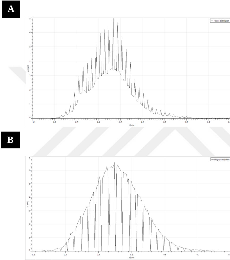
Figure 3.5: Height distribution analysis in LIPSS (A) and microcolumn (B) topography by height distribution function P(Z) .
