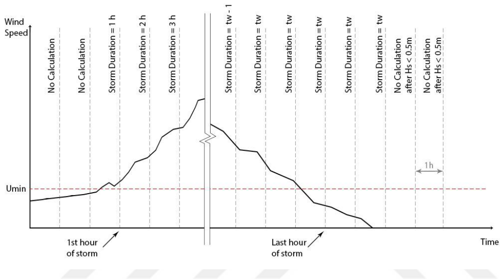
Figure 3-2 Storm-Based with User-Defined Duration Concept
