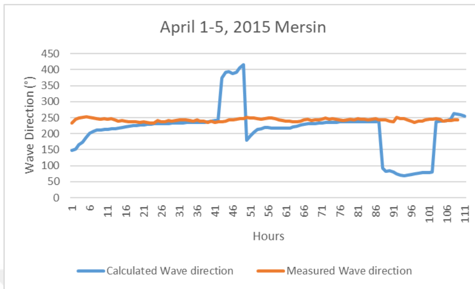
Figure 4-27 Wave Directions, Mersin 1-5 April 2015
