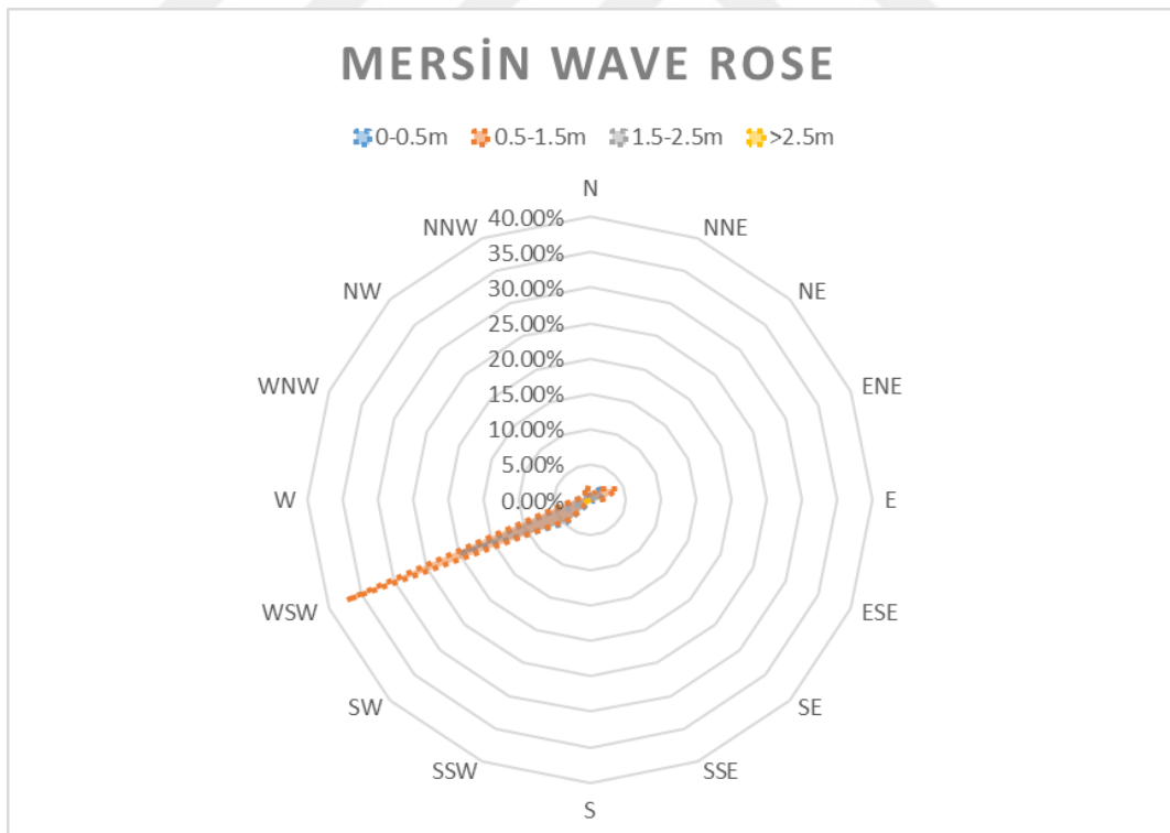
Figure 3-17 Mersin Wave Rose
