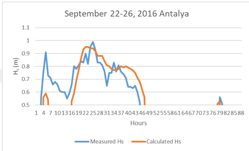
Figure 4-20 Wave Heights, Antalya 22-26 September 2016
