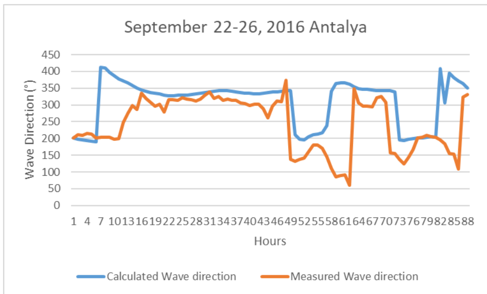
Figure 4-22 Wave Directions, Antalya 22-26 September 2016
