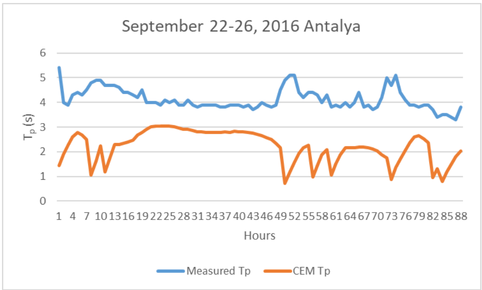
Figure 4-21 Wave Periods, Antalya 22-26 September 2016
