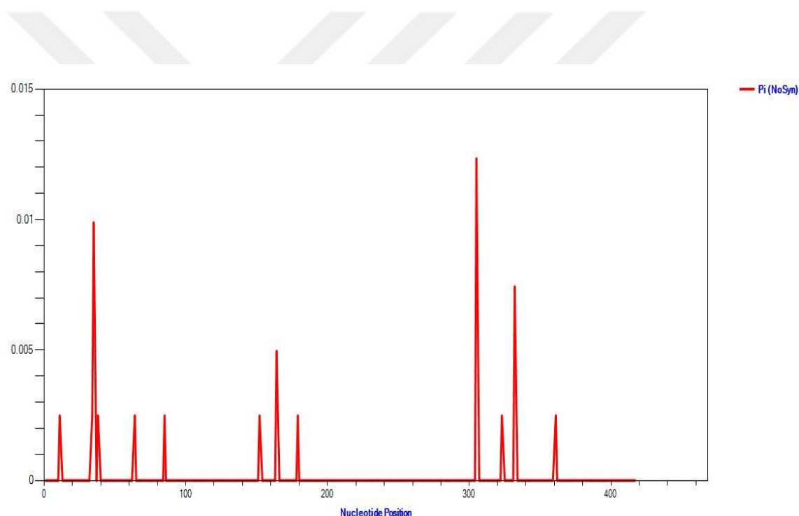
Figure 8. Sliding Window analysis of nonsynonymous nucleotide diversity for Nsp10
