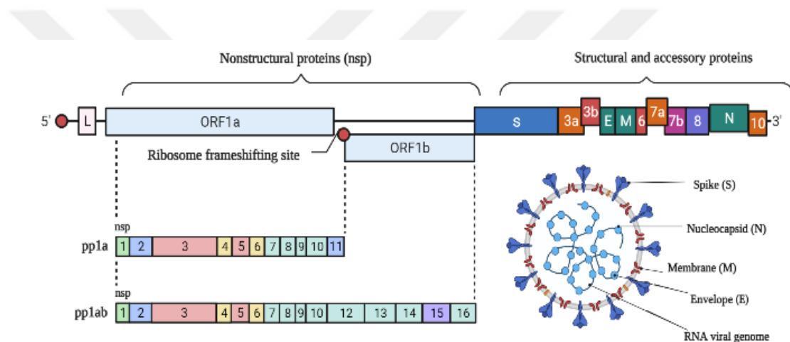
Figure 3. The genomic organization of SARS-CoV-2. (Created with BioRender)
