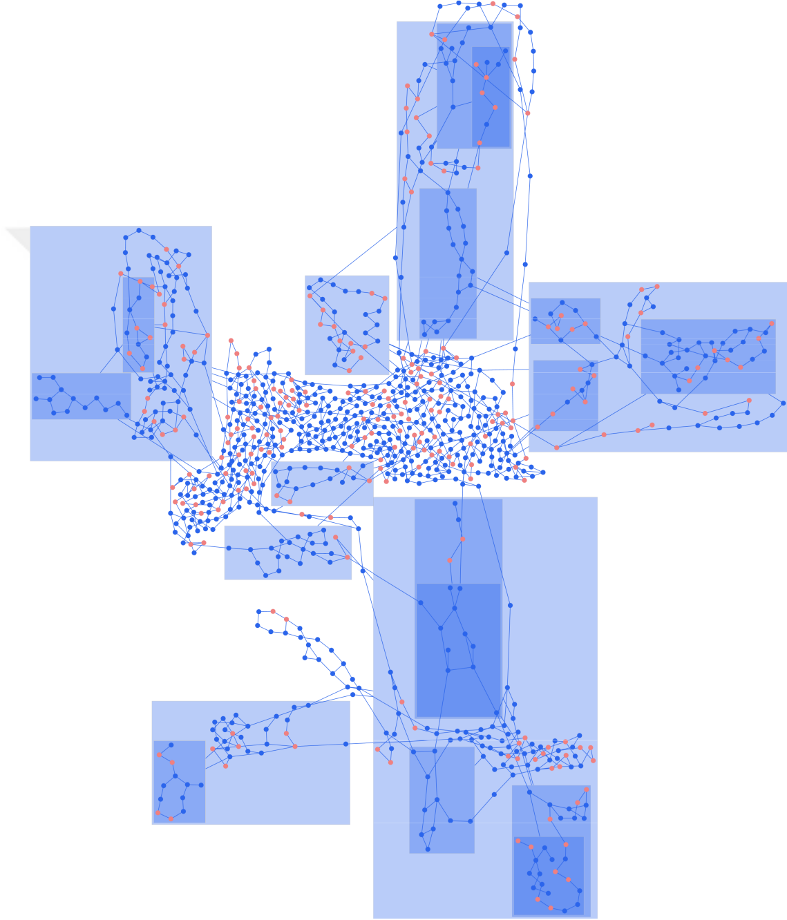
Figure 5.7: A sample layout of a medium-sized graph from our dataset generated using Rome graphs ( |V| = 1022 , |E| = 1228 , d(G) = 2.4 ). 25% of the simple nodes have alignment constraints shown in red. The layout is generated in 1031.6 ms and has the following quality metrics: average edge length: 130.2, number of edge crossings: 880, number of node-node overlaps: 29, number of node-edge overlaps: 513, and total area: 26225364 square units.
