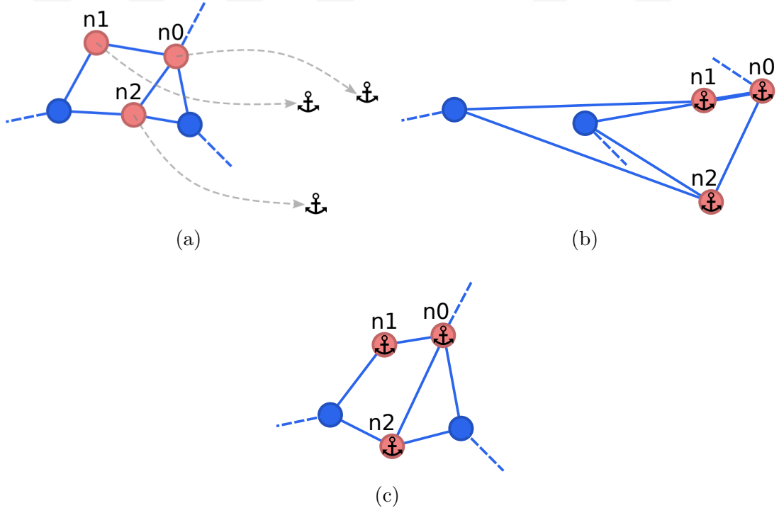
Figure 4.8: (a) Transformed draft layout (same as the one in Figure 4.5b) along with the anchor positions of fixed nodes (b) First, the fixed nodes are moved to anchor positions. (c) Then, the rest of the graph is moved based on the displacement of the fixed nodes.
