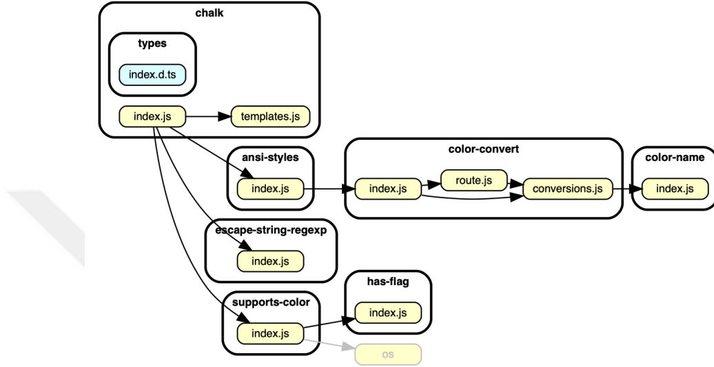
Figure 1.4: A sample layout of a dependency graph that positions nodes (JavaScript files) from left to right based on their dependency relationships and vertically aligns those at the same level [4]
