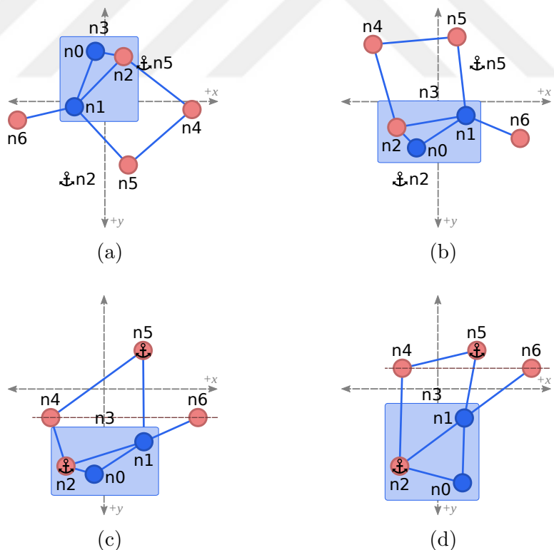
Figure 4.2: The process of applying fCoSE on a sample compound graph with two fixed node constraints ( n2 \dagger [-50, 100] , n5 \dagger [50, -50] ) and one alignment constraint ( n4 - n6 ). (a) After generating a draft layout in Phase I, (b) a transformation is first applied based on the fixed node constraints (transformed draft layout) and then (c) all constraints are enforced (constrained draft layout) in Phase II. (d) The final layout is obtained by applying a modified version of CoSE in Phase III.
