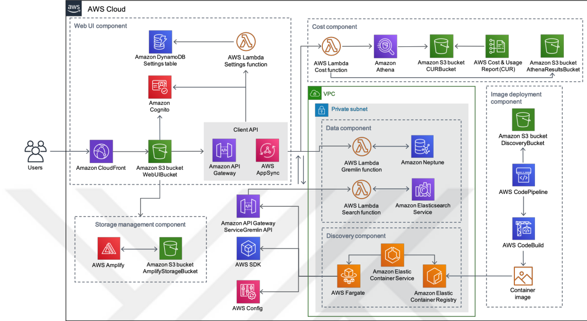
Figure 1.3: Architecture diagram of AWS Perspective, a visualization tool for cloud workloads. [3]
