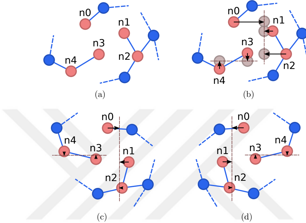
Figure 4.6: (a) Part of a draft layout with alignment constraints n0 \mid n1 \mid n2 and n3 - n4 (b) Black arrows show the required movement for the constrained nodes to be aligned in the corresponding average coordinate to form the target configuration. (c) The transformation step based on the alignment constraints rotates the draft layout by 44.5^\circ clockwise. (d) Additional process of relative placement constraints n1 < n3 , n2 < n4 , n0 \wedge n1 and n2 \wedge n4 on the transformed draft layout in (c) reflects the graph on y -axis.
