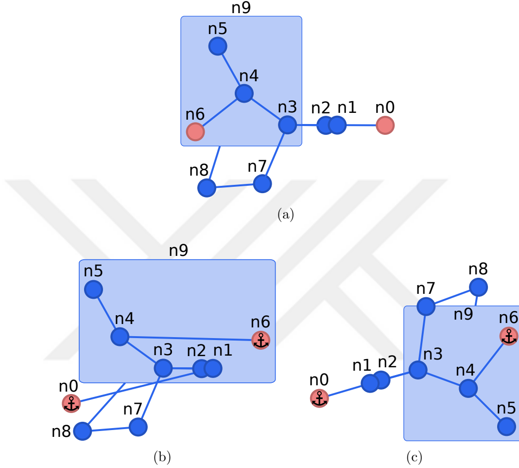
Figure 4.4: (a) A sample draft layout with two fixed node constraints n0 \dagger [-150, 50] and n6 \dagger [150, -50] (b) Constrained draft layout obtained by skipping the transformation step and (c) by applying a transformation step that rotates the draft layout by 163.5^\circ clockwise
