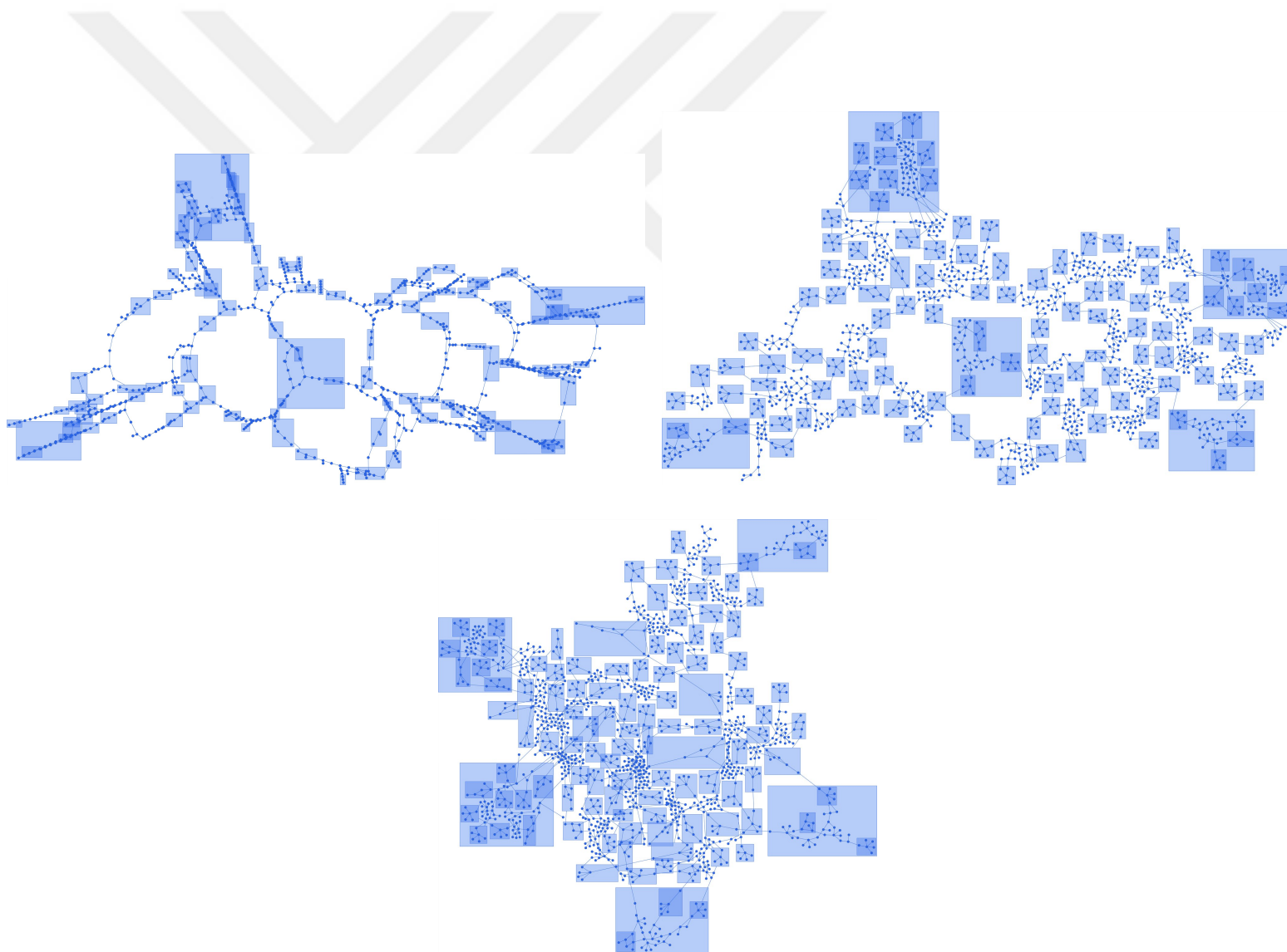
Figure 5.9: Comparison between fCoSE and CoSE algorithms on a randomly generated compound graph ( |V| = 1525 , |E| = 1527 , d(G) = 2 ). Draft layout generated after Phase I of fCoSE, run time: 123.4 ms (top-left). Final layout after Phase III is applied directly on top of the draft layout for polishing, run time 175.9 ms (top-right). Same graph laid out with CoSE, run time: 579.4 ms (bottom). Notice how the construction of a draft layout as a first step of fCoSE beautifies the layout and makes it run faster (299.3 ms in total vs 579.4 ms) when compared to directly applying CoSE algorithm.
