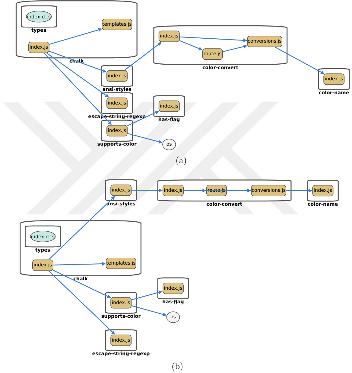
Figure 5.1: A sample dependency graph of a JavaScript project [4] with |V| = 20 , |E| = 11 and d(G) = 1.1 where the nodes are constrained with relative placement constraints in such a way that each target node will be on the right of the source node while alignment constraints are also introduced for the nodes in the same level to be aligned vertically. Sample layouts generated by (a) fCoSE and (b) CoLa have the following performance and quality metrics (fCoSE - CoLa): run time: 11.79 ms - 167.14 ms, average edge length: 122.19 - 113.23, number of edge crossings: 0 - 2, number of node-node overlaps: 0 - 0, number of node-edge overlaps: 0 - 1, and total area: 267314 - 303002 square units.
