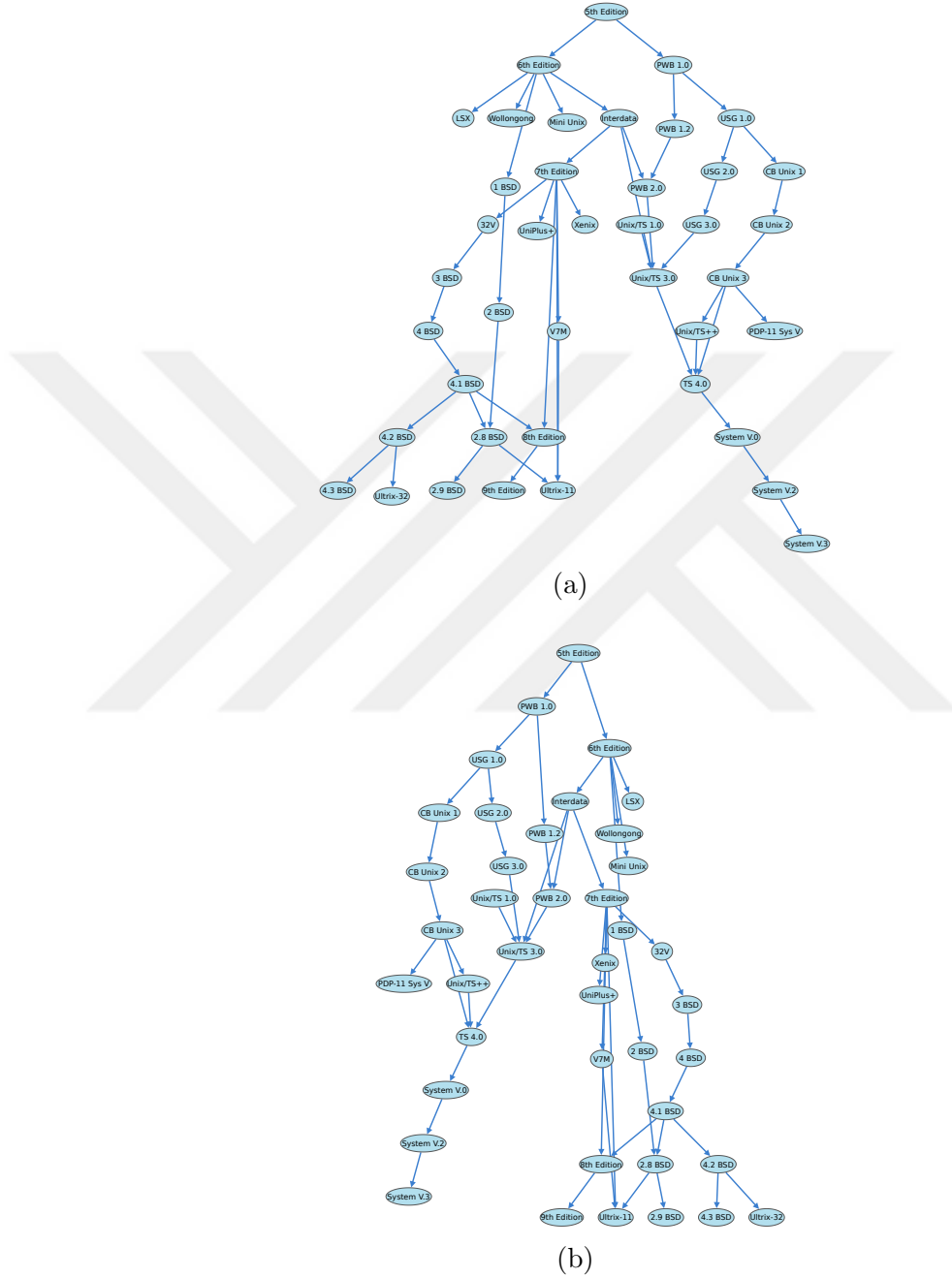
Figure 5.4: Unix family tree [11] with |V| = 41 , |E| = 49 and d(G) = 2.38 where the nodes are constrained with relative placement constraints in such a way that each target node will be below of the source node. Sample layouts generated by (a) fCoSE and (b) CoLa have the following performance and quality metrics (fCoSE - CoLa): run time: 15.25 ms - 317.78 ms, average edge length: 99.37 - 101.93, number of edge crossings: 3 - 4, number of node-node overlaps: 0 - 0, number of node-edge overlaps: 9 - 19, and total area: 579961 - 492325 square units.
