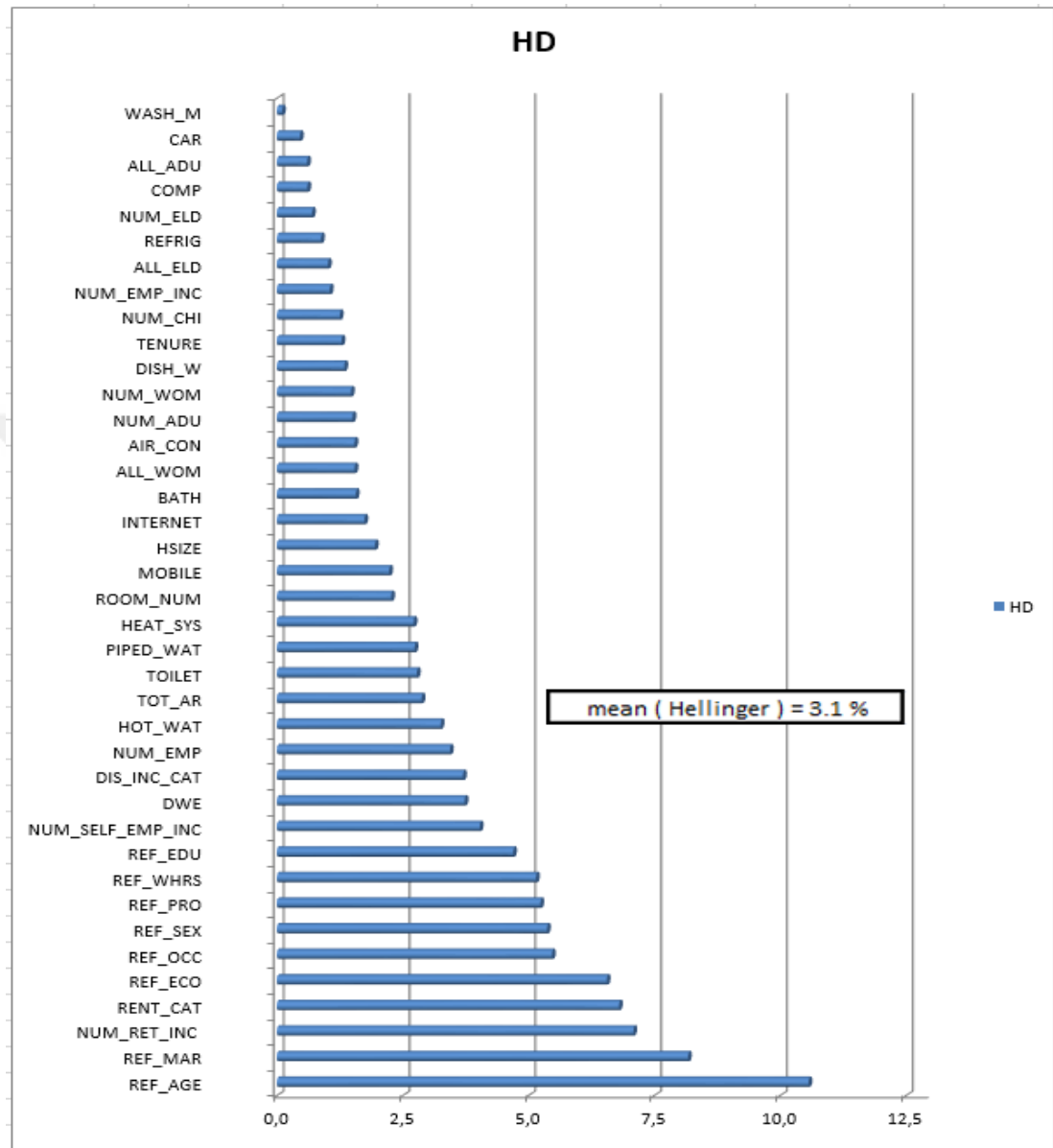
Figure 3.1. Unweighted Hellinger Distance Scores of Common Variables
