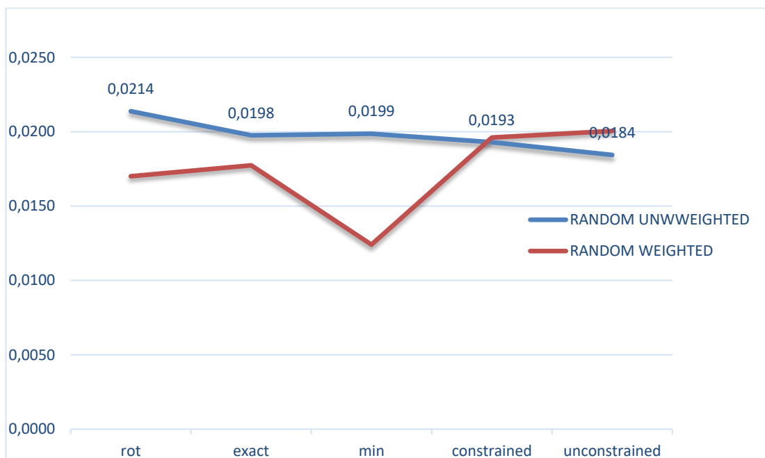
Figure 4.10. Match.vars=Null Results (%)
