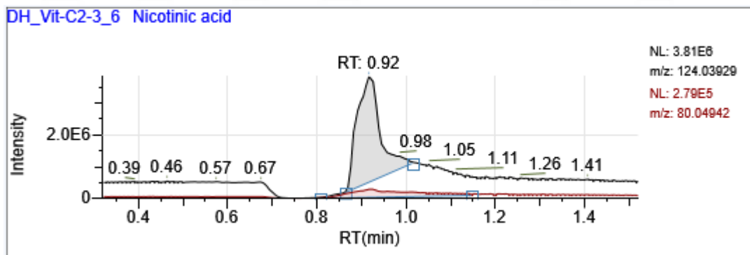
Figure C.10. LC-MS chromatograms of Nicotinic acid of Control PBRs 1-2-3.
