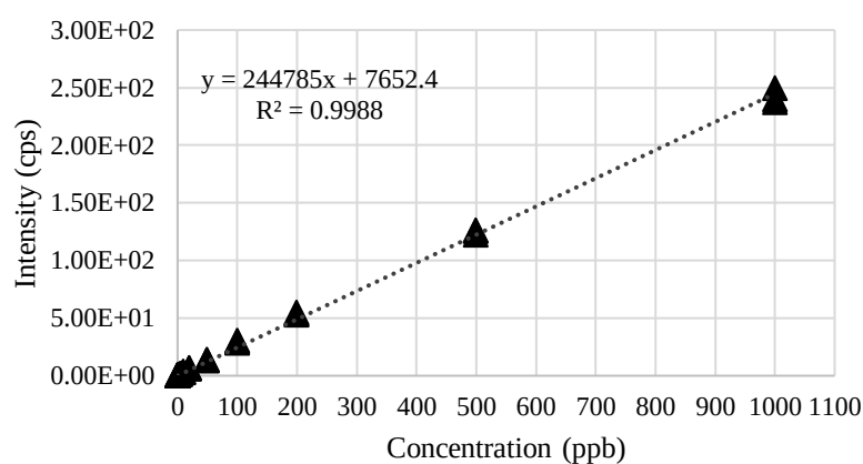
Figure 3.60. Calibration curve of ^{208}\text{Pb} .
