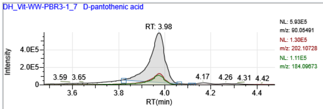
Figure C.3. LC-MS chromatograms of Pantothenic acid of FWW PBRs 1-2-3.
