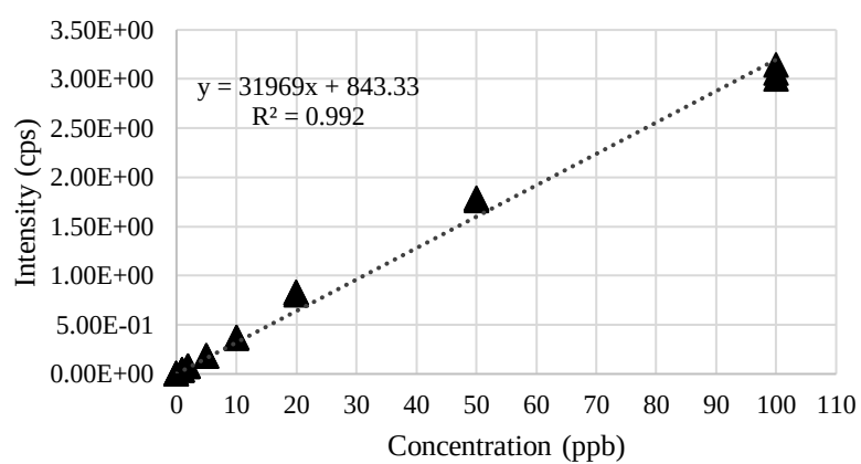
Figure 3.57. Calibration curve of ^{88}\text{Sr} .
