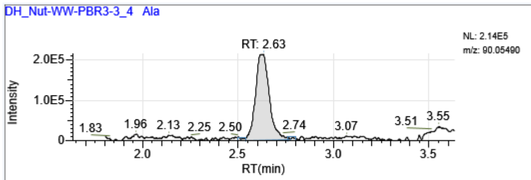
Figure B.2. LC-MS chromatograms of ALA of FWW PBRs 1-2-3
