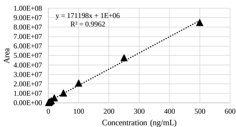
Figure 3.22. Calibration curve of Biotin (B7).
