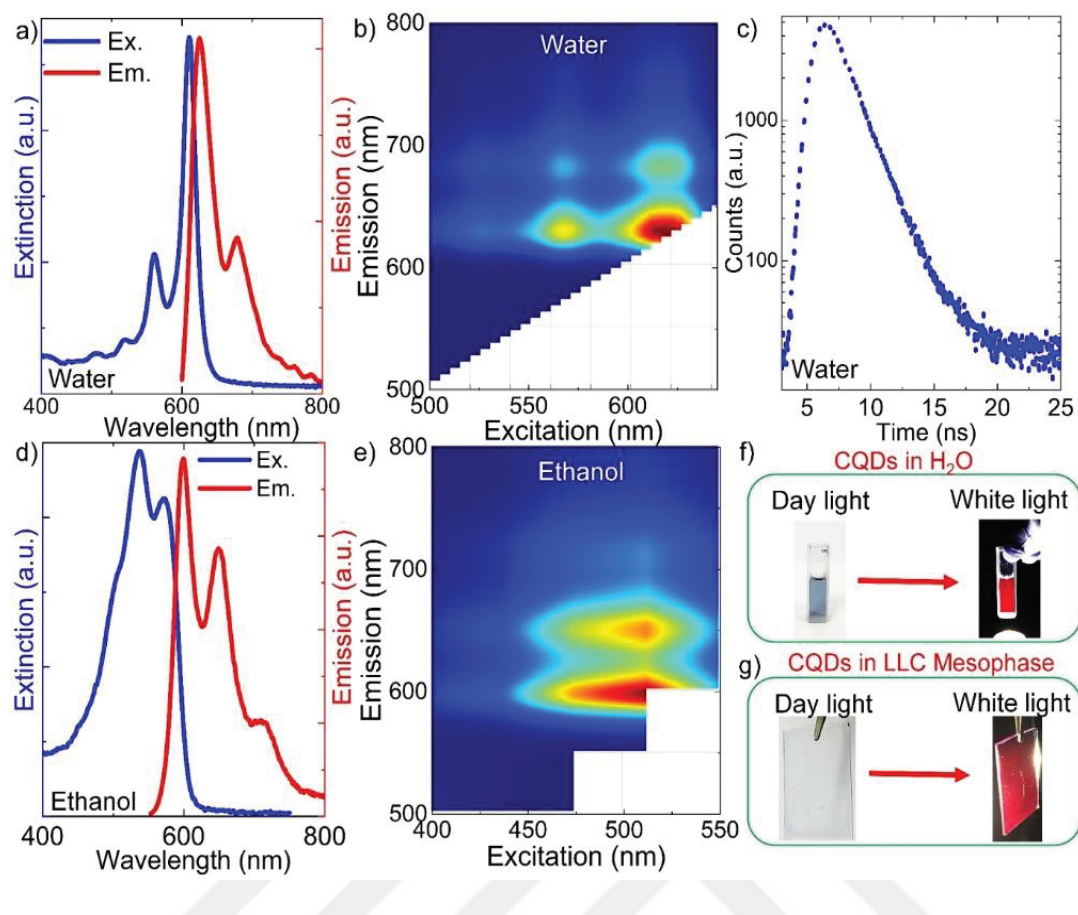
Figure 3.22. Linear optical characteristics of CDs. (a) Extinction and photoluminescence (PL) spectra of CDs measurements in water. (b) 2D excitation-emission map of CDs in water. (c) PL lifetime of CDs in water. The measured PL lifetime of CDs is about 2 ns in water. (d) Extinction and PL spectra of CDs in ethanol. (e) 2D excitation-emission map of CDs in ethanol. (f) Photo of CDs in water was left in the daylight and exposed to white light. (g) Photo of CDs dispersed in the LLC mesophase spin coated on a glass substrate was left in daylight and exposed white light. Red fluorescence emission is exhibited by both aqueous solution and LLC thin films containing CDs. 13 Reprinted with permission from Sarisozen, S.; Polat, N.; Mert Balci, F.; Guvenc, C. M.; Kocabas, C.; Yaglioglu, H. G.; Balci, S. Strong Coupling of Carbon Quantum Dots in Liquid Crystals. The Journal of Physical Chemistry Letters 2022, 3562–3570. https://doi.org/10.1021/acs.jpclett.1c03937 . Copyright 2022 American Chemical Society.
