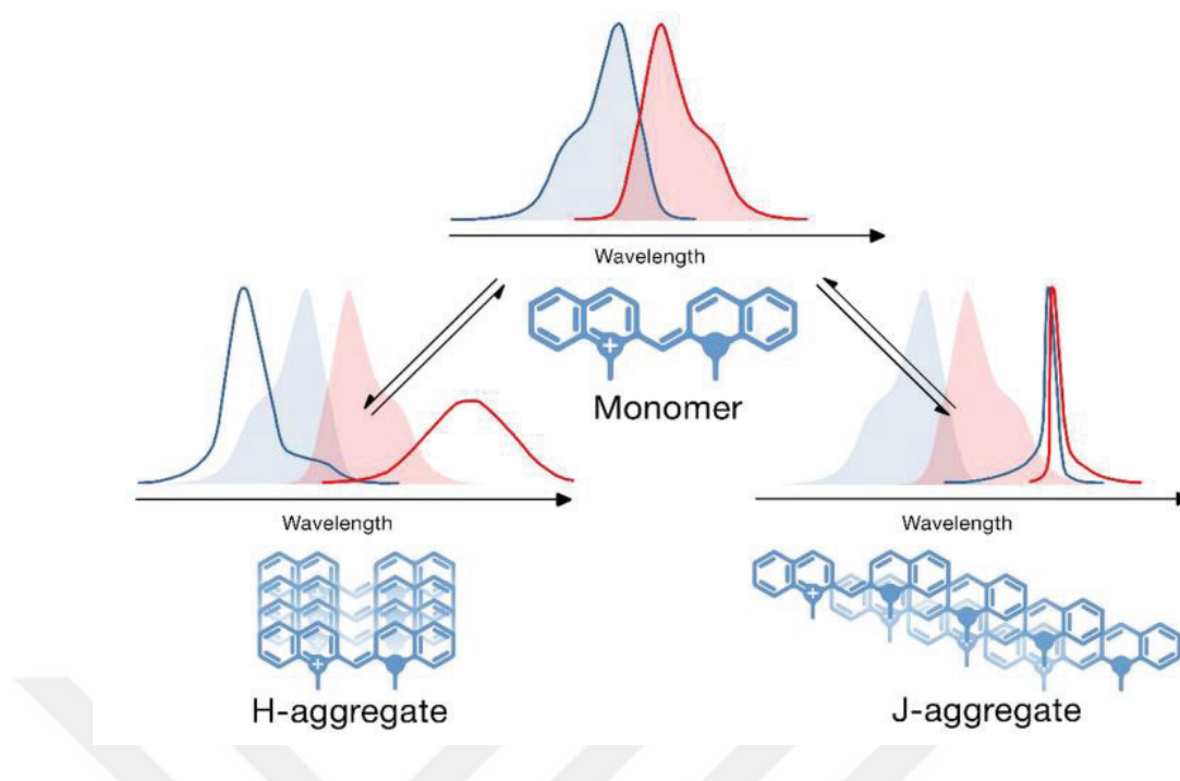
Figure 1.10. Schematic representation of the formation of H- and J-aggregates. 8
