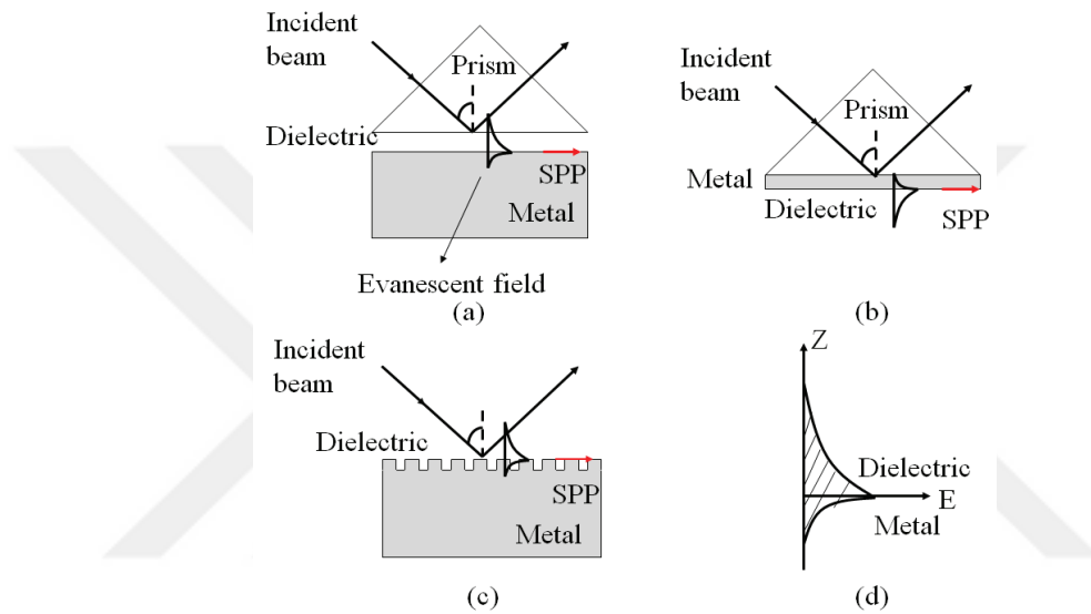
Figure 1.7. Surface plasmon resonance: (a) Otto configuration, (b) Kretschmann configuration, (c) a diffraction grating, and (d) an evanescent field at the interface. 5
