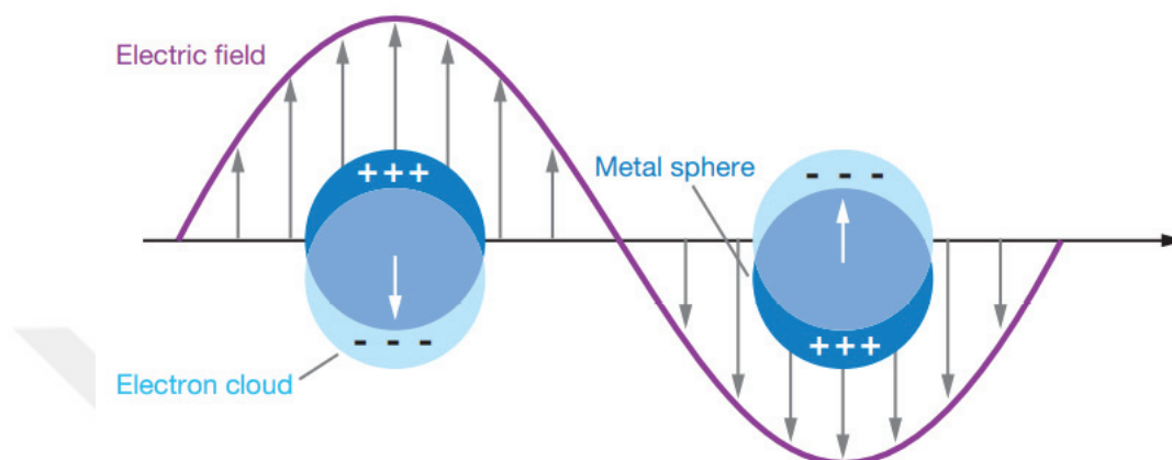
Figure 1.6. A localized surface plasmon polariton in a metal nanoparticle. 4
