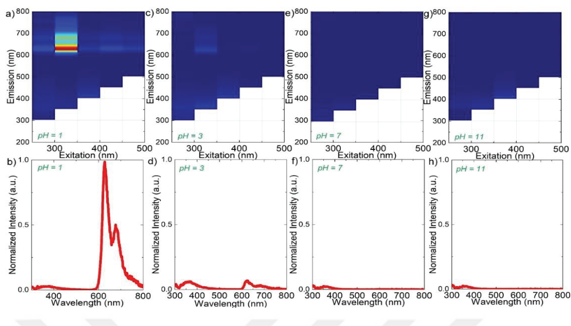
Figure 3.18. 2D excitation-emission topographical maps of CDs that are pH-dependent. (a-b) pH = 1, (c-d) pH = 3, (e-f) pH = 7, (g-h) pH = 11. The greatest PL emission intensity is shown by the red-colored region on the map, while the least PL emission intensity is indicated by the blue-colored region. 13 Reprinted with permission from Sarisozen, S.; Polat, N.; Mert Balci, F.; Guvenc, C. M.; Kocabas, C.; Yaglioglu, H. G.; Balci, S. Strong Coupling of Carbon Quantum Dots in Liquid Crystals. The Journal of Physical Chemistry Letters 2022, 3562–3570. https://doi.org/10.1021/acs.jpcllett.1c03937 . Copyright 2022 American Chemical Society.
