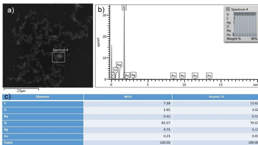
Figure 3.12. (a) Large area SEM image of the Ag-Au bimetallic decahedral shaped nanoparticles. (b) EDX spectrum of the selected area in SEM image. (c) Detected elements by the EDX analysis. The Ag-Au bimetallic decahedral shaped nanoparticles were dropped on a silicon wafer and thus silicon elements also appear in the spectrum. 12 Reprinted with permission from Balci, F. M.; Sarisozen, S.; Polat, N.; Guvenc, C. M.; Karadeniz, U.; Tertemiz, A.; Balci, S. Laser Assisted Synthesis of Anisotropic Metal Nanocrystals and Strong Light-Matter Coupling in Decahedral Bimetallic Nanocrystals. Nanoscale Advances 2021, 3 (6) https://doi.org/10.1039/d0na00829j . Copyright 2021 Royal Society of Chemistry.
