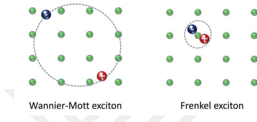
Figure 1.8. Schematic illustration of representative exciton models. 6
