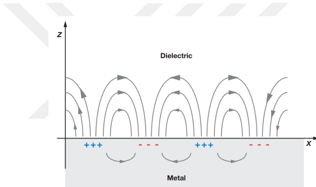
Figure 1.5. Surface plasmon polaritons (SPPs) on a metal-dielectric interface. 4
