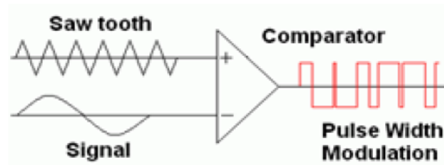
Figure 15 Principles of PWM generation (Hamza, et al., 2014).
