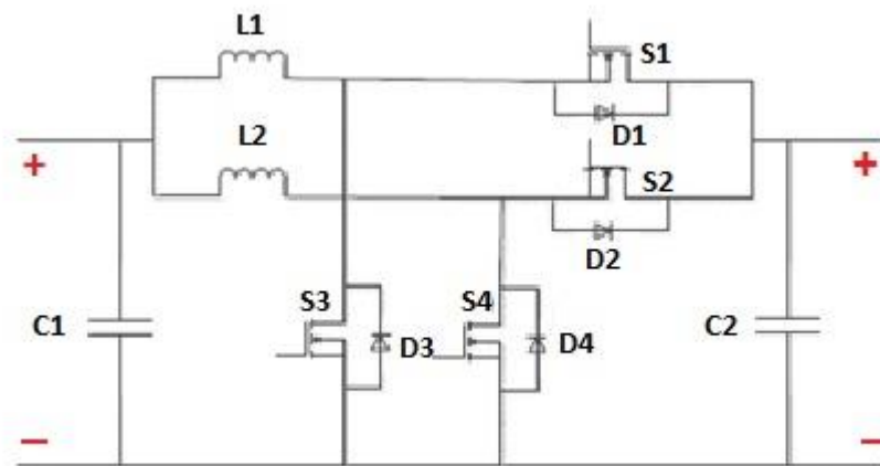
Figure 14 Parallel staggered DC / DC converter.
