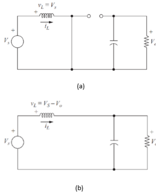
Figure 12 Switching sequence of the boost converter (Tutkun, 2021).
