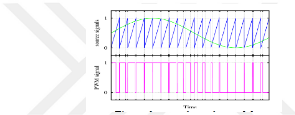
Figure 16 Wave form of PWM (Hamza, et al., 2014).
