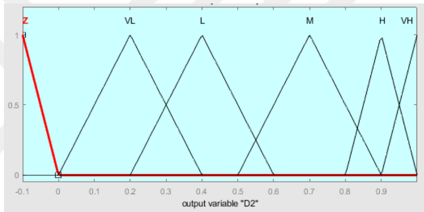
Figure 31 The membership function of D2.
