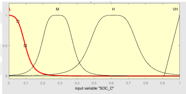
Figure 28 The membership function of SOC-C.
