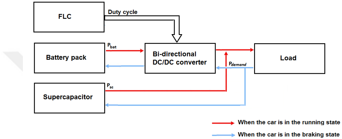
Figure 8 Intelligent energy storage system structure.
