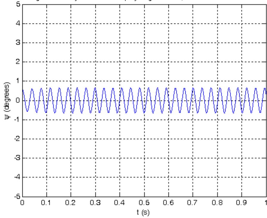
Figure 6.3: \psi for \psi_{fp}=0.5^\circ , v=50 m/s, c=100 Nm/rad/s and \psi(0)=0.01 .
