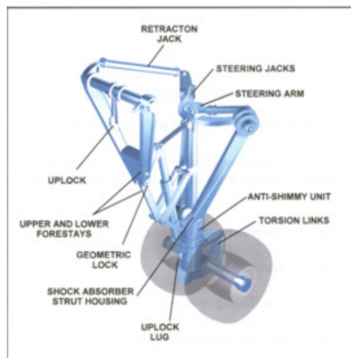
Figure 2.8: Schematic of a nose gear.
