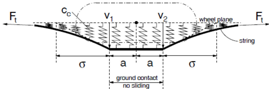
Figure 2.29: Stretched string model [1].
