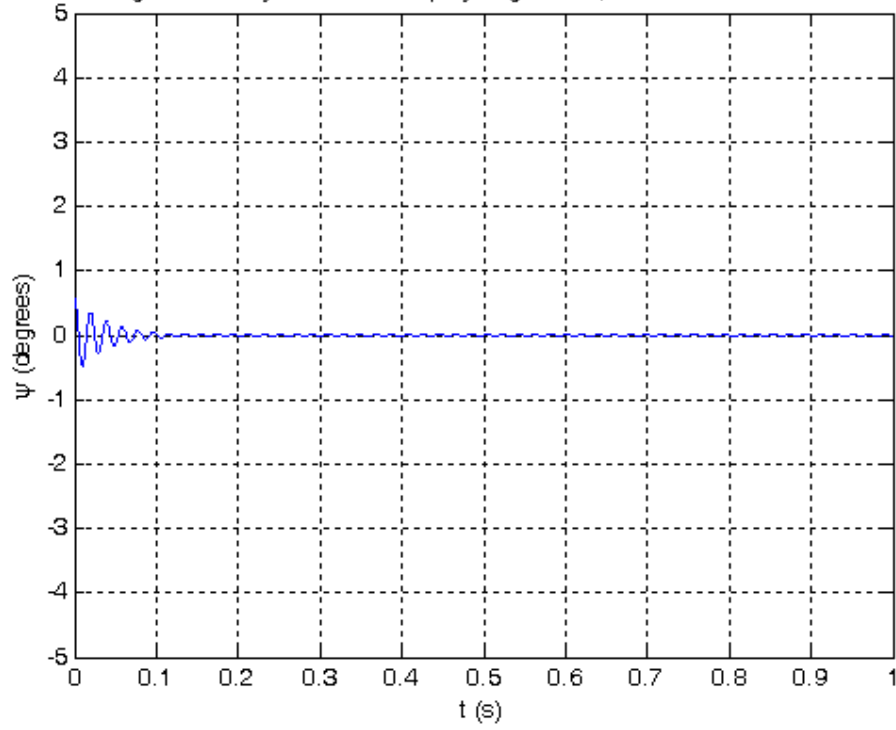
Figure 6.2: \psi for \psi_{fp}=0^\circ , v=50 m/s, c=100 Nm/rad/s and \psi(0)=0.01 .
