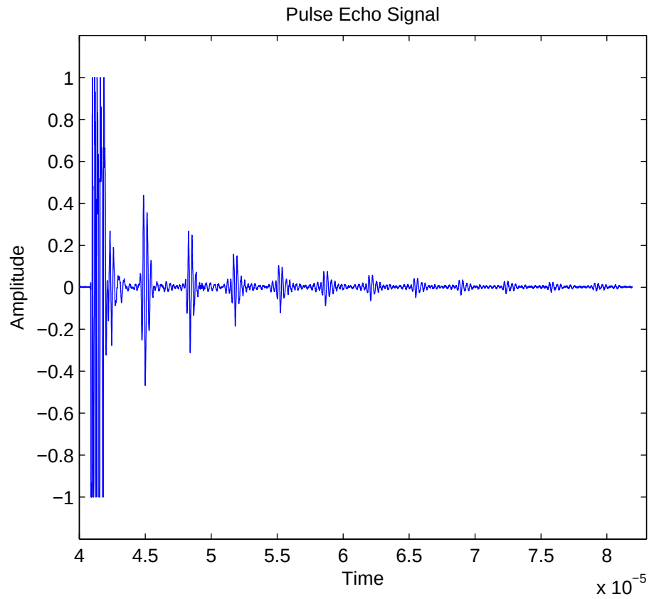
Figure 4.1. Pulse-Echo signal.
