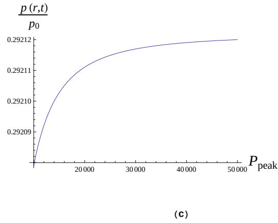
Figure 2.5. Normalized pressure wave \frac{p(r,t)}{p_0} vs. P_{peak} at t = 5 \mu s for (a) \frac{R}{\tau} = 1 (b) \frac{R}{\tau} = 5 (c) \frac{R}{\tau} = 10 where \frac{r}{R} = 2 and E = 0.2 mJ.
