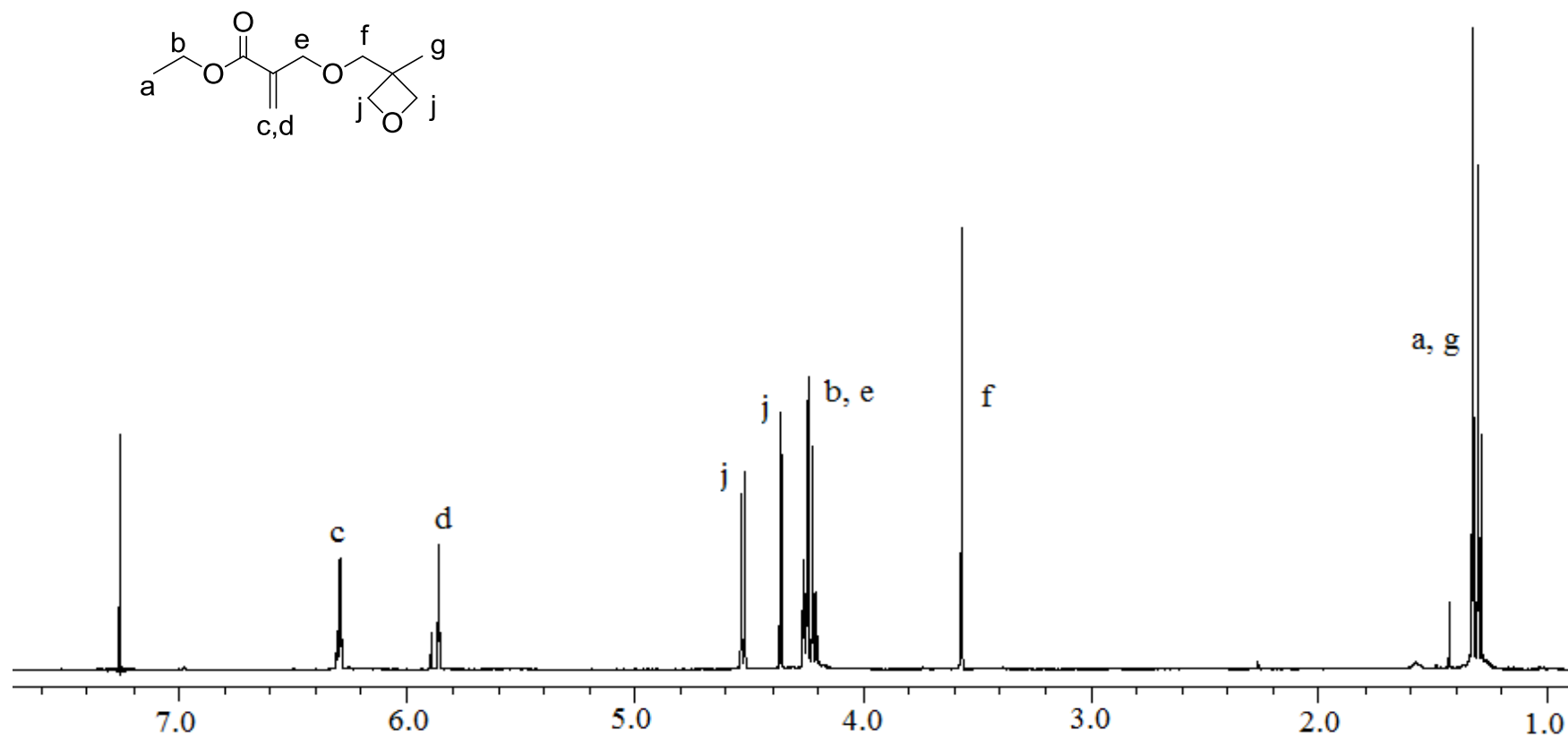
Figure A.7. ^1\text{H} -NMR spectra of monomer A5.
