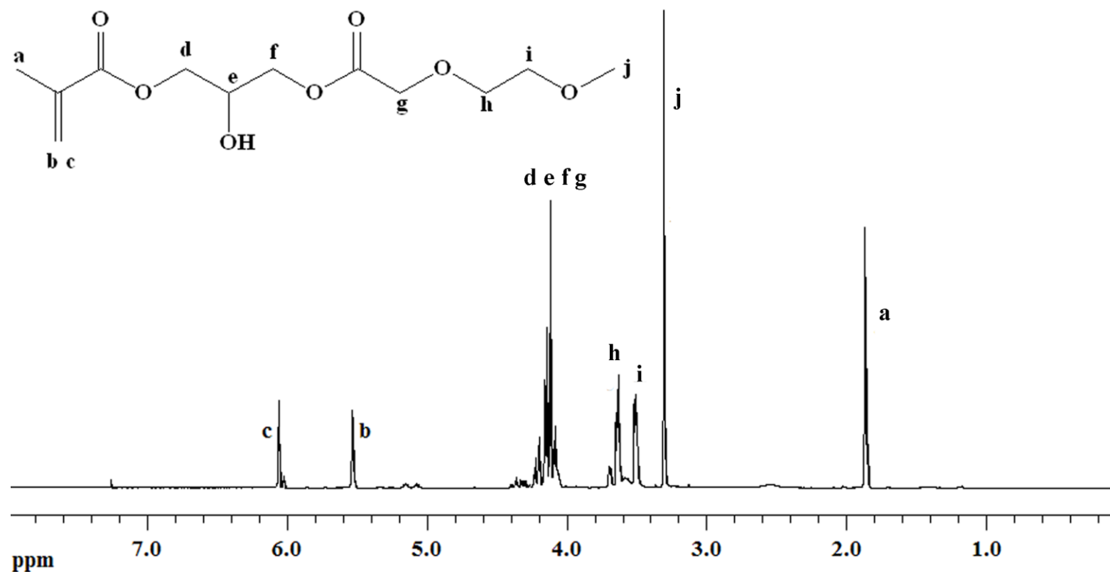
Figure 6.4. ^1\text{H} NMR spectra of monomer D1 .
