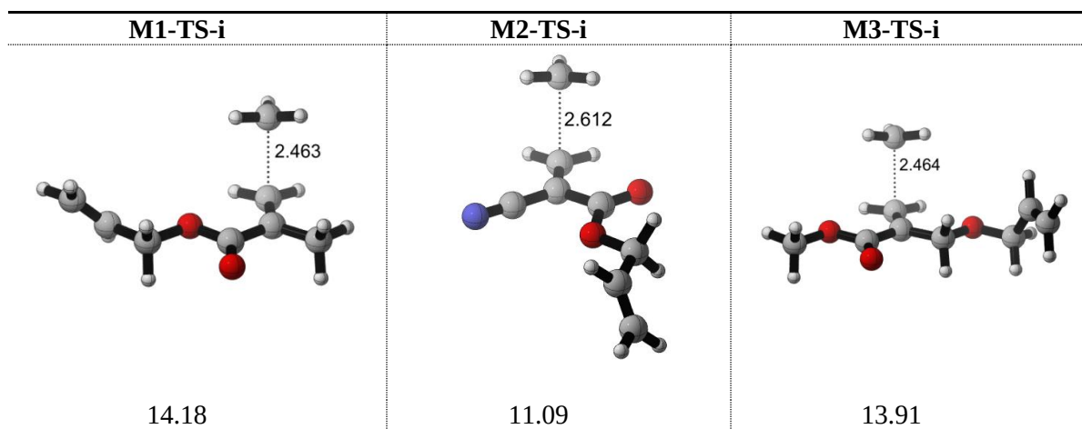
Figure 8.4. 3D structures and Gibbs free energies of activation ( \Delta G^\ddagger ) at 298 K for initiation (B3LYP/6-31+G*).
