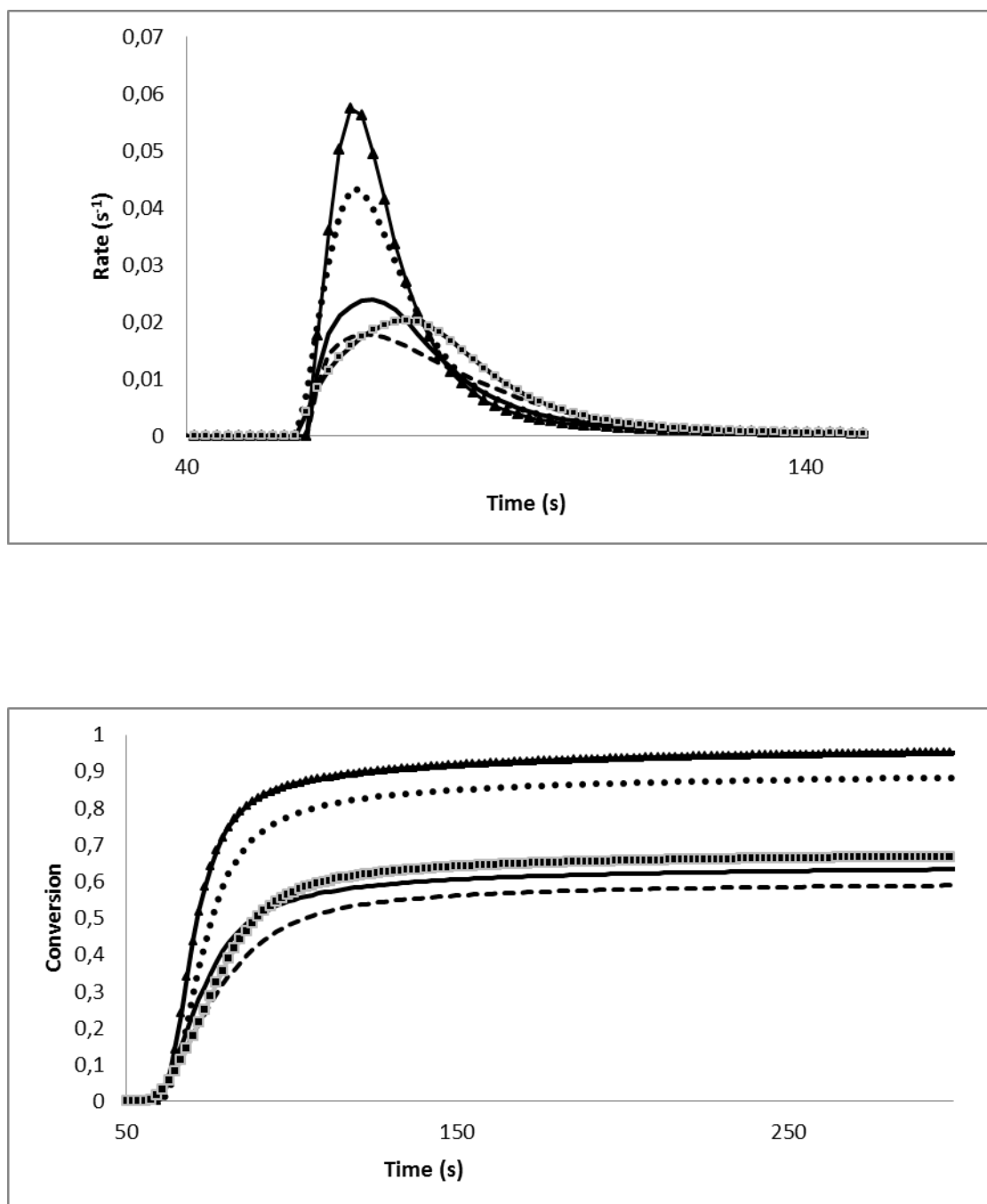
Figure 7.20. Rate-time and conversion-time plots for the photopolymerization of HDDA initiated by (-) BP/DMAEM; (--) P(E1-co-DMAEM) 1/1; ( \blacksquare ) E1/DMAEM, ( \bullet ) poly-E1/poly-DMAEM; ( \blacktriangle ) poly-E1/DMAEM. Photoinitiator and amine (N,N-dimethyl-p-toluidine) concentrations in monomer are 1 and 3 mol%.
