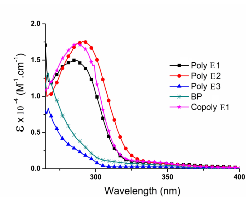
Figure 7.9. UV/Vis absorption spectra of polymeric photoinitiators and BP in DMF solution.
