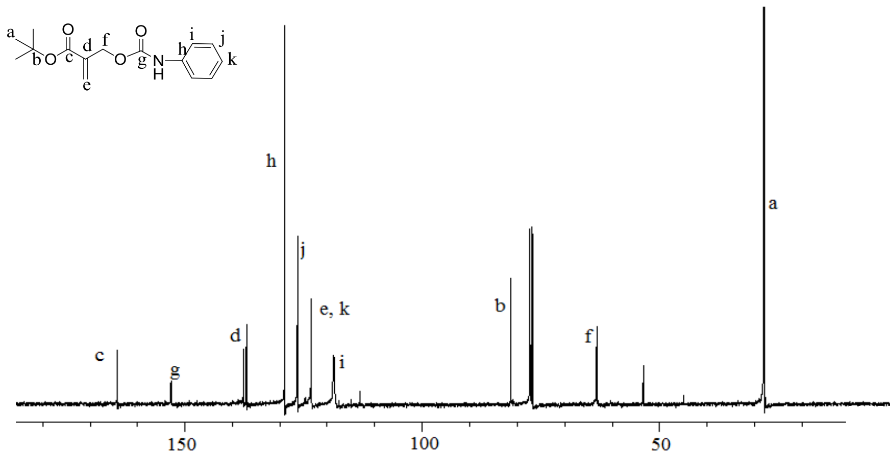
Figure A.18. ^{13}\text{C} -NMR spectra of monomer A14 .
