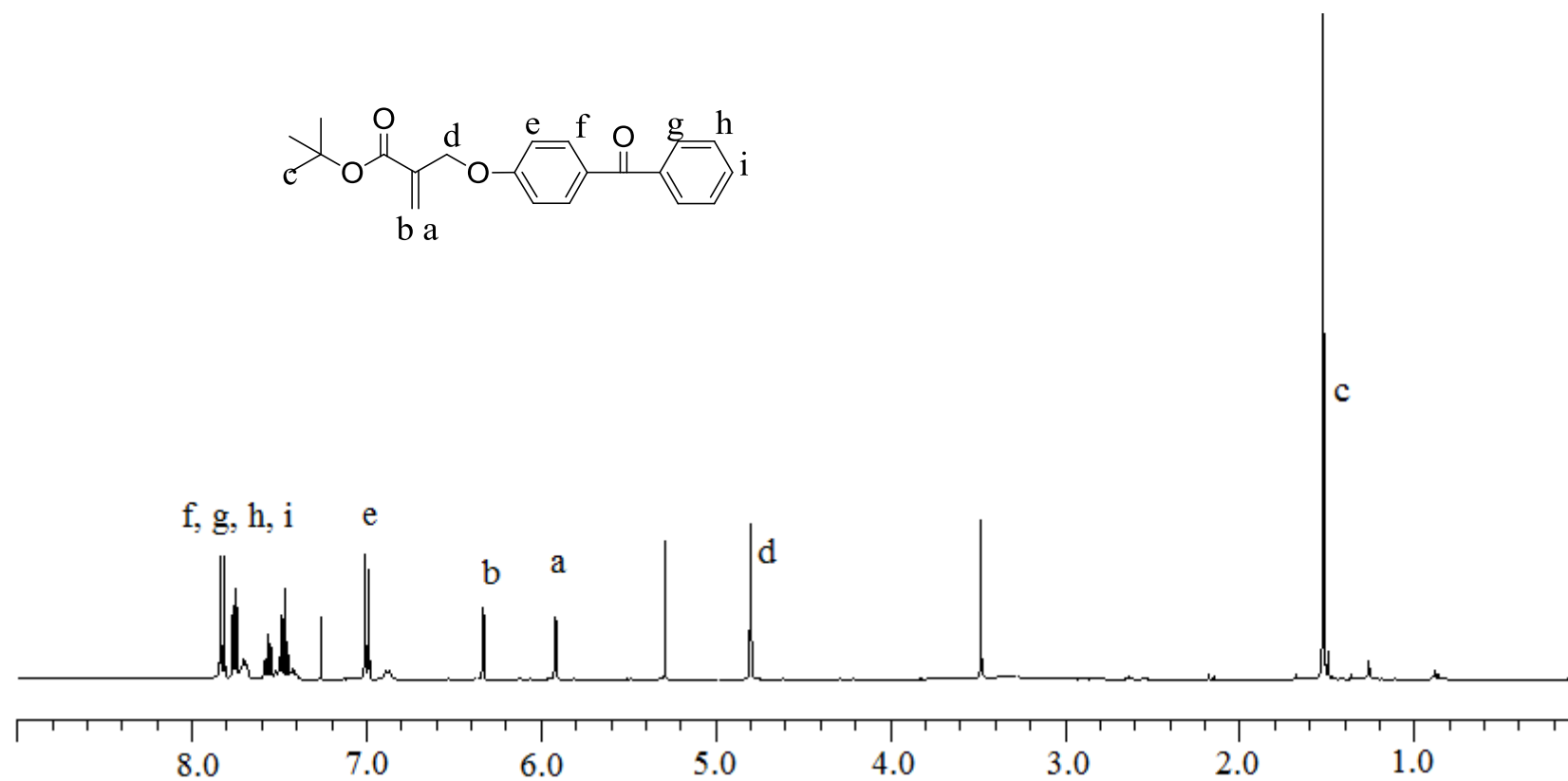
Figure A.41. ^1\text{H} -NMR spectra of monomer E1 .
