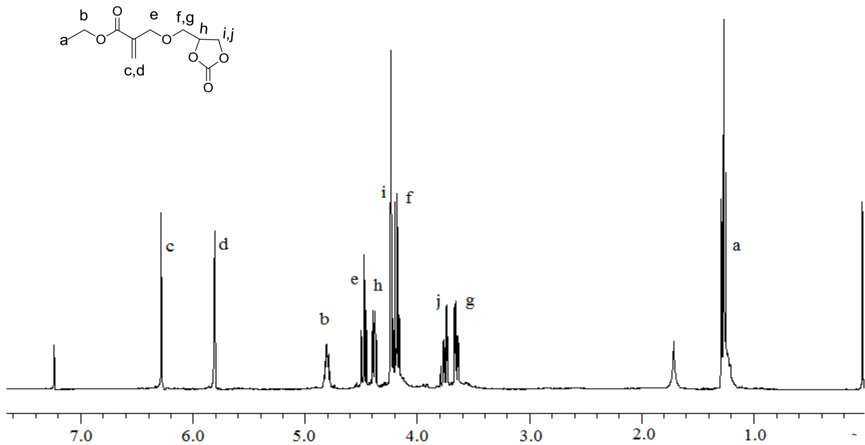
Figure A.9. ^1\text{H} -NMR spectra of monomer A6.
