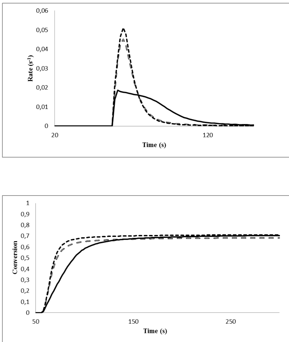
Figure 7.19 Rate-time and conversion-time plots for the photopolymerization of HDDA initiated by (-) BP; (--) poly-E1; (·) poly-E3. Photoinitiator and amine (N,N-dimethyl-p-toluidine) concentrations in monomer are 1 and 3 mol%.
