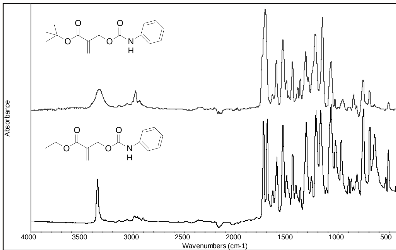
Figure 3.5. FTIR spectra of monomers A13 and A14 .
