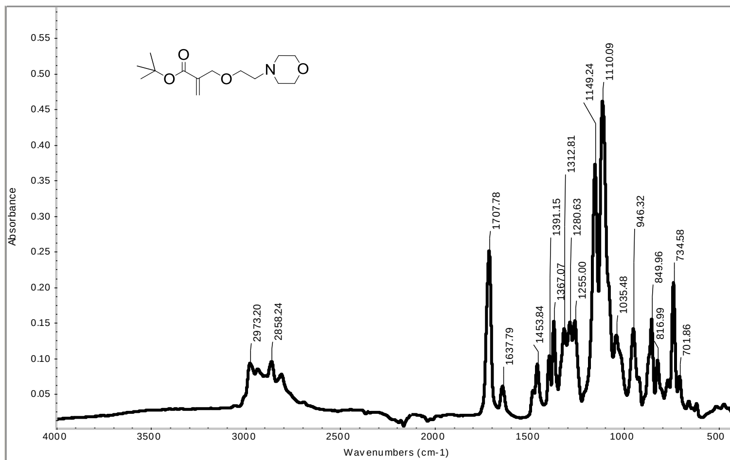
Figure A.24. FTIR spectra of monomer A2.
