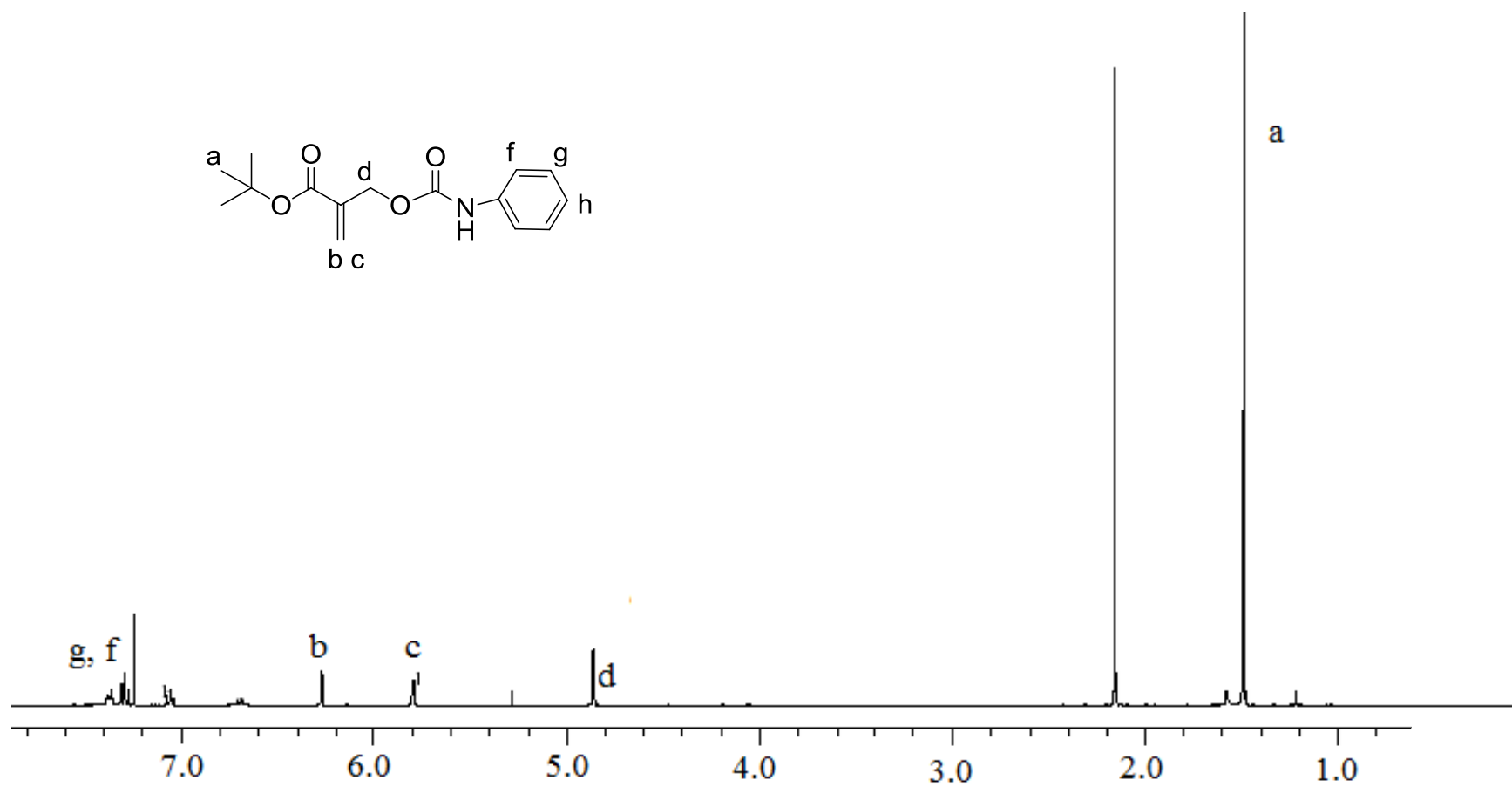
Figure A.17. ^1\text{H} -NMR spectra of monomer A14 .
