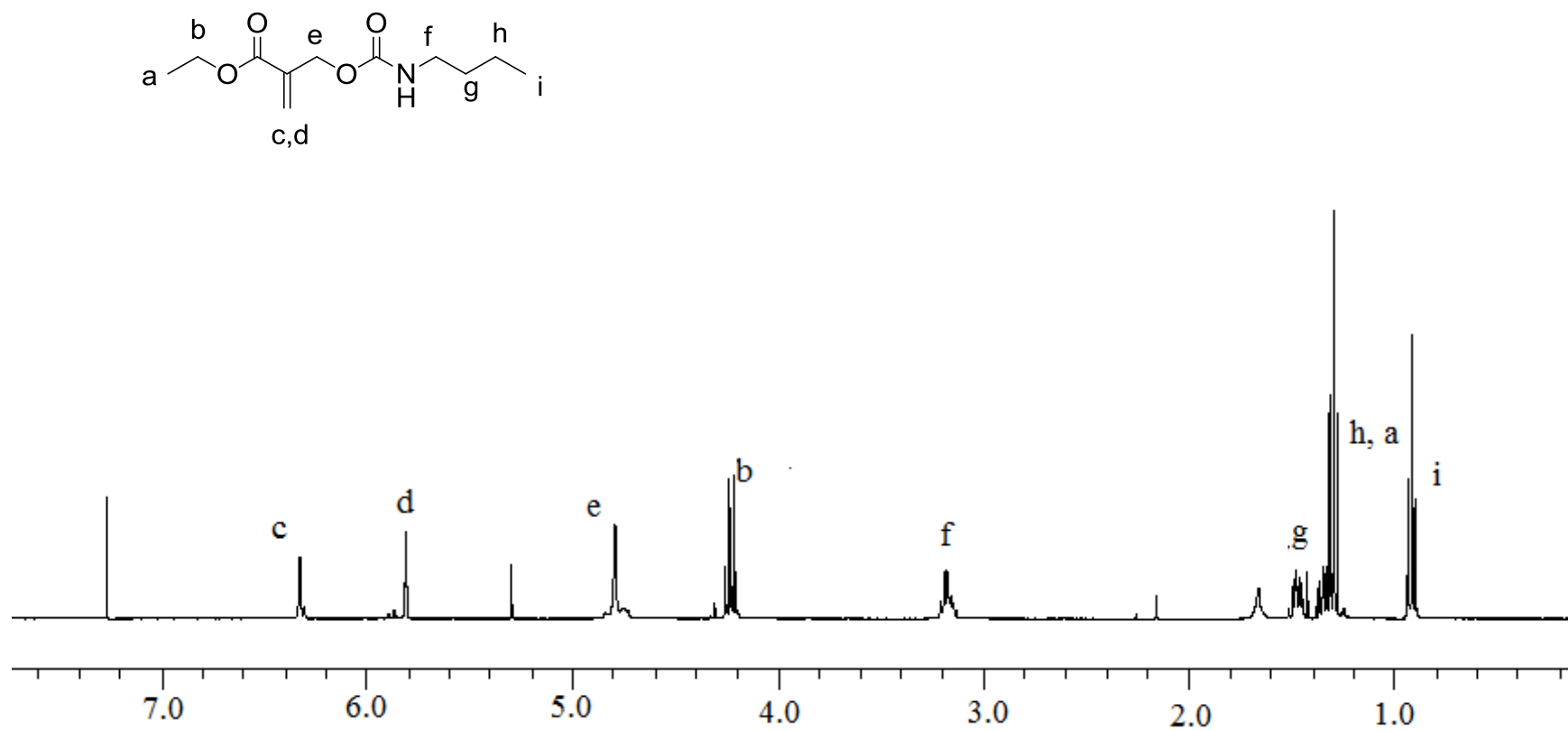
Figure A.19. ^1\text{H} -NMR spectra of monomer A15 .
