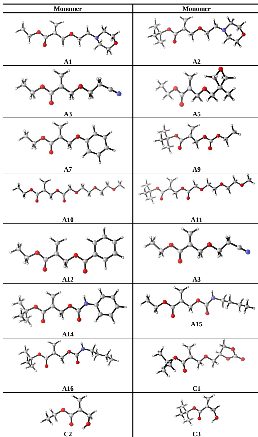
Figure 5.3. 3D structures of the most stable conformers of RHMA monomers.
