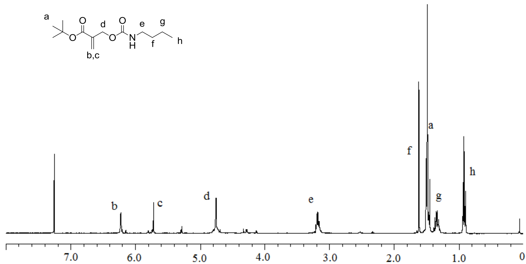
Figure A.21. ^1\text{H} -NMR spectra of monomer A16 .
