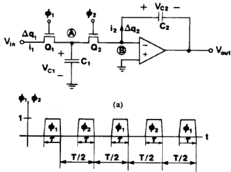
Figure 2.5. Switched capacitor integrator using shunt switched capacitor circuit (a) Circuit diagram (b) Clock waveforms [13].
