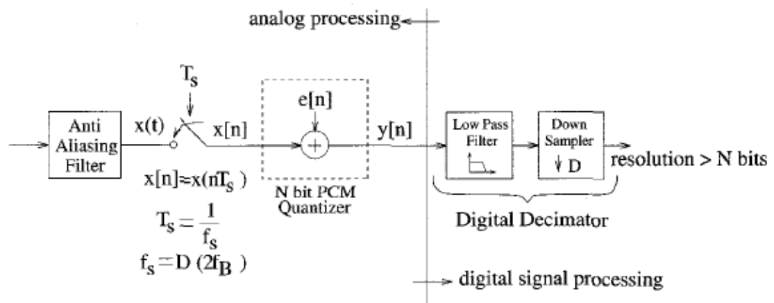
Figure 1.3. Block diagram of an oversampling converter [1].
