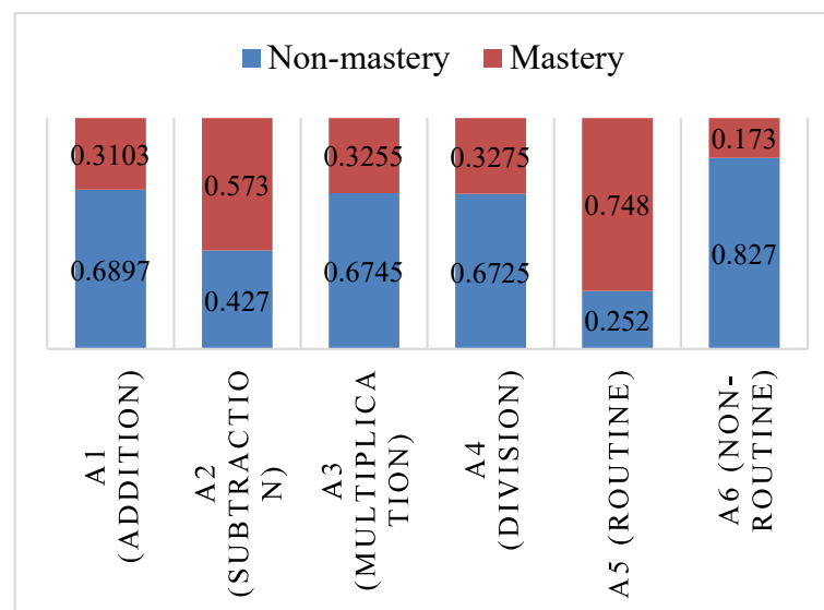
Figure 4.7. Attribute Probabilities.
