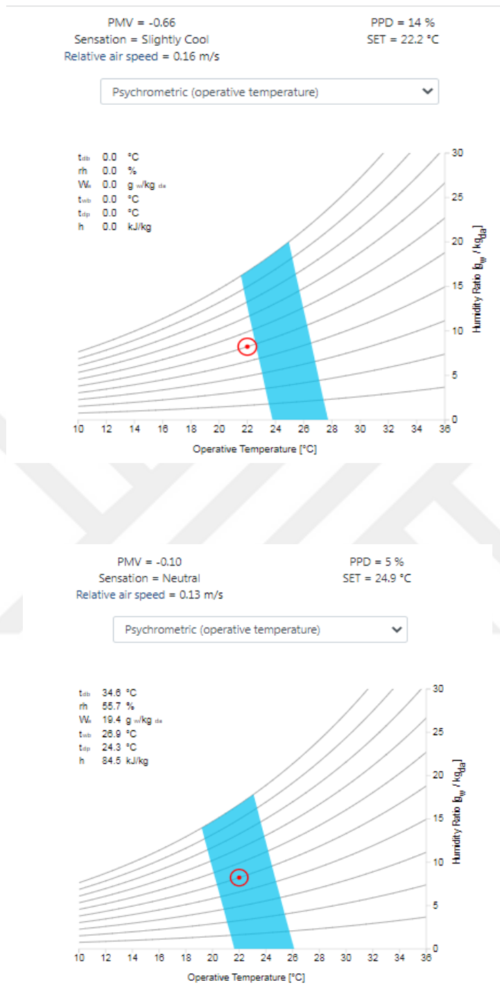
Figure 4.8 Graph of PMV a) 22 C for indoor temperature, 50% for humidity, and observed values for met and clo b) 22 C for indoor temperature, 50% for humidity, 1 Clo for the thermal insulation value for winter clothes
