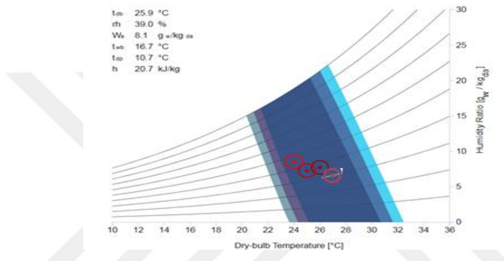
Figure 4.7 Comparative graph of thermal condition for 4 climate regions where self-report carried out.
