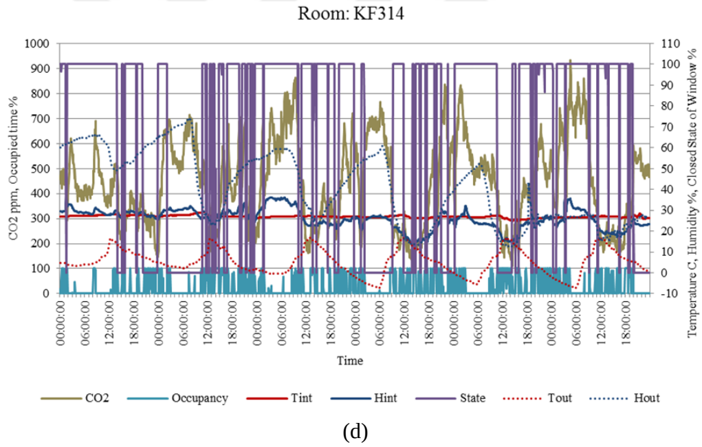
Figure P.5 recorded data in the rooms in the 5 th Climatic Region (Kars) (a, b, c, d)
