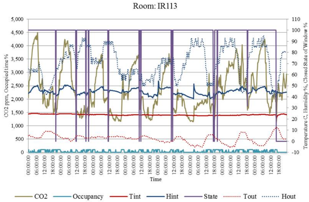
Figure P.2 recorded data in the rooms in the 1st Climatic Region (İzmir) (a, b, c, d)
