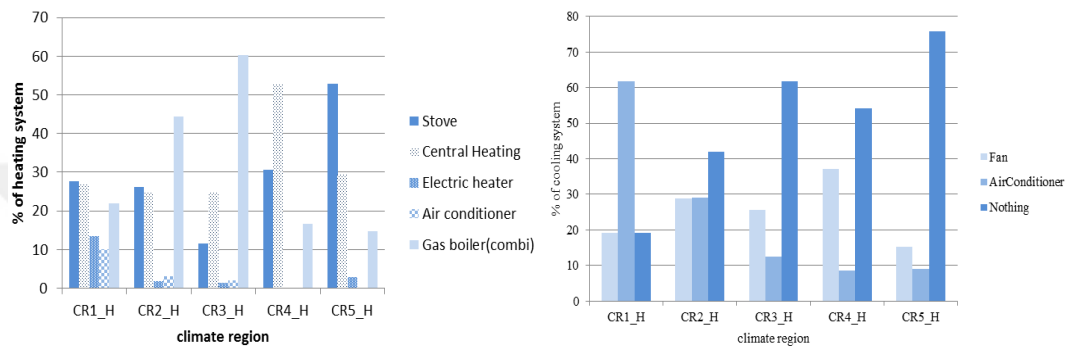
Figure 4.15 Relation of heating system (a) and cooling system (b) variables with climate regions.
